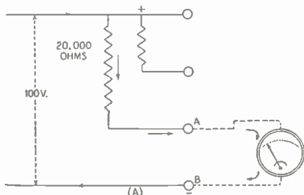
High-resistance Voltmeter
