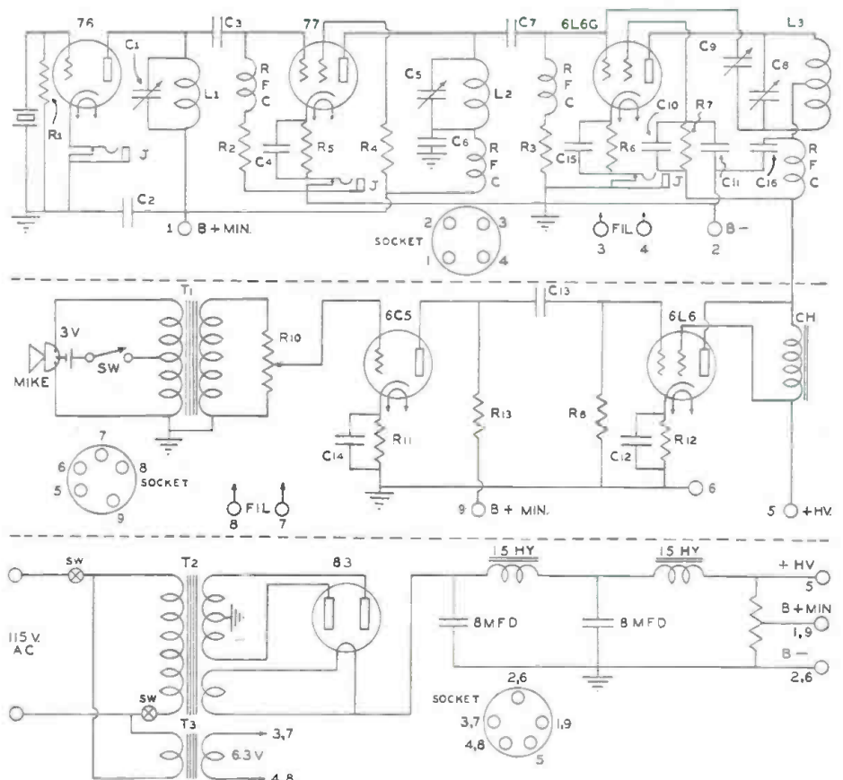
The complete transmitter circuit.
