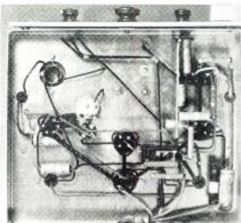
Underside the chassis. A cleanly wired receiver works better.
