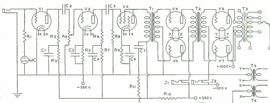
The circuit of the TZ-40 modulator.
