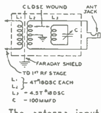
The antenna input.
