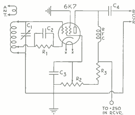
The One Tube Preselector. C1—35 mufd var. cond. C2—.0001 mfd mica cond. C3—.01 mfd mica cond. C4—.1 paper cond. 250 v. R1—500 ohm 1 watt res. R2—50,000 ohm pot. R3—25,000 ohm 2 watt res. RFC—Radio Frequency Ch.
