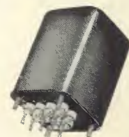
H-Type. Steel base cover deep-seal soldered into case. Terminals hermetically sealed. Ceramic bushings. Stud-mounted unit. Meets MIL-T-27 Specifications.
