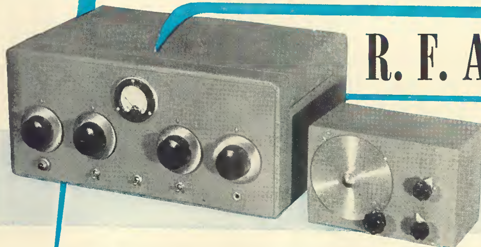
Front view of amplifier, shown with the exciter unit described by the author in last month's issue. The power supply for the amplifier is also used to operate the exciter section.
