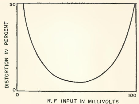
Fig. 2. Typical distortion vs input signal intensity of a receiver. Large amounts of audio distortion occur on either very weak or very strong signals.
