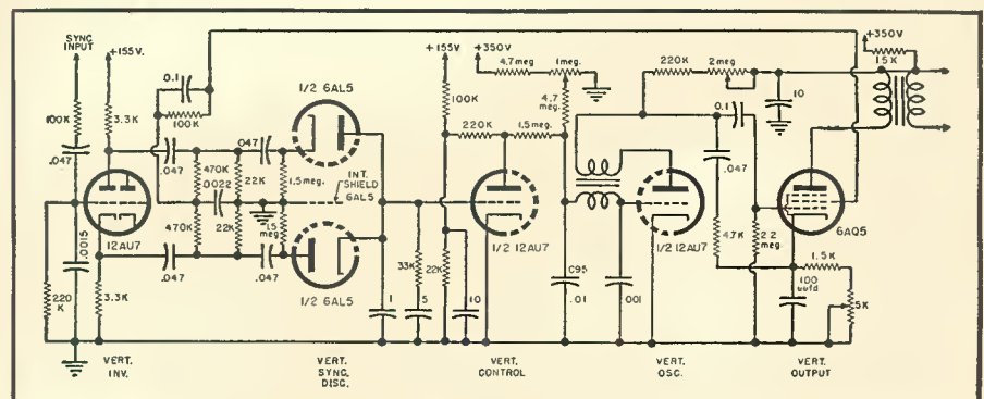
Fig. 2. The vertical deflection circuit used in the Radio Craftmen Model RC-100.
