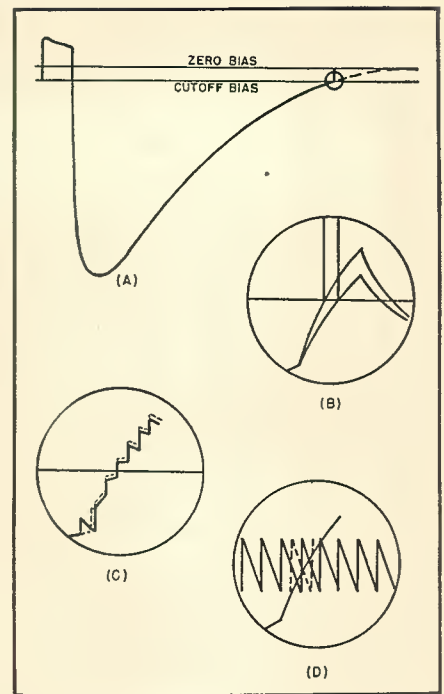
Fig. 1. Grid voltage waveforms in saw-tooth oscillators. See text for complete details.
