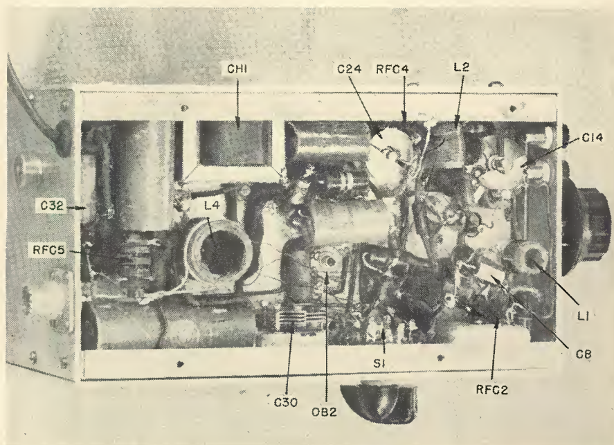
Underchassis view of variable frequency exciter. For parts identification, see Fig. 1.
