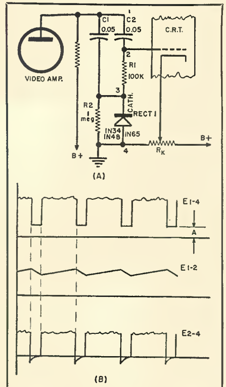
Fig. 3. Operation of a d.c. restorer. (B) Signal voltages which exist in (A). E_{1-4} represents the voltage across points 1 and 4 in the circuit, E_{1-2} across points 1 and 2, and E_{2-4} across points 2 and 4.
