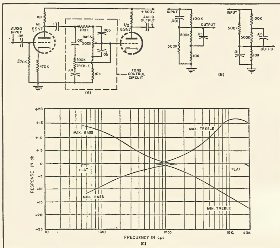
Fig. 4. (A) Variable tone control circuit, showing method of matching into amplifier circuit. (B) Simplified schematics showing operation of circuit at extreme control settings—maximum bass and maximum treble (left) and minimum bass and minimum treble (right). (C) Frequency response curves obtained with circuit shown in (A).
