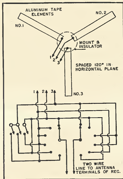
Fig. 1. An indoor "Direcronic" type antenna with aluminum tape adhesive elements and circuit of switching device.
