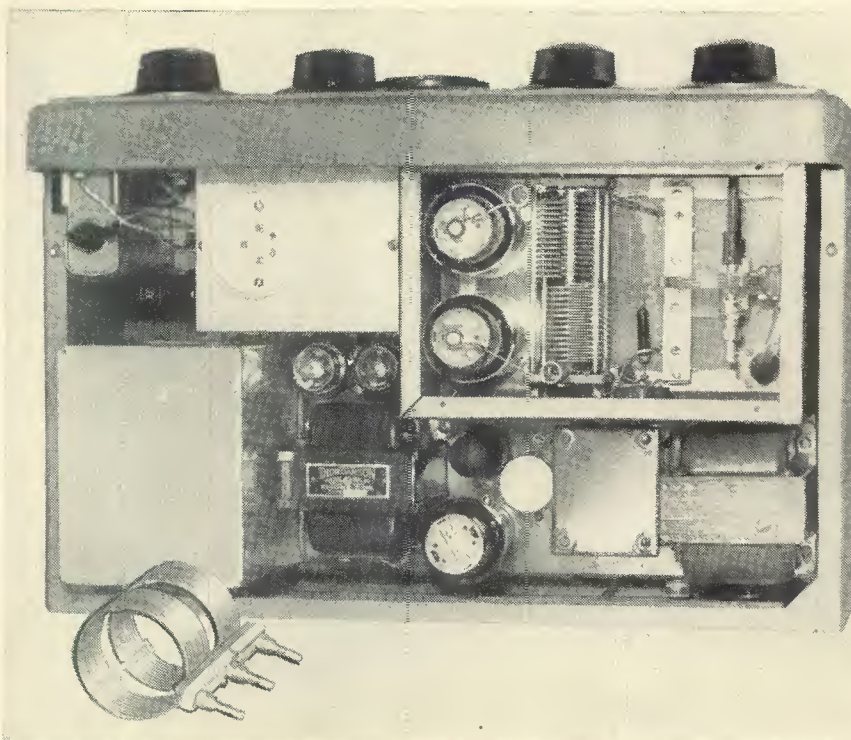
Top view. The copper screen wire shield has been removed to show interior of final amplifier compartment. The 6AG7 is mounted horizontally on small shield compartment.
