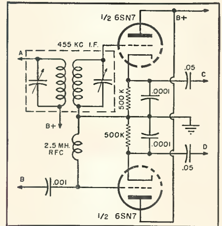
Fig. 3. Alternate form of second detector that may be used in the tuner circuit. Terminals A, B, C, and D connect to corresponding terminals shown in diagram of Fig. 4.
