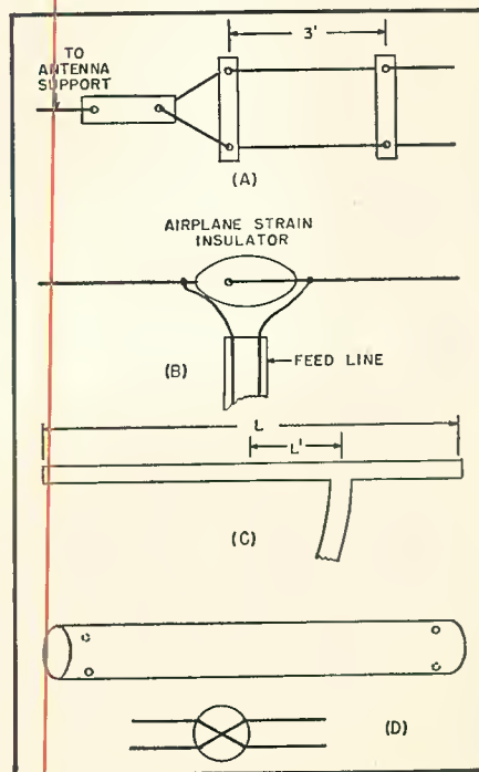
Fig. 3. Construction details. Note that (D) shows method of drilling plastic tubing so that tension of antenna will hold spacers.
