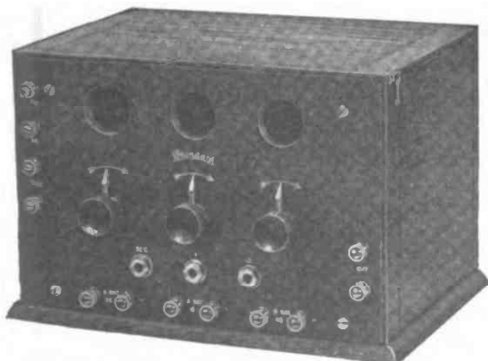
Detector and Two-Step Amplifier —Your choice of two types, Commercial or Amateur. The commercial type is assembled from the most costly, efficient units available. Radio Corporation UV-712 transformers and General Radio tube receptacles typify the quality thru-out. The Amateur type is an exact duplicate, except that transformers and sockets of high efficiency, but lower cost, are used.
