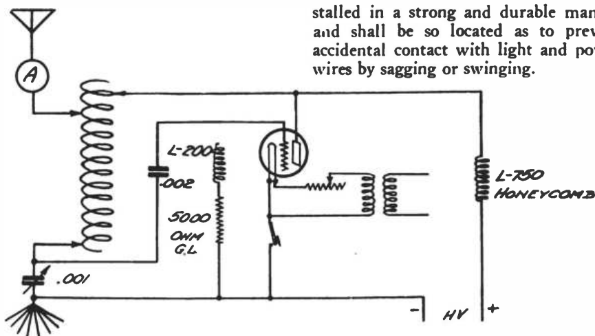
Circuit Diagram, 2LH
