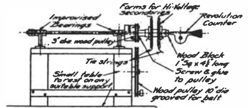
Fig. 7. Winding Rig
