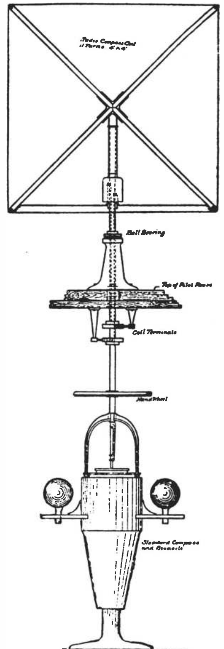
Fig. 5. Radio Compass as Installed on Tulip
