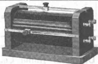
LAMB Tuning Coils. Two nickel sliders and rods; four nickel binding posts. Coil contains about ½ lb. No. 22 enameled Magnet Wire. Mounted in hard wood ends and base. Price $3.00. Code word, ACE.
