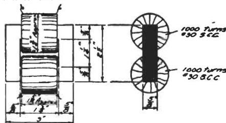
Fig. 10. Smoothing Choke
