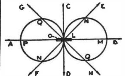
Fig. 4. Theoretical Directional Characteristics of Closed Coil Antenna
