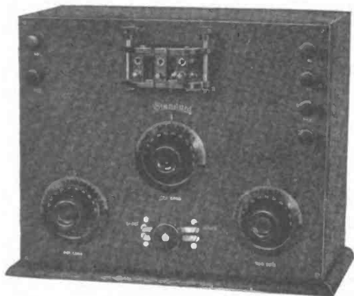
Multiple Wave Tuner —Here you obtain in a single instrument the equipment to receive all classes of signals on all known wave-lengths—150 to 25,000 meters. Minimum number of controls provide extreme simplicity of operation, yet the design renders the tuning especially sensitive and selective. Price, completely assembled, F. O. B. New York, $48.00
