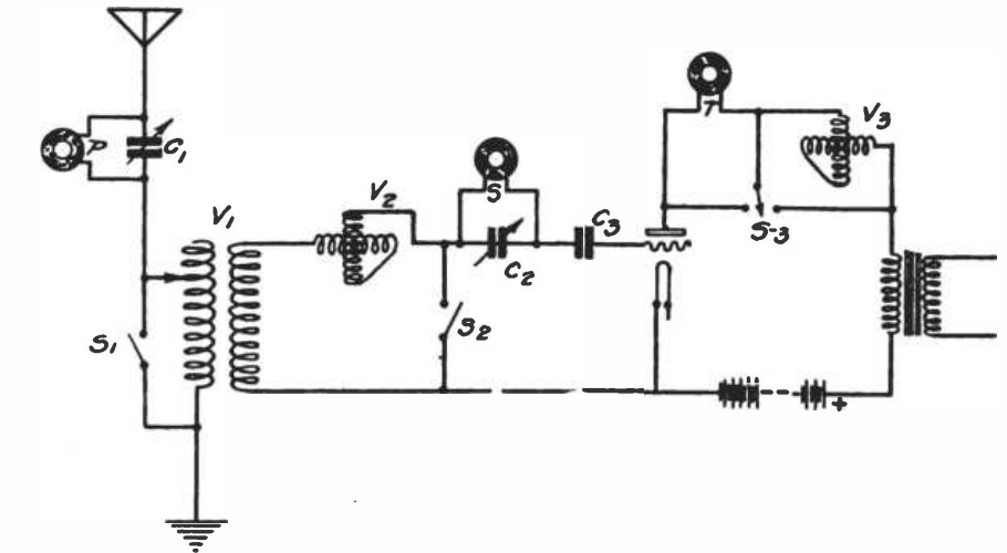
Diagram of All-Wave Receiver
