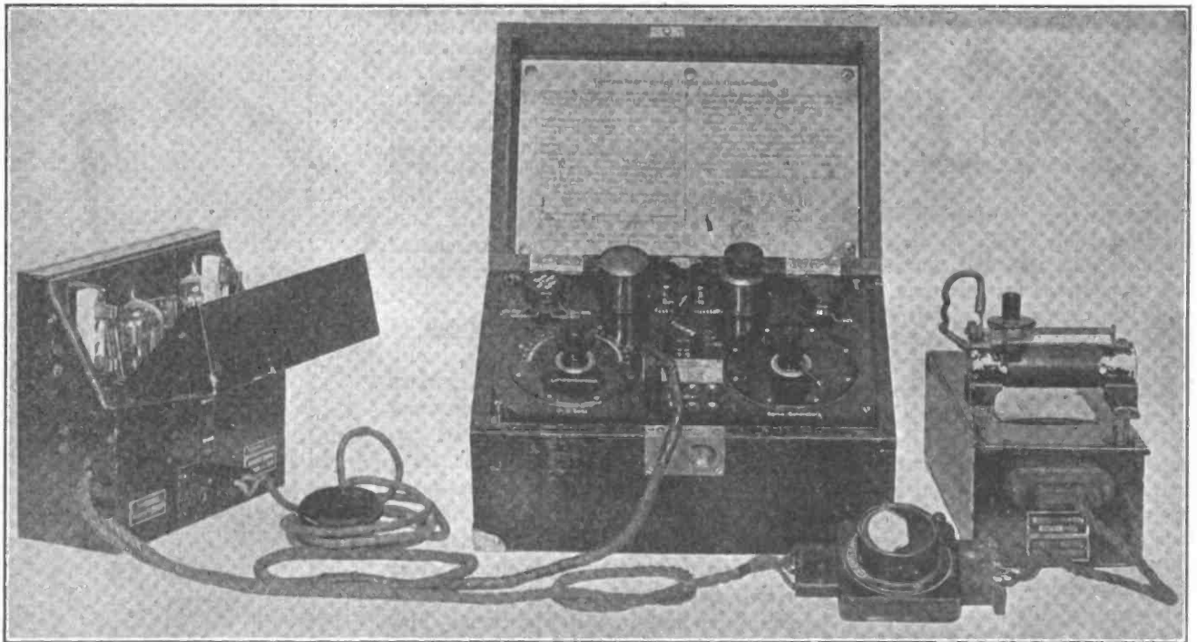
Fig. 1. Complete German Army Field Receiving Set
