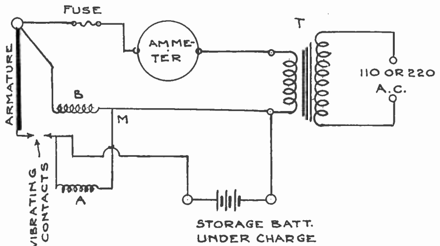
Fig. 12. Schematic Diagram of Vibrating Contact Charger
