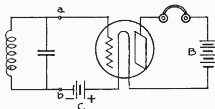
Fig. 4. Wiring Diagram of V. T. Detector Circuit With Grid Biasing Battery
