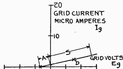
Fig. 3. Curve Showing Variation of Grid Current With Grid Voltage
