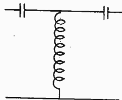
Fig. 2. High-Pass Filter, T Type
