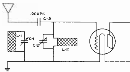
Fig. 1. Selector for Single-Circuit Set
