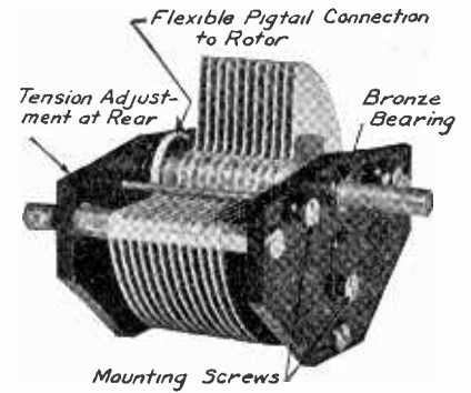
View Showing Typical Construction
