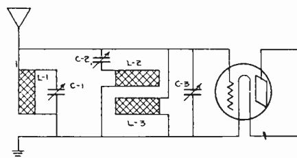
Fig. 2. Selector for Double-Circuit Set
