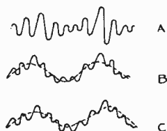
Fig. 7. Curves in Detector Circuit Using Grid Condenser
