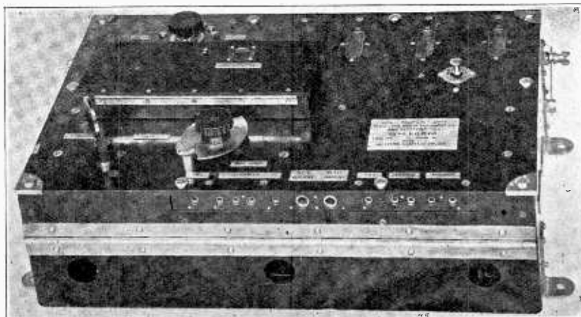
Airplane Radio Transmitting and Receiving Set Which Reported Air Positions by Voice Modulation for 100 Miles Distance
