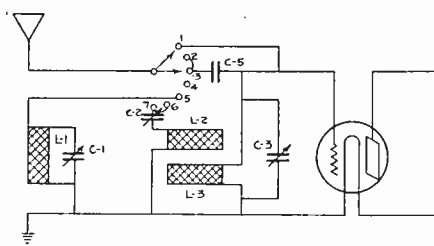
Fig. 3. Selector for Combination Set
