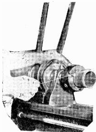
Fig. 1. How to Mount Tubing in Lathe
