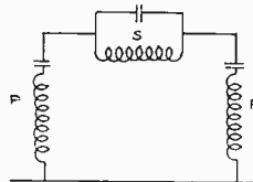
Fig. 4. High and Low-Pass Filter
