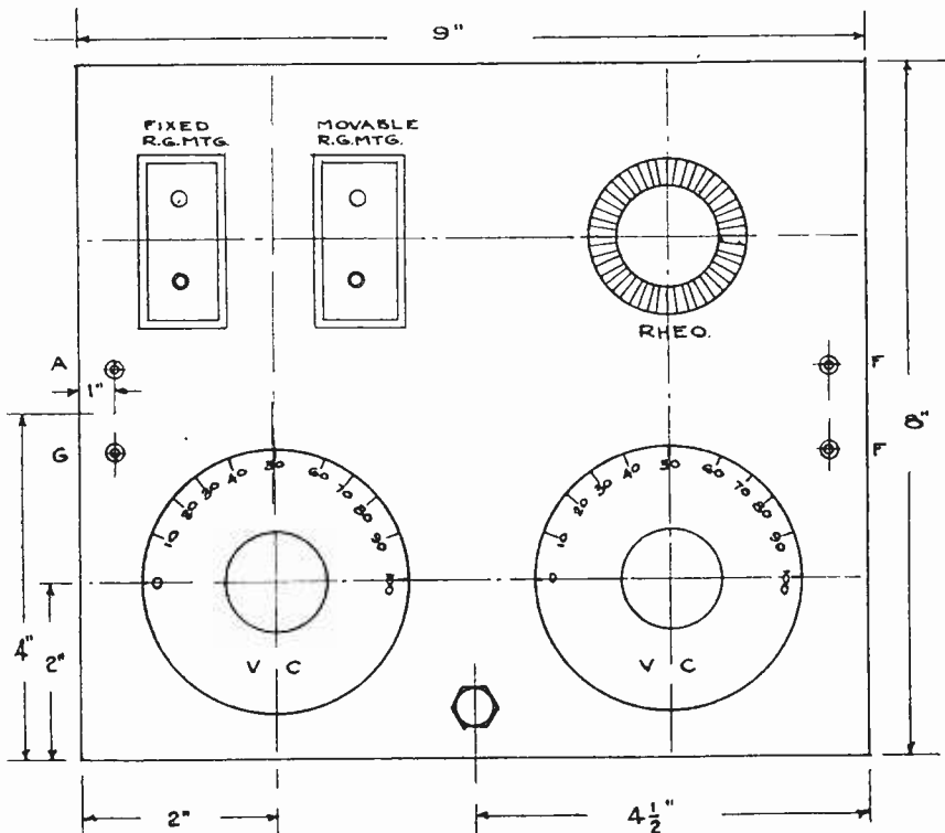
Fig. 2. Panel Layout
