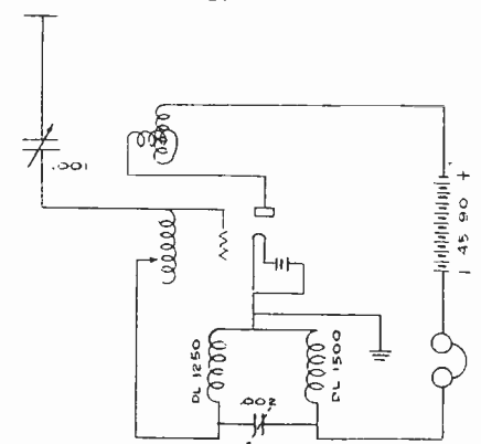
Fig. 5. Adaptation to Single-Tube "Super"
