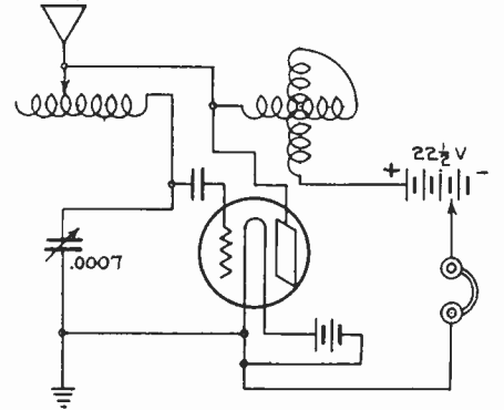
Fig. 3. Adaptation to Gibbons' Circuit
