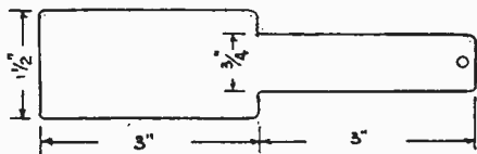
Fig. 2. Dimensions of Plates for Chemical Rectifier
