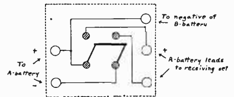
Diagram of Connections
