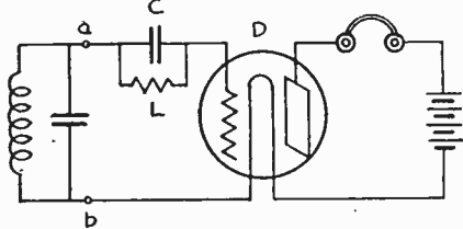
Fig. 6. Detector Circuit With Grid Condenser
