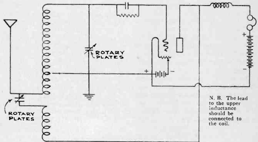
Hook-up for "Ham Special" Receiver
