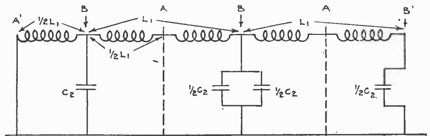
Fig. 6. 2\frac{1}{2} Section Filter, T Type from Left to Right, \pi Type from Right to Left
