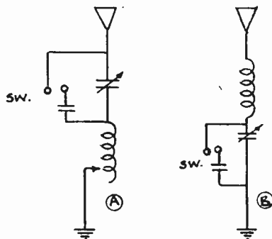
Fig. 3. Use of Shunt Condenser
