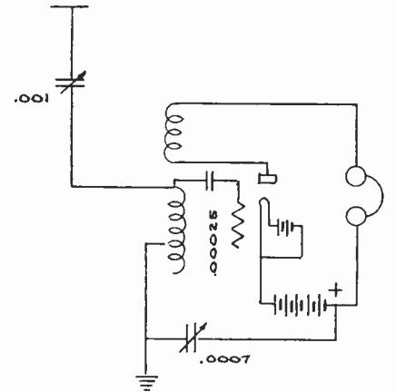
Fig. 4. Adaptation to Tickler Feed Back Circuit
