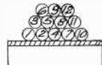
Fig. 5. Three-Banked Winding
