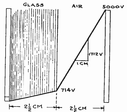
Fig. 2. Voltage Distribution Through Non-Homogeneous Insulation
