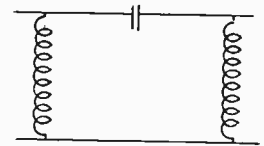
Fig. 3. High-Pass Filter, \pi Type
