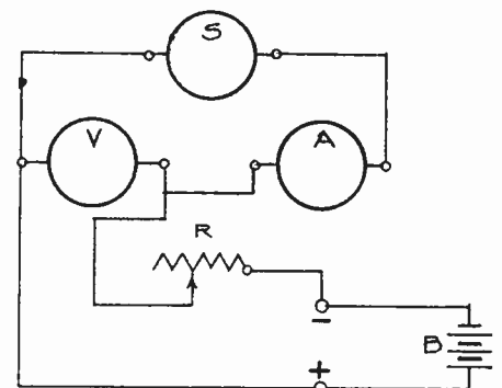
Fig. 3. Hook-up
