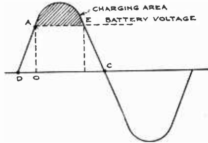
Fig. 10. Diagram of Charging Cycle
