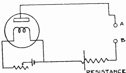
Fig. 2. Gas Filled Tube Rectifier
