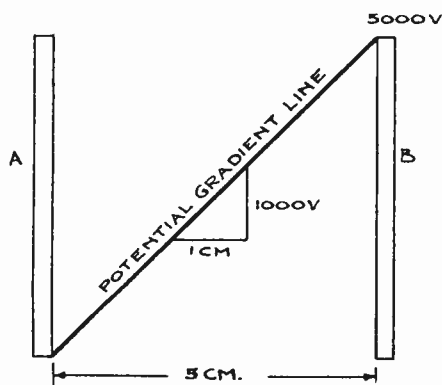
Fig. 1. Voltage Distribution Through Homogeneous Insulation
