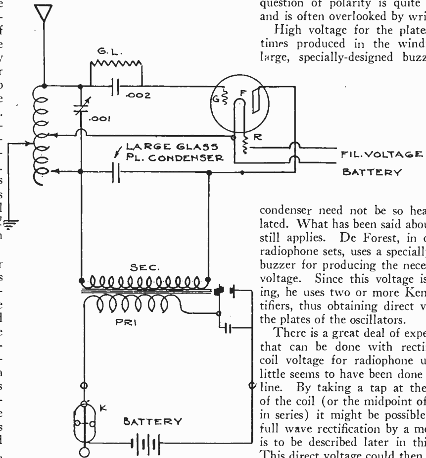
Fig. 1. Circuit Diagram for C. W. Transmitter with Spark Coil
