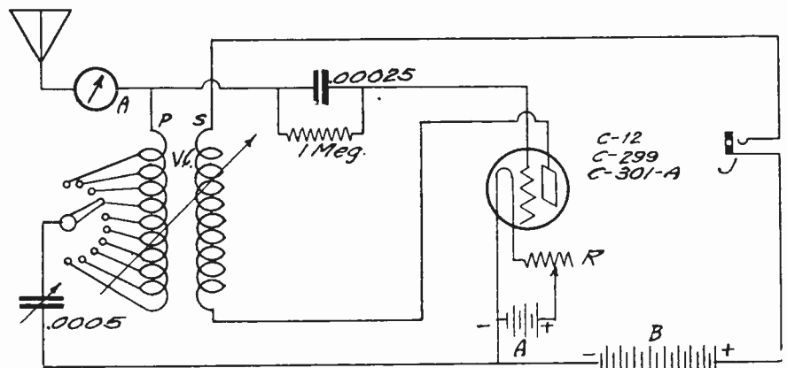
Fig. 1. Hook-up for Groundless Receiver
