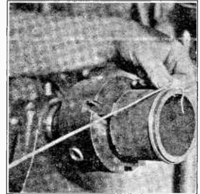
Fig. 3. Starting the Bank Winding
