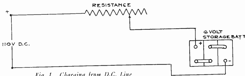
Fig. 1. Charging from D.C. Line
