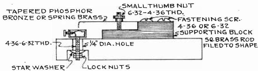
Detector Stand
