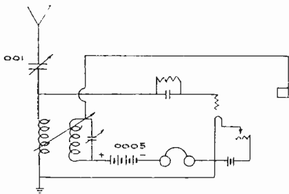
Fig. 1. Hook-up for One-Tube Receiver
