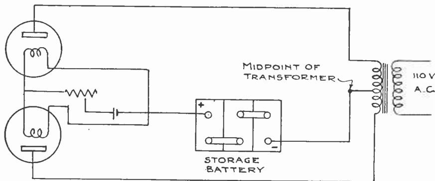
Fig. 6. Full Wave Rectification
