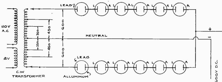
Fig. 3. Connections for Electrolytic Rectifier
