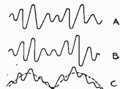
Fig. 5. Curves in Detector Circuit Using Grid Bias; A , Grid Voltage; B , Resultant Plate Current; C , Rectified Plate Current.
