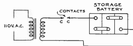
Fig. 9. Elementary Circuit for Vibrating Contact Charger
