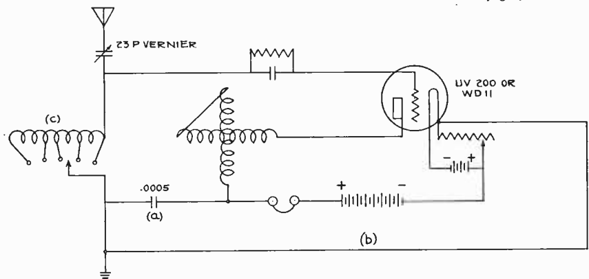
Fig. 1. Modified Circuit
