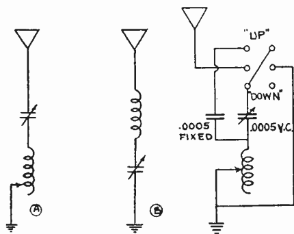
Fig. 1. Condenser Position in Primary Circuit
