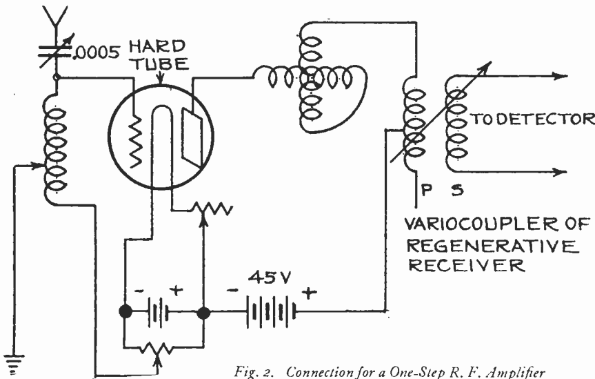
Fig. 2. Connection for a One-Step R. F. Amplifier
