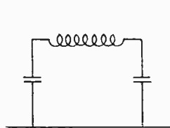
Fig. 1. Low-Pass Filter
