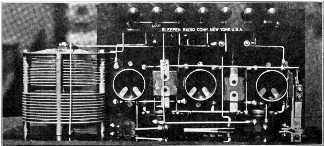
Fig. 2. Interior View of Monotrol
