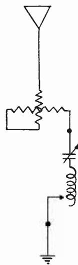
Fig. 4. Circuit with Variometer
