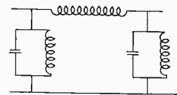
Fig. 5. Band Pass Filter
