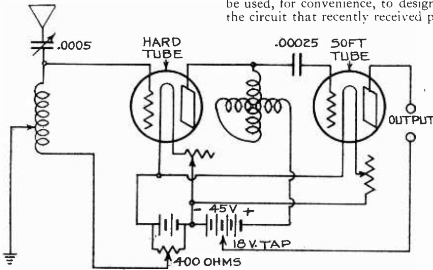
Fig. 1. Connection for a One-Step R. F. Amplifier
