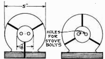
Fig. 2. Double Spiderweb Forms
