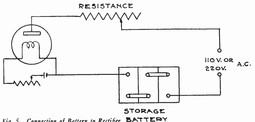
Fig. 5. Connection of Battery to Rectifier
