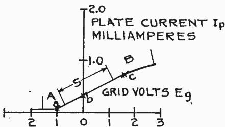
Fig. 2. Curve Showing Variation of Plate Current With Grid Voltage
