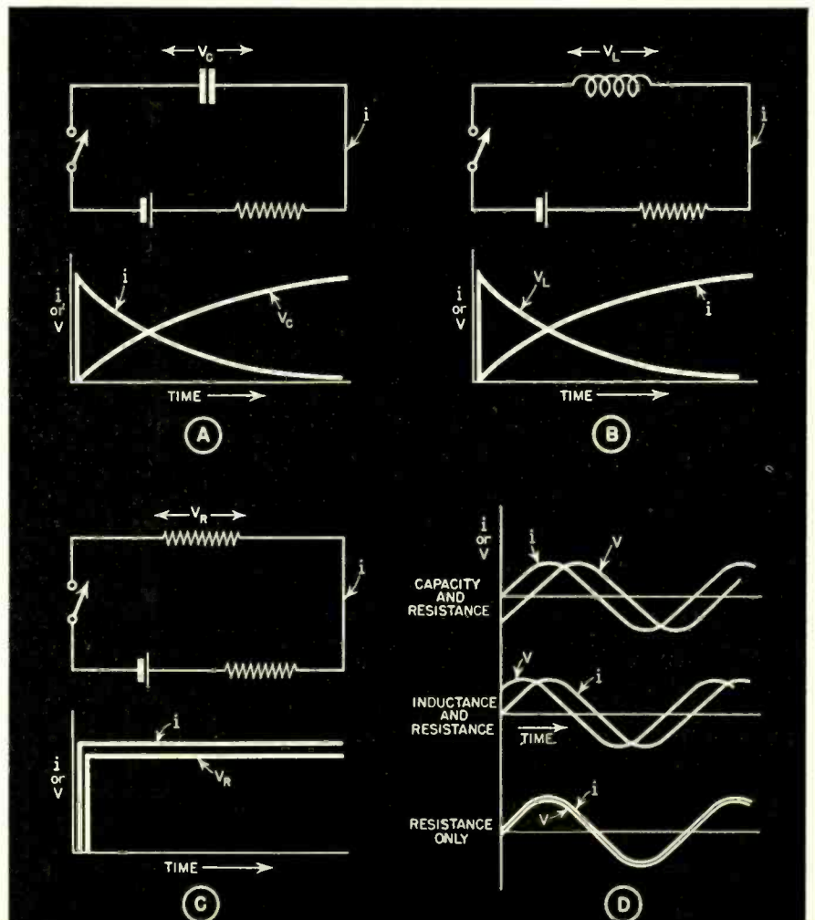
Fig. 1. Phase difference between current and voltage for inductance, capacitance and resistance.
