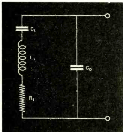
Fig. 10. Equivalent circuit of plated type of crystal unit
