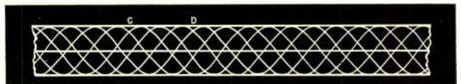
Fig. 5. Electric field in a coaxial line with unity standing wave ratio
