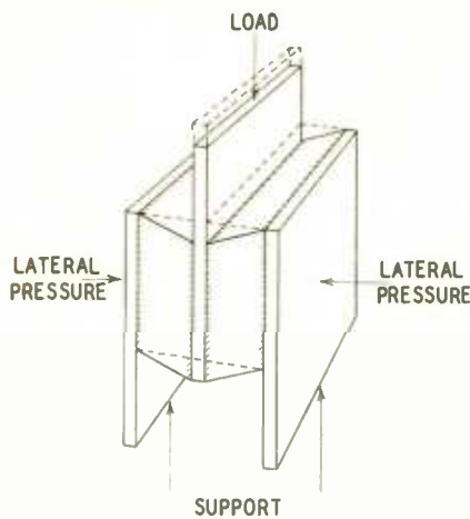
Fig. 14. Simple shear sandwich
