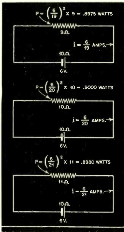
Fig. 2. Illustration of impedance matching to obtain maximum energy transfer from source to load
