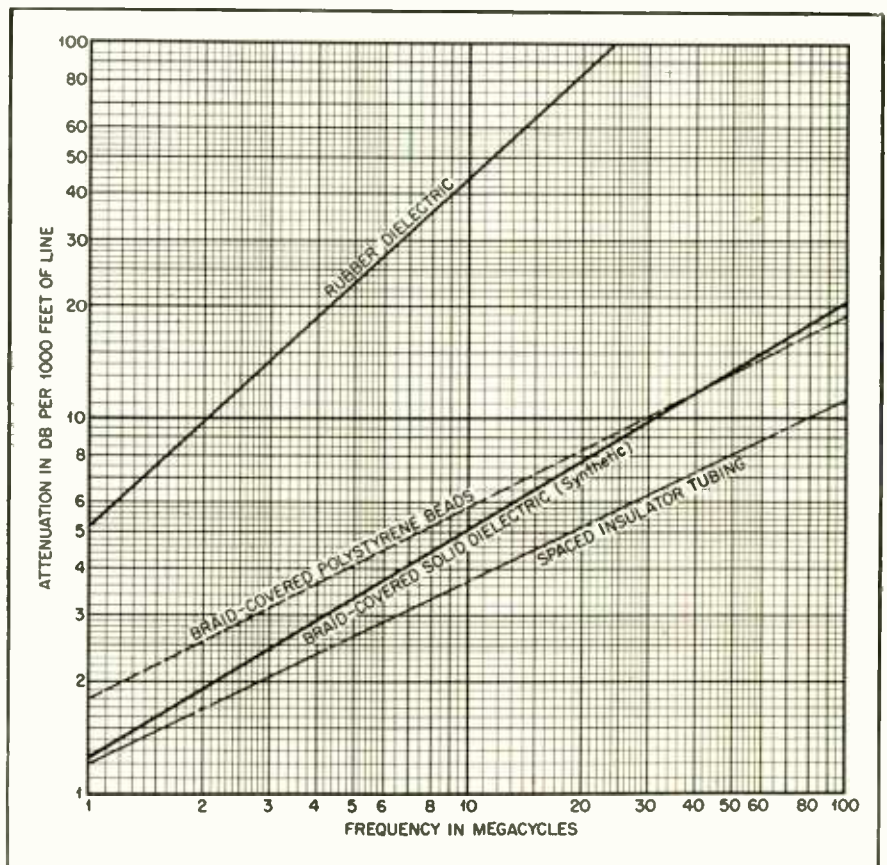
Fig. 1. Attenuation of typical coaxial cables
