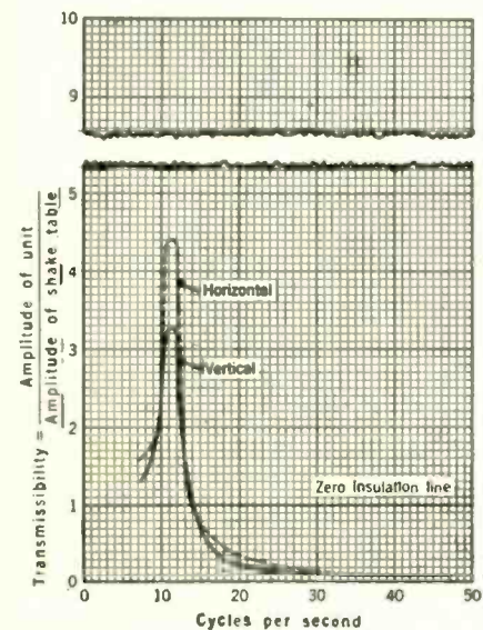
Fig. 5. Transmissibility curve with resilient supports in horizontal plane at center of gravity
