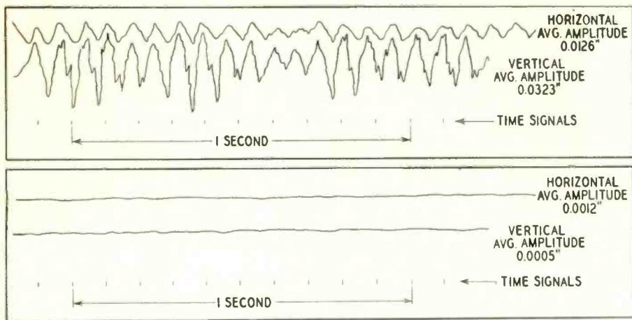
Fig. 4. Photographic record of actual results accomplished in vibration insulation using rubber mountings. Upper record shows vibration amplitude without rubber mountings
