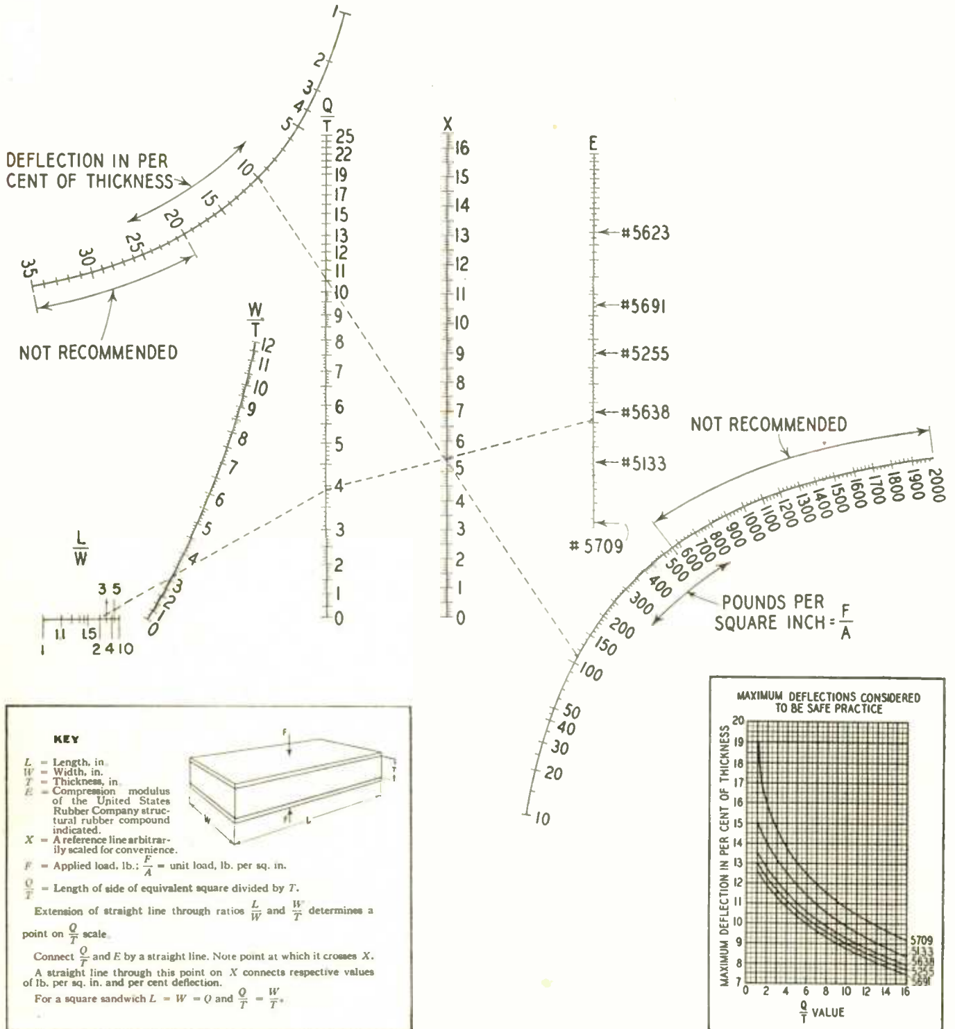
Fig. 13. Nomograph for determining deflections of rubber adhered between parallel metal plates and stressed in compression
