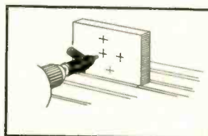
ON A HORIZONTAL MILL—the ability to center a layout, edge block or rotary table plug while spindle is running. Permits quick and easy set-up for high precision work.
