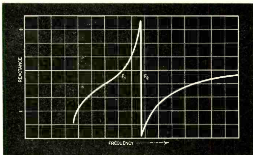
Fig. 9. Typical reactance curve of crystal oscillator plate
