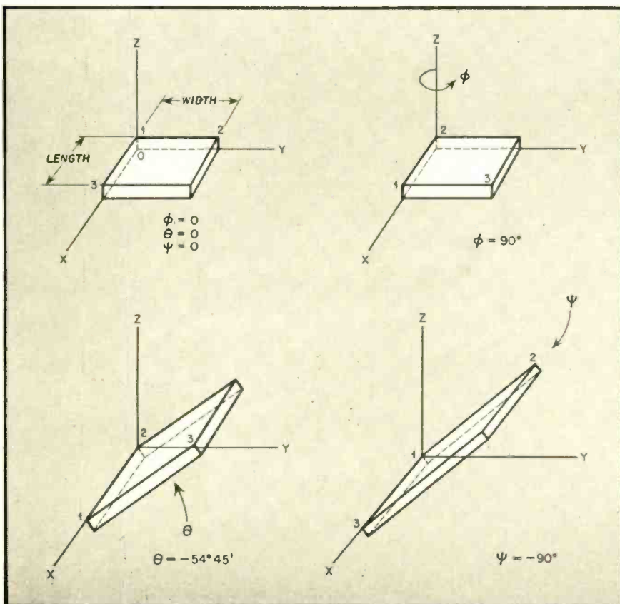
Fig. 13. Orientation for AT-cut crystal (IRE nomenclature). For all orientations viewing from 1 to 0 and 2 to 1 counter-clockwise is positive
