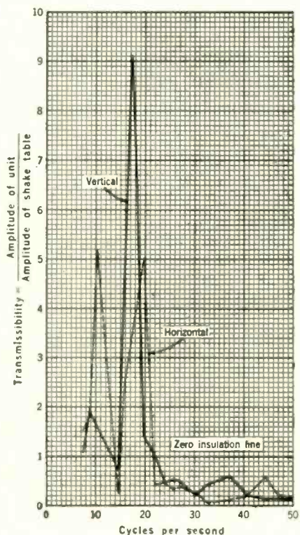
Fig. 6. Transmissibility curve with resilient supports in a horizontal plane approximately six inches below center of gravity
