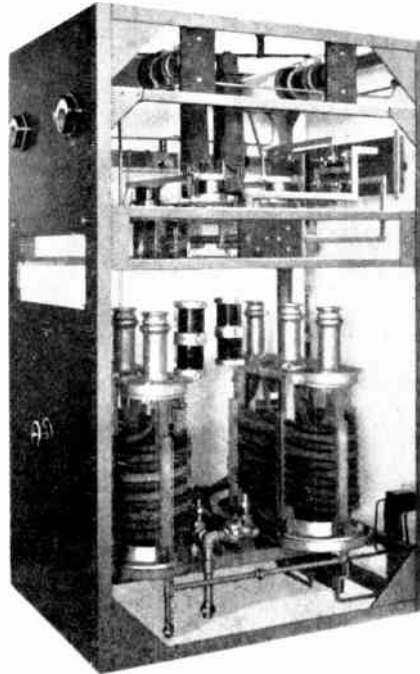
A side view of the last-stage tube unit before the tubes were placed in their jackets
