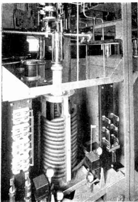
Rear view of the tube unit for the next-to-last stage
