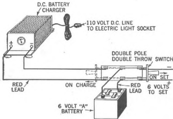
A practical hook-up of a direct current battery charger
