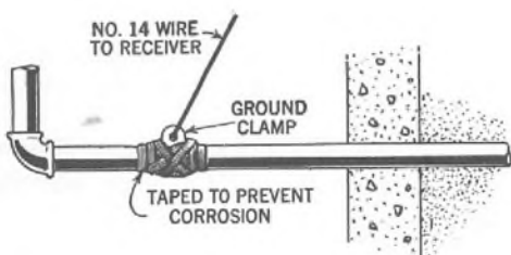
An ideal ground connection on the inlet of the cold water system.
