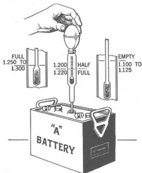
Illustrating the use of the hydrometer with a simple explanation of three specific gravity readings
