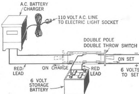
A practical hook-up of an alternating current battery charger
