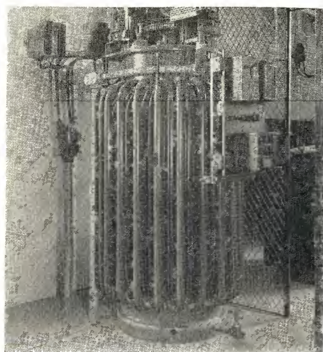
Automatic induction regulator keeping constant the voltage on the 100-kilowatt tubes.
