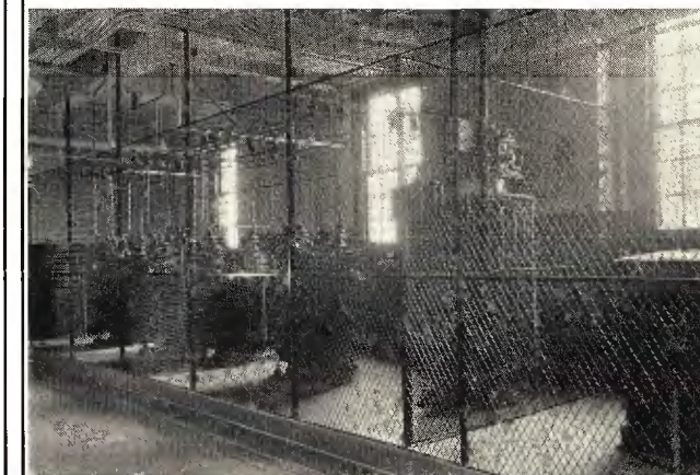
High voltage transformers increase 2,300 volts alternating current to 20,000 volts.
