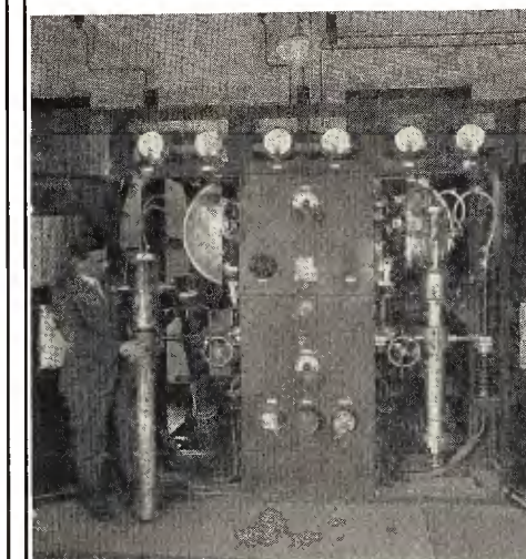
An operator removes a tube in the 50-kilowatt section from its water-cooled socket.
