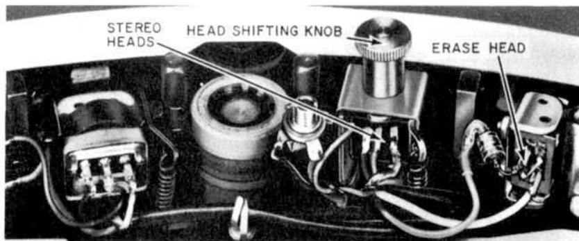
Fig. 412. Four-track conversion kits are adaptable for most commercial tape recorders. (The Nortronics Co., Inc.)
