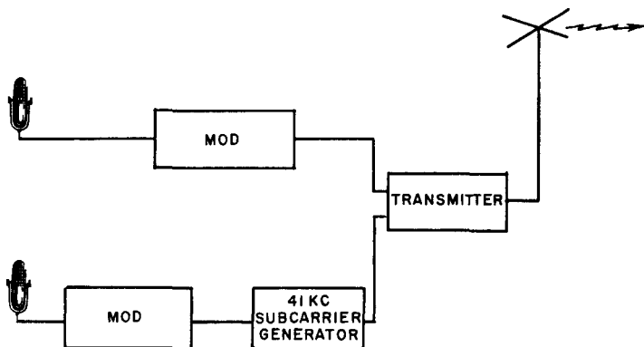
Fig. 609. Schematic diagram of the multiplex method used in musiccasting. The subcarrier signal is added at the transmitter.
