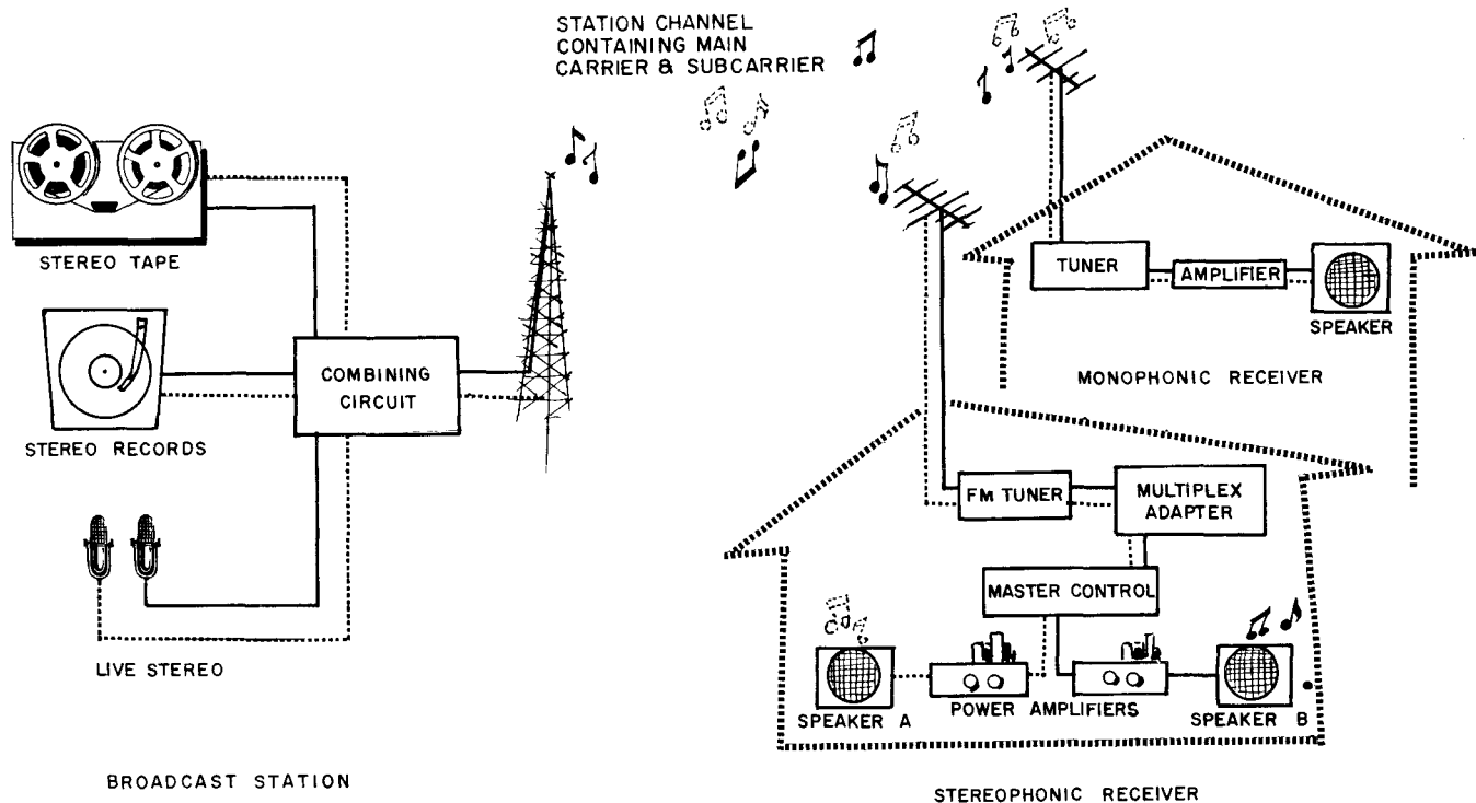
Fig. 616. The Crosby compatible sum-and-difference system permits the monophonic listener to receive both channels, hearing the program as he would any normal FM broadcast. The stereophonic listener unscrambles the signals he receives and feeds them to separate amplifiers and speakers for the stereo effect.
