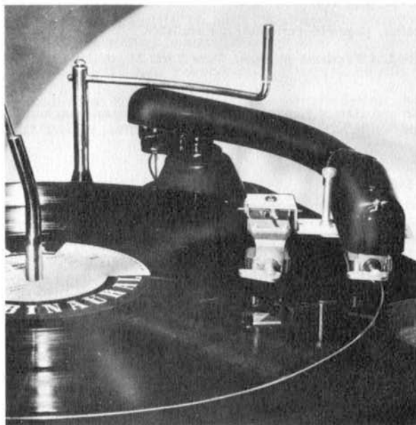
Fig. 215. Double tone arm system used a clip-on device for the second cartridge. (Cook Laboratories, Inc.)
