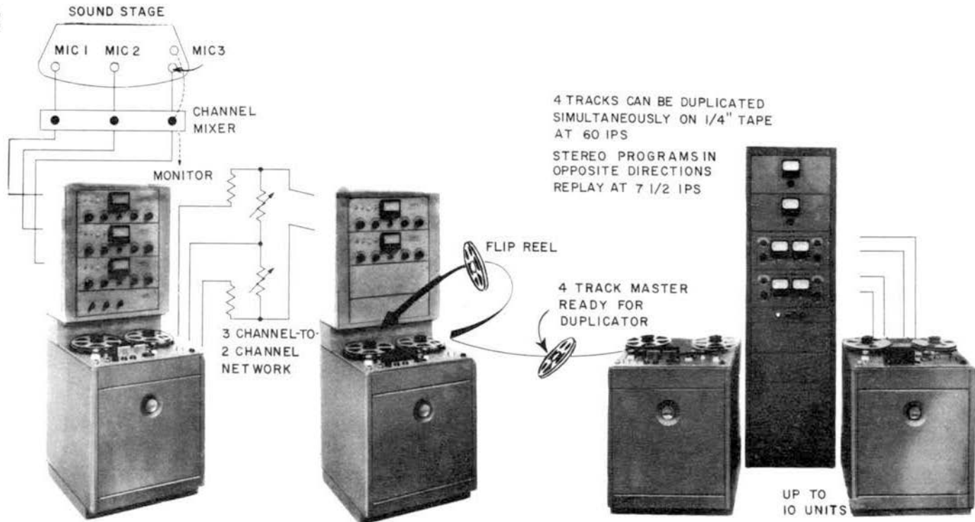
Fig. 407. The actual steps in preparing a master tape start with a multi-channel first master. This tape is then fed through a mixer to reduce the signals to two channels and recorded on a four-track tape. The new tape is flipped, two more channels dubbed on the other two tracks, and the new master is ready for duplication. (Ampex)
