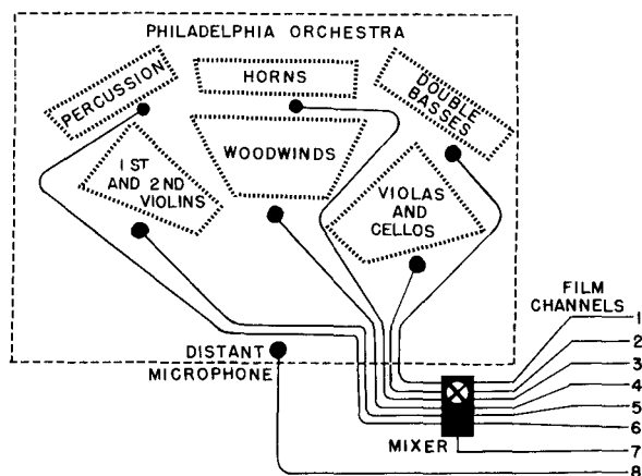
Fig. 304. The stereophonic recording arrangement used for "Fantasia".
