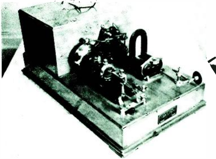
Early receiving equipment which, with the simple coherer as a "heart," first felt the pulse of wireless.
