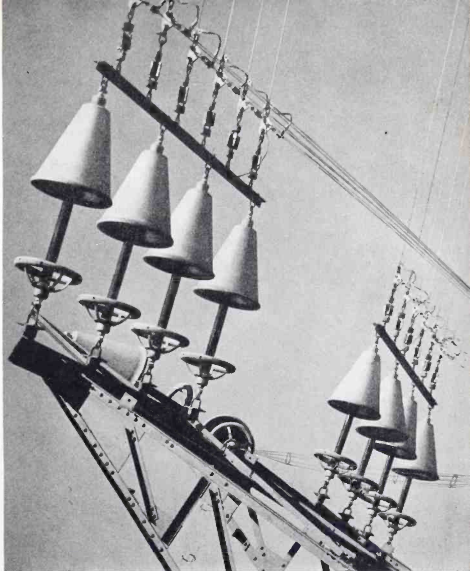
Insulators on the long-wave antenna at the transmitting station
