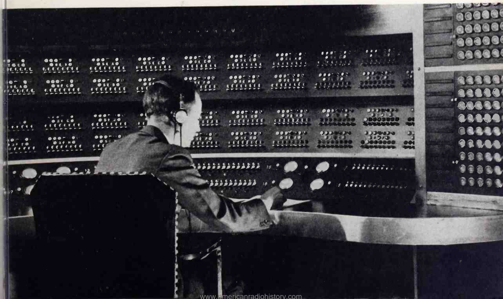
Close-up view of the master control desk
