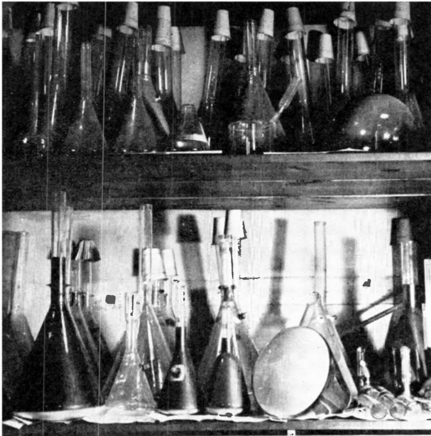
Experimental cathode ray tubes waiting to receive their electron guns. The tube at lower right shows the fluorescent material on the flat end
