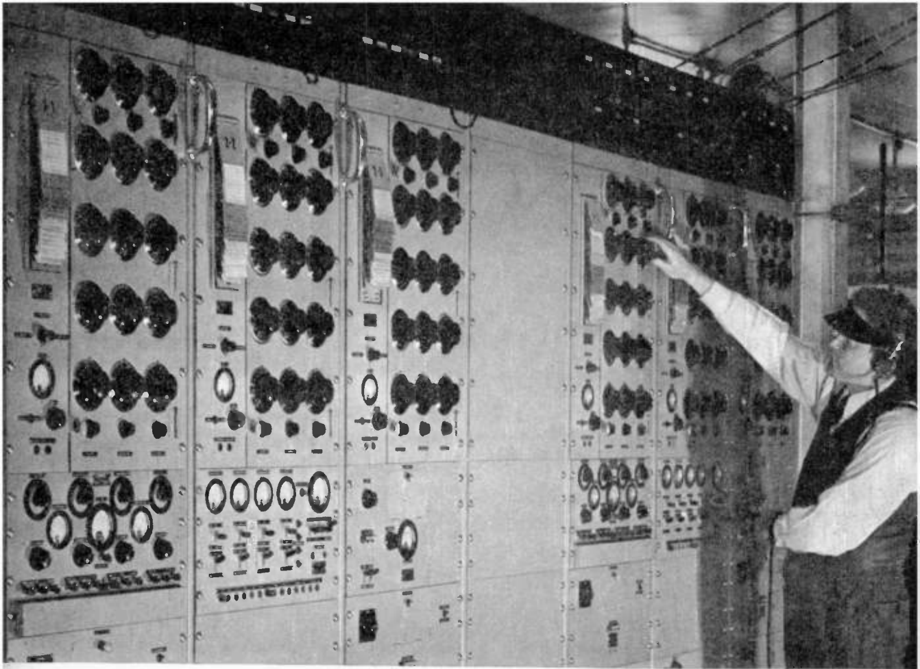
A bank of "diversity" receivers in the receiving station
