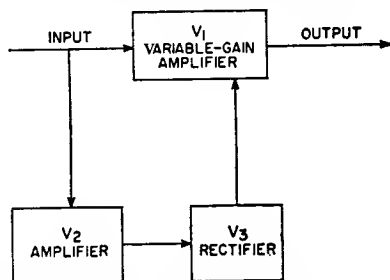
Fig. 33—Block diagram of volume compressor or expander circuit.
