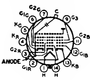
14AU ANODE = O_4 + G_5 + CL FOCUSING ELECTRODE = O_3
