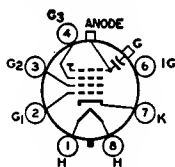
8JR ANODE = O_4 + CL FOCUSING ELECTRODE = O_3
