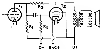
Fig. 29—Resistance-coupled stages using feedback resistor.
