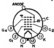
12AR ANODE = O_5 + O_5 + CL FOCUSING ELECTRODE = G_4
