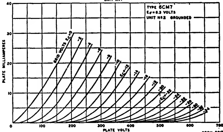
AVERAGE CHARACTERISTICS UNIT NR1
