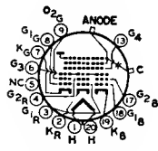
20A ANODE = G_5 + G_6 + CL FOCUSING ELECTRODE = O_3
