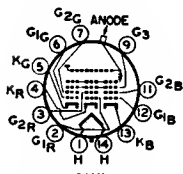
14AH ANODE = O_4 + G_5 + CL + R FOCUSING ELECTRODE = O_3
