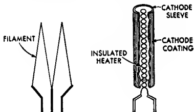
Fig. 1—Filament or directly heated cathode. Fig. 2—Indirectly heated heater-cathode.
