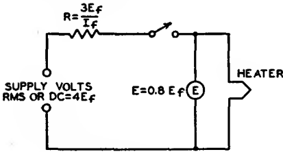
Fig. 94—Test circuit for measuring heater warm-up time.
