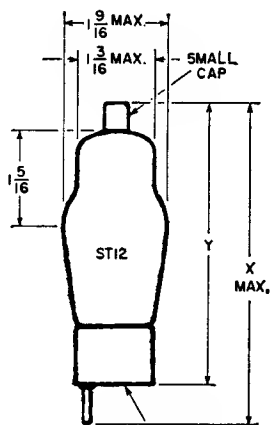
SMALL-SHELL SMALL 4-, 5-, 6-, OR 7-PIN -24-
