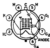
8KP ANODE = G_2 + G_5 + CL FOCUSING ELECTRODE = O_4
