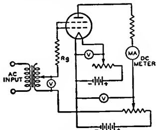
Fig. 104—Fundamental circuit of a power-output tester for class B operation of tubes.
