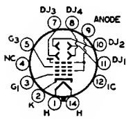
14R ANODE = G_3 + G_5 + CL FOCUSING ELECTRODE = O_3
