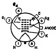
8KW ANODE = G_3 + G_5 + CL FOCUSING ELECTRODE = O_4
