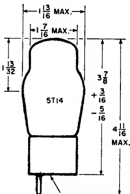
MEDIUM-SHELL SMALL 4-, 5-, OR 6-PIN; MEDIUM 7-PIN -26-
