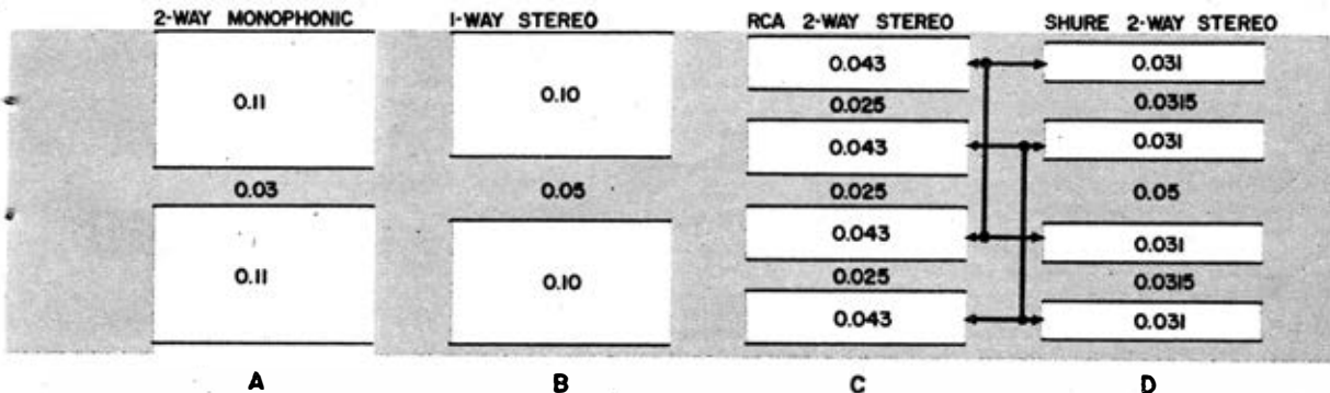
FIG. 2, above, shows in schematic form one piece of tape and what happens to it when exposed to the various head configurations of the different systems. See text for fuller explanation of this subject.
