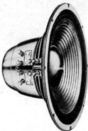
Dual voice coil 12-inch University woofer can be adjusted for 700, 2,500 or 5,000 cps high-end cutoff to suit requirement of the tweeter.
