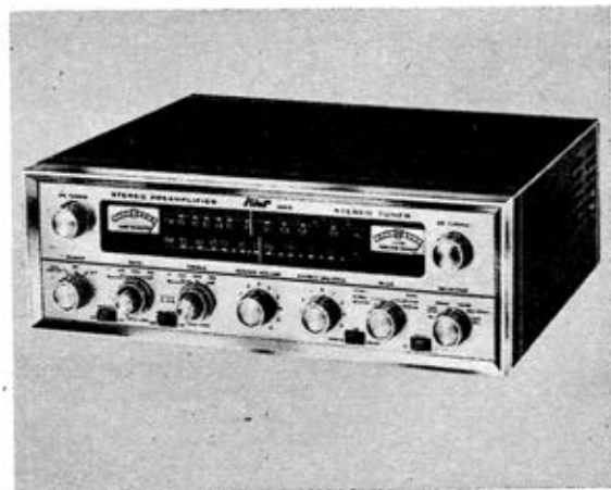
Pilot stereo FM-AM tuner and dual preamp costs $289.50, has AM and FM meter, 2 mv sensitivity for AM, 1 mv for 20 db FM, dual cathode output.
