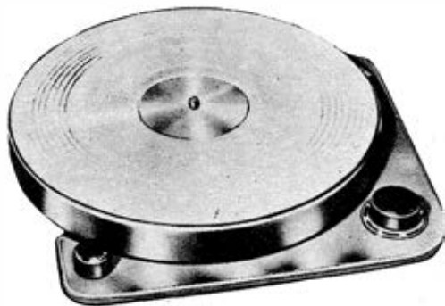
Lafayette 4-speed turntable sells for $37.50, has 3 lb. aluminum table, 4-pole motor. Noise and rumble is 50 db below average recorded level.
