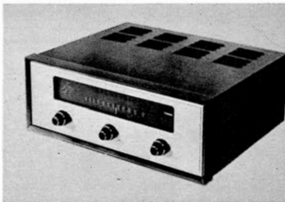
Fisher FM-100 tuner has main channel and Multiplex channel switch, four wide-band IF stages with limiters, bridge-connected mixer and oscillator.
