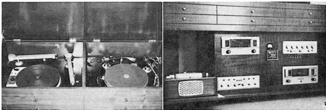
Components of system shown above include a Fisher AM-FM tuner, H. H. Scott 299 stereo amplifier, Fisher 90X FM tuner, Marantz preamplifier, VU meter and program clock, Tandberg stereo tape recorder. Closeup view of turn table setup shows, left, stereo arrangement with Garrard 301 turntable and two Pickering arms. At right is a Presto K-10 turntable with two Rek-O-Kut 120 arms. Total cost of system: $4,855.40.
