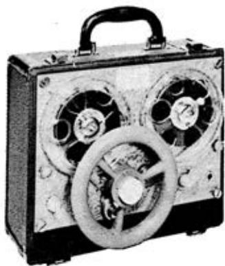
Magnemite recorder is similar to model shown at left, has no meter. It employs flywheel, weighs 15 lbs., operates for 1½ hours at 1½ ips.
