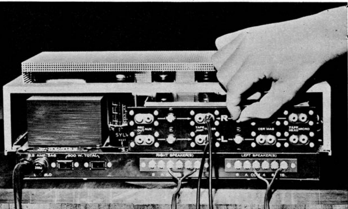
Rear view of Bell stereo amplifier showing speaker connections, input and output jacks.
