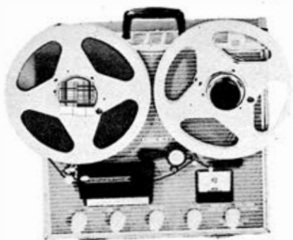
Concertone VII has frequency response of 30-17,000 cps \pm 2 db at 7½ ips, plays two- or four-track stereo, has 3-motor drive, weighs 39 lbs.
