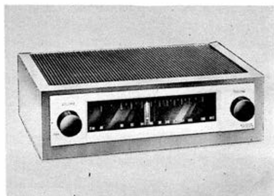
Eico FM tuner is available in kit form or assembled. Response is 20-20,000 \pm 1 db. It has Multiplex adaptor output, cathode follower tube.
