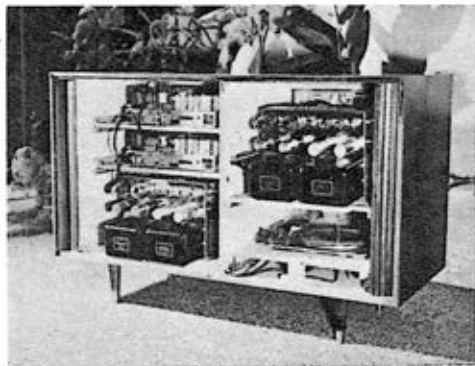
Compact installation in cabinet, front and rear view, includes two McIntosh MR-55 AM-FM tuners, two McIntosh preamplifiers, Magnadette tape recorder and stereo preamp with two VU meters. Turntable is a Miracord XS-200 automatic. Rear view shows two 60-watt McIntosh basic amplifiers installed vertically. Note ample area provided for good circulation of cooling air currents.
