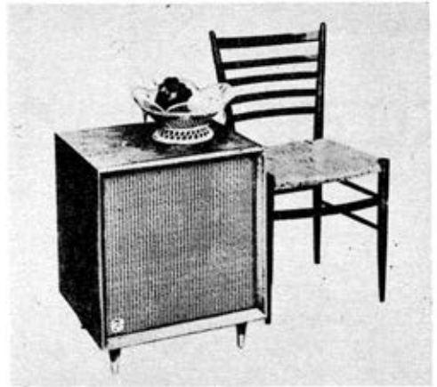
Floor model RJ enclosure for 12-inch speakers extends the bass range to 50 cps without resonant peaks. Enclosure is slightly larger than speaker.
