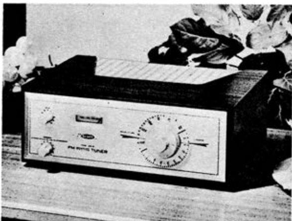
FM-only tuner by H. H. Scott features automatic gain control, interstation noise suppressor, a signal strength and tuning meter, Multiplex jack.
