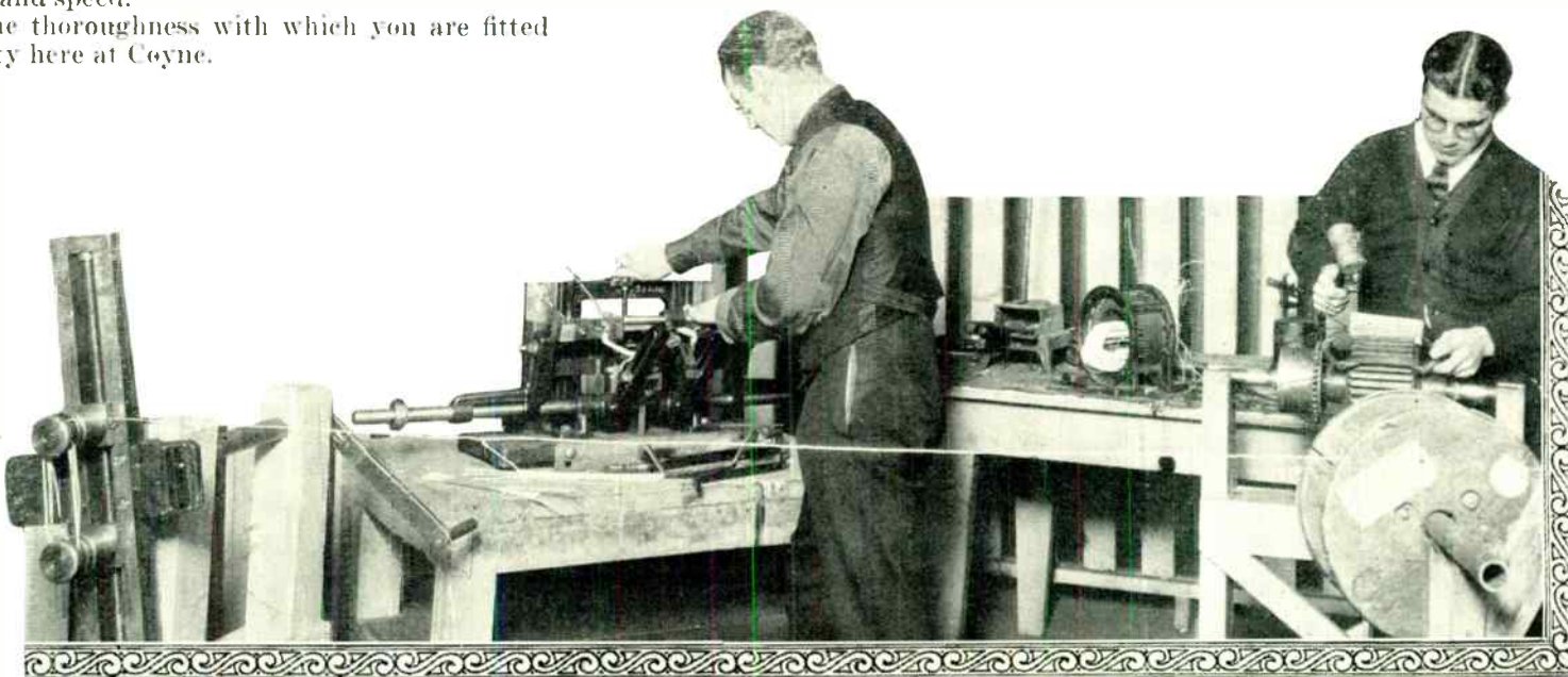
Operating Coil Winding and Coil Forming Machinery
