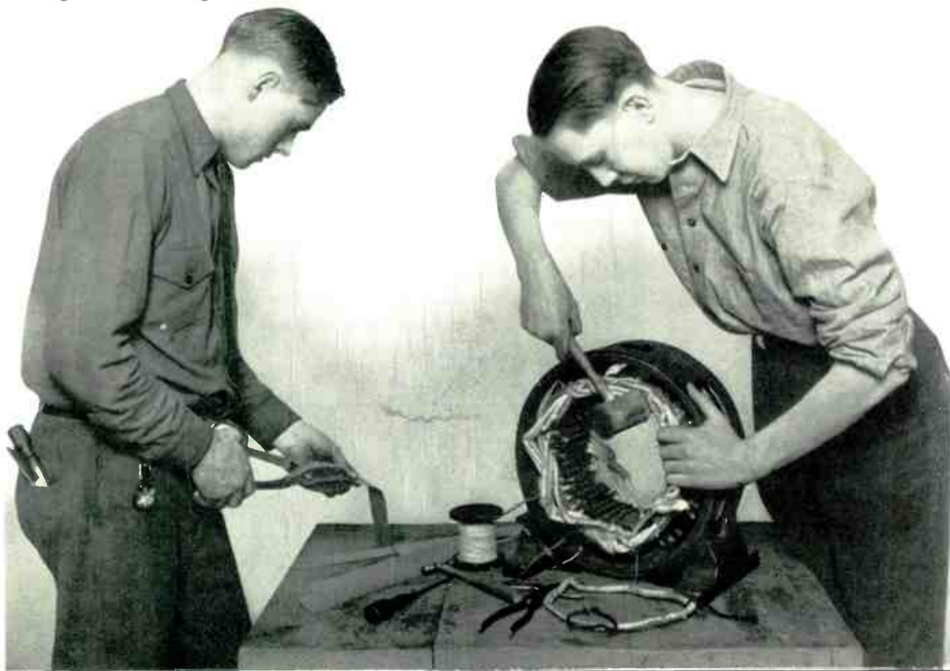
Overhauling and Testing a Motor Before Rewinding
