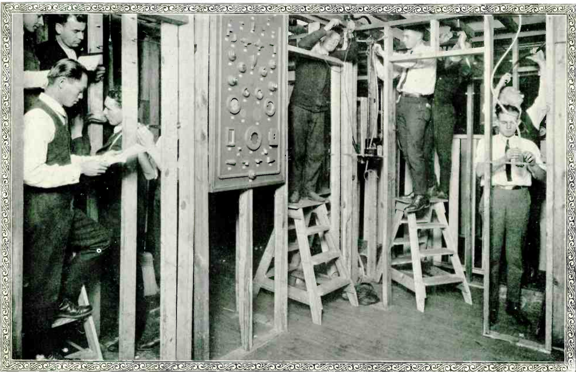
House Wiring—Showing B. X. Work—Just Like You Do It Out on the Job
