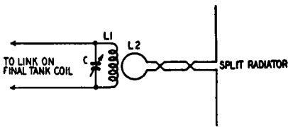
Fig. 604. Link coupling of sky wire to final means easier adjustment, more output.
