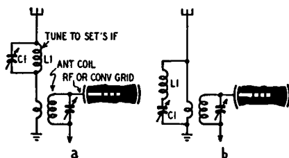
Fig. 404. I.F. interference eliminator.
