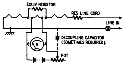
Fig. 410. Heater-to-cathode leakage causes hum.
