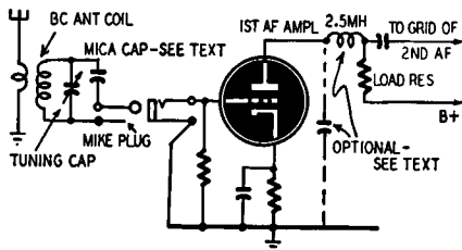
Fig. 517. Amplifier tube as detector.
