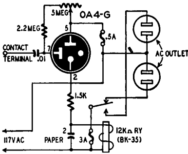
Fig. 613. Electronic relay control.
