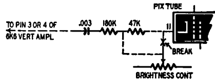
Fig. 313. Vertical retrace blanking circuit.
