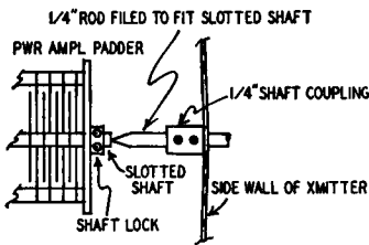
Fig. 611. Coupling extension shaft to padder.
