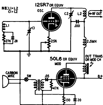
Fig. 708. Methods for improving oscillator stability.
