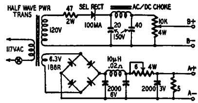
Fig. 419. Power supply for portables.
