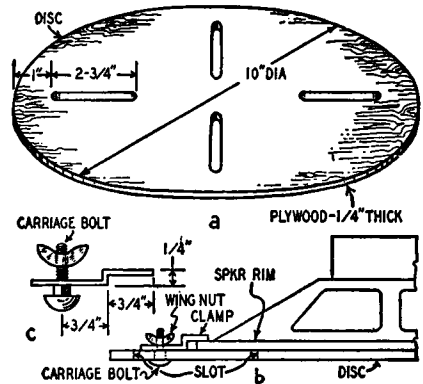
Fig. 520. Kink to protect speaker cones.
