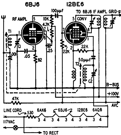
Fig. 418. Hint for removing heterodyning.
