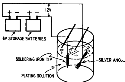
Fig. 401. Silver plating soldering-iron tips.
