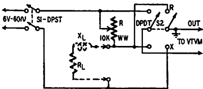
Fig. 705. The measurement of inductance.
