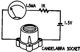
Fig. 128. Setup for checking pilot lights.
