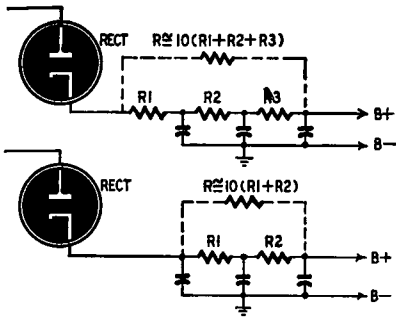
Fig. 412. Easy modification of the filter in transformerless power supplies will give good hum reduction.
