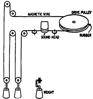
Fig. 513. Arrangement for endless wire recording.
