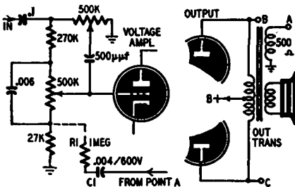
Fig. 512. Bass-boost and inverse-feedback.
