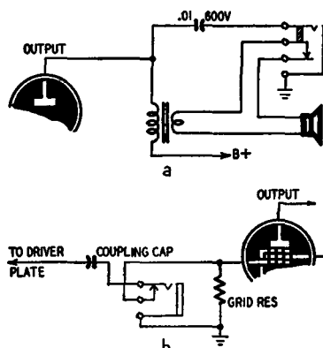
Fig. 427. Two ways to connect headphones to a radio or TV receiver.
