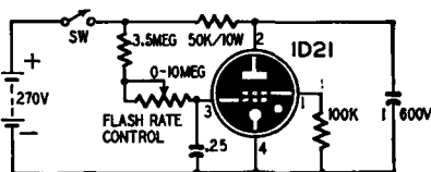
Fig. 117. Circuit of portable stroboscope.
