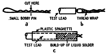
Fig. 210. Modified bobby pin used as a miniature test-lead clip.
