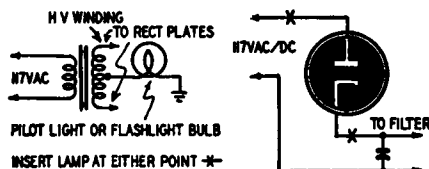
Fig. 408. Flashlight bulb used as a fuse.
