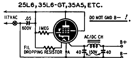
Fig. 403. Use weak output tubes as rectifiers.
