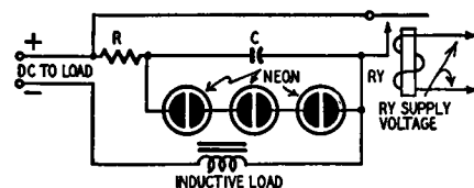
Fig. 701. Use neon lamps for suppression of sparking at relay contacts.
