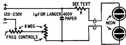
Fig. 126. Relaxation oscillator used as a stroboscope.
