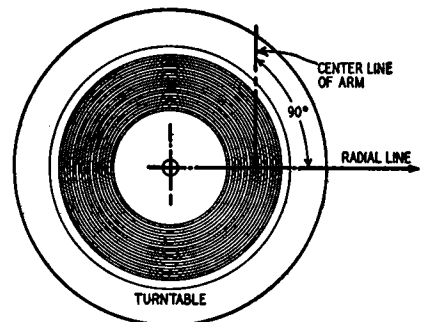
Fig. 511. Hint for finding correct position of record-player pickup arm.
