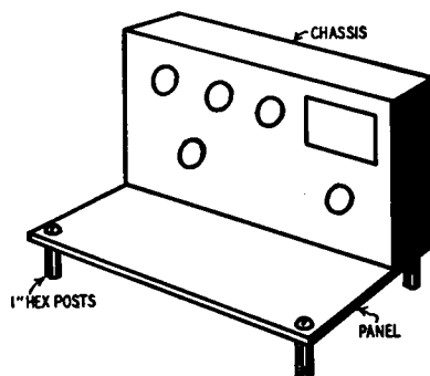
Fig. 707. Protect panel from scratches.
