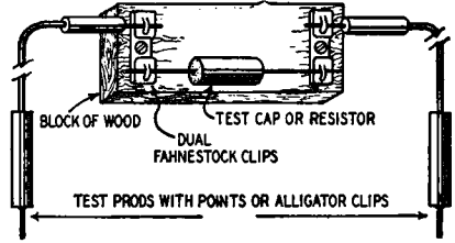
Fig. 133. Experimental substitution block.
