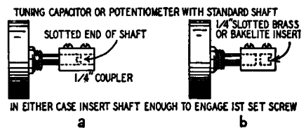
Fig. 612. These ideas will eliminate fumbling around trying to get a screwdriver into a slotted control.
