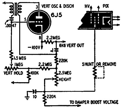
Fig. 311. Circuit modification for suppressing a beam after TV set is turned off.
