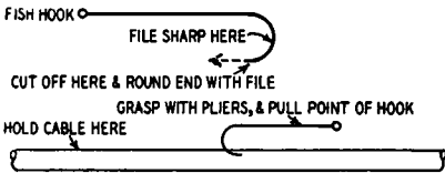
Fig. 209. Fish hook as braid remover.
