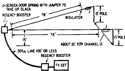
Fig. 303. V-beam for long-range TV.
