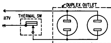
Fig. 202. Soldering iron heat regulator.
