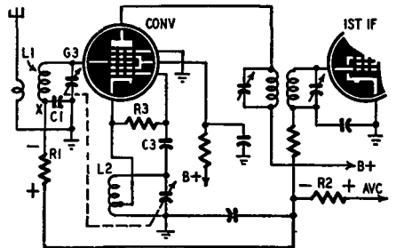
Fig. 415. Excessive local oscillation can cause poor sensitivity.
