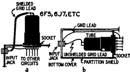
Fig. 515. Mount for high-gain preamplifier.
