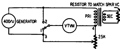
Fig. 510. Use this idea for finding impedance of transformers, chokes, voice coils, etc.
