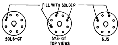
Fig. 406. Use tubes with broken keyways.
