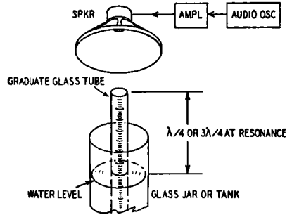
Fig. 130. Oscillator calibration setup.
