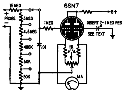
Fig. 107. Method for stabilizing the v.t.v.m.
