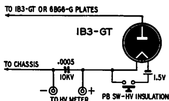
Fig. 307. Adapter circuit for measuring pulse voltages on plates of horizontal output tube and high-voltage rectifier.
