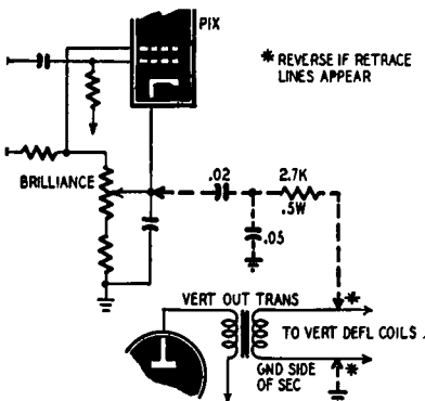
Fig. 312. Retrace line elimination circuit.
