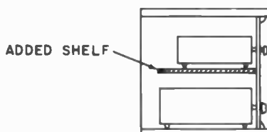
Fig. 1309. When a separate tuner and amplifier are "stacked", it is best to insert a \frac{1}{2} " plywood shelf to support the upper unit.
