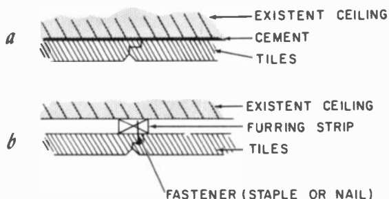
Fig. 902. Installation of acoustic tile (a) by cementing directly to ceiling, (b) by attaching to furring strips.
