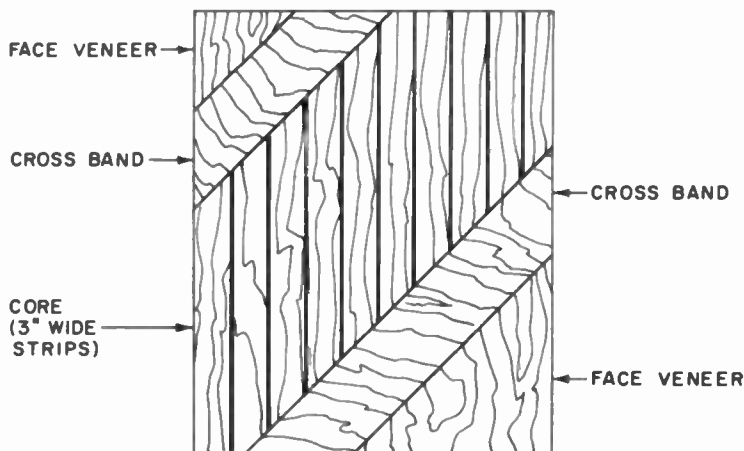
Fig. 1202. Details of solid core plywood construction.
