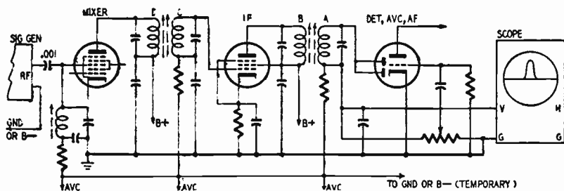
Fig. 502. Connections to scope for alignment of peak-tuned i.f.
