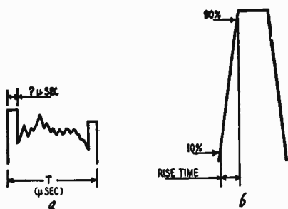
Fig. 619-a, -b. Typical pulse appears in composite video signal (a). Rise time of pulse is shown in illustration (b).
