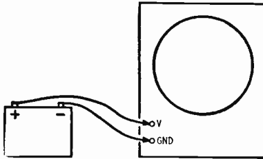
Fig. 618. Means for determining deflection polarity of scope.
