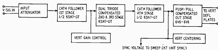
Fig. 401. Block diagram of vertical amplifier section of 208B scope.
