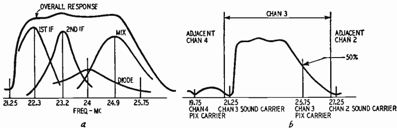
Fig. 507-a, -b. Response curve of stagger-tuned i.f. (left) and frequency relationship of sound and picture signals in the i.f. (right).
