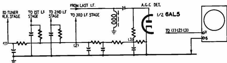
Fig. 706. The a.g.c. network can be tested with the scope.
