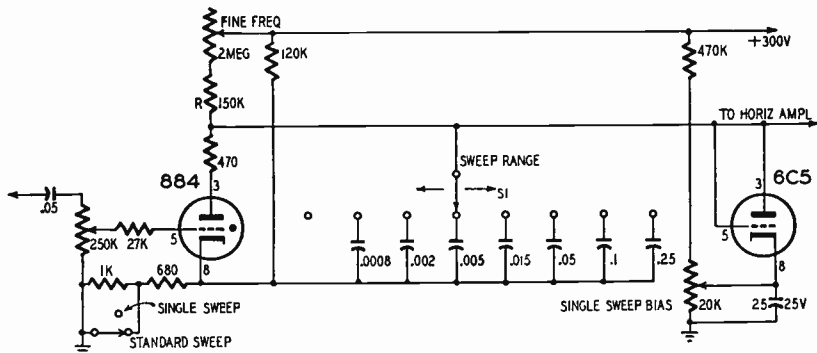
Fig. 309. Thyratron sweep circuit used in connection with study of transients
