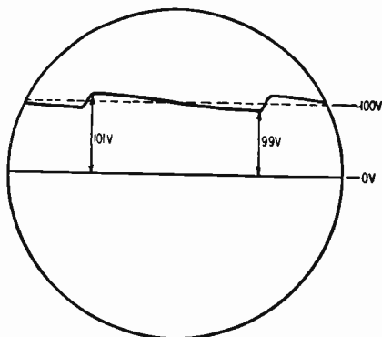
Fig. 717. Method for measuring ripple voltage.
