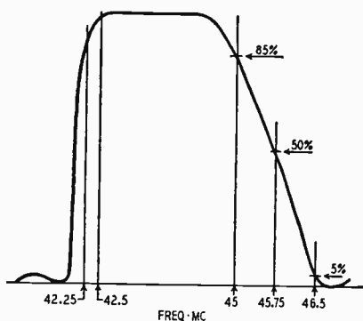
Fig. 512. Marker points are used to check the response curve.
