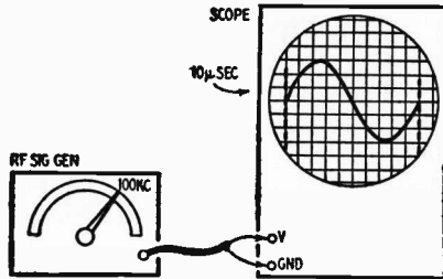
Fig. 620. Technique for calibrating scope sweep in microseconds.
