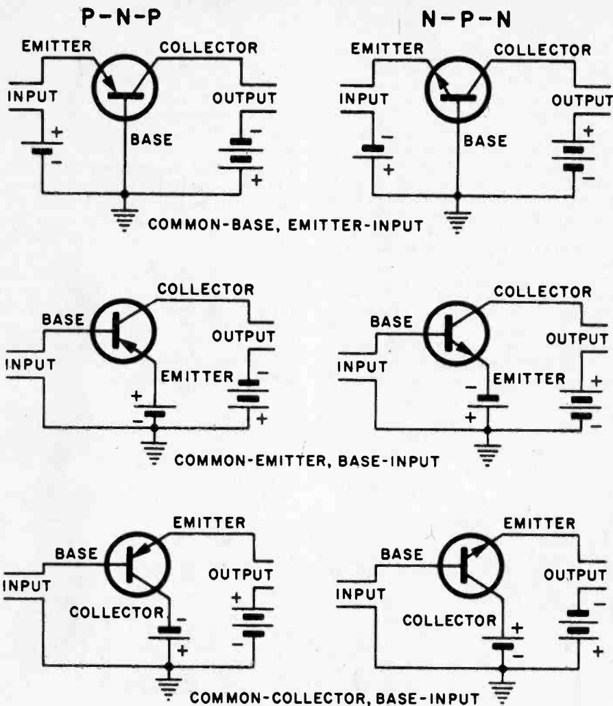
FIG. 10. Three modes of connection are possible with each of the two transistor types. Circuit connections are shown above with the P-N-P type at left and the N-P-N transistor on the right.
