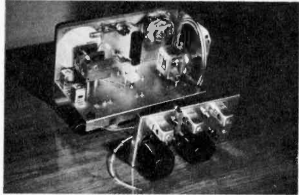
Rear view of completed radio compass without case. Meter controls are at front, speaker at side.
