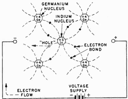
FIG. 3. When germanium is doped with a valence-3 material, the electron flow is effected by the movement of "holes" toward negative terminal.
