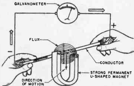
Schematic representation of experiment shows conductor cutting invisible flux.
