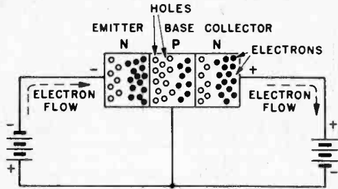
FIG. 8. In the N-P-N transistor, above, internal conduction takes place by movement of electrons rather than by holes. See text for details.
