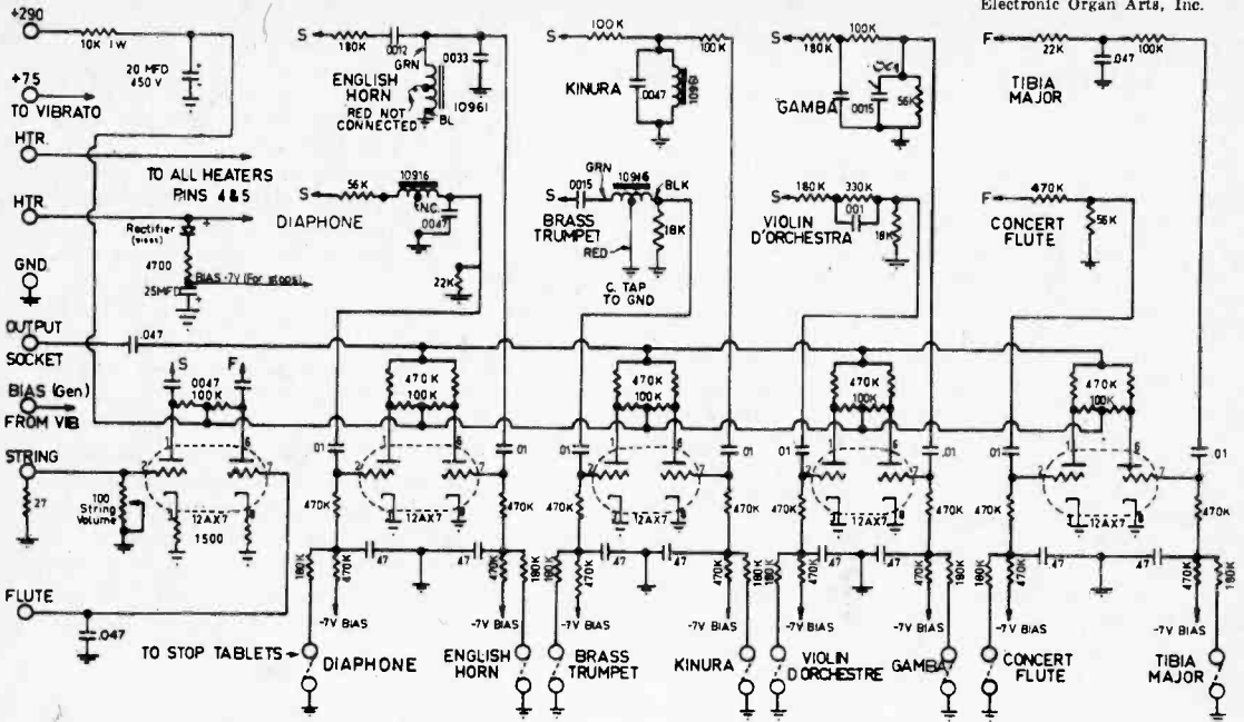
SOLO TONE CHANGER SCHEMATIC
