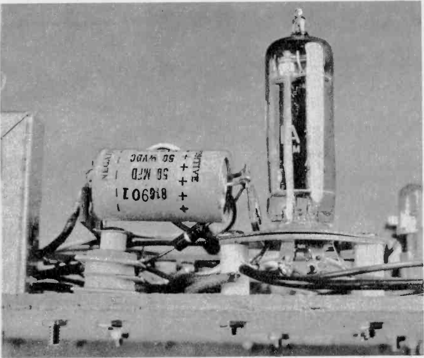
Tiny selenium rectifier above is dwarfed even by miniature tube. Rectifier is water stack under left end of tubular capacitor. Cover plate (below) encloses complete power supply plus electron tube.
