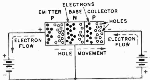
FIG. 7. When the P-N-P transistor is correctly biased, there is a flow of electrons in external circuit, but a flow of "holes" within crystal.
