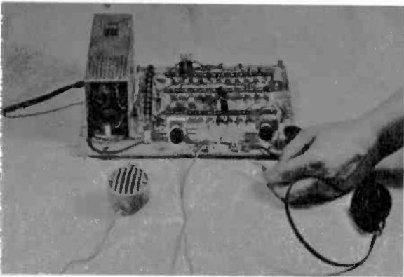
Final steps in construction comprise insertion of microphone and headphone tips in the Fahstock clips.
