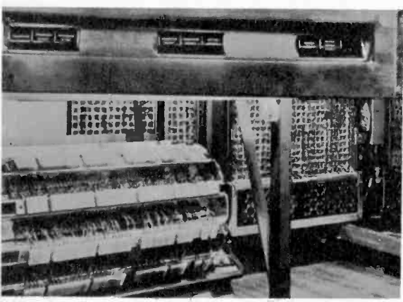
International Business Machines Another memory unit is the IBM's 650 magnetic drum. It turns at the rate of 12,500 rpm and has magnetized spots on its surface. The drum holds up to 20,000 digits at 2,000 "addresses."
