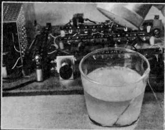
Detecting element (above) can be made by stripping the ends of a pair of wires, keeping them closely spaced.
