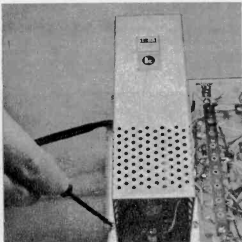
Tiny selenium rectifier above is dwarfed even by miniature tube. Rectifier is water stack under left end of tubular capacitor. Cover plate (below) encloses complete power supply plus electron tube.
