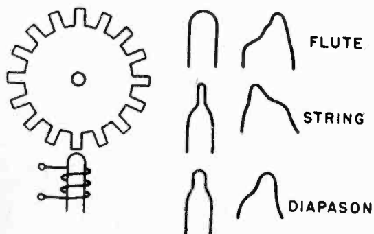
FIG. 3. Goodell and Swedien tone wheel and poles.
