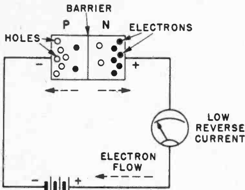
FIG. 5. When the voltage is reversed, with the negative terminal to P and the positive to N, the resulting current flow will be almost zero.
