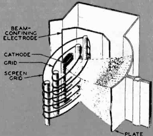
FIG. 9. In a beam power tube sheets of electrons travel to the plate from the cathode in center.
