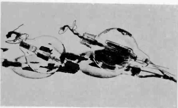
Bell Telephone Laboratories DeForest's audion tube, developed in 1912, is shown at left. At right is the high-vacuum tube developed in 1913 for the telephone repeater.
