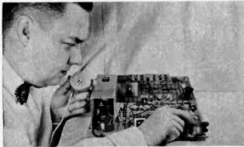
Sensitivity adjustment is made, speaking into microphone at normal voice level.
