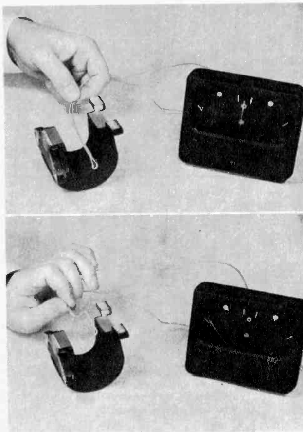
Folded pair of wires generates no current externally, as two currents flowing in opposite directions cancel each other.
