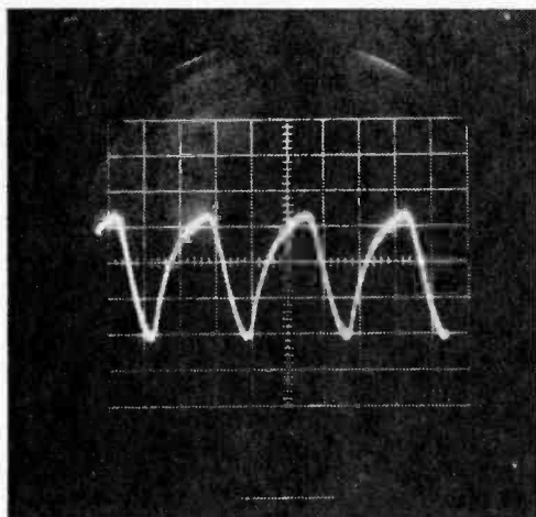
Fig. 16. Almost sawtooth wave form, representing extreme bass response, is obtained when bass control has been cranked full on.
