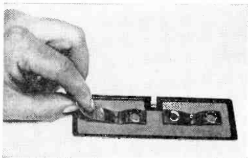
Making battery contacts bright and shiny (above) prevents intermittent operation. Magnetic field at tip of soldering gun (below) is demagnetizing recorder heads.
