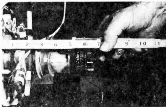
Fig. 5. (top) While you are making notes be sure to mark down the measurements so you can replace the yoke assembly physically before worrying about convergence, purity. Fig. 6. (below) Here author is pointing to blue lateral magnet and the tab inside the neck of the CRT. Tab is not obscured by blue lateral magnet in Fig. 4. By first replacing the components according to the measurements most adjustments are minor.
