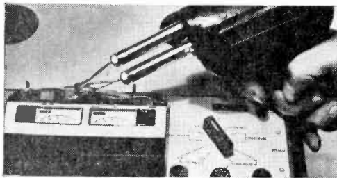
Making battery contacts bright and shiny (above) prevents intermittent operation. Magnetic field at tip of soldering gun (below) is demagnetizing recorder heads.
