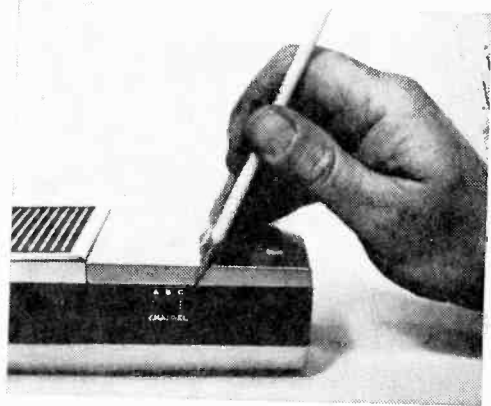
Common source of "no sound" is flimsy headphone jack (above) which might fail to make normal/through-speaker connection; remedy is to clean or replace jack in effort to increase spring tension. At right, non-technical users often assume W-T is defective when selector has been accidentally moved to unused channel.
