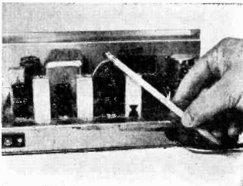
Loose elements in a tube cause microphonics and can actually sound like a concert of electronic music when you tap the faulty tube with your finger or the eraser end of a lead pencil.
