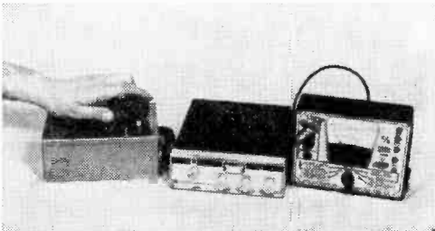
Placing mike on top of speaker emitting steady tone saves talking when checking modulator.
