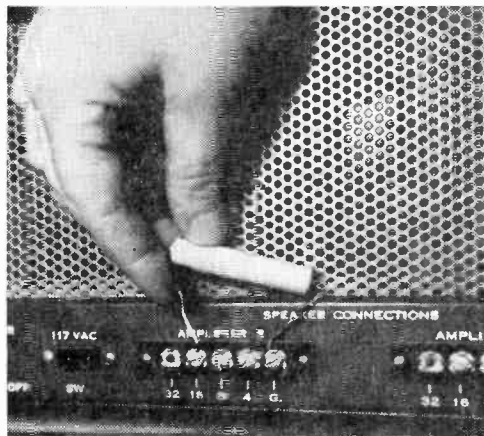
Fig. 7. A load resistor is placed across output terminals of amplifier, then scope is connected. Leads from amplifier go to vertical input.
