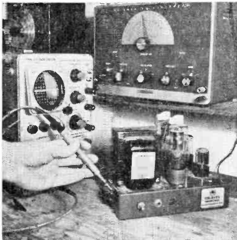
Fig. 6. Heathkit Model 1G-82 Sine-Square Generator and Tektronix 317 Oscilloscope being used to check output of hi-fi amplifier.
