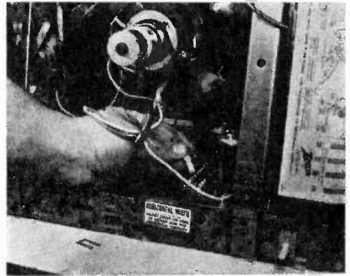
Fig. 10. One type of focusing arrangement is adjusted simply by selecting proper tap.
