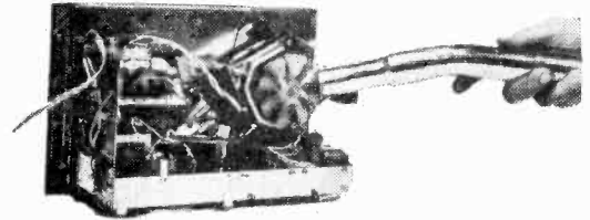
Strobe wheel indicates speed of tape (top) not capstan; quickly indicating slippage. Vacuum removes loose dust (below). Small paint brush will help remove the residue.
