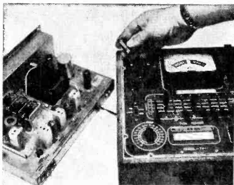
Always check out vacuum tubes first, since roughly 80-percent of tuner troubles can be attributed to tubes. As mentioned in text, tube troubles are often indicated by specific symptoms in quality of audio performance.
