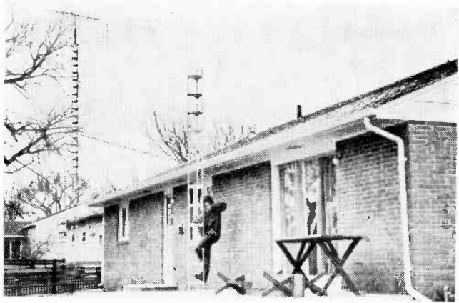
Concrete must be firmly set before you start adding the other sections to the section set in the concrete base.
