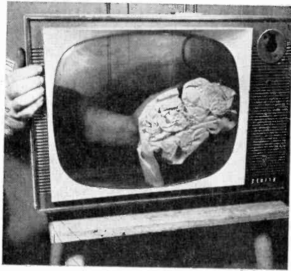
While picture tube is out of cabinet, take advantage and give safety glass a thorough cleaning with water and a drop of detergent.
