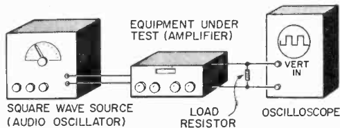
Fig. 5. Pictorial of test setup for square wave testing shows load resistor connected. Always set bass and treble controls in "flat" position.
