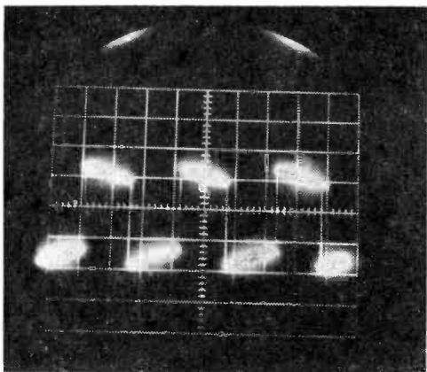
Fig. 11. Slope of square waves across top and bottom indicates amplifier has poor low-frequency response. Text gives probable causes.
