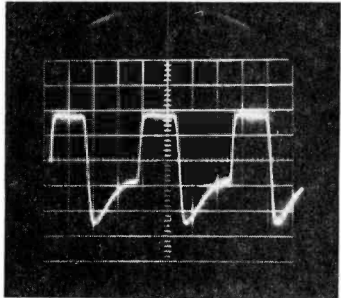
Fig. 10. Lack of symmetry between top and bottom of square wave indicates excessive signal input. Reduce gain of audio oscillator.
