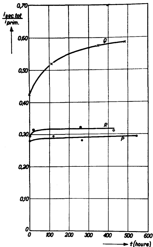
Fig. 24 - Change of capability for secondary emission of different soot surfaces face to face with an oxide cathode as a function of time.
