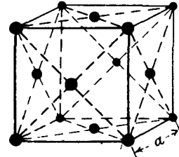
Fig. 2 - Face-Centered-Cubic Crystal Structure (Courtesy of Metals and Alloys)
