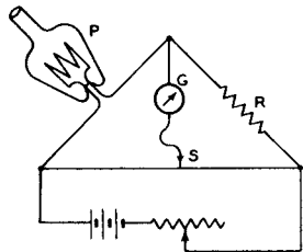
Fig. 11 - Electrical diagram of the Pirani gauge.
