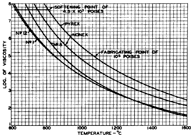
Fig. 3 - Viscosity curves of several glasses.
