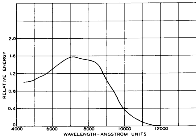
Fig. 21 - Spectral distribution curve for semitransparent photosurface having white-light sensitivity of 16-17 \mu\text{a/lumen} .
