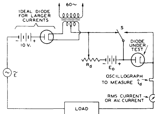
Fig. 3 - Half-wave circuit for measuring \hat{r}_d , \bar{r}_d , and |r_d| .
