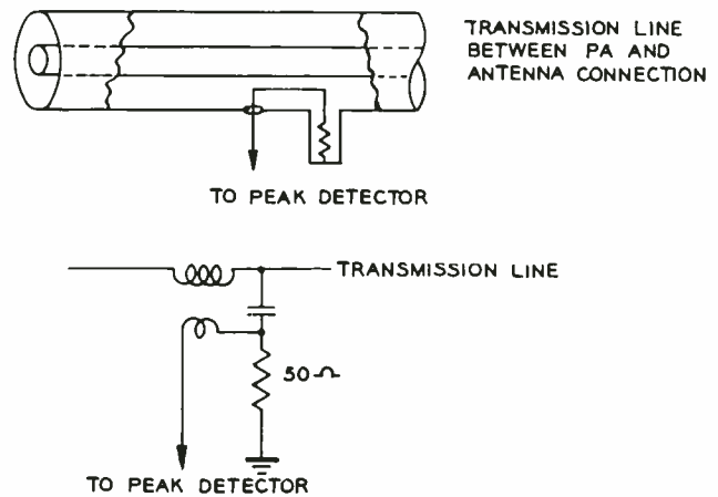
FIG. 18. Directional coupler.
