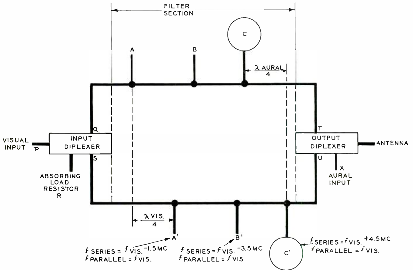
FIG. 3. Simplified schematic diagram UHF Filterplexer.
