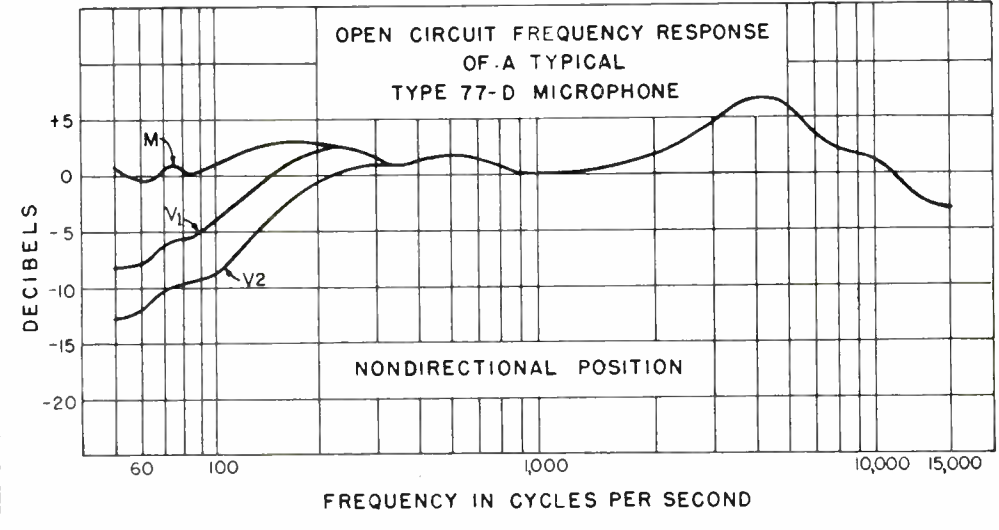
FIG. 5 (above). Directional patterns and frequency response curves for the RCA Type 77-D microphone.
