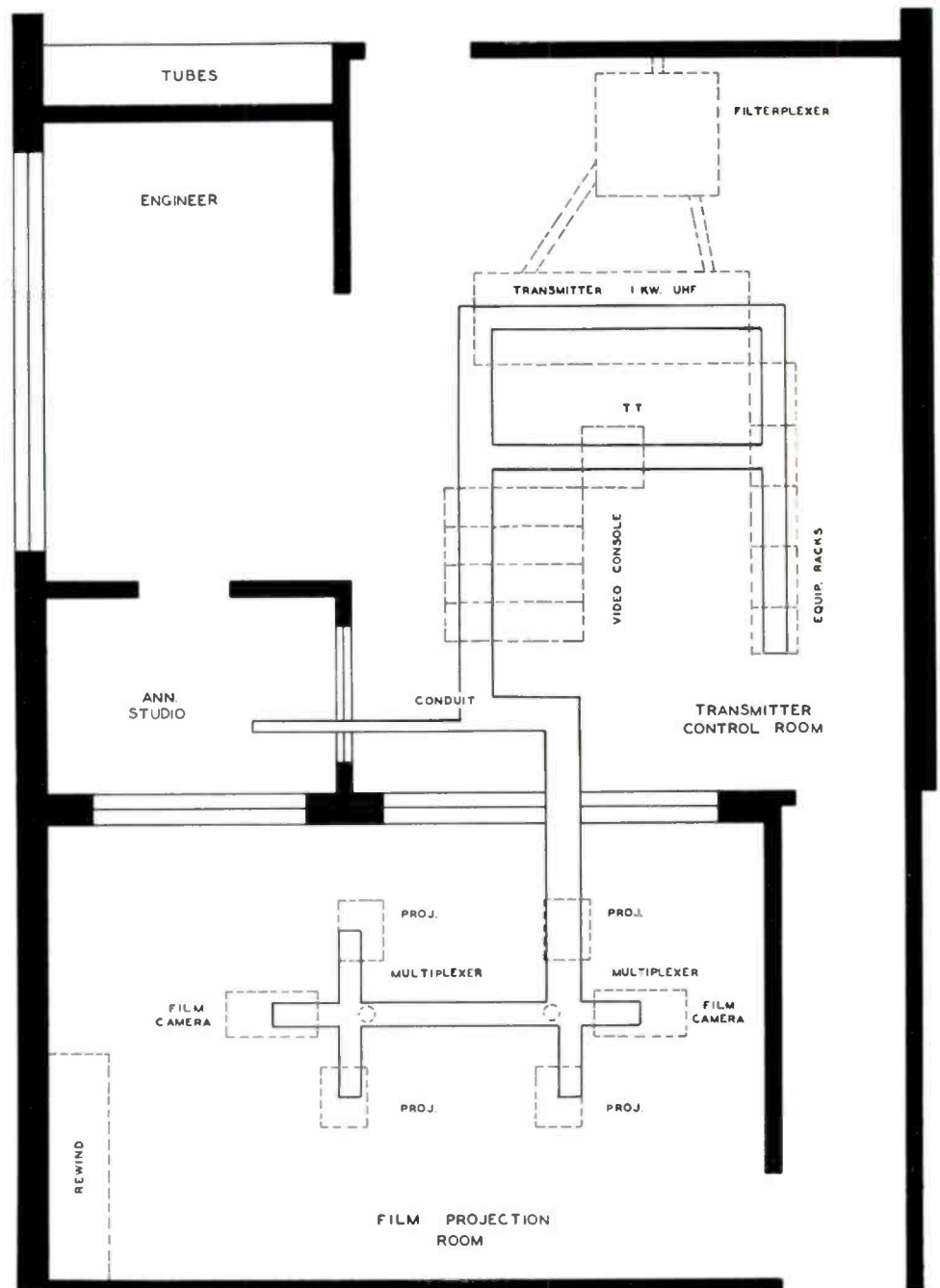
FIG. 8. A sample transmitter, rack and console duct layout. Practical planning should make provision for possible future addition of racks, console sections and transmitter cabinets.
