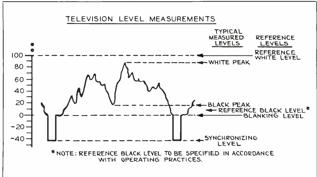
FIG. 1. Waveforms showing significant levels and details of the standard scale for measuring video levels.
