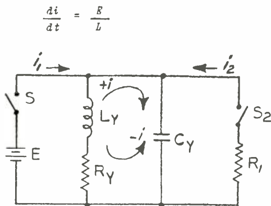
FIG. 45. Equivalent horizontal deflection circuit.
