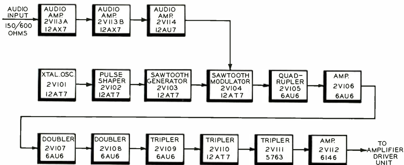
FIG. 4. Block diagram of FM Exciter for TT-10.
