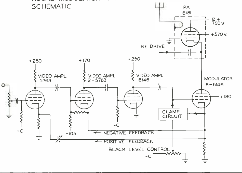
FIG. 7. Visual modulator simplified schematic.
