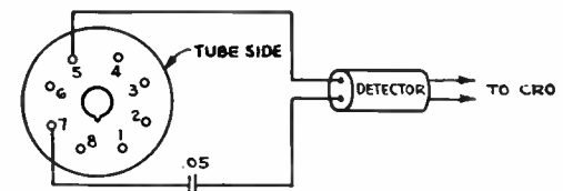
FIG. 10. Socket connections used between View Finder Kinescope (5FP4) and "CRO".
