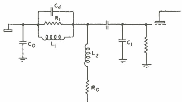
FIG. 54. Effect of coil capacity on constant-K filter.
