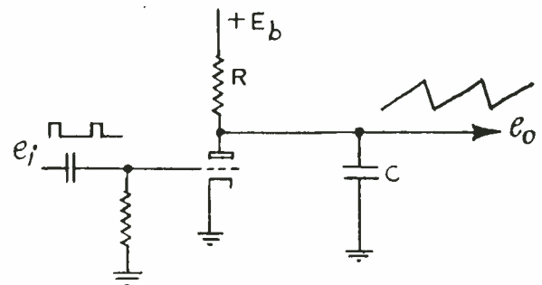
FIG. 35. Sawtooth generator circuit.
