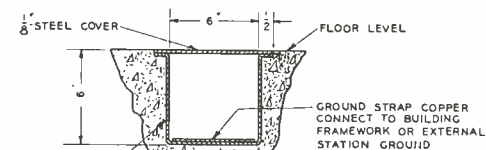
SECTION-AA TYPICAL WIRE DUCT CONSTRUCTION
