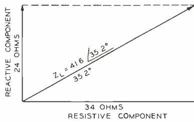
VECTOR DIAGRAM OF LOAD IMPEDANCE
