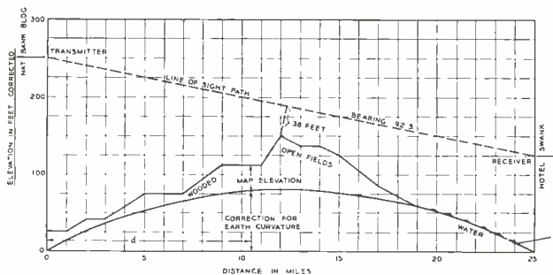
FIG. 7. Typical profile plot for line-of-sight path calculations.
