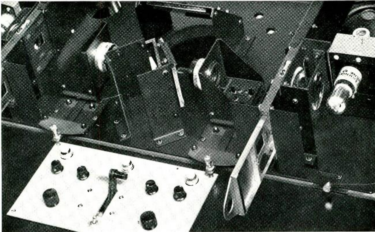
FIG. 4. Closeup view of Slide Scanner with top cover removed to illustrate the optical system employed.
