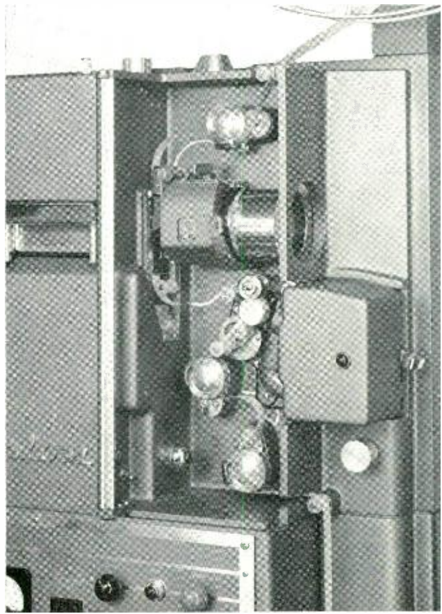
FIG. 13. Closeup of projection optical system and film transport of the TP-6A projector
