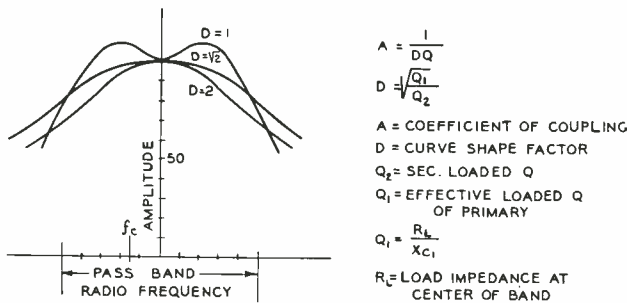
FIG. 20. Amplitude characteristic of coupled resonant circuits.
