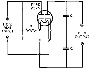
VOLTAGE-DOUBLER CIRCUIT
