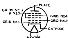
Pentagrid Converter
