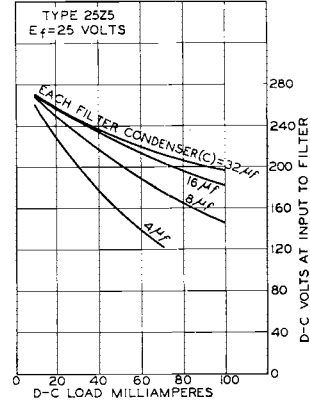
OPERATION CHARACTERISTICS VOLTAGE DOUBLER
