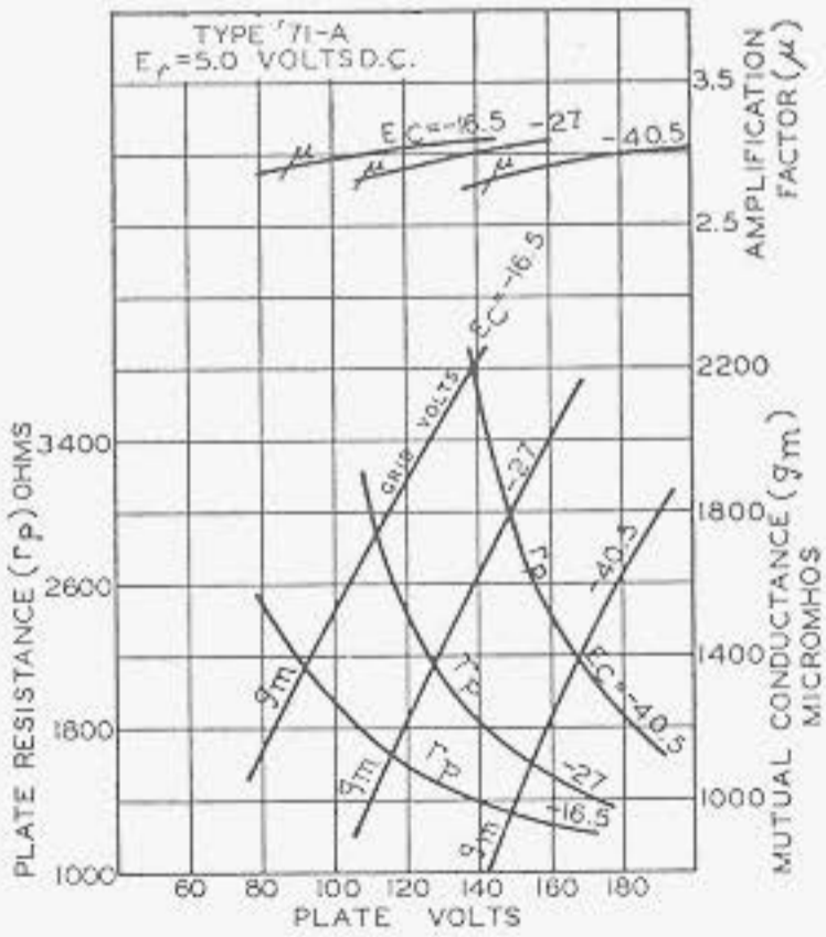
AVERAGE CHARACTERISTICS
