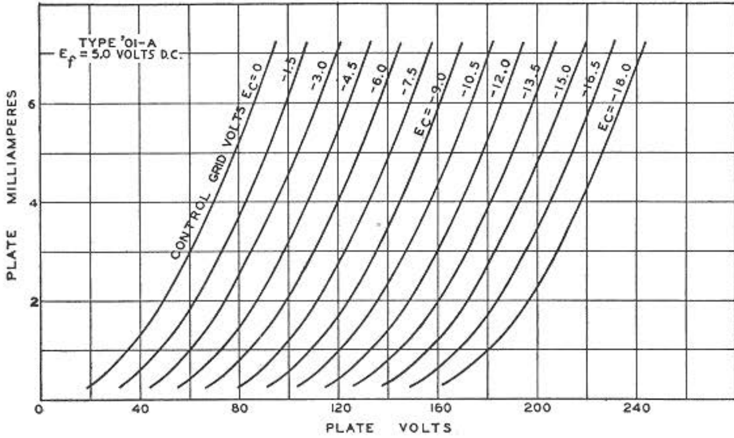
AVERAGE CHARACTERISTICS
