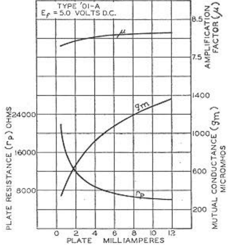
AVERAGE CHARACTERISTICS
