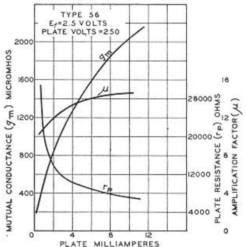
AVERAGE CHARACTERISTICS
