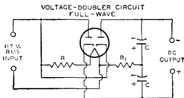
R = HEATERS OF OTHER TUBES IN SERIES WITH VOLTAGE-DROPPING RESISTOR
