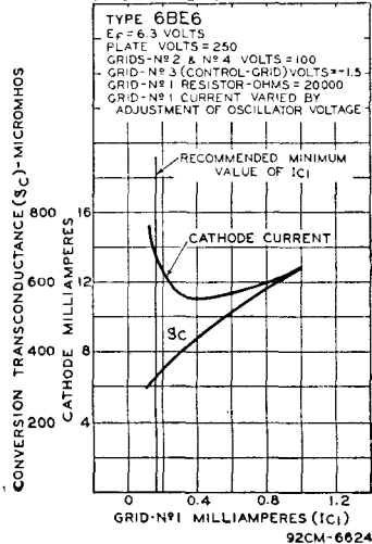
OPERATION CHARACTERISTICS WITH SEPARATE OSCILLATOR EXCITATION
