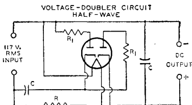
R_1 = PROTECTIVE RESISTOR
