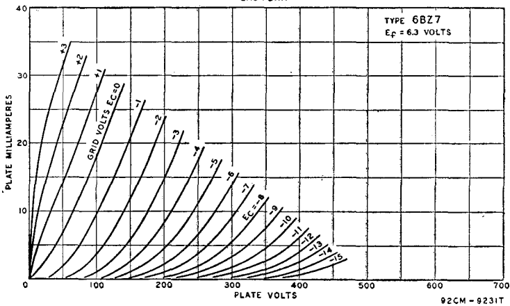
AVERAGE CHARACTERISTICS EACH UNIT
