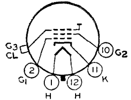
12D ULTOR = G_3 + CL
