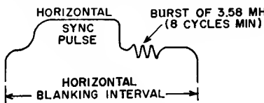
Fig. 96—Waveform for synchronizing signal.
