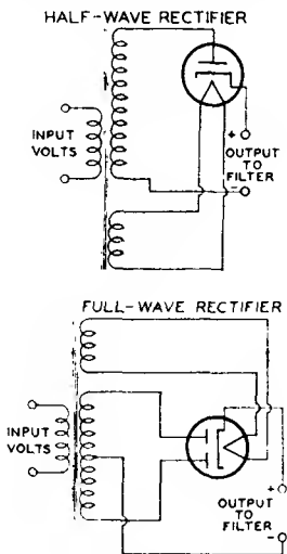
Fig. 18—Half-wave and full-wave rectifier circuits.
