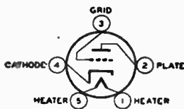
RCA-843
