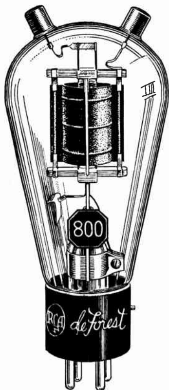
RCA-800
