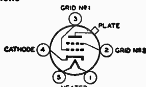
RCA-844
