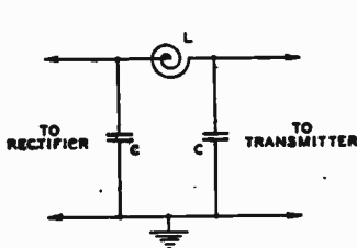
C = R-F BY-PASS CONDENSER, MICA L = R-F CHOKE
