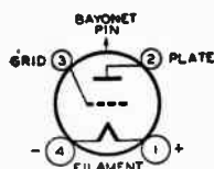
RCA-841 and 842
