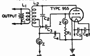
ULTRA-HIGH-FREQUENCY HARTLEY OSCILLATOR
