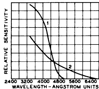
Fig. 10 - (1) Sensitivity curve for barium metal in Corex D glass. (2) Sensitivity curve for the vaporized deposit from a barium oxide coated cathode. (Rentschler & Henry, J.O.S.A., Vol. 26, p. 31, 1936)
