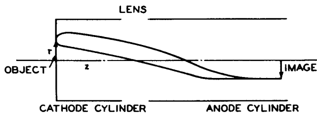
Fig. 17 - Cathode lens.
