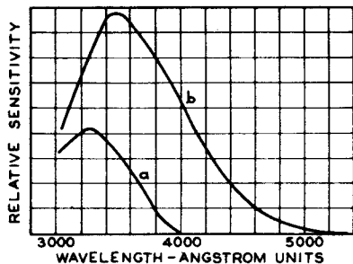
Fig. 9 - (a) Sensitivity curve for a calcium cell in Corex D glass. (b) Sensitivity curve for the same cell treated with the oxygen from a tube at 40 mm pressure. (Rentschler & Henry, J.O.S.A., Vol. 26, p. 31, 1936)
