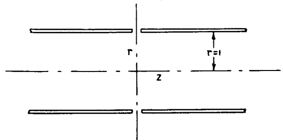
Fig. 14 - Coordinates for electrostatic cylinder lens.
