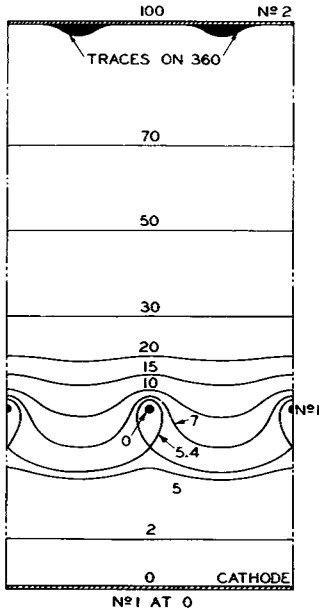
Fig. 7 - Equipotential map on scale model, with grid No.1 at zero potential. (Courtesy of The Institute of Radio Engineers)
