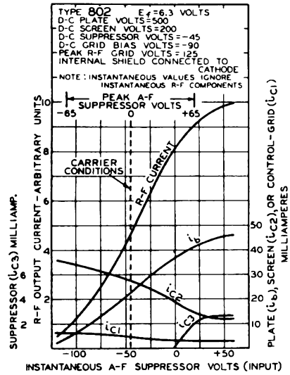
Fig. 11 - Typical suppressor-modulation characteristic.
