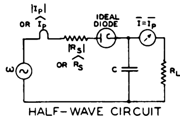
HALF-WAVE CIRCUIT
