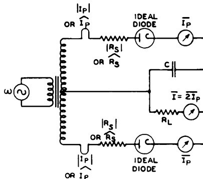
FULL-WAVE CIRCUIT
