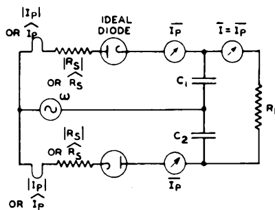
VOLTAGE-DOUBLING CIRCUIT
