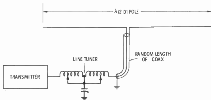
Fig. 4. Use of line tuner.
