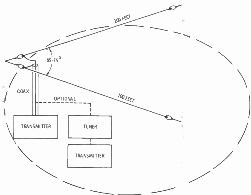
Fig. 64. Multiband 100-footer.
