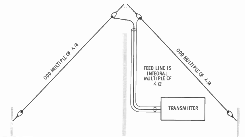
Fig. 28. Basic plan of a resonant and matched long-wire inverted vee.
