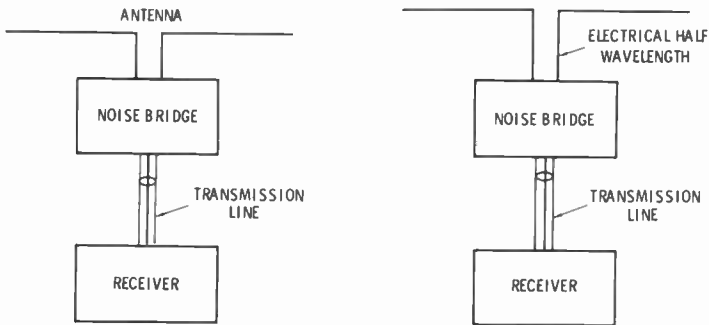
(A) Bridge at feed point of antenna. (B) Bridge at half wave from antenna terminals.
