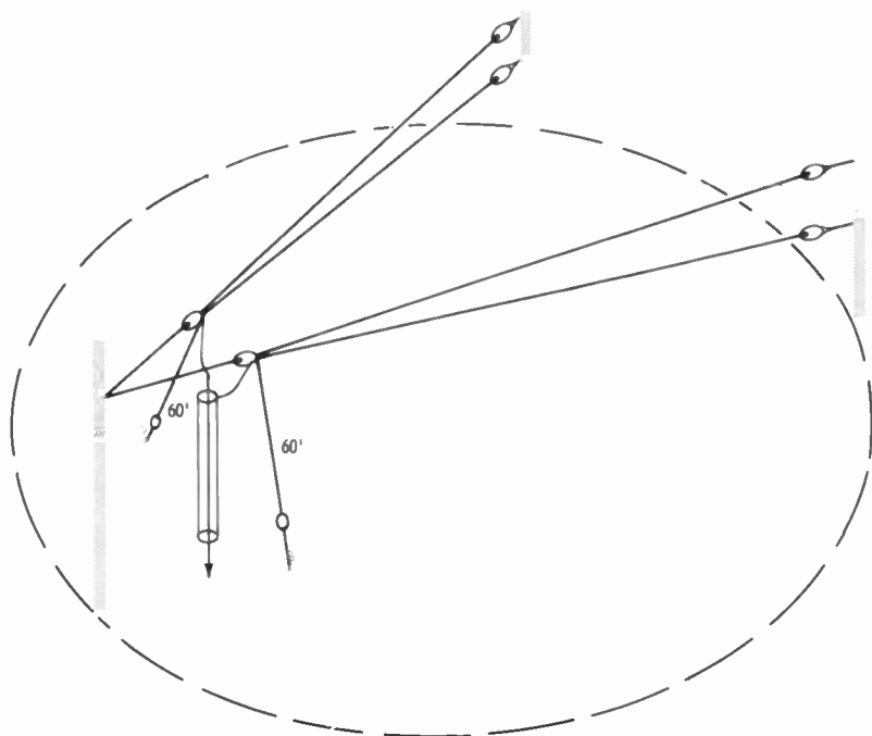
Fig. 66. Short vee-beam antenna of Fig. 65 with an attached 80-meter inverted dipole.
