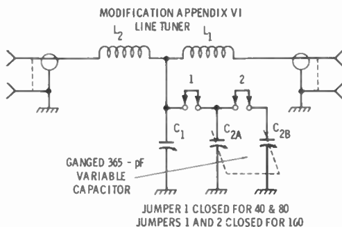
(A) Tuner modification.
