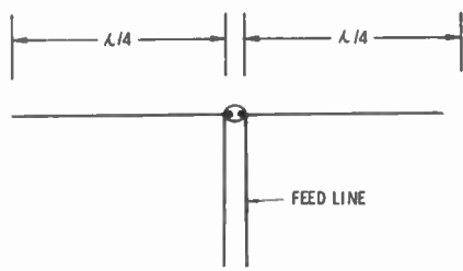
Fig. 1. Half-wavelength dipole antenna.
