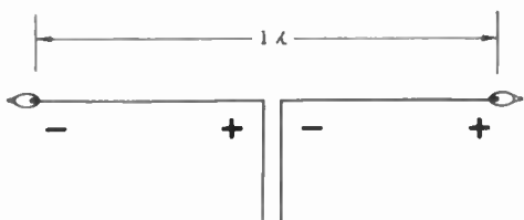
(B) Full-wave dipole.
