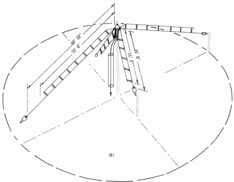
Fig. 27. Inverted dipoles (A) and four-band 15-20-40-80 dipole pairs (B).
