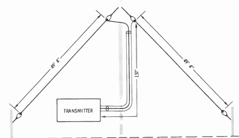
Fig. 29. Twenty-meter long-wire inverted vee—3/4 wavelength on each leg.
