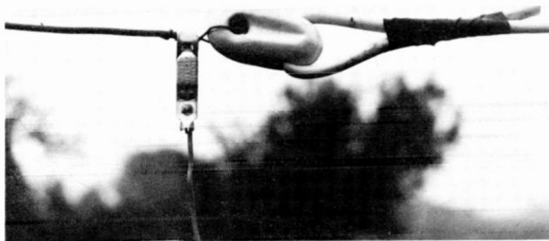
Fig. 18. Clip-on extension to lower resonant frequency of antennas.
