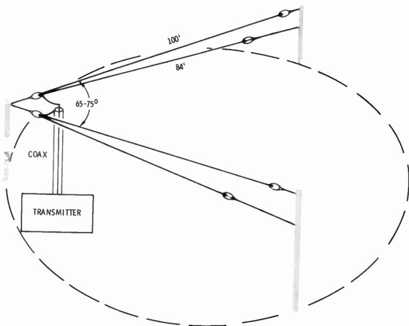
Fig. 65. 10-15-20-40 short vee beam.
