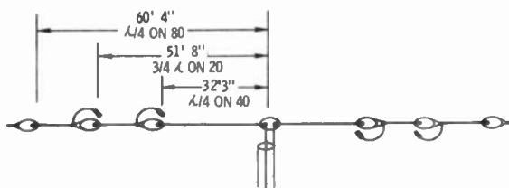
(A) Overall length is used for 80.
