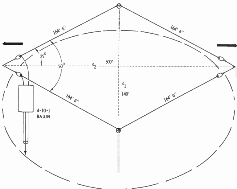
Fig. 77. 10-15 rhombic.
