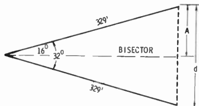
Fig. 69. Vee-beam angles and sides.
