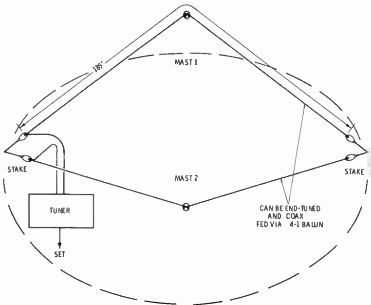
Fig. 96. Two-mast rhombic.
