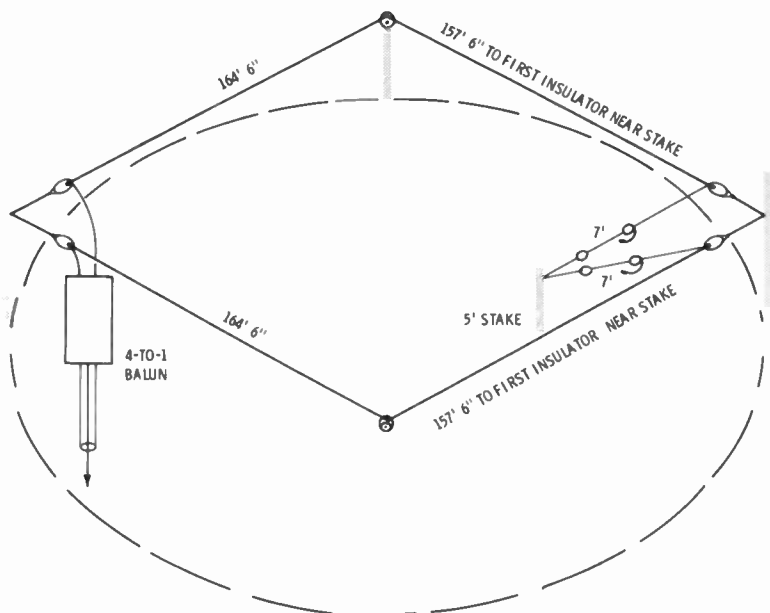
Fig. 79. 10-15-20 end-tuned rhombic.
