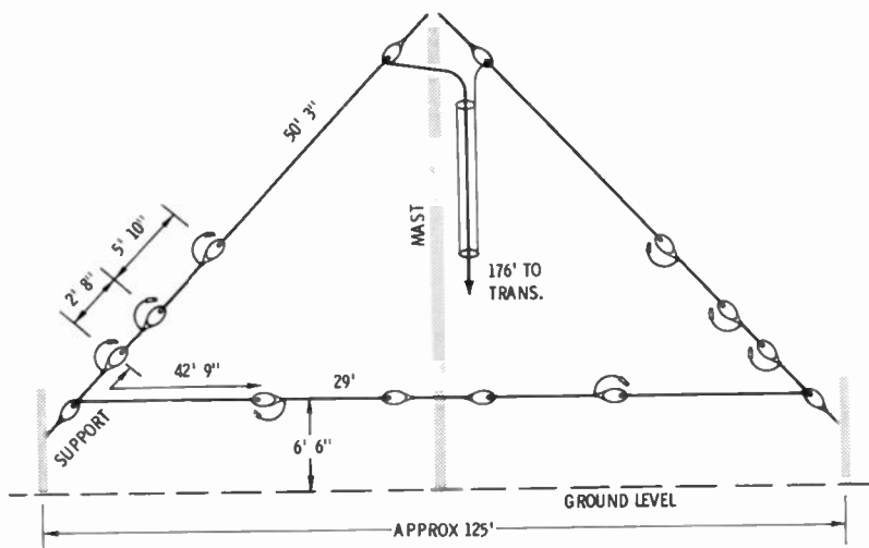
Fig. 34. 6-160 meter inverted dipole and long-wire inverted-vee system.
