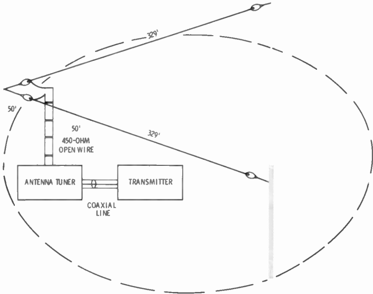
Fig. 72. Use of antenna tuner with vee-beam antenna.
