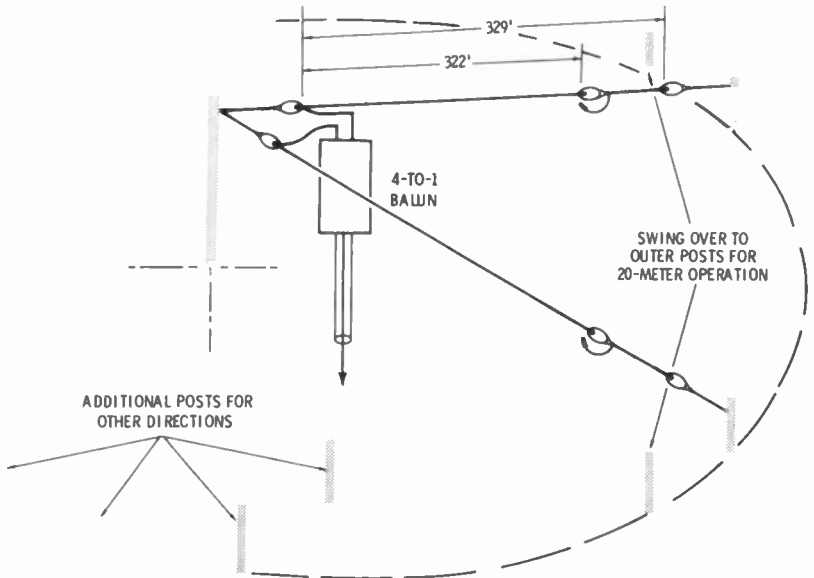
Fig. 74. 10-15-20 sloping end-loaded vee beam.
