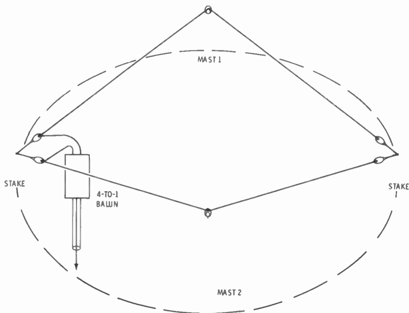
Fig. 95. General plan of a two-mast rhombic.
