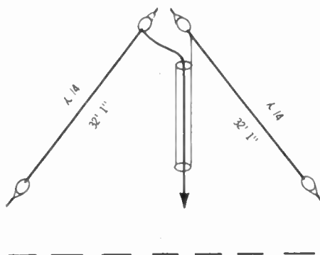
(B) Inverted dipole.
