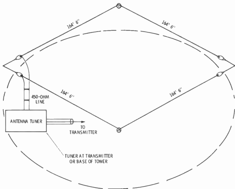
Fig. 82. Rhombic with open-wire line and antenna tuner.
