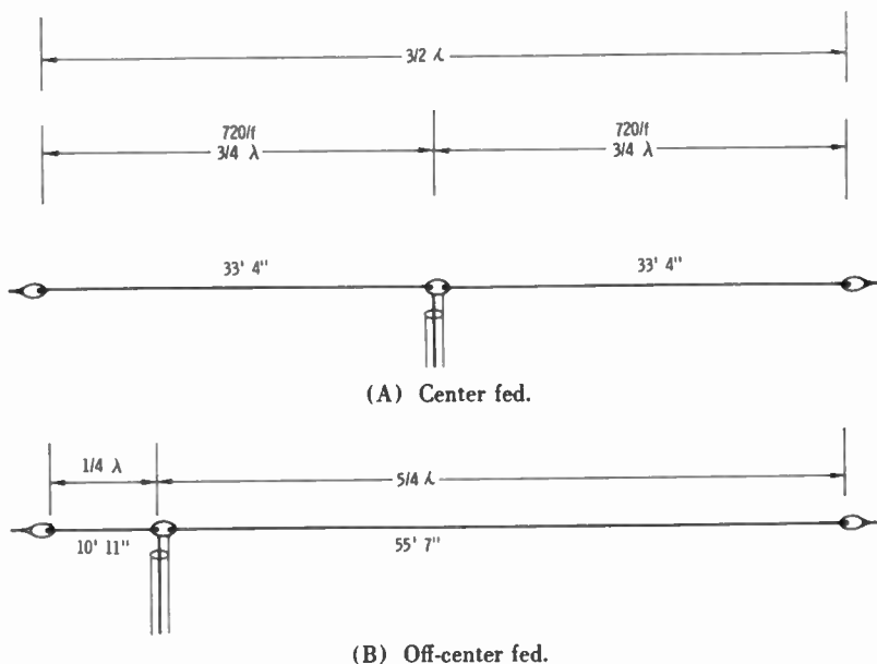
Fig. 22. 3/2 -wavelength antenna.
