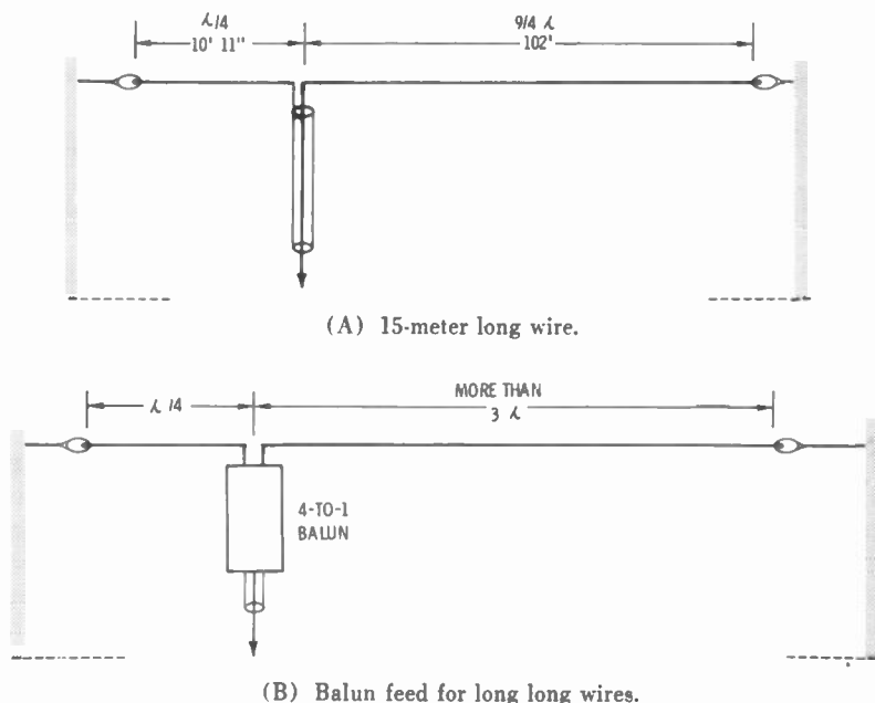
Fig. 44. End-fed long-wire antennas.
