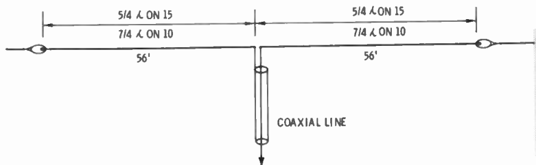
Fig. 43. Long-wire center-fed antenna for 10 and 15 meters.
