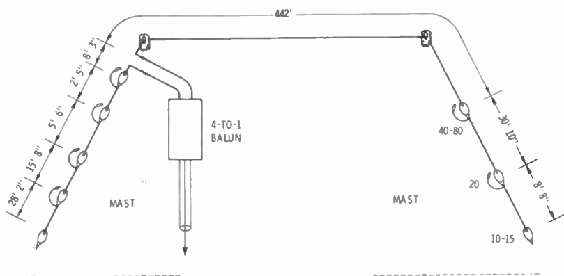
Fig. 86. End-tuned very-long wire.
