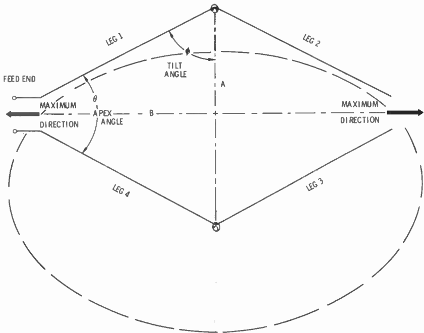
Fig. 76. Resonant rhombic.
