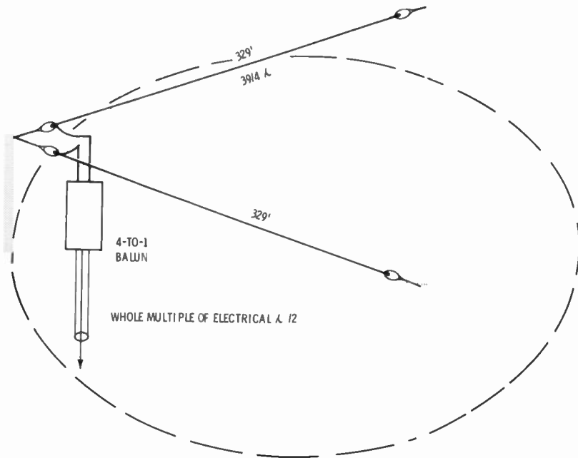
Fig. 68. Ten-meter long vee beam.
