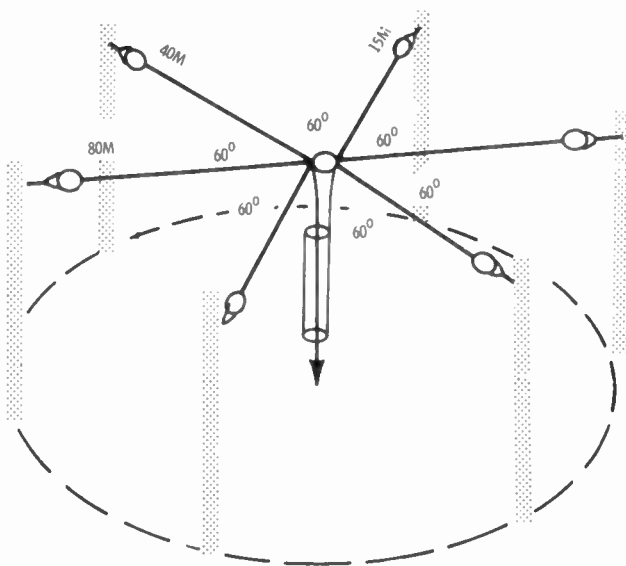
(A) Horizontal dipoles.
