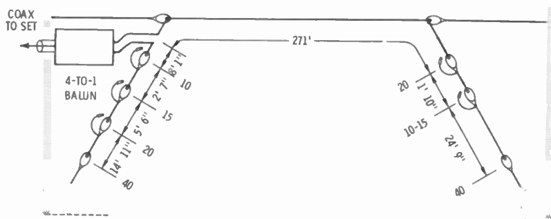
Fig. 46. 10-15-20-40 segmented end-fed long wire.
