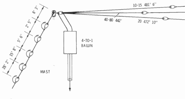
Fig. 87. Long-wire 5DXCC special.
