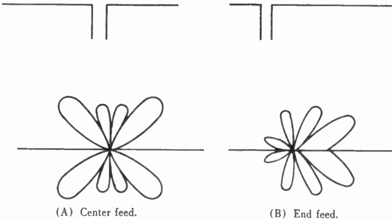
Fig. 41. Lobes of 2-wavelength long wire.
