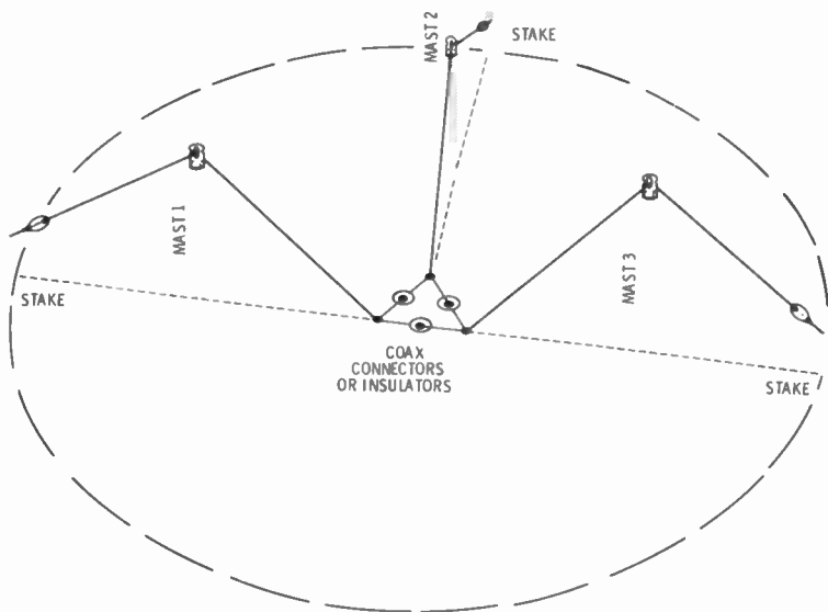
(A) Three mast.
