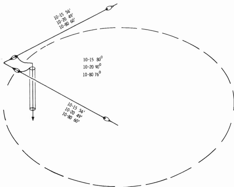
Fig. 60. Duo-band short vee beams.
