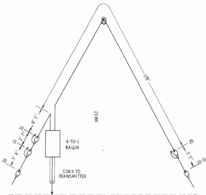
Fig. 51. 10-15-20 inverted-vee beam.
