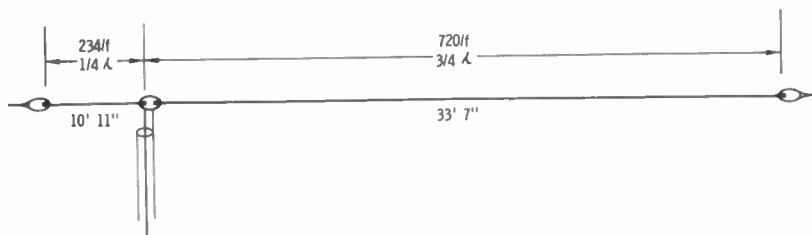
Fig. 20. One-wavelength antenna.
