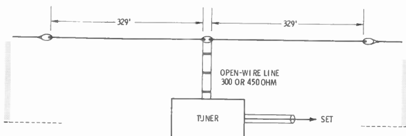
(C) Open-wire line with tuner.
