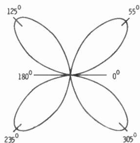
Fig. 19. Comparisons in length and horizontal pattern of horizontal dipole and one-wavelength antennas.
