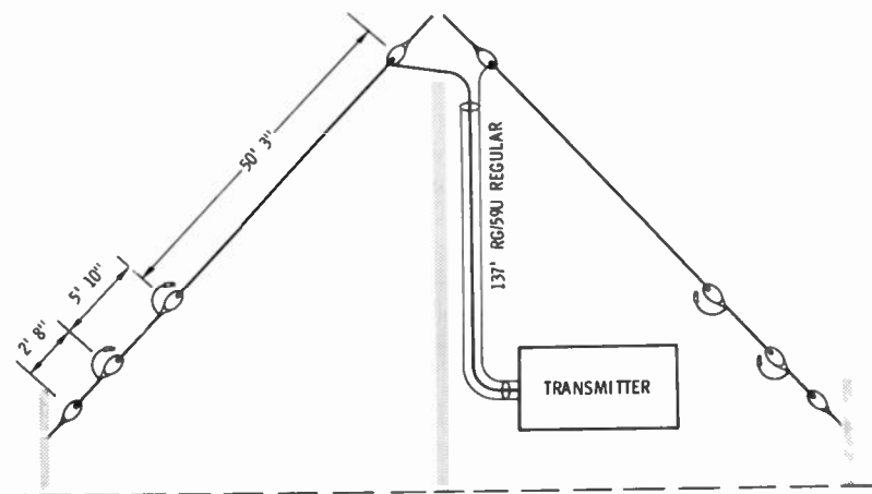
Fig. 33. 10-15-20 sideband long-wire inverted vee.
