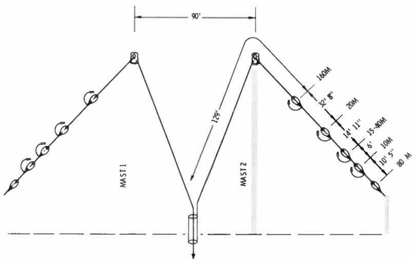
Fig. 91. Two-mast end-tuned inverted vee.
