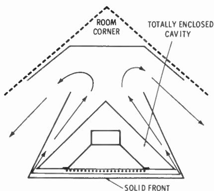
Fig. 3-10. A folded corner horn.
