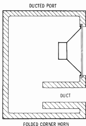
Fig. 3-12. A modified version of the bass-reflex speaker enclosure with a ducted port.
