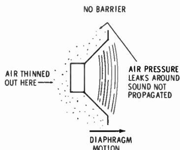
Fig. 3-8. The cancelling effect of sound when no baffle is employed with a speaker.
