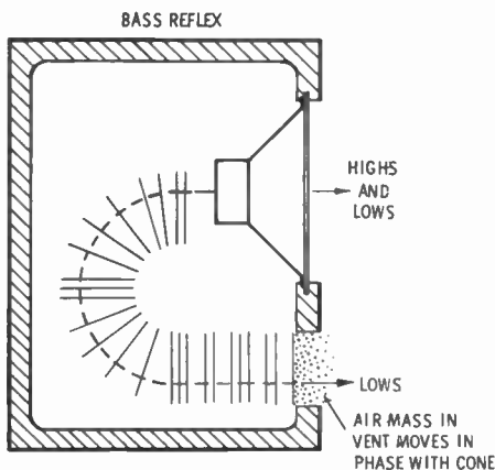
Fig. 3-11. A bass-reflex enclosure.
