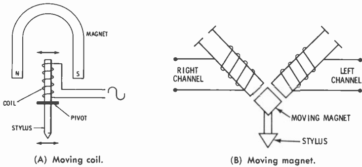
Fig. 2-9. Operating principles of magnetic pickup cartridges.
