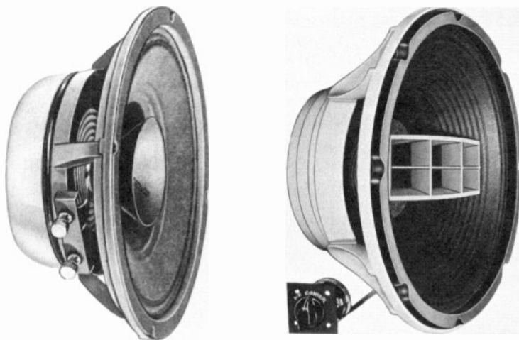
(A) Single-cone 8" midrange.
