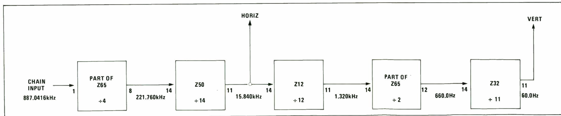
FIGURE 6. Divider Chain Block Diagram
