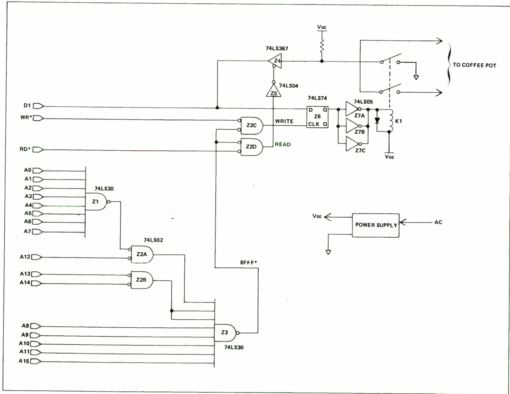
FIGURE 20. Memory Mapped Coffee Pot Control
