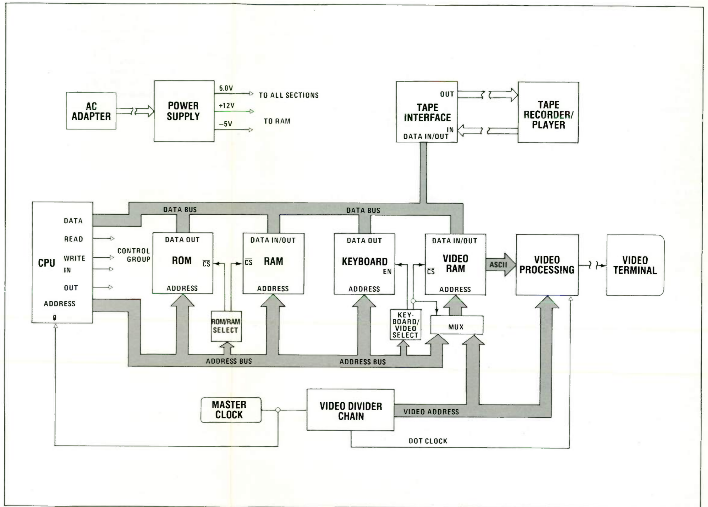
FIGURE 1. TRS-80 System Block Diagram
