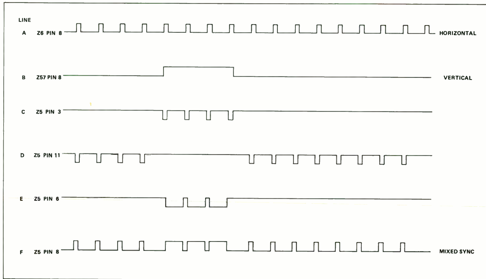
FIGURE 8. Sync Mixing
