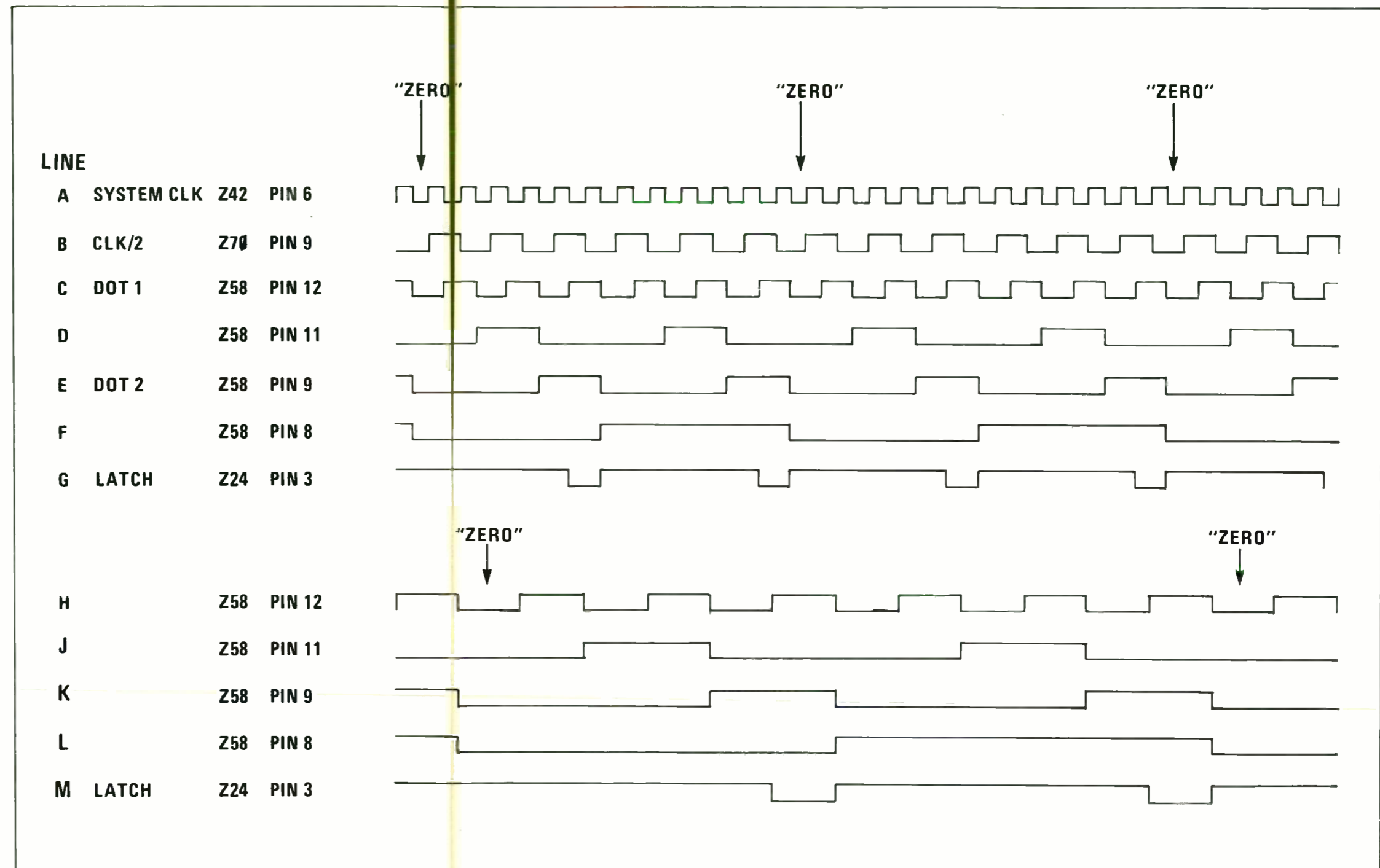
FIGURE 5. Input Conditioning Waveform
