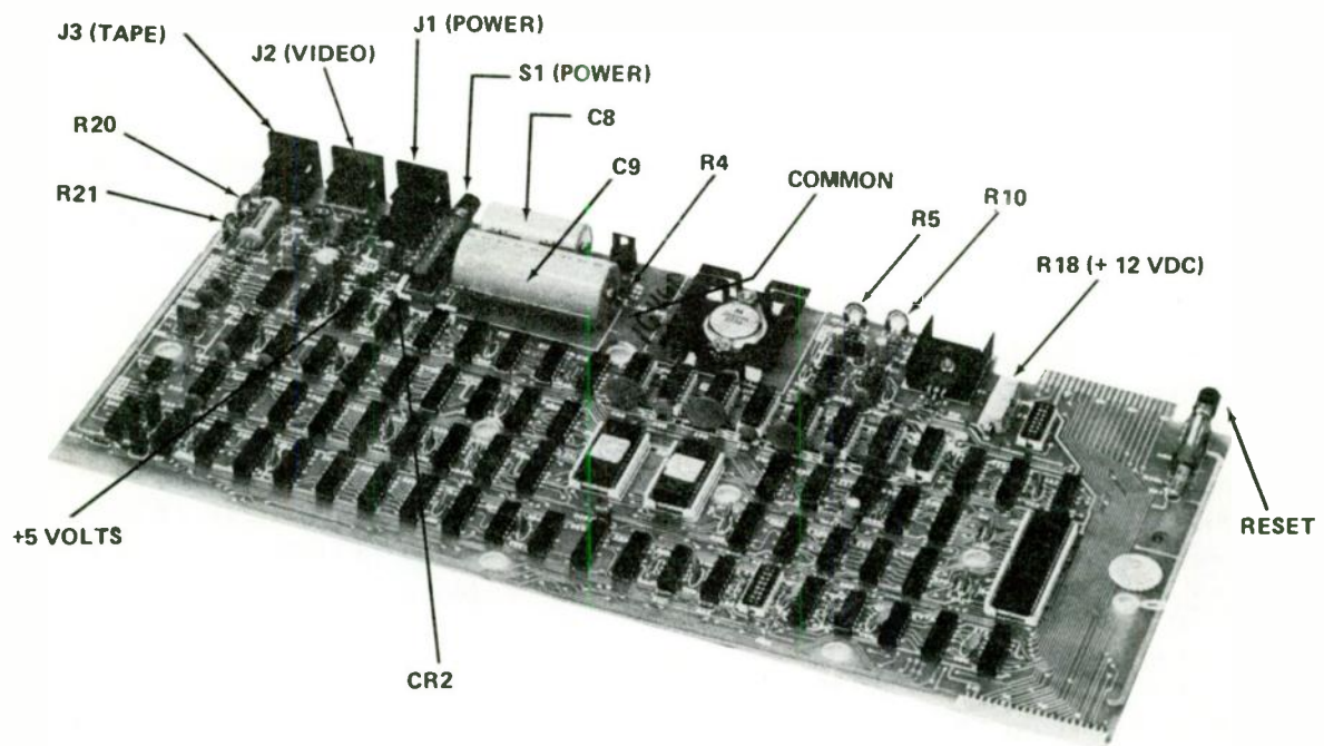
FIGURE 2. LOGIC BOARD
