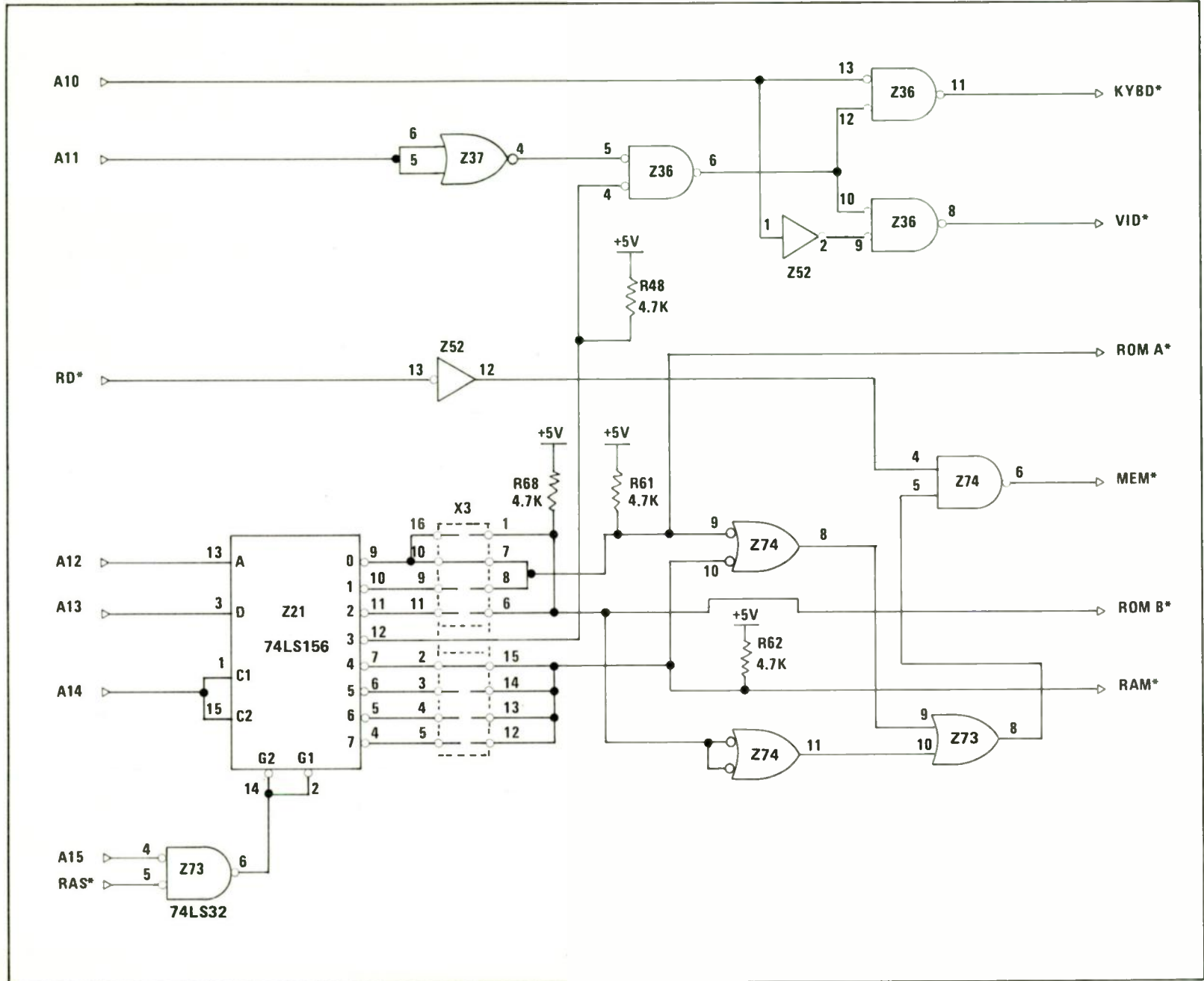
FIGURE 3. Address Decoder
