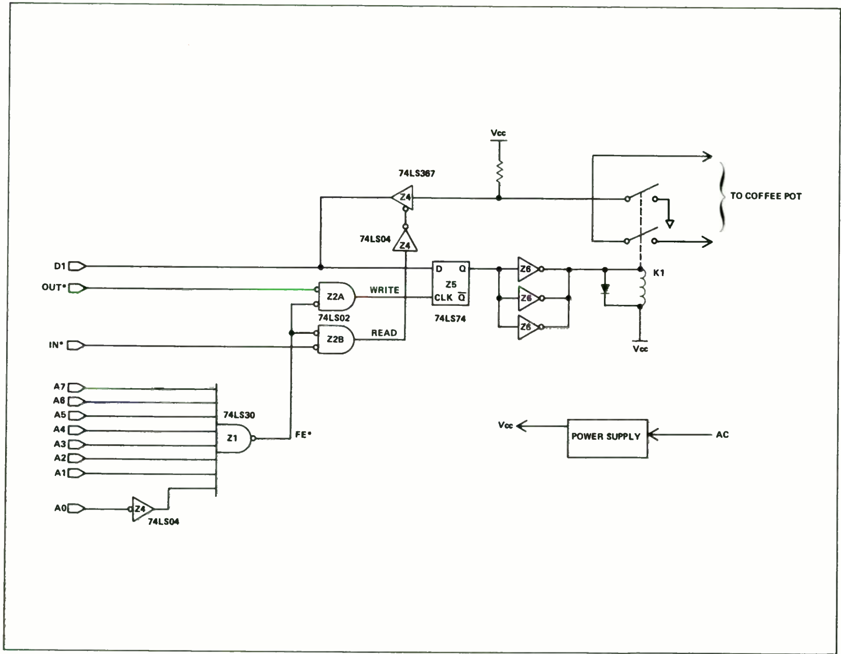
FIGURE 21. Port Based Coffee Pot Control
