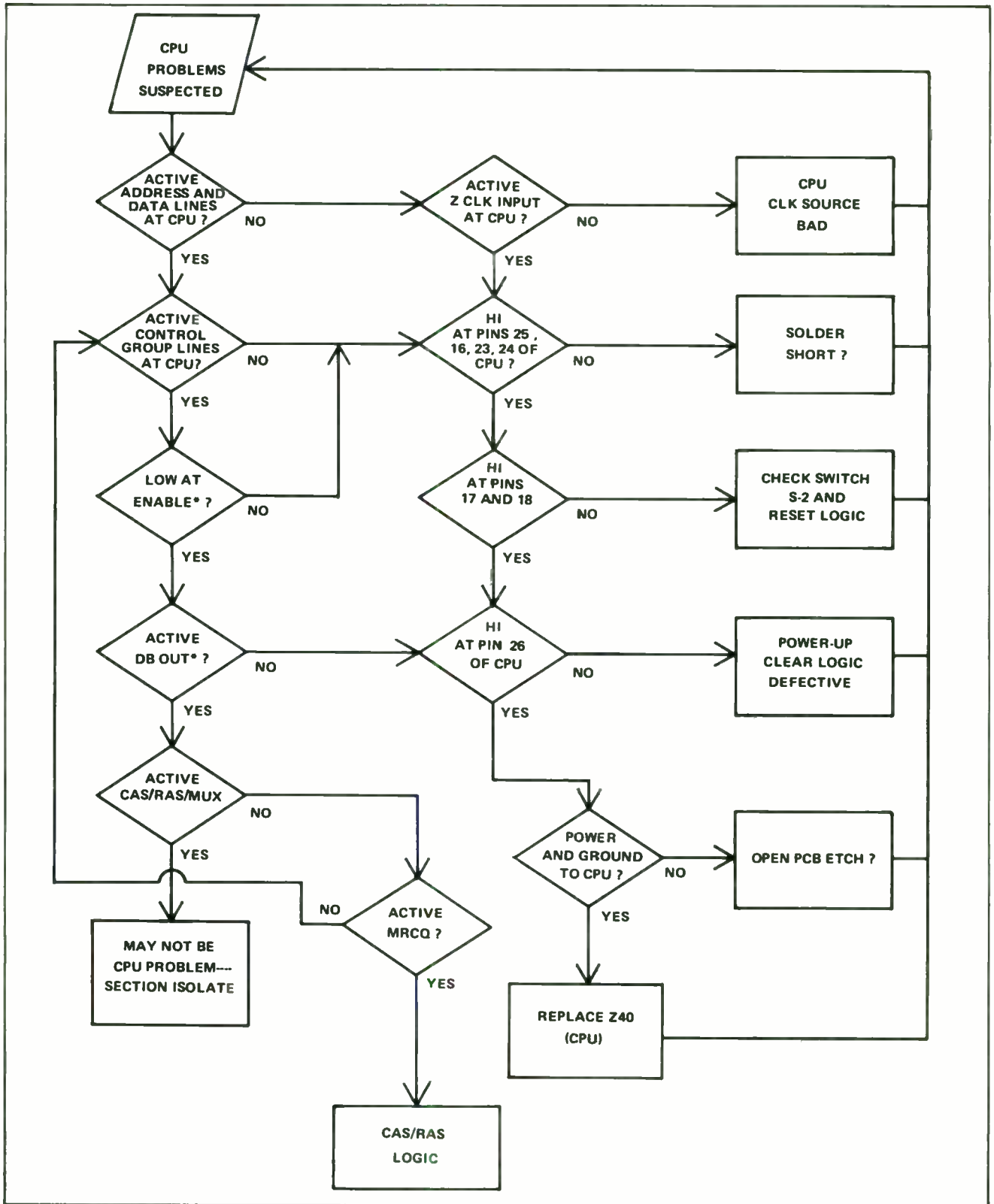
FIGURE 17. CPU Flowchart
