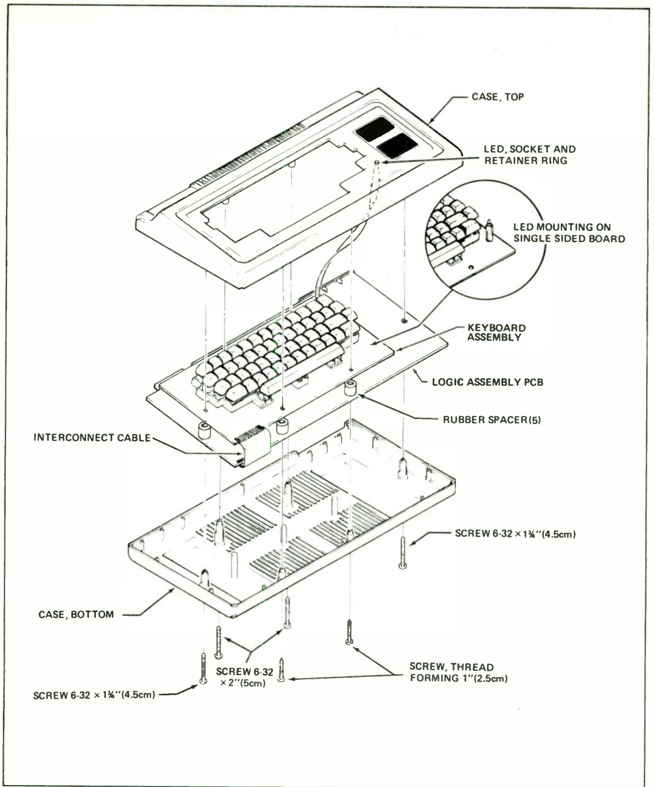
FIGURE 14. Exploded View
