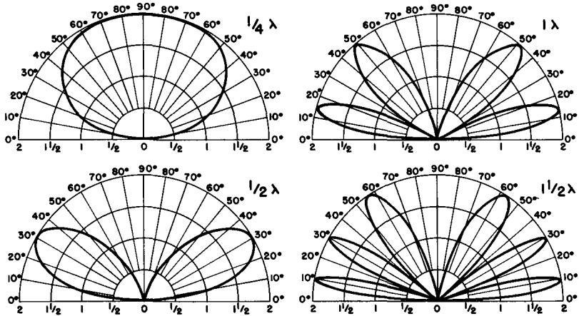
HORIZONTAL ANTENNA
