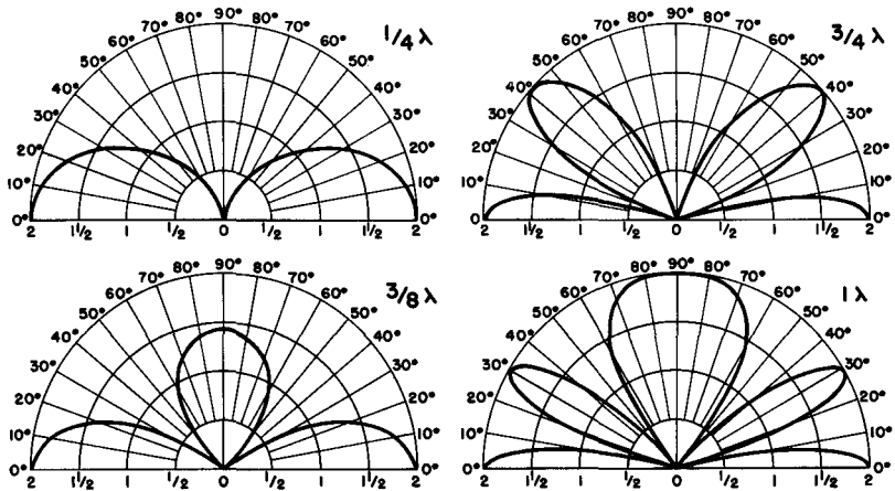
VERTICAL ANTENNA
