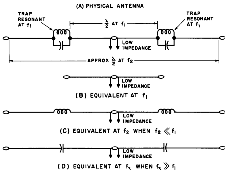
Fig. 55. Typical trap-type multi-frequency antenna, showing its equivalent circuit at several different frequencies.
