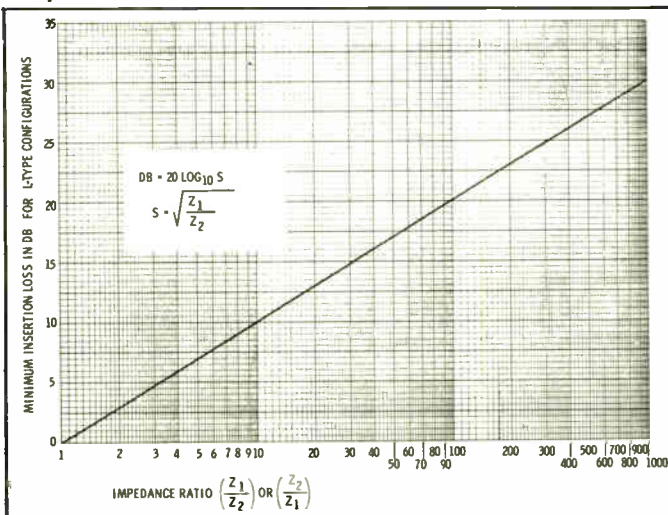
Fig. 7. Minimum loss graph for L-type attenuators.
