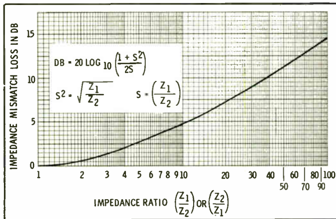
Fig. 1. Loss in level because of impedance mismatch.
