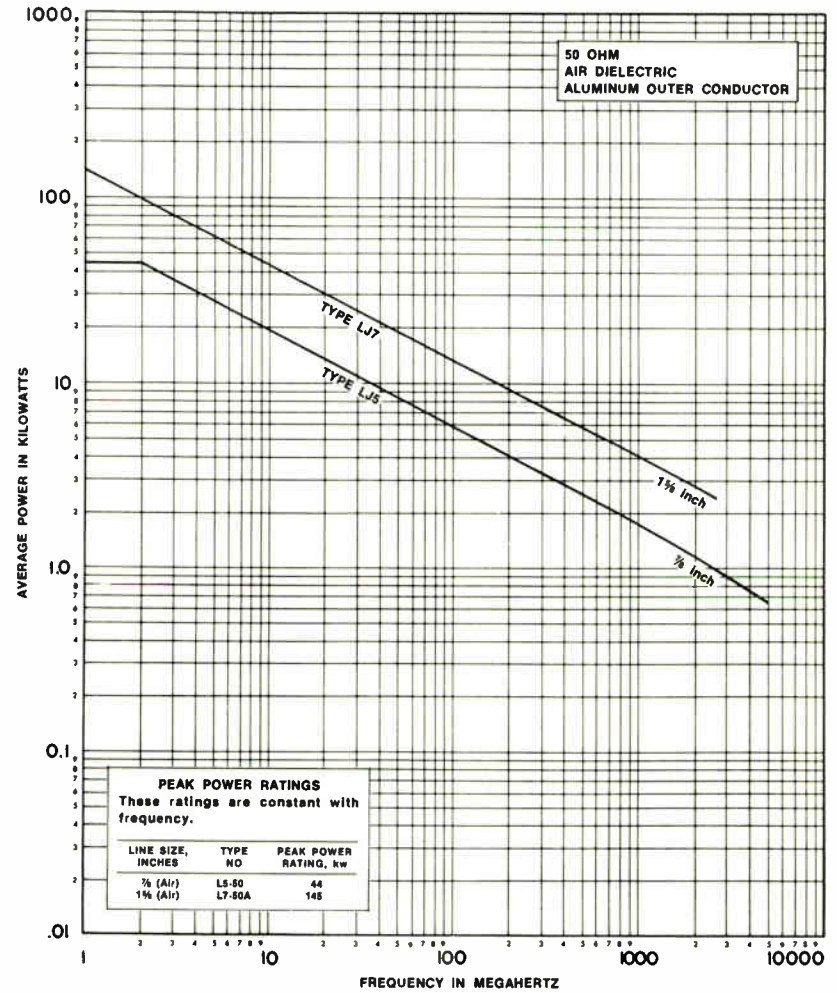
Power Rating of Heliax Coaxial Cables
