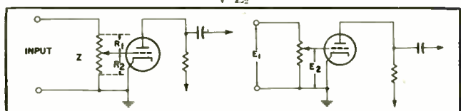
Fig. 11. Grid-circuit potentiometers.
