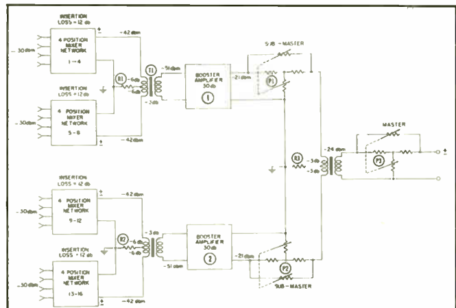
Fig. 20. A 16-position hybrid-coil mixer network.
