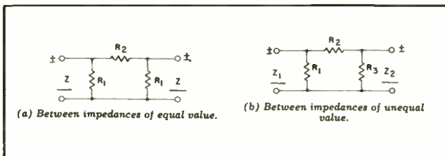
Fig. 9. Pi-type configurations.
