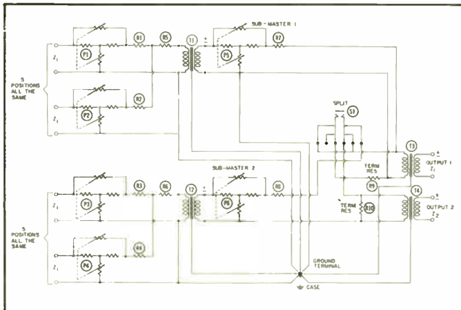
Fig. 19. A 10-position, split mixer network with keyswitch for combining the two sections into a single network.
