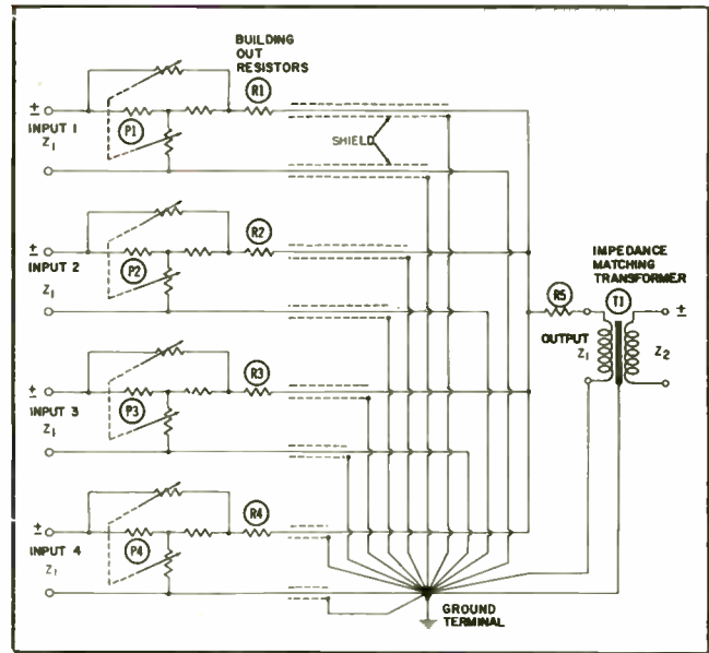
Fig. 18. A four-position, parallel-connected, unbalanced mixer network.
