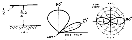
Horizontal Antenna, \frac{3}{4} Wave High. Radiates Mainly Upward.
