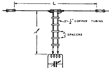
COLLINS MULTI-BAND ANTENNA
