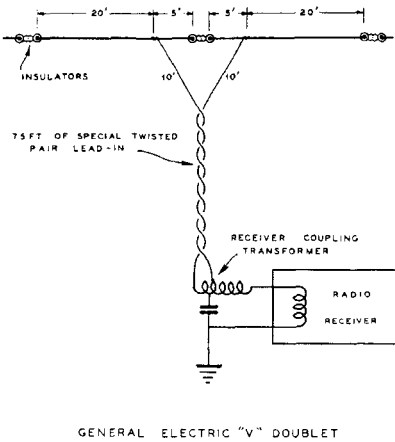
GENERAL ELECTRIC "V" DOUBLET
