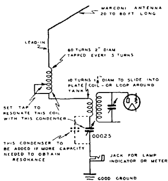
Fig. 46 Loading System for Short Marconi Antenna for Boats, Aeroplanes, Etc.
