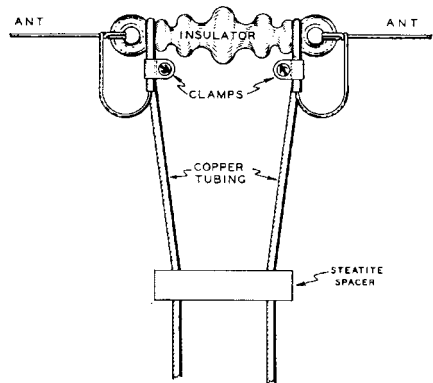
COLLINS MULTI-BAND ANTENNA
