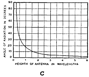
Fig. 68 Diamond and "V" Antenna Design Curves.
