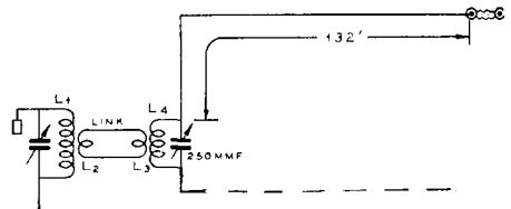
Fig. 35 80 Meter End Fed Antenna with Counterpoise for 160 Meter Operation.
