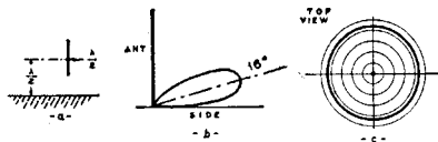
Half Wave Antenna, Same Height as Full Wave Antenna Above. Here the Radiation Is Known as 16-Degree "Low Angle" Radiation.
