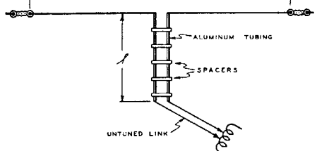
JOHNSON "Q" ANTENNA
