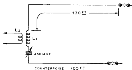
Fig. 73 L2—Final Plate Coil.
