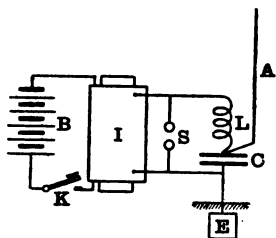
FIG. 14.—BRAUN'S RADIATOR. B, battery; I, induction coil; K, key; S, spark-gap; L, inductance coil; C, condenser; A, aerial.
