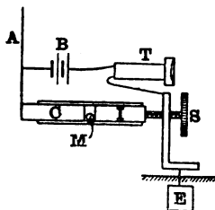
FIG. 17.—ITALIAN NAVY SELF-RESTORING KUMASCOPE. C, carbon plug; I, iron plug; M, mercury globule; A, aerial; B, battery; T, telephone; S, adjusting screw.
