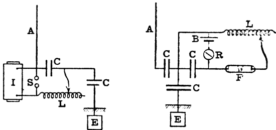
FIG. 25.—LODGE-MUIRHEAD SYNTONIC RECEIVER. I, induction coil; S, spark gap; A, aerial; CC, condensers; E, earth plate; R, relay; L, variable inductance; F, flings tube; B, battery.
