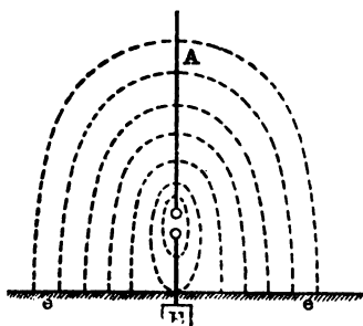
FIG. 4.—LINES OF ELECTRIC STRAIN (DOTTED LINES) EXTENDING BETWEEN A MARCONI AERIAL, A, AND THE EARTH as BEFORE DISCHARGE.
