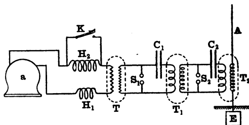
FIG. 15. — ALTERNATING-CURRENT DOUBLE-TRANSFORMATION POWER PLANT FOR GENERATING ELECTRIC WAVES (Fleming). a , alternator; H_1H_2 , choking coil; K , signalling key; T , step-up transformer; S_1S_2 , spark-gap; C_1C_2 , condensers; T_1T_2 , oscillation transformers; A , aerial; E , earthplate.
