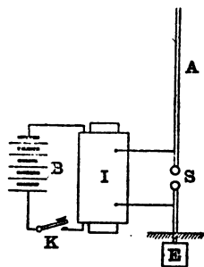
FIG. 3.—SIMPLE MARCONI RADIATOR. B, battery; I, induction coil; K, signalling key; S, spark gap; A, aerial wire; E, earth plate.
