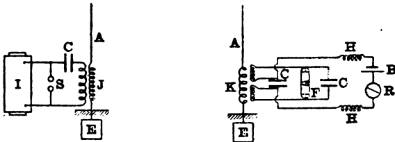
FIG. 23.—MARCONI TRANSMITTER AND RECEIVER. I, induction coil; A, aerial; E, earth plate; HH, choking coils; S, spark gap; J, transmitting jigger; K, receiving jigger; B, relay; C, condenser; F, filings tube; B, battery. Many practical details are omitted.
