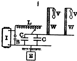
FIG. 22.—SEIBT'S APPARATUS FOR EXHIBITING ELECTRIC RESONANCE. I, induction coil; S, spark gap; CC, condensers; L, variable inductance; E, earth plate; WW, wire spirals; VV, vacuum tubes.
