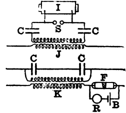
FIG. 21.—BRAUN'S NON-EARTHED RECEIVER. I, induction coil; CC, condensers; S, spark gap; J, transmitting jigger; K, receiving jigger; F, flings tube; R, relay; B, battery.
