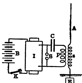
FIG. 9.—MARCONI-BRAUN SYSTEM OF INDUCING ELECTROMOTIVE FORCE IN AN AERIAL, A, B, battery; K, key; I, induction coil; S, spark gap; C, Leyden jar; E, earth plate; ps, oscillation transformer.
