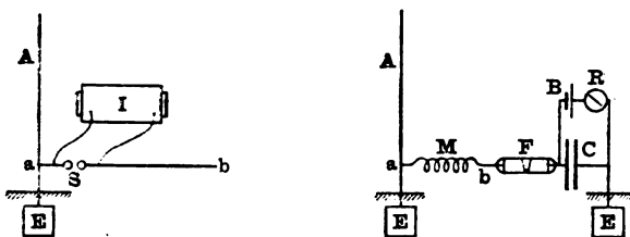
FIG. 24.—SLABY-ARCO SYNTONIC TRANSMITTER AND RECEIVER. I, induction coil; M, multiplier; B, battery; A, aerial; F, flings tube; R, relay; E, earth plate; C, condenser.
