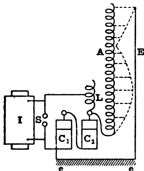
FIG. 11.—HARMONIC OSCILLATIONS IN LONG SOLENOID SHOWN WITH SEIBT'S APPARATUS.
