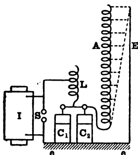
FIG. 10.—SEIBT'S APPARATUS FOR SHOWING STATIONARY WAVES IN LONG SOLENOID A. I, induction coil; S, spark gap; L, inductance coil; C 1 C 2 , Leyden jars; E, earth wire.
