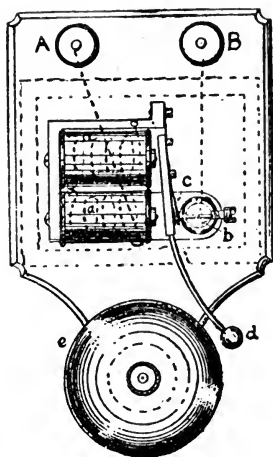
FIG. 11 ELECTRIC BELL (ORDINARY PATTERN)
