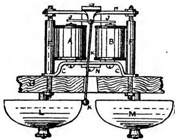
FIG. 12. (Scale \frac{1}{3} ) MAGNETO RINGER
