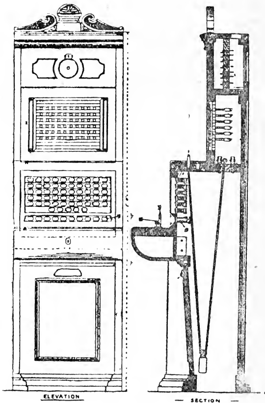
FIG. 42 (Scale \frac{1}{16} ) STANDARD SWITCHBOARD
