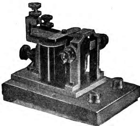
FIG. 18 P.O. "PONY" SOUNDER
