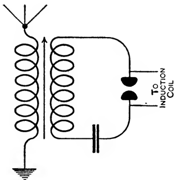
FIG. 62 "INDUCTIVE" COUPLING
