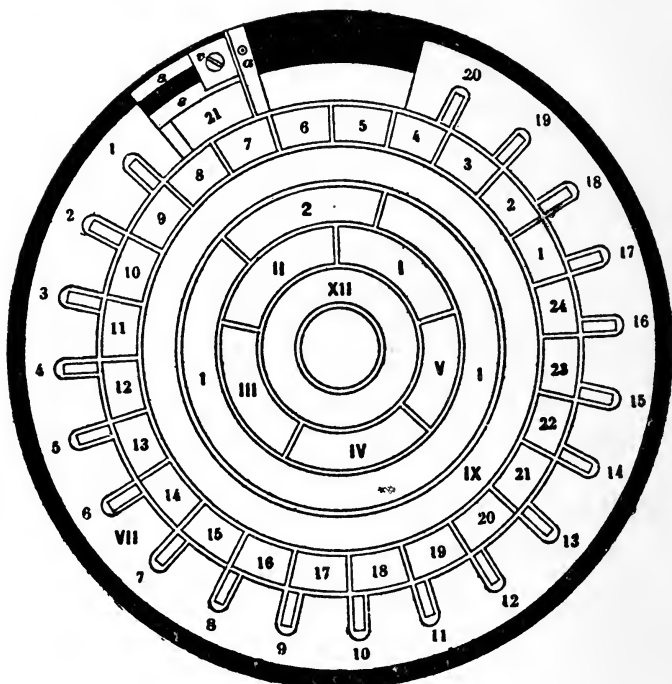
FIG. 28 BAUDÔT MULTIPLEX FRONT PLATE RINGS AND SEGMENTS
