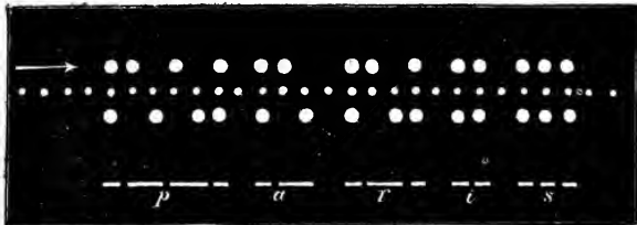
FIG. 25 PERFORATIONS FOR WHEATSTONE AUTOMATIC
