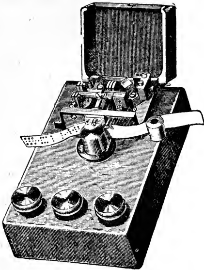
FIG. 24 WHEATSTONE PERFORATOR
