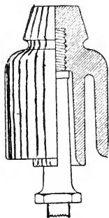
FIG. 54 CORDEAUX INSULATOR
