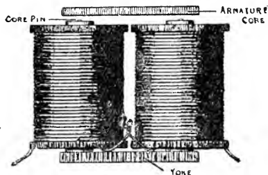
FIG. 4 ELECTRO-MAGNET
