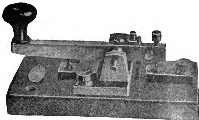
FIG. 17 SINGLE-CURRENT MORSE KEY
