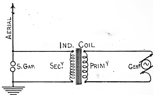
FIG. 61 MARCONI'S "PLAIN-AERIAL" ARRANGEMENT
