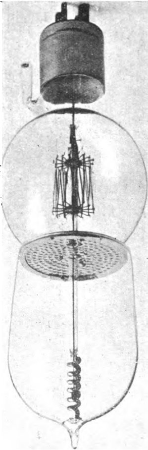
FIG. 72.—Perspective view of Lieben-Reisz Thermionic Relay.
