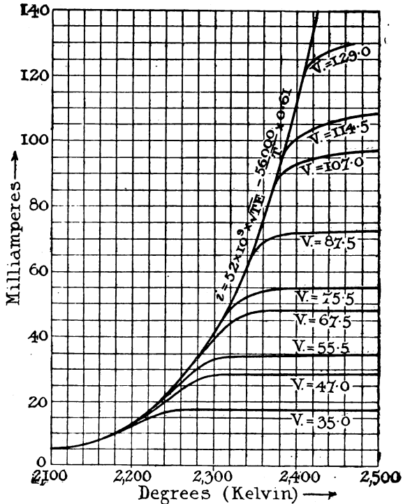
FIG. 40.—Curves given by Dr. Langmuir showing the Thermionic Current of a High Vacuum Valve in terms of absolute Temperature (Kelvin) Degrees for various Impressed Voltages.
