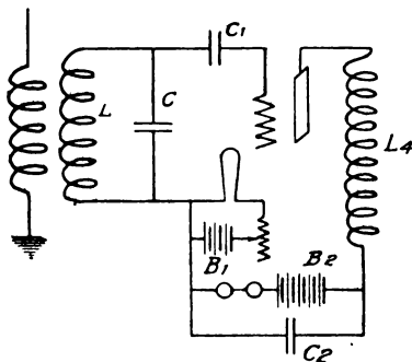
FIG. 74.—Armstrong's Second Method of Re-enforcing the Plate Oscillations in Three-electrode Valve Receiver Circuits. (In this diagram and that in Fig. 73 the bulb of the valve is not shown, but the filament, grid, and plate are denoted by a loop, zig-zag and rectangle respectively.)
