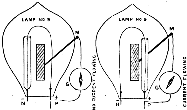
FIG. 8.—Glass or Metal Tube surrounding one leg of horseshoe carbon filament in a glow lamp to show the annulment of the "Edison effect" when it surrounds the negative leg.
