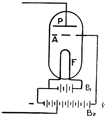
FIG. 87.—Diagram showing the Principle of the Dynatron. F, Tungsten Filament rendered Incandescent by Battery, B 1 . A, Perforated Anode and P, Plate Anode.
