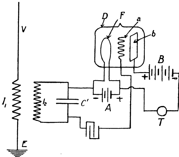
FIG. 58.—LEE DE FOREST'S THREE-ELECTRODE Audion OF 1907. D, Glass Bulb. F, Filament. a, Grid. b, Plate. A, Filament Battery. B, Plate Battery. T, Telephone.
