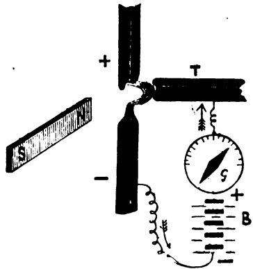
FIG. 15.—An experiment with the electric arc having a third carbon to show that a current of negative electricity can pass under low E.M.F. between the negative terminal of the arc and the third carbon electrode.
