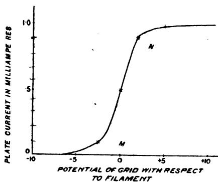
FIG. 59.—Characteristic Curve of Three-Electrode Thermionic Valve
