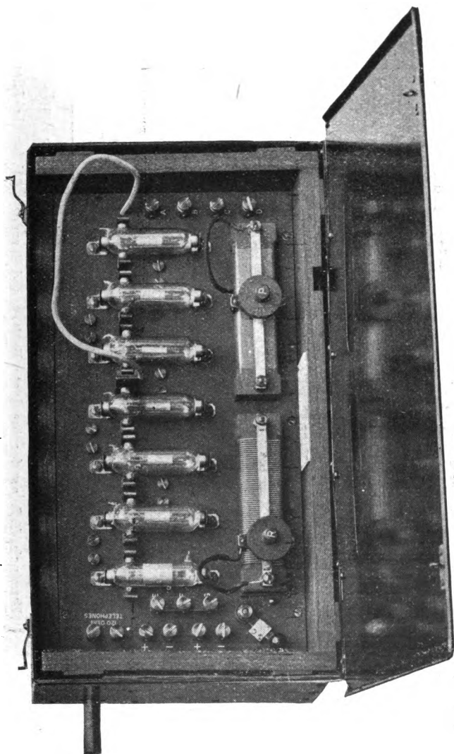
FIG. 129.—The Marconi Company's Valve Amplifier and Detector, Type 55.
