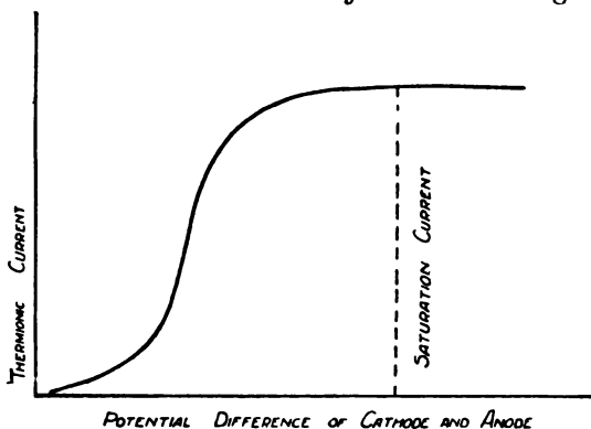
FIG. 23.—Characteristic or Volt-ampere Curve of a highly rarefied gas or nearly perfect vacuous space.
