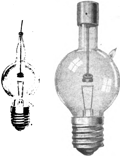
FIG. 45.—Two-ampere and Six-ampere Tungars or Low Vacuum Argon-filled Oscillation Rectifying Valves.
