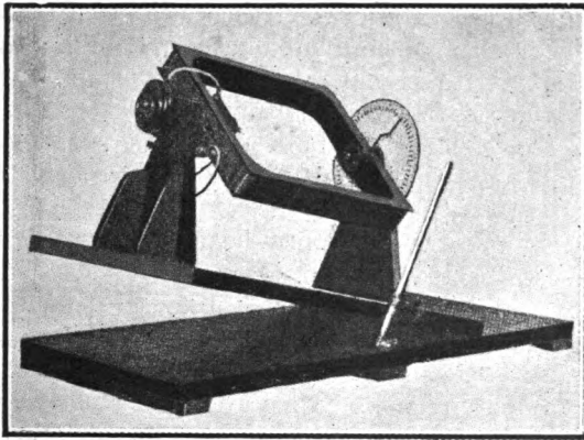
FIG. 49.—Photograph showing details of construction of the Tilting Receiving Coil, L_2 .
