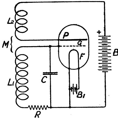
FIG. 144.—Typical Thermionic Circuits for Auto-production of Oscillations.
