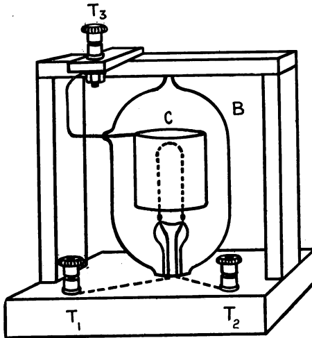
FIG. 27.—FLEMING OSCILLATION VALVE. B, MOUNTED ON WOODEN STAND.
