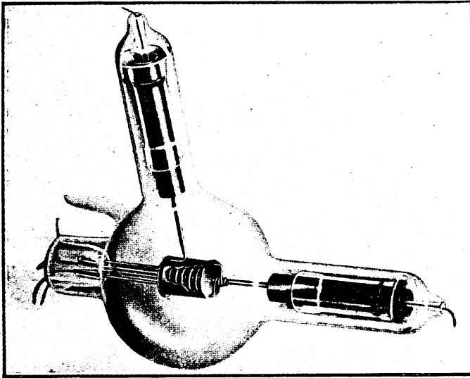
FIG. 88.—Perspective View of the Dynatron.
