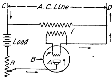
FIG. 46.—Scheme of Connections for using Tungar Rectifying Valve to Rectify a Low-frequency Alternating Current.
