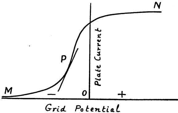
FIG. 94.—Characteristic Curve of a Three-electrode Thermion.
