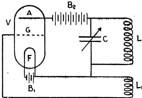
FIG. 83.—Scheme of Circuits for using a Three-electrode Valve, V, as a Generator of Oscillations by inter-coupling Grid and Plate Circuits by Mutual Inductance Coils, L , L_1 .
