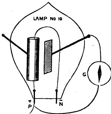
FIG. 9.—Incandescent Lamp with horseshoe carbon filament and metal cylinder surrounding one leg of filament to show the "Edison effect."
