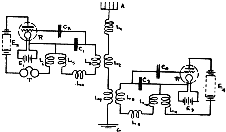
FIG. 115.—Heterodyne Method of Reception for Undamped Waves Employing a Three-electrode Valve to Produce the Local Oscillations required for "Beating" with the Incoming Oscillations. (J. J. Hogan.)
