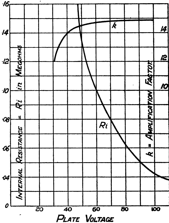
FIG. 143.—Curves representing the Variation of Amplification Factor k , and Internal Resistance R_i , of a Thermion.
