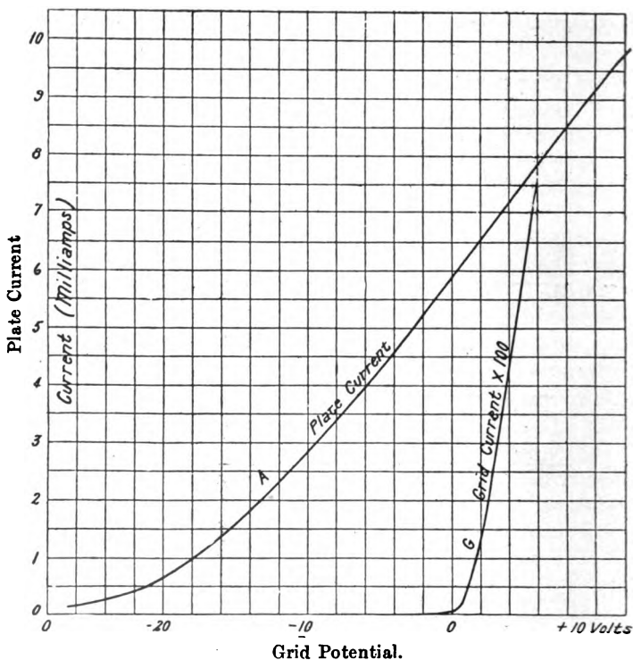
Fig. 65.—Characteristic Curves of High Vacuum Three-electrode Thermionic Valve Detector, called a small Pliotron.
