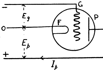
FIG. 95.—CONVENTIONAL DIAGRAM REPRESENTING A THREE-ELECTRODE THERMION.
