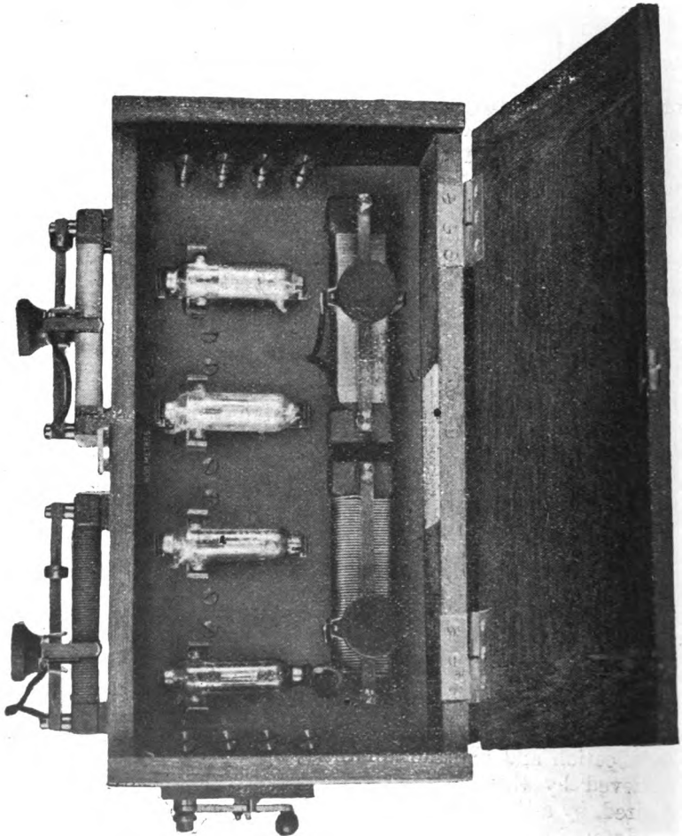
FIG. 128.—The Marconi Company's Valve Amplifier and Detector, Type 50.
