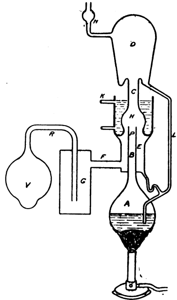
FIG. 54.—Irving Langmuir High-Vacuum Boiling Mercury Pump.
