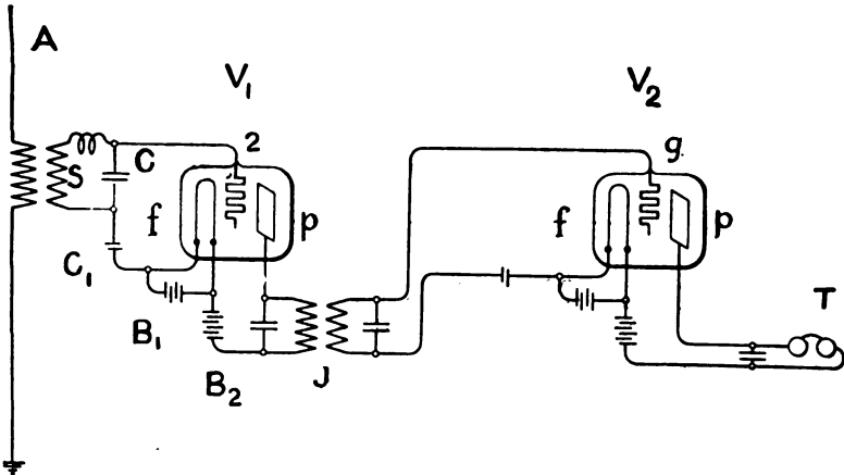
FIG. 78.—Two Three-electrode Amplifiers, V_1 and V_2 , worked in Cascade, being Coupled by an Oscillation Transformer, J .
