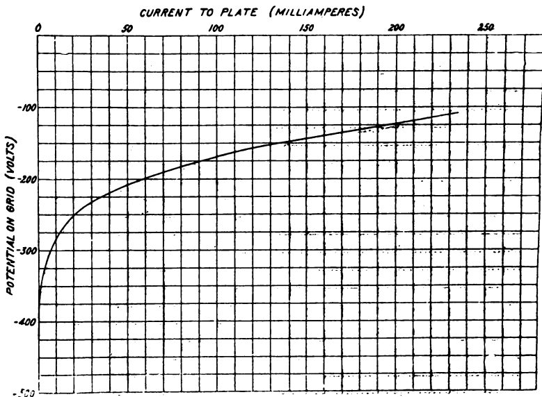
FIG. 70.—Part of Characteristic Curve of Large Pliotron.
