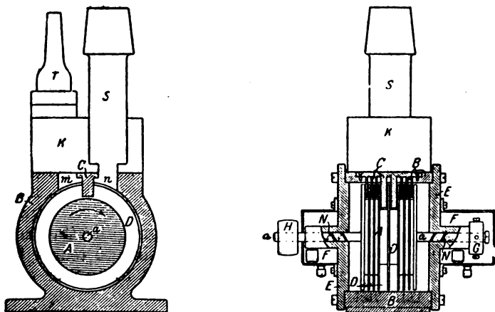
FIG. 50.—Sections of a Gaede Molecular Pump.
