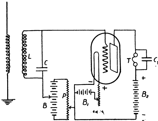
FIG. 61.—Scheme of Connections for Using the Three-electrode Valve as a Simple Oscillation Detector. (E. H. Armstrong.)
