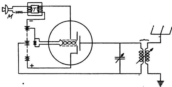
FIG. 127.—Scheme of Circuits for a Radiotelephonic Transmitter Employing a Pliodynatron, made by the General Electric Company of U.S.A., as Oscillation Generator.
