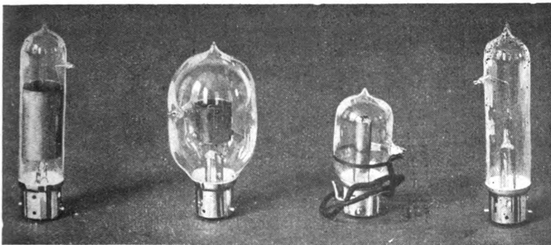
FIG. 28A.—Photographs of various types of Fleming Valve.
