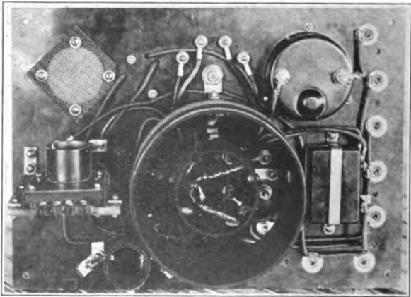
Mounting of Apparatus on Under Side of Panel
