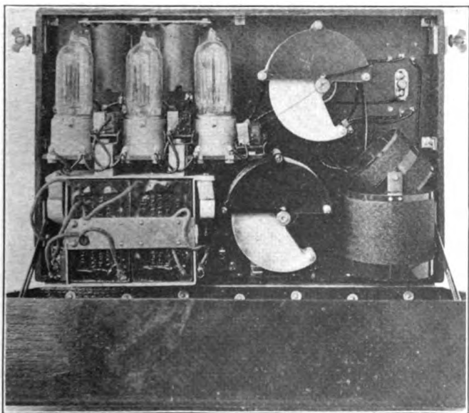
FIG. 28.—Mounting of Apparatus on the Panel of Set Box Type BC-20.
