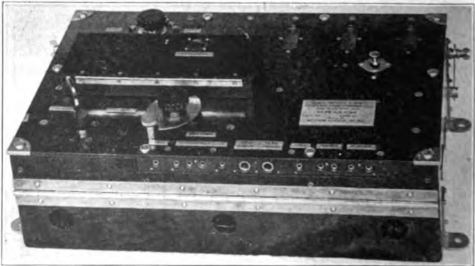
FIG. 7.—Operating Panel of Set Box Type BC-11 Used in Set Type SCR-68, Showing Jacks Along the Bottom Edge.
