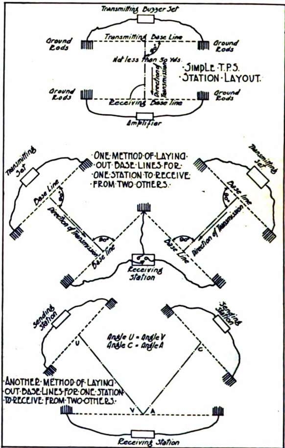
Fig. 1—How to Lay Out Base Lines.
