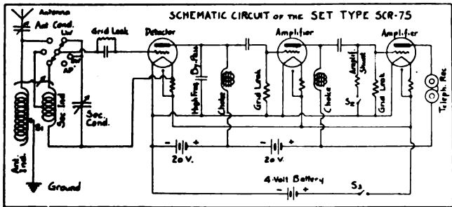
FIG. 26.—Schematic Circuit Diagram of Set Type SCR-75.
