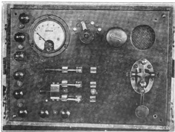
Operating Panel of Type SCR-69 Transmitting Set
