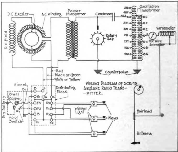
Fig. 2—Schematic Wiring Diagram of Type SCR-73 Set.
