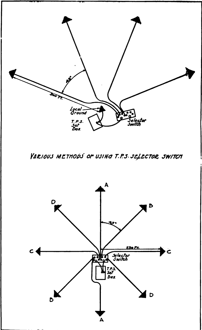
Fig. 6—Methods of Laying Out Central T.P.S. Stations.
