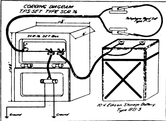
Fig. 4—Cording Diagram of Type SCR-76 Set.
