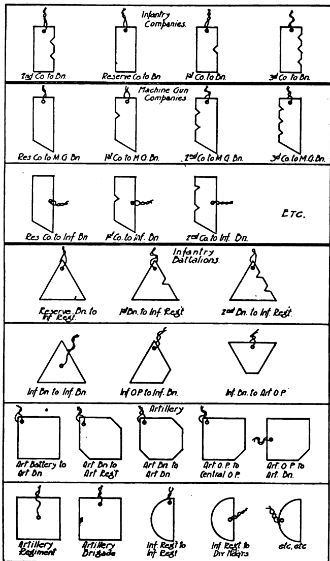
Scheme No. 1 for Tagging Trench Lines
