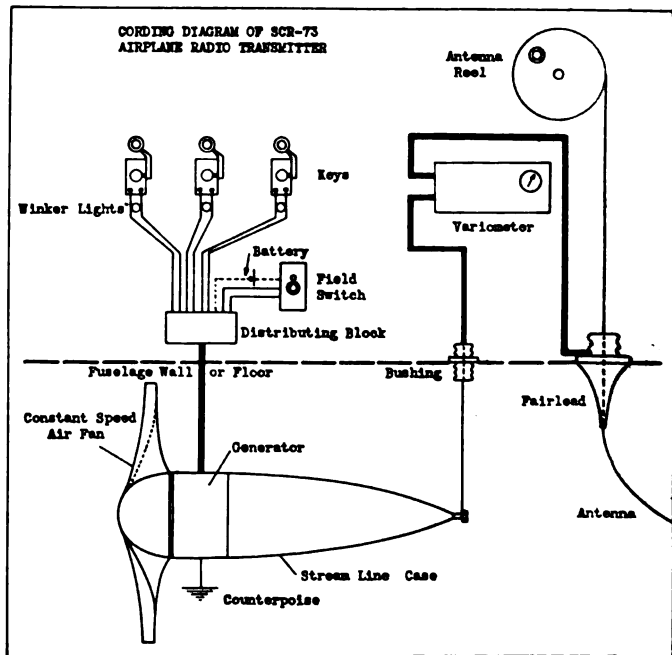
Fig. 4—Interconnection Between Parts of Type SCR-73 Set.
