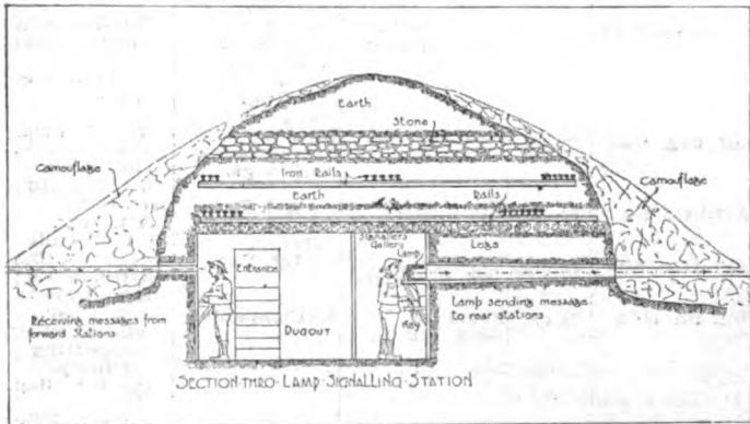
Central Receiving Station, Vertical Section.
