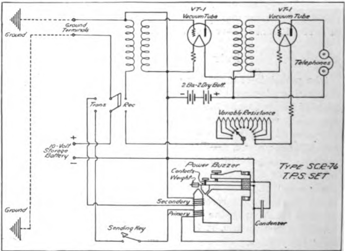
Fig. 1—Schematic Circuit Diagram of Two-Way T.P.S. Set.
