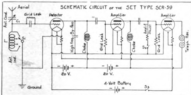
FIG. 23.—Schematic Circuit Diagram of Set Type SCR-59.
