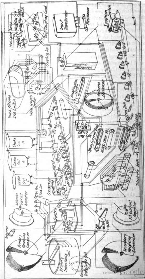
FIG. 5.—Actual Wiring Connections Within the Set Box Type BC-13, Which Forms Part of the Set Type SCR-67.
