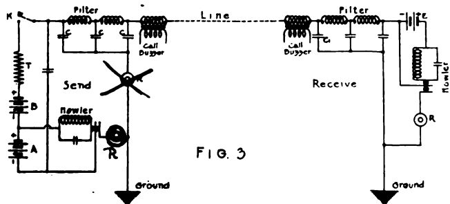
Fig. 1. Schematic Diagram of Complete Buzzerphone Circuits— Fig. 2. "Stand-By" and "Call" Circuit Elements—Fig. 3. "Send" and "Receive" Circuit Elements.
