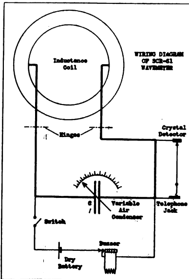
Fig. 6. Schematic Circuit Diagram of the SCR-61 Wavemeter.
