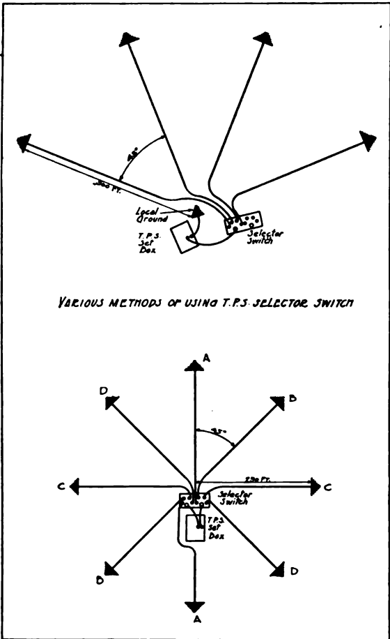
Fig. 2—Two Ways of Laying Out a Central T. P. E. Station.
