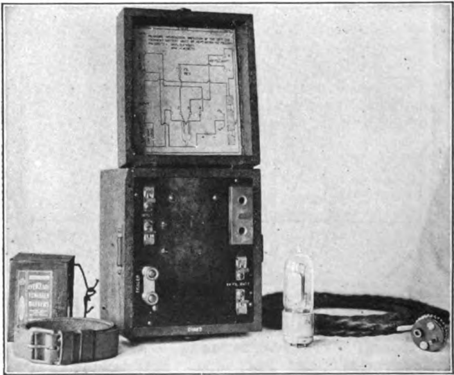
Fig. 7—Operating Panel of the Type DT-3-A Detector.
