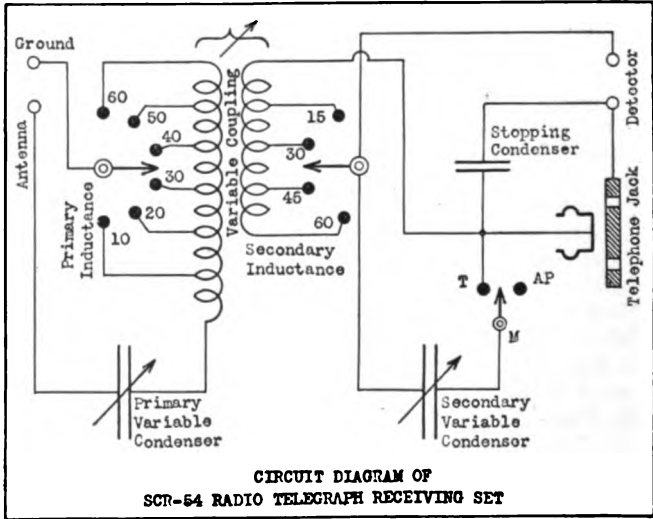
Fig. 1—Schematic Wiring Diagram of the Type SCR-54 Set.
