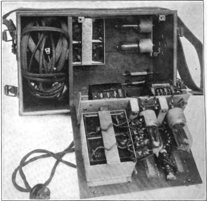
Fig. 8—Mounting of Apparatus and Spare Tubes and Batteries in the Type BC-44 Set Box
