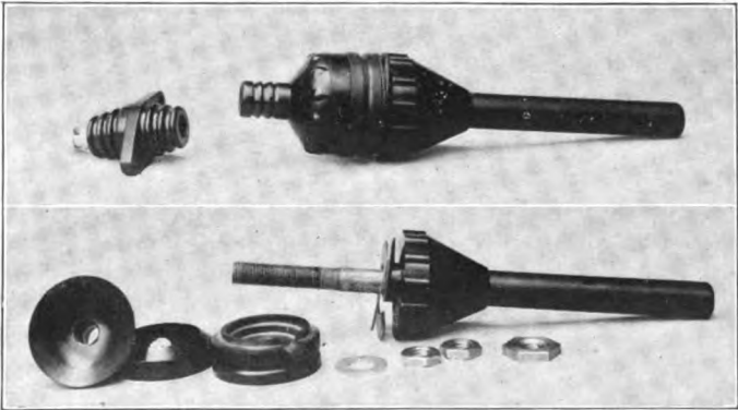
Fig. 6—Type F-1 Fairlead and Type BU-1 Insulating Bushing at Left of the Upper Insert.
