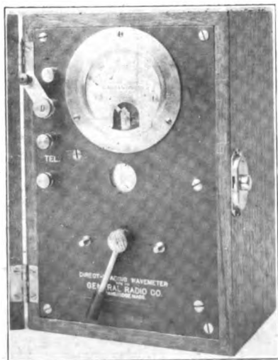
Fig. 5. Operating Panel of the SCR-60 Wavemeter.
