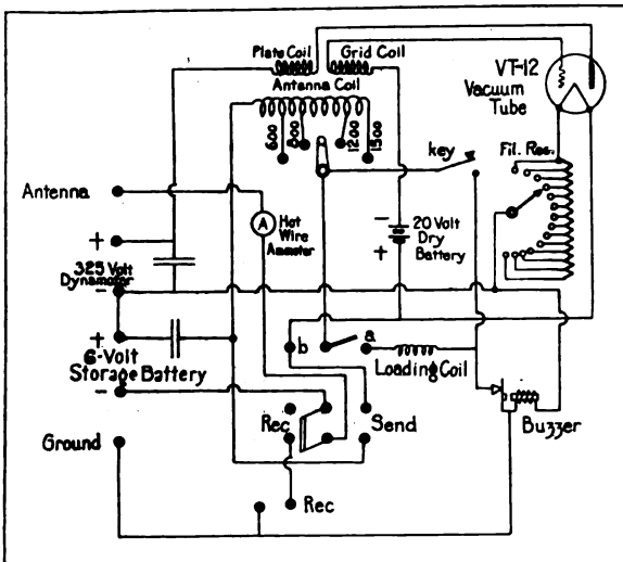
Fig. 1—Wiring Diagram of the Type SCR-69 Set
