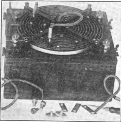
FIG. 2.—Inductance Spiral on Set Box Type BC-15 of the Type SCB-65 Set.
