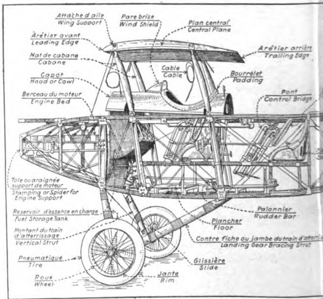
FIG. 6.—Skeleton View of Tractor Biplane
