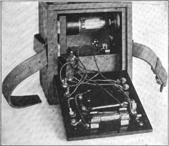
Fig. 8—DT-3-A Panel Removed Showing Vacuum Tube.
