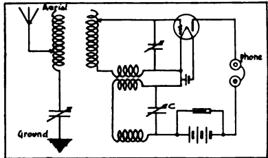
Fig. 15—Schematic Circuit of an Autodyne Receiving Set.
