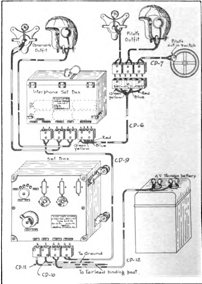
FIG. 22.—Cording Diagram of Sets Type SCR-50, SCR-50-A and SCR-75.
