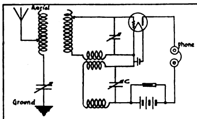
Fig. 15—Schematic Circuit of an Autodyne Receiving Set.
