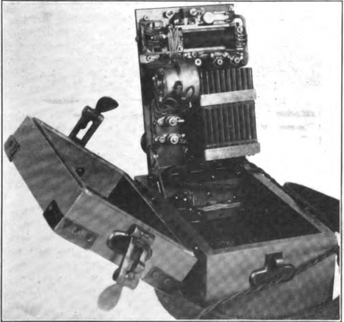
Fig. 5. Howler, Condensers, Switch, Call Buzzer and and Sending resistance Mounted on Underside of Panel, EE-1 Buzzerphone.
