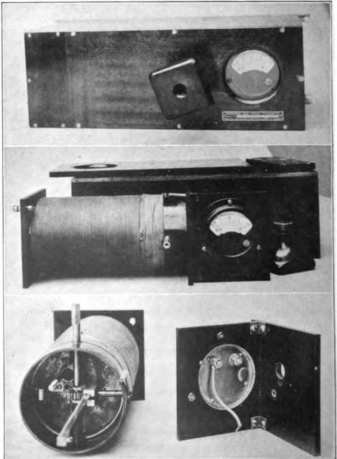
Fig. 3—Type VA-1 Variometer Assembled and Disassembled to Show the Coil, and Pinion and Ratchet-Actuated Sliding Contact.
