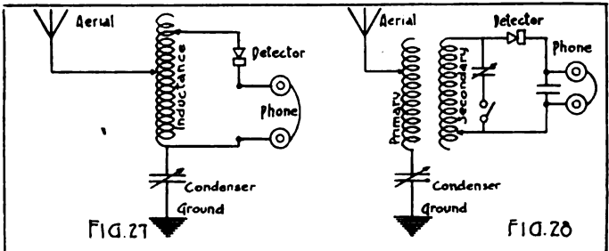
Damped Wave Receiving Circuits. Fig. 27—Inductively and Conductively Coupled. Fig. 28—Inductively Coupled.
