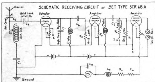
FIG. 6.—Schematic Diagram of the Receiving Circuit of Set Type SCR-68-A.
