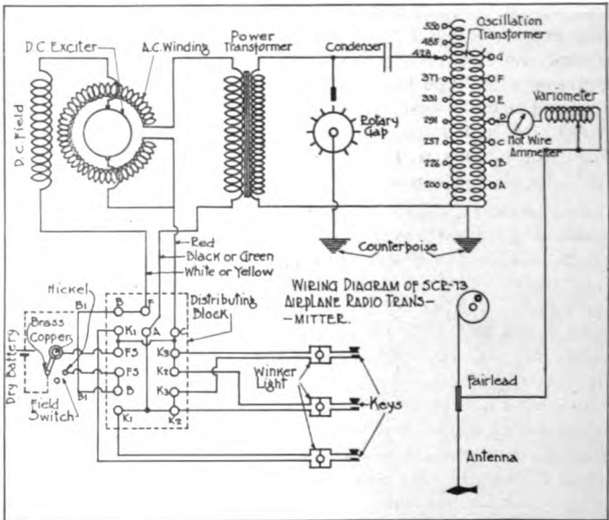
Fig. 2.—Schematic Wiring Diagram of Type SCR-73 Set.
