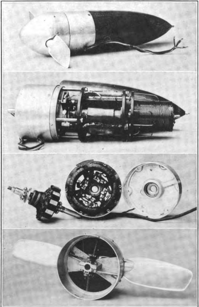
Fig. 1—Top to Bottom: Type SCR-73 Set Assembled. Casing Removed Showing Radio Apparatus. Rotor and Stator of Alternator. Airfan and Governor.
