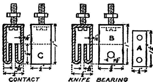
Fig. 72. Detail of Contacts.
