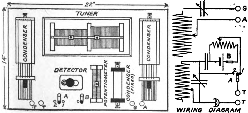
Fig. 15. Receiving Set.
