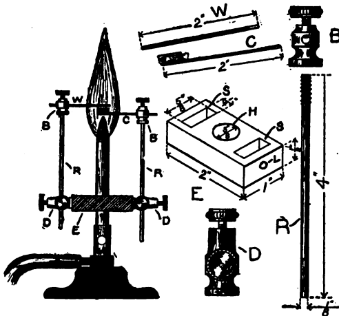
Fig. 119. Flame Audion.
