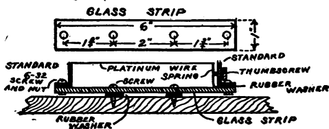
Fig. 82. Glass Compensating Strip.
