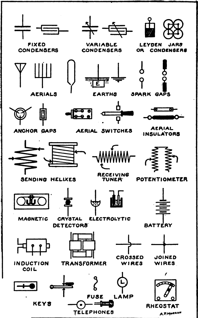
Plate I. Electrical Conventions.
