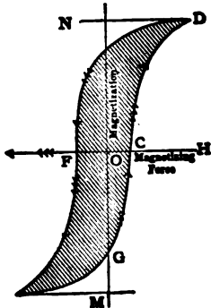
FIG. 83.—HYSTERESIS CURVE.
