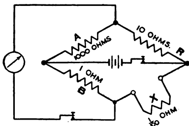
FIG. 75.—RESISTANCE MEASUREMENTS.
