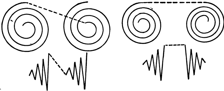
FIG. 93.—CONNECTING DISKS OF SECONDARY. FIG. 94.—CONNECTING TERMINALS OF SECONDARY DISKS.
