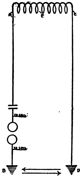
FIG. 63.— SLABY'S CLOSED EMITTER. CIRCUIT
