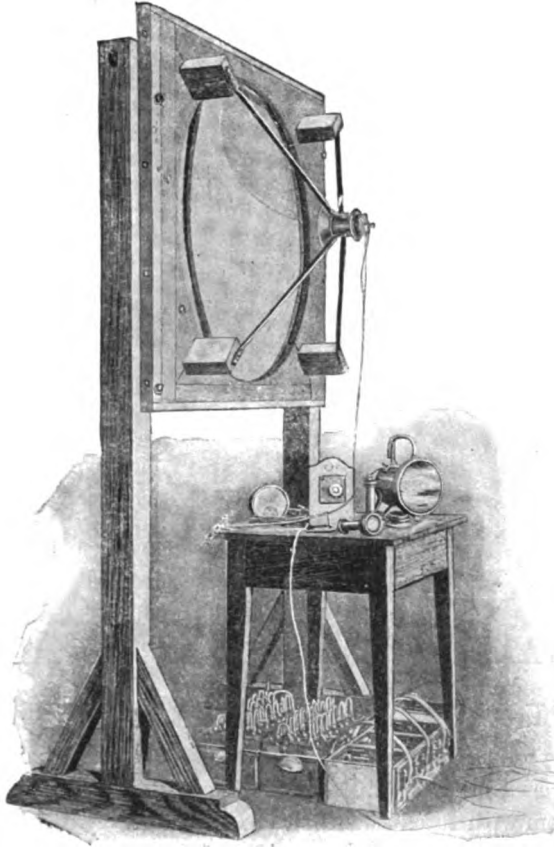
FIG. 315.—RUHMER PHOTO-ELECTRIC RECEIVER.
