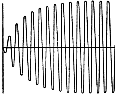
FIG. 287.—RESONANT OSCILLATIONS
