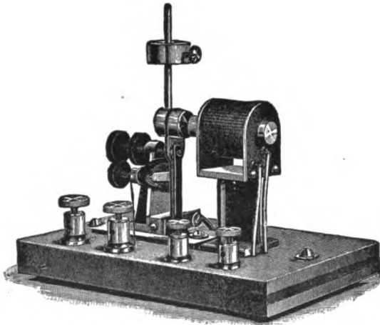
FIG. 107.—INDEPENDENT INTERRUPTOR.
