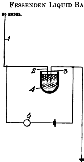
FIG. 159a.—FESSENDEN LIQUID BARRETTOR.
