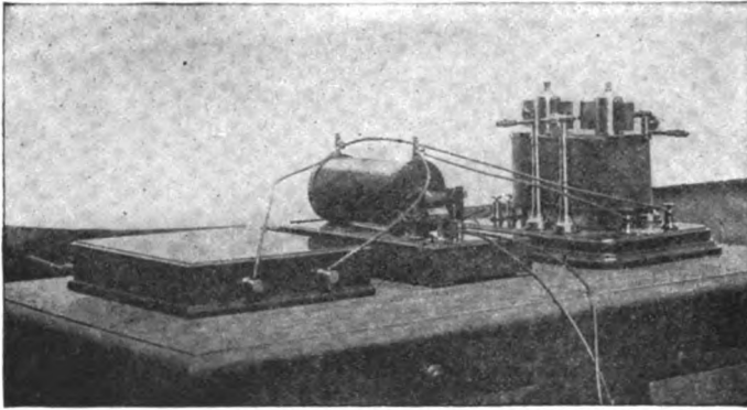
FIG. 120.—DISRUPTIVE DISCHARGE INTERRUPTOR.
