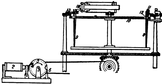
FIG. 306.—DETAIL OF TRANSMITTER.
