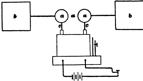
FIG. 19.—HERTZ OSCILLATOR WITH INDUCTION COIL.
