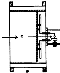
FIG. 26b. HERTZ OSCILLATOR AND RESONATOR.
