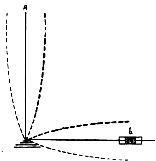
FIG. 295.—POTENTIAL LOOPS AND NODES.
