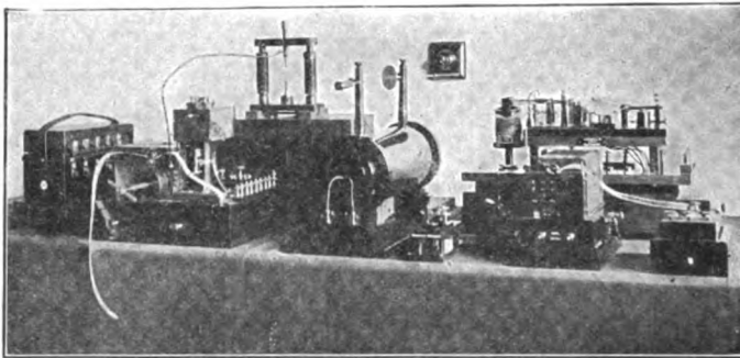
FIG. 188.—LODGE-MUIRHEAD SYSTEM.
