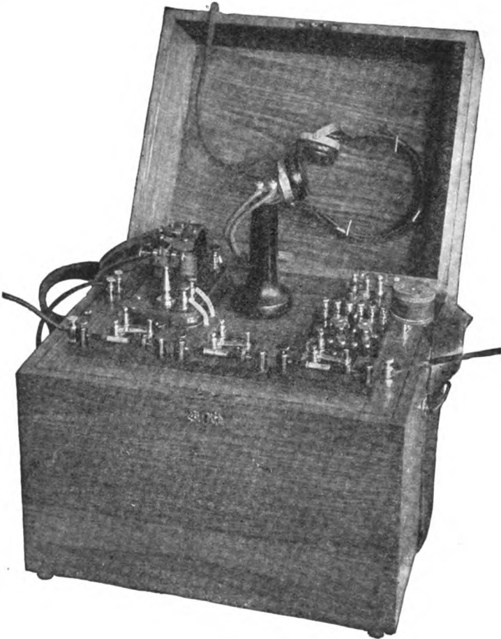
FIG. 209.—DEFOREST RECEPTOR.
