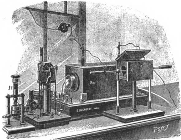
FIG. 179.—POPOFF-DUCRETET TRANSMITTER.
