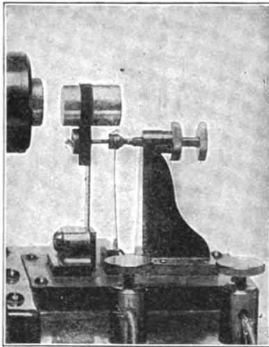
FIG. 106.—DOUBLE SPRING INTERRUPTOR.
