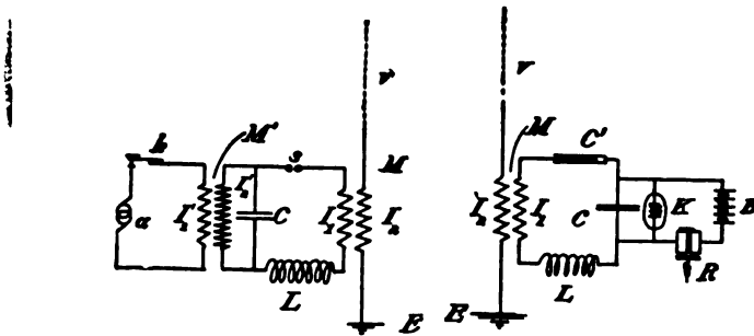
FIG. 302.—STONE MULTIPLEX SYSTEM.
