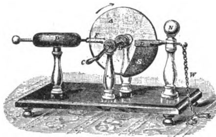
FIG. 125.—FRICTIONAL MACHINE.
