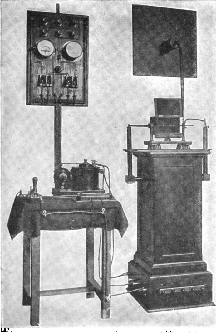
FIG. 184.—POPP-BRANLY TRANSMITTER.
