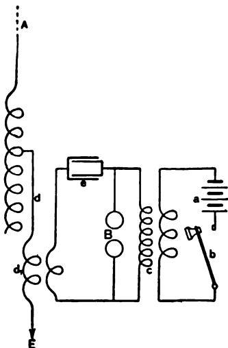
FIG. 297.—MARCONI SYNTONIC SYSTEM. (Second Form.)
