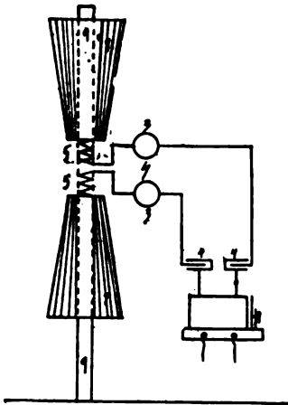
FIG. 165.—LODGE TRANSMITTER. (First Form.)
