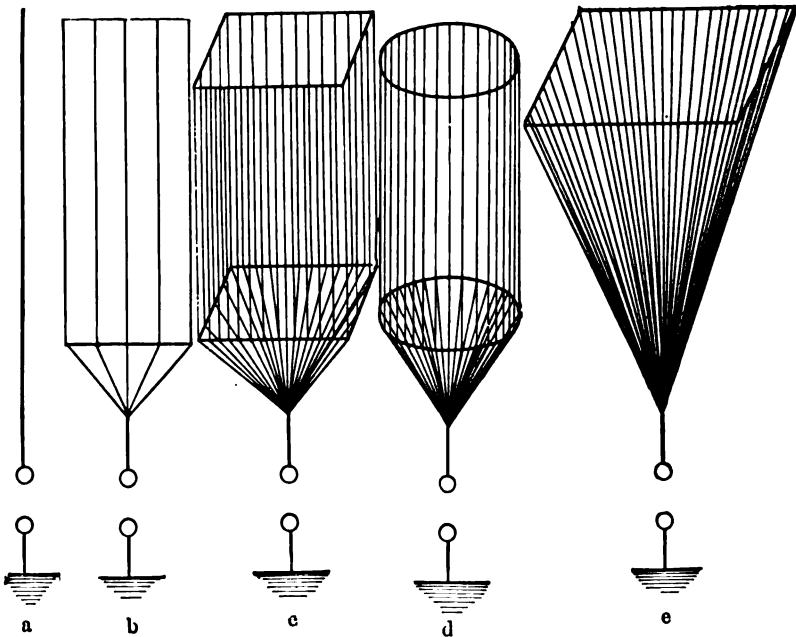
FIG. 255.—FORMS OF AERIALS.
