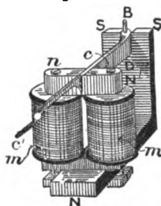
FIG. 240.—POLARIZED RELAY.
