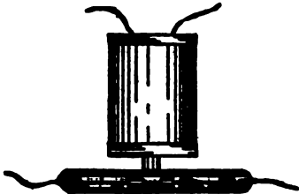
FIG. 238.—COLLINS MAGNETIC DE-COHERER.
