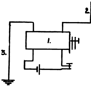
FIG. 171.—GUARINI TRANSMITTER. (First Form.)
