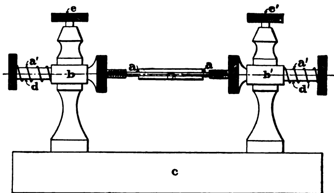
FIG. 143.—EXPERIMENTAL COHERER.
