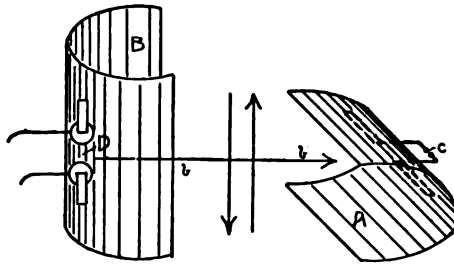
FIG. 31.—POLARIZING ELECTRIC WAVES.
