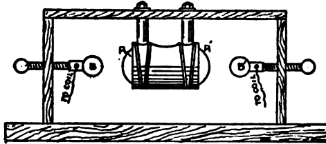
FIG. 55.—RIGHI'S OSCILLATOR.
