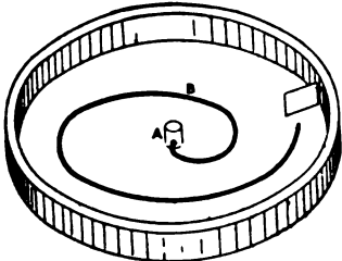
FIG. 136b.— SINGLE CONTACT COHERER.
