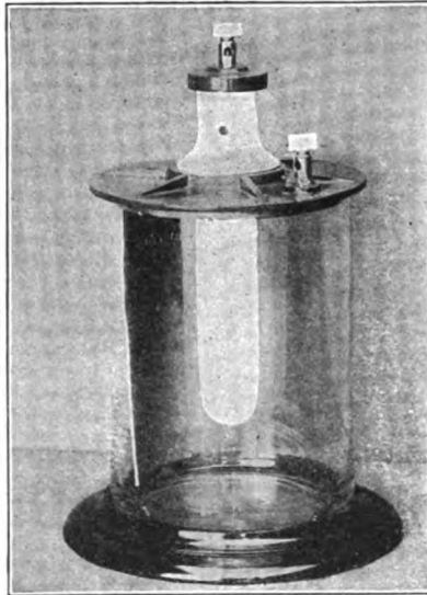
FIG. 115.—ELECTROLYTIC INTERRUPTOR.
