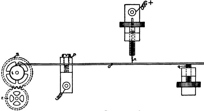
FIG. 137.—POINT AND DIAPHRAGM COHERER.
