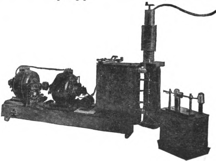
FIG. 181.—DEFOREST TRANSMITTER.
