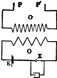
FIG. 85.—THE INDUCTION COIL.
