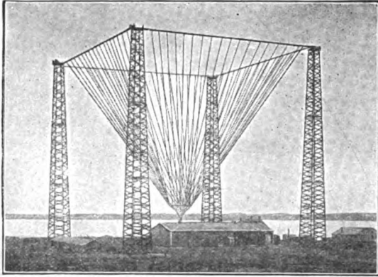
FIG. 280.—MARCONI CABLELESS STATION.
