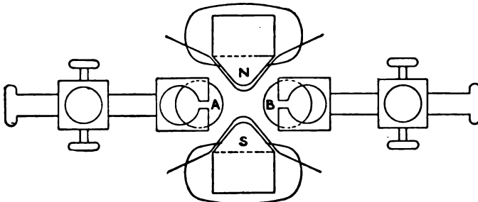
FIG. 221.—MAGNETIC BLOWOUT.
