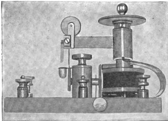
FIG. 160.—FESSENDEN LIQUID BARRETTOR.
