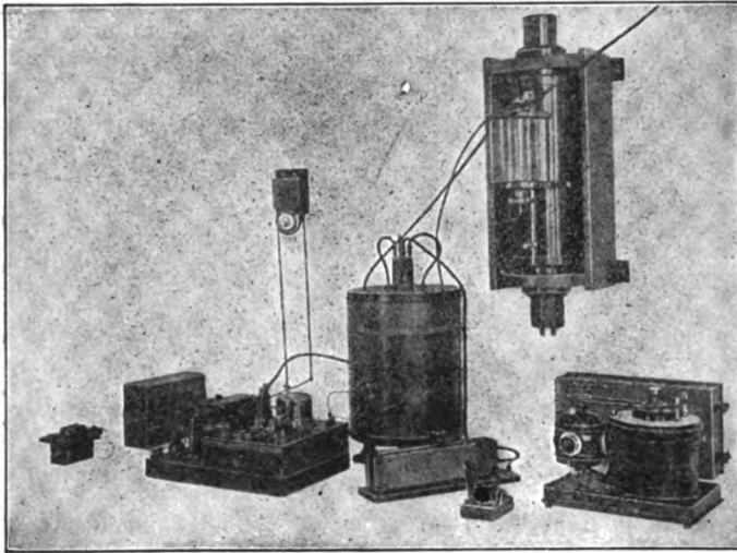
FIG. 170.—SLABY-ARCO SYSTEM.
