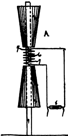
FIG. 194.—LODGE RECEPTOR.
