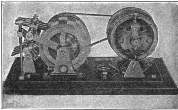
FIG. 122.—ROTARY CONVERTER.
