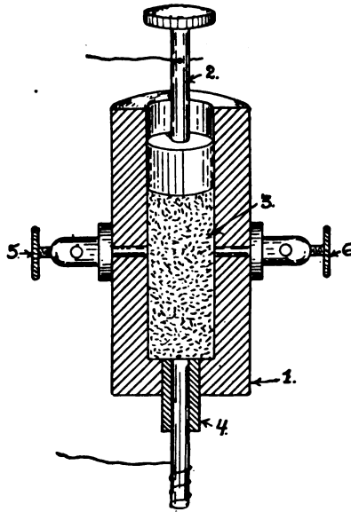
FIG. 133.—BRANLY RADIO-CONDUCTOR.
