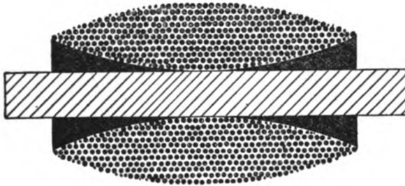
FIG. 95.—CONVEX SECONDARY WINDING.
