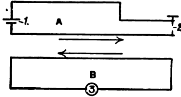
FIG. 78.—INDUCED CURRENTS.
