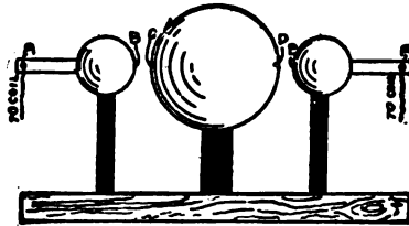
FIG. 56.—LODGE'S OSCILLATOR.
