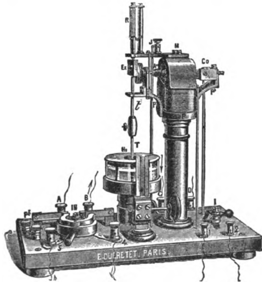
FIG. 111.—ROTATING INTERRUPTOR.
