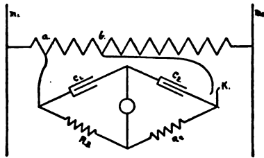
FIG. 70.—POTENTIOMETER METHOD.
