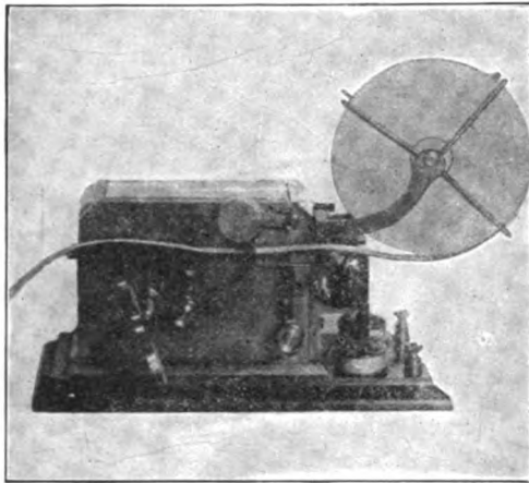
FIG. 244.—MORSE REGISTER.
