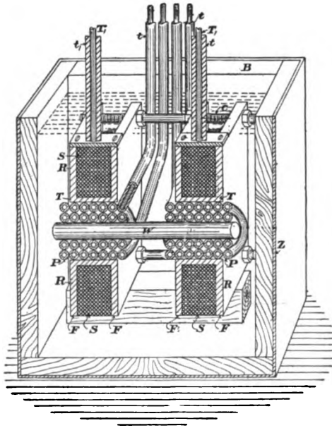
FIG. 128.—TESLA COIL.
