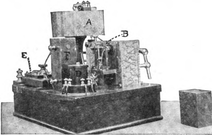
FIG. 216.—LODGE-MUIRHEAD RECEPTOR.
