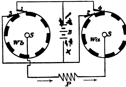
FIG. 118.—ROTARY INTERRUPTOR.
