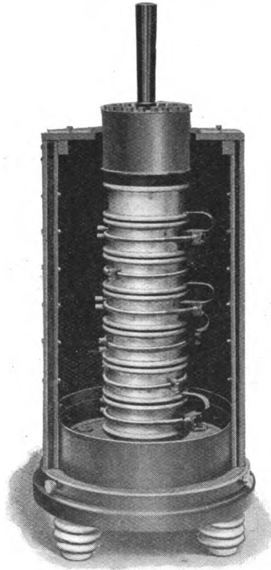
FIG. 49.—"Annular Multiplex Spark-gap."
