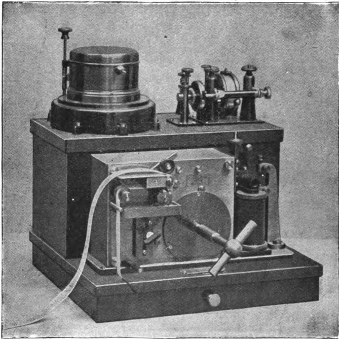
FIG. 61.—Receiving Apparatus.
