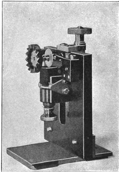
FIG. 59.—Lodge-Muirhead Coherer.
