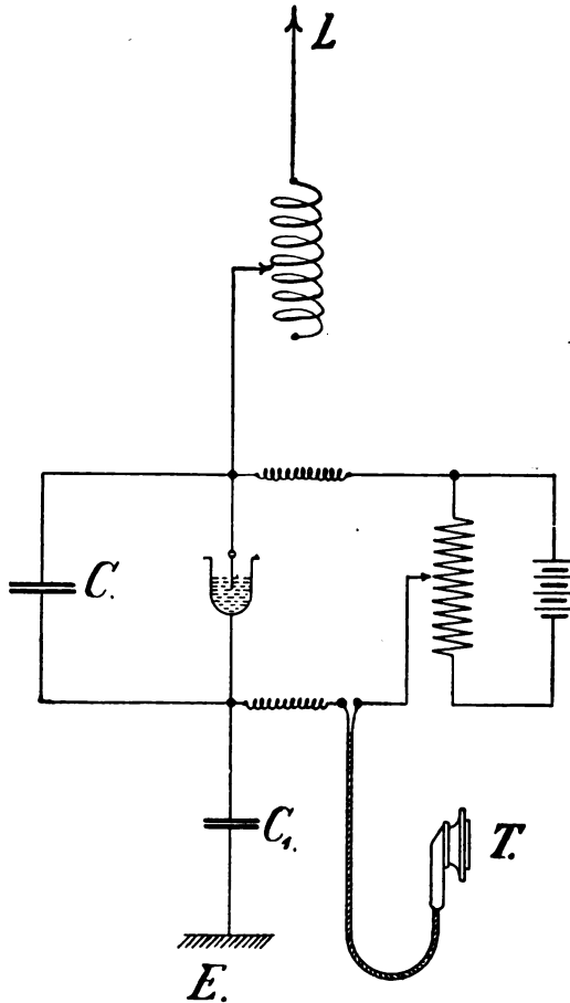
FIG. 54.—Method of Mounting the Schloemilch Detector.
