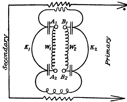
FIG. 25.—Energy System used at the Baltic Stations.
