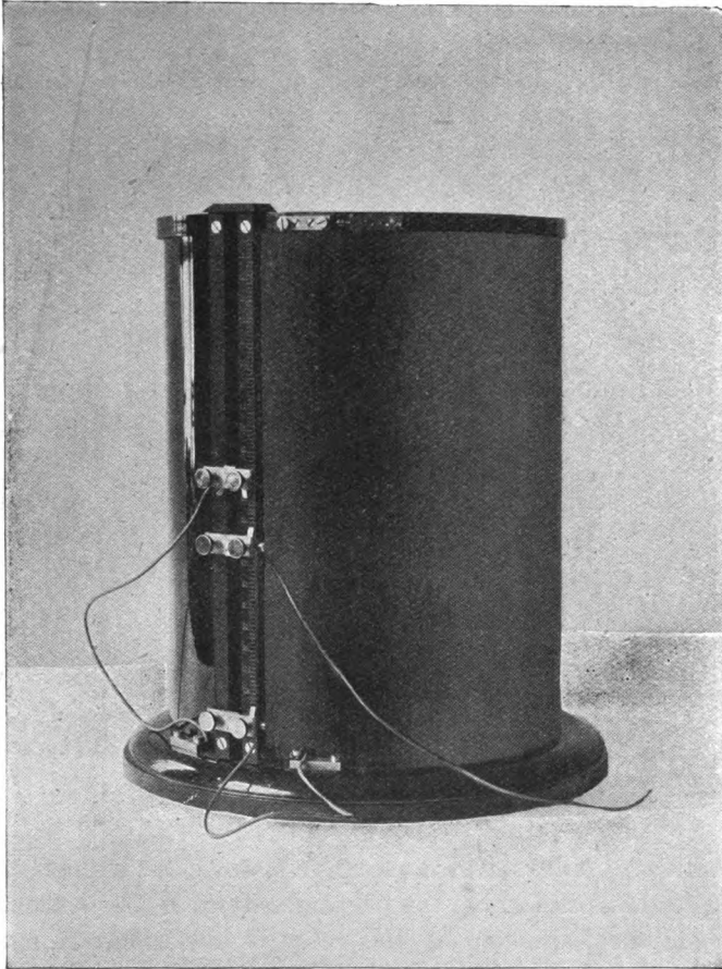
FIG. 65.—Receiving Transformer for Close Coupling.
