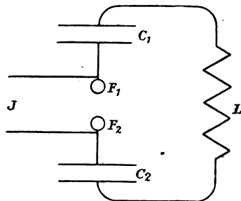
FIG. 4.—Braun's closed Oscillation Circuit.
