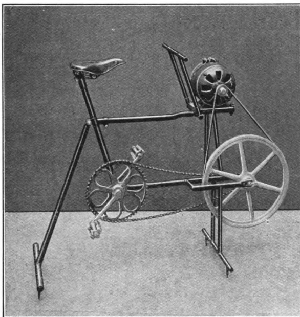
FIG. 50.—Current Generator for Light Portable Stations.
