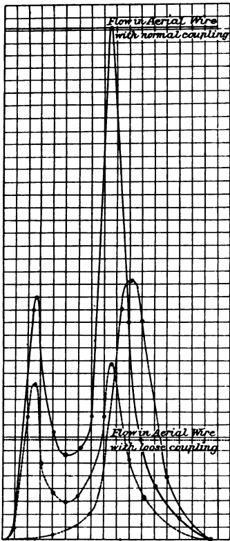
FIG. 18.—Resonance Curves.
