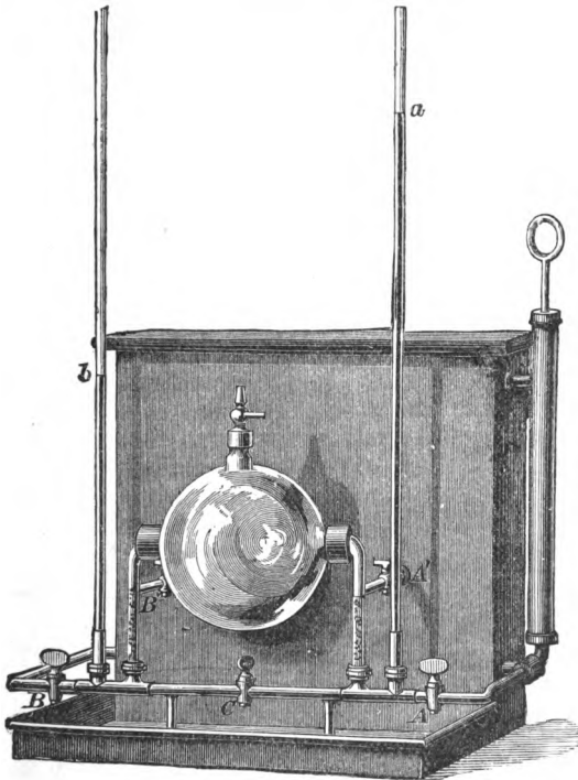
FIG. 9. —Lodge's Hydraulic Model of Leyden Jar.
