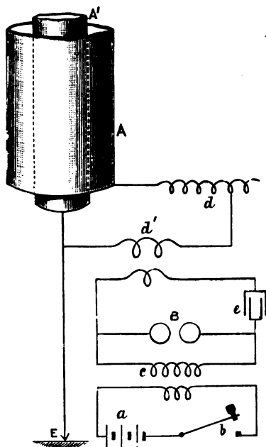
FIG. 30.—Syntonic Transmitter.
