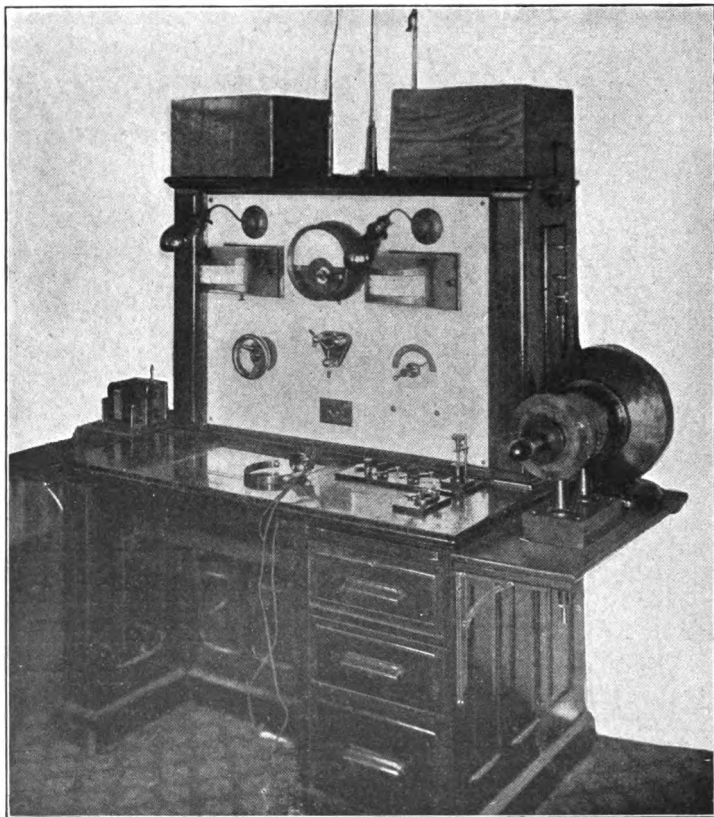
FIG. 20.—WIRELESS OPERATOR'S DESK, SIGNAL CORPS U. S. A.
