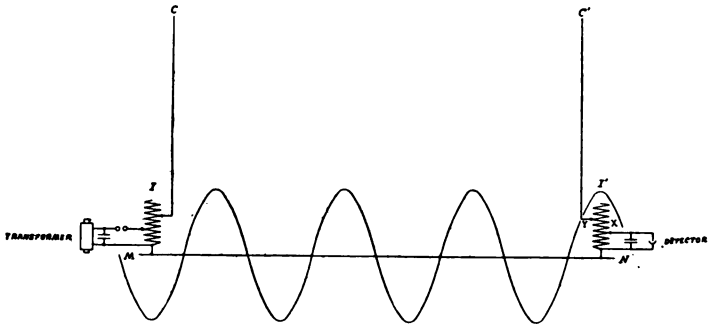
FIG. 3.—THEORY OF WIRELESS TELEGRAPHY.
