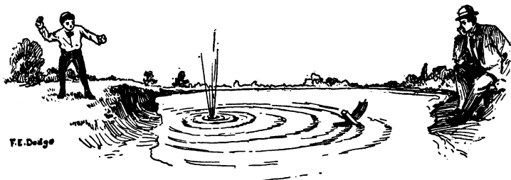
FIG. 1.—WAVE MOTION IN WATER.
