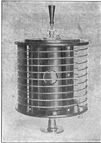
FIG. 6.—SPARK-GAP WITH MUFFER, SURROUNDED BY INDUCTANCE.
