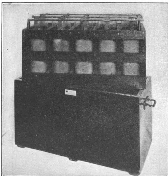
FIG. 44.—Leyden jar set for oil immersion to prevent losses from brush discharges.
