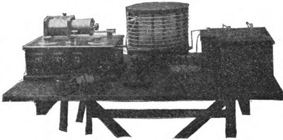
FIG. 99.—Complete receiving and transmitting outfit.
