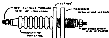
FIG. 26.—Leading-in insulator.
