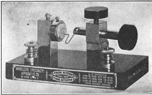
FIG. 69.—Pyron detector in which a fine wire is brought to bear against a crystal of iron pyrites.
