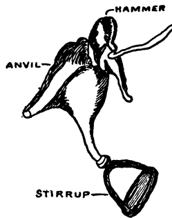
FIG. 121.—The ossicles.
