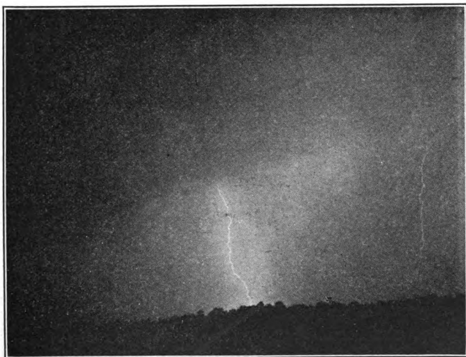
FIG. 13.—Lightning discharge near Montclair, N. J.
