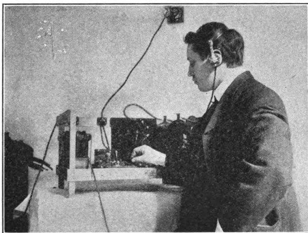
FIG. III.—Operating the U. S. Signal Corps airship wireless apparatus.
