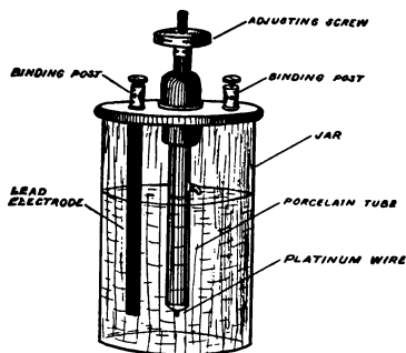
FIG. 38.—Electrolytic interrupter.
