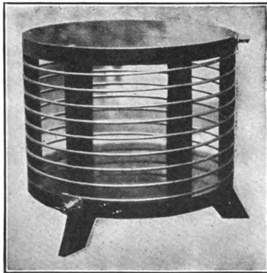
FIG. 49.—Close coupled helix.
