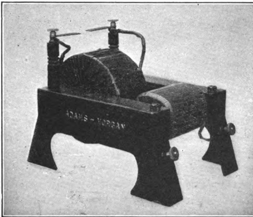
FIG. 43.—High potential closed core transformer for wireless work.
