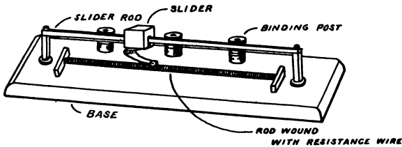
FIG. 74.—Potentiometer.
