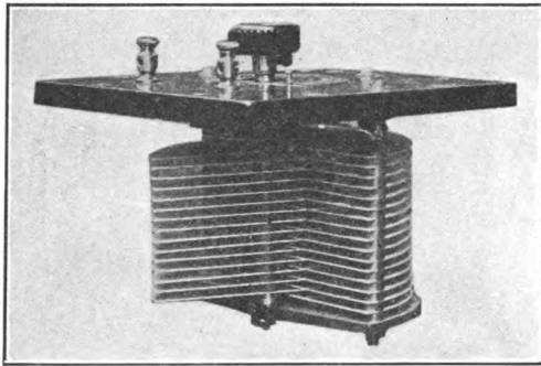
FIG. 82.—Interior of rotary variable condenser showing construction.
