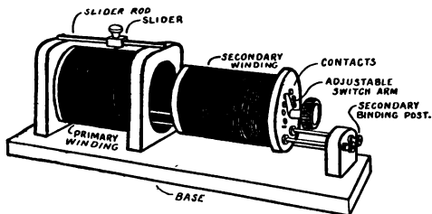
FIG. 91.—Loose coupled tuning coil.
