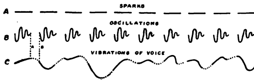
FIG. 143.—Diagram illustrating the reason why damped oscillations will not carry the voice.
