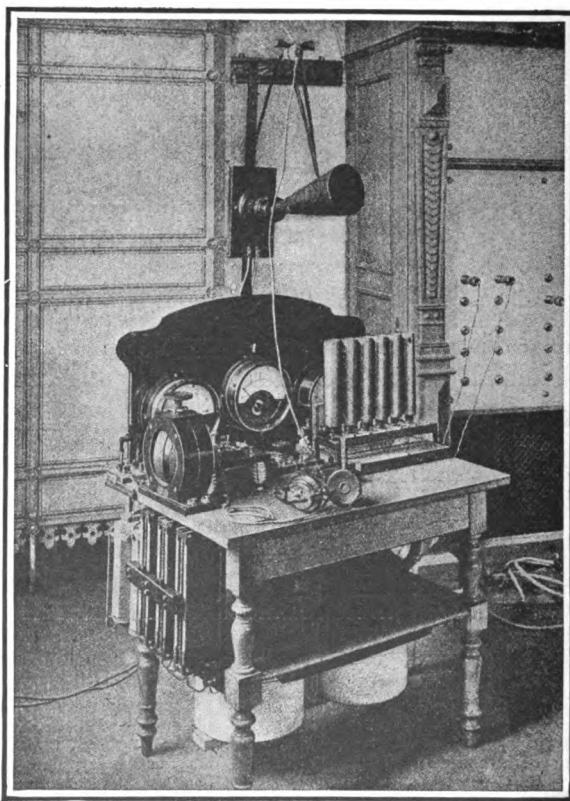
FIG. 147.—Poulsen wireless telephone equipment.
