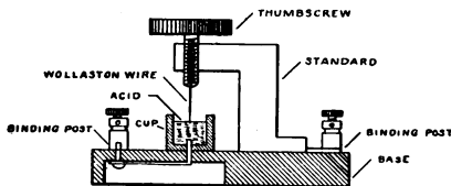
FIG. 72.—Electrolytic detector.
