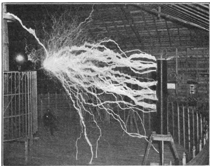
FIG. 156.—Twenty-five foot sparks from a Tesla transformer.
