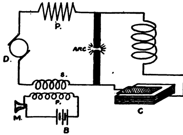
FIG. 145.—Arrangement of the speaking arc.
