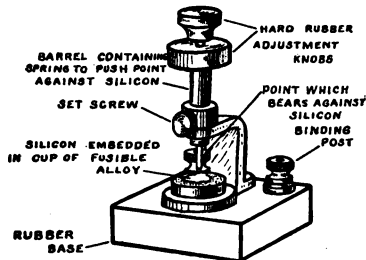
FIG. 71.—Silicon detector.
