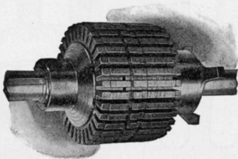
FIG. 355. —Western Electric slotted armature core. The laminations are of sheet steel, annealed and japanned. They are mounted directly on the shaft, (except in the large sizes) and held in place by substantial end plates.
