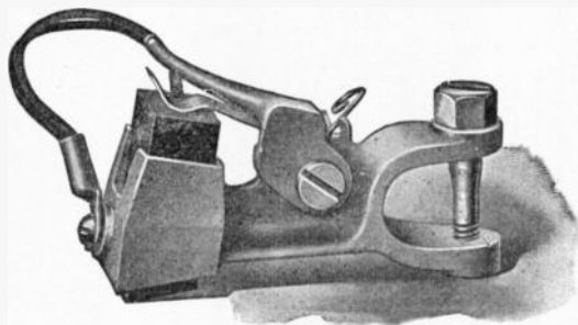
FIG. 336. —Western Electric box type brush holder. The box which holds the brush is broached to allow the brush to slide freely, but not loosely, to and from the commutator against which it is normally held by a lever acting directly upon the brush head. This avoids the possibility of uneven bearing on the commutator, as the brushes are allowed very slight lateral or angular motion. The adjustment of a brush is also simplified after it has been removed and then replaced. Tension on the brush head is obtained by a special spring which maintains any given tension for which it may be set. An auxiliary flat steel spring on the lower side of the lever acts as a shock absorber between the lever and the brush head, absorbing all minor vibrations caused by a worn commutator. Side contact between brush and brush holder is not relied upon to carry the current, flexible copper pigtails performing this function to the exclusion of sliding contacts or tension springs, in order to reduce the brush loss. It is not necessary to take the brush rigging apart or loosen cable connections when it is desired either to remove or reverse the brushes to change the direction of armature rotation.
