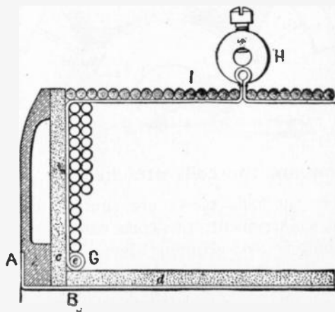
FIG. 241.—Another mode of bringing out the coil ends. A narrow insulated strip of thin copper G, leading to terminal H, is connected with the end c of the coil before winding.
