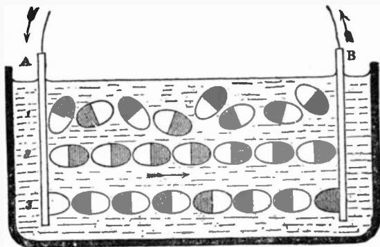
FIG. 91.—Grotthuss' theory of electrolysis. Grotthuss in (1806), announced his theory that the molecules in an electrolyte have their individual electro-positive and electro-negative atoms charged positively and negatively respectively. In an ordinary liquid, for instance in water, the molecules are arranged indifferently, like row 1, with their positive and negative ends pointing in all directions. When the charged plates A and B connected to the + and - poles of a battery are inserted in the water, the molecules under the action of the laws of electrostatic action turn as shown in row 2, so that all the hydrogen or shaded ends (+) are turned towards the (-) plate B and all the oxygen or unshaded ends (-) towards the (+) plate A. All along the row the electrical forces are supposed to tear the molecules asunder, depositing H on B and O on A. The atoms in the middle of the liquid, however, recombine, for the hydrogen atoms in their journey towards B meet the oxygen atoms travelling in the opposite direction, and we get the state of affairs represented in row 3. The next step is to rotate once more the atoms into the positions shown in row 2, and so on. In this way the theory accounts for the products only appearing at the electrodes and not in the body of the liquid.
