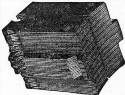
FIG. 234.—Port Wayne laminated pole piece before being cast welded into frame. In the faces of solid pole pieces there exist minute electric currents called eddy currents which cause heating of the iron and increase the energy required to maintain a magnetic circuit in much the same manner as does reluctance. This loss is reduced by dividing the magnetic circuit in the line of flux into numerous parallel paths separated by some material of relatively high resistance. In construction, the above core and pole piece is made up of sheets of annealed steel of two different widths assembled together to form proper size and shape. The minute spacing between these laminations and the slight oxidizing on each surface is sufficient to reduce considerably the eddy currents. By cast welding the pole piece into the frame, a low reluctance is secured.
