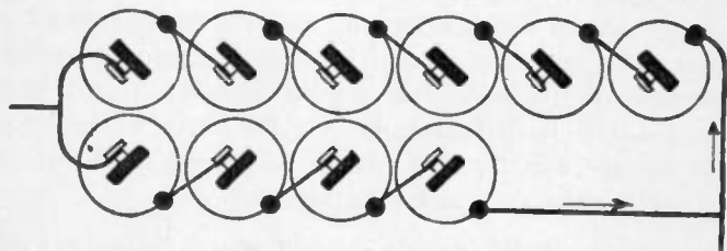
FIG. 75.—Diagram to illustrate incorrect wiring. The current pressure of the six cell battery being greater than that of the smaller unit, current will flow from the former through the latter until the pressure of the six cells is equal to that of the four cells.
