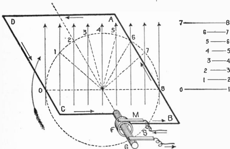
FIG. 167. —Illustrating the increase and decrease in the rate magnetic lines are cut by a revolving loop. The initial position of the loop is taken at right angles to the direction of the lines of force. Since the loop rotates at a constant speed, it is evident that it does not cut the magnetic lines at uniform rate, because the intercepted arcs 0-1, 1-2, etc., are unequal. These arcs, rectified at the right by the horizontal lines 0-1, 1-2, etc., show more clearly the increase and decrease in the rate at which the magnetic lines are cut.
