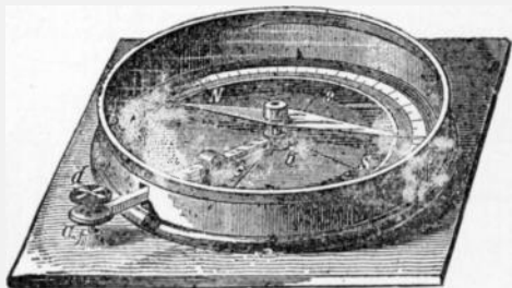
FIG. 93. — Simple compass. It consists of a magnetic needle resting on a steel pivot, protected by a brass case covered with glass, and a graduated circle marked with the letters N, E, S, W, to indicate the cardinal points; a b is a lever which arrests the needle by pushing it against the glass when the button d is pressed.
