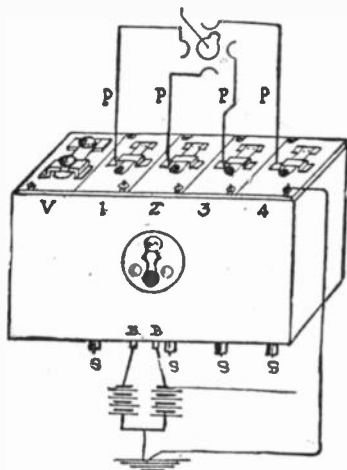
FIG. 145.—The Splittdorf master vibrator coil. As shown in the illustration the several unit coils are indicated by the figures 1, 2, 3, and 4. A fifth unit V at the left contains the master vibrator. The primary wires P connect with the timer and the secondary wires S with the plugs. B B shows the battery connections.
