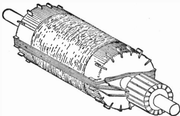
FIG. 251.—Illustrating the principle of Siemens' drum winding. In order to make the winding and connections clear, one coil and the commutator is shown assembled, although the latter is not put in place until after all the sections have been wound, the ends of the wires being temporarily twisted together until all can be soldered to the risers. The cores of these early machines were of wood overspun circumferentially with iron wire before receiving the longitudinal copper windings.
