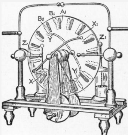
FIG 34.—The Wimshurst Electric Machine.
