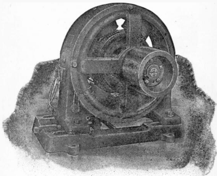
FIG. 163.—General Electric 16 K W multipolar dynamo designed to operate at moderate and slow speeds. The outer structure of the machine consists of a magnet frame having feet in one casting. Adjustment is provided for moving the machine on its bed plate to tighten the belt. The field coils are former wound and the series windings permit of any degree of compounding up to 10% by the use of suitable German silver shunts connected across the series field.
