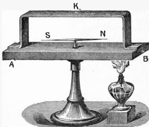
FIG. 88. — The Seebeck effect: If in a complete metallic circuit having junctions of dissimilar metals, the junctions are at different temperatures, then generally a steady current will flow in the circuit as long as the differences of the temperatures of the junction is maintained. To demonstrate this, a piece of copper K bent in the shape seen in the figure, was placed on a block of bismuth A B, carrying a pivoted magnetic needle N S; as soon as the equality of temperatures was altered by either heating or cooling one of the junctions of the two metals, the needle indicated a current which continued to flow as long as the difference of temperature was maintained at the junctions. The movement of the needle indicated the direction in which the current flowed. If, for instance, the north junction B were heated, the N pole moved eastwards, showing that at the heated junction the current flows from the bismuth to the copper, at the cold junction from the copper to the bismuth.
