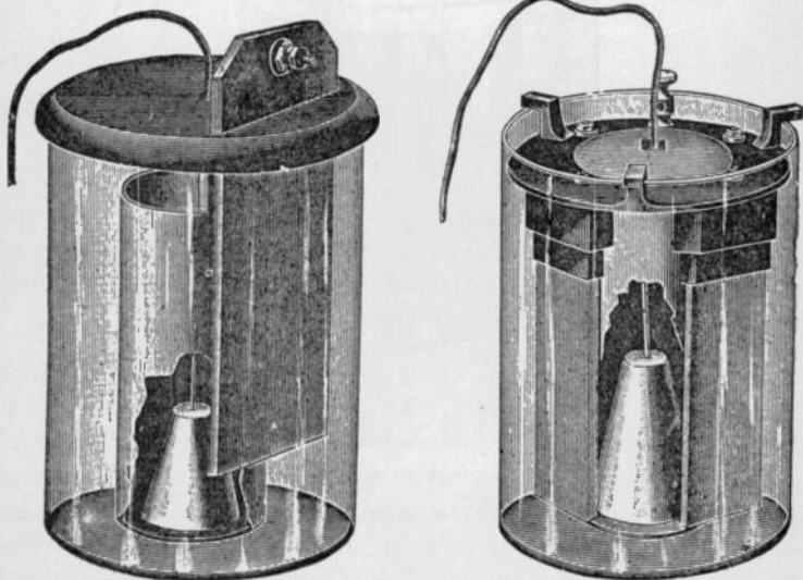
FIGS. 46 and 47.—The telephone standard and compound forms of Fuller cell. The type shown in fig. 46 is especially adapted to long distance telephoning, and that shown in fig. 47 to incandescent lamps, motors, nickel and other electroplating. The Fuller cell is of the double fluid variety and has the advantage over the Grenet type, in that the zinc is always kept well amalgamated and does not require removal from the solution. The Fuller cell is suitable for open and semi-closed circuit work; its electromotive force is about 2.14 volts.
