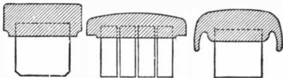
FIGS. 207 to 209.—Various sections of cast iron yoke. In form, these yokes may be either circular or segmental as shown in figs. 205 and 206.
