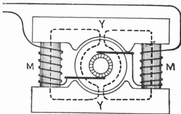
FIG. 203.—Consequent pole bipolar field magnet with two coils on the cores. This is known as the "Manchester" type in which the cores are connected at the ends by two yokes—so named from its original place of manufacture at Manchester, England.
