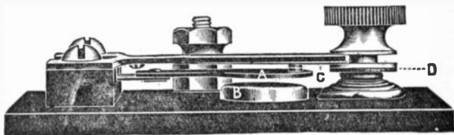
FIG. 146.—A hammer vibrator. When at rest, the upward tension of the spring, which carries the armature A, holds the platinum points in contact and causes the upper spring C, to leave shoulder of adjusting screw D, and rest against the heavy brass plate above it. When the iron core B, attracts the armature A, the downward tension on the upper spring, C, causes the latter to follow the armature down, holding the platinum point in contact, until the end of the upper spring C, strikes the lower shoulder of the adjusting screw, D, which gives it a "hammer break." The adjusting screw is held firmly in position by a bronze spiral spring under shoulder D.
