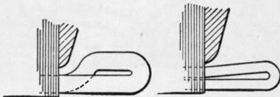
FIGS. 375 and 376.—Single layer and double layer barrel winding. Barrel winding is a method of arranging the ends of armature coils as they pass from one pole to the next, in which, instead of using involute or butterfly connections, V-shaped end connections are used which lie on a cylindrical surface, which is a continuation of the armature surface. The coil ends must of necessity be arranged in two layers, but the method may be used for either one or two coils per slot, the difference in arrangement for these is here illustrated.
