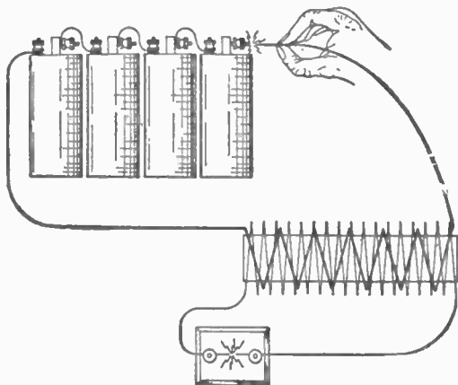
FIG. 137. —Production of spark with plain coil. Connect the ends or leads of the secondary winding to fixed insulators and bend the ends so they are from one-sixteenth to one-eighth inch apart. Connect one end of the primary winding to an electric battery, and with the other lead of the primary winding brush against the other terminal of the battery, as indicated. When the contact is broken there will be a spark both at the point of rupture in the primary circuit and at the gap. An electric impulse is also induced in the secondary circuit when the primary circuit is closed and the current flowing in it gradually rises to its maximum value, but this impulse is too feeble to cause a spark to jump across the gap. Only the impulse induced in the secondary during the dying out of the current in the primary is utilized.
