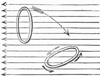
FIG. 128. —Electromagnetic induction: If a coil be given a motion of rotation from any point within its own plane so that it passes through a uniform magnetic field, a current will be induced in the coil because the number of lines of force passing through it is altered.
