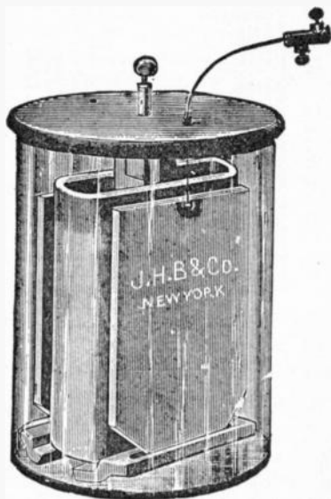
FIG. 55.—Wheelock cell; the elements are carbon and zinc. To set up, place the grid in the bottom of the jar and fill its two troughs each about half full of mercury. Place the porous cell in position on the grid so that it sits perfectly upright, resting in the recess of the latter. The zincs stand with lower ends resting in mercury in the troughs of the grid. Into the porous cell, to a height of only two thirds full, pour solution consisting of equal parts water and sulphuric acid, by measure. Add to this \frac{1}{2} pound nitrate soda, 1 ounce chromic acid. This solution may be made up in the above proportion and kept in covered receptacle in any desired quantity, ready for use. In the outer jar for 6 x 8 size, 2\frac{1}{2} pints of water, and \frac{1}{2} gill sulphuric acid, 1 part sulphuric acid to 20 parts water, or as much sulphuric acid as it will take without boiling. When a charge becomes exhausted it may be renewed by adding sulphuric acid and salts in the proportions given above, after drawing out with syringe enough of the old solutions to make room for the additions, but the best action is obtained with entirely new solutions. Zincs must be kept thoroughly amalgamated by keeping a good supply of mercury in the troughs.
