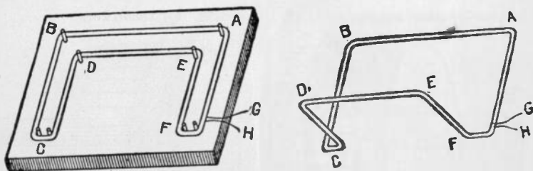
Fig. 381.—Method of winding evolute coils. In preparing the former, it is necessary to know the dimensions of the coil, hence, a pattern coil must first be made, from which the spacing of the pins can be taken so that the completed coil will fit into the slots for which it is intended. After the pins have been properly spaced on the board, the wire is wound around them as indicated, as many turns being taken as decided on for each coil. When the coil is thus completely wound, it is taken from the pins, and the lower ends, C and F, placed in a suitable clamp. The two halves of the coil are then spread apart, the coil assuming the shape illustrated in fig. 382.
