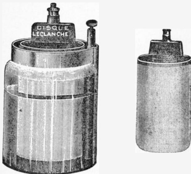
FIGS. 44 and 45. —Leclanche cell and porous cup. This very common form of cell is an example of the single fluid type, with a solid depolarizer surrounding the negative element; the latter is generally carbon, the positive element being zinc. The liquid used is a strong solution of ammonium chloride, commonly known as sal-ammoniac, and which resembles table salt. In the porous cup type of cell, a carbon slab is placed in the porous cup, and is surrounded by a mixture of small pieces of carbon and manganese dioxide, the top being covered by means of pitch, leaving one or two small holes for air and gas to pass through. The depolarizer will take care of a limited amount of the hydrogen produced when the cell is on closed circuit, but if the circuit be closed for any length of time polarization occurs. The cell is thus of the open circuit class, and will furnish a good current where it is required only intermittently. Zinc is dissolved only when the cell is being used. This type of cell, or its modification, is used for gas lighting and bell work. The cell requires very little attention. Water must be added as the solution evaporates, and the zinc rod replenished when necessary. The electromotive force is about 1.48 volts and the internal resistance about 4 ohms.
