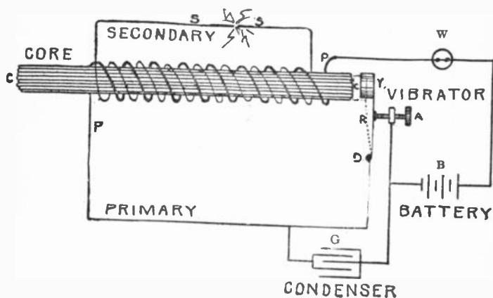
FIG. 143.—Diagram of a vibrator coil. The parts are as follows: A, contact screw; B, battery; C, core; D, vibrator terminal; G, condenser; P, primary winding; S, secondary winding; W, switch; Y, vibrator. When the switch is closed, the following cycle of actions take place: 1, the primary current flows and magnetizes core; 2, magnetized core attracts the vibrator and breaks primary circuit; 3, the magnetism vanishes, including a momentary high tension current in the secondary winding; 4, magnetic attraction of the core having ceased, vibrator spring renews contact; 5, primary circuit is again completed and the cycle begins anew.
