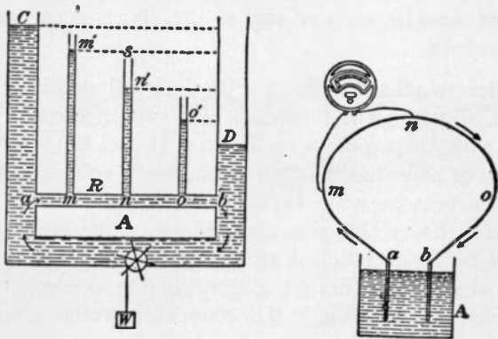
FIG. 38.—Hydrostatic analogy of fall of potential in an electrical circuit.
