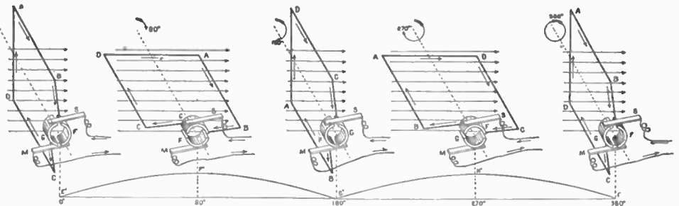
Figs. 174 to 178. —Commutation of the current. These figures show how a dynamo transforms alternating into the so called direct current. During the first half of the revolution the current flows in the direction A B, out through segment F of the commutator and brush M, returning through brush S and segment G, figs. 174 and 175. At the beginning of the second half of the revolution, fig. 176, the current in the armature reverses and flows around the loop in the direction B A. At this instant the brushes M and S pass the gaps between the commutator segments, thus reversing contact with the segments, and causing the current in the external circuit to remain in the same direction.
