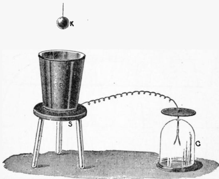
FIG. 25.—Paraday's ice pail experiment. An ice pail P connected with the gold leaves of an electroscope C , is placed on an insulating stand S . A charged conductor K , carried by a silk thread, is lowered into the pail, and finally touches it at the bottom. While it is being lowered the leaves of the electroscope diverge farther and farther, until K is well within the pail, after which they diverge no more, even when K touches the pail or is afterwards withdrawn by the insulating thread. After withdrawal, K is found to be completely discharged.
