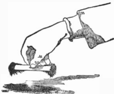
FIG. 99.—Magnetic poles. If a bar magnet be plunged into iron filings and then lifted, as illustrated in the figure, a mass of filings will cling to the ends of the magnet but not to the middle. The ends are called the poles of the magnet.
