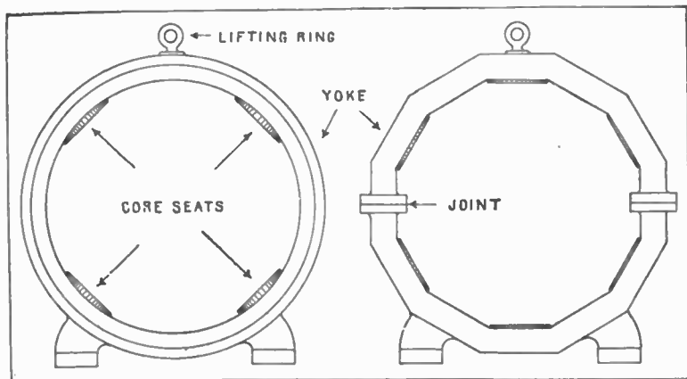
FIGS. 205 and 206. —Solid and split construction of yoke for multi-polar dynamos. In the latter type the yoke is in two halves joined along a horizontal diameter; while the upper half may be conveniently removed to give access to the armature, it has the disadvantage of the joint, which, no matter how well made, will add to the reluctance of the magnetic circuit. The figures also illustrate the circular and segmental forms of yoke construction.
