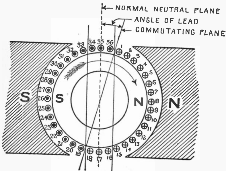
FIG. 289.—Diagram illustrating the demagnetizing effect of armature reaction. This results from the forward lead given the brushes in order to secure sparkless commutation.
