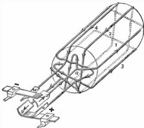
FIG. 252.—Elementary four coil drum winding, showing the connections with the commutator segments, and directions of currents in the several coils. The action of this type of armature is fully explained in the text.
