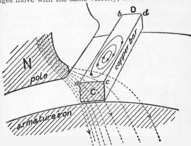
FIG. 291. —Formation of eddy currents in a solid bar inductor. On account of its appreciable size, the field is sometimes weaker at one point than another, hence the unequal electromotive forces thus produced will induce eddy currents.
