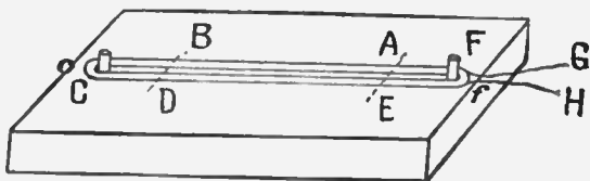
FIG. 386. —Another and simpler method of winding a "straight out" coil. A board with only two pins is employed as shown; this plan, however, gives more trouble in the subsequent opening out of the coil.
