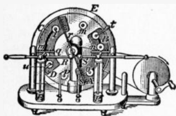
FIG. 32.—The Toeppler-Holtz electric machine.
