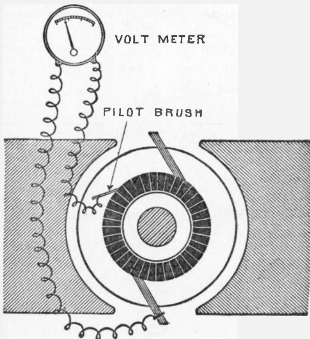
FIG. 284. —Morday's method of measuring the variation of voltage around the commutator by use of a single exploring brush and voltmeter. It consists in connecting one terminal of the voltmeter (preferably an electrostatic one) to one brush of the machine, and the other terminal to the exploring brush, which can be moved from point to point, readings being taken at each point.
