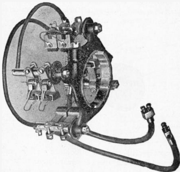
FIG. 341—Western Electric brush gear. The brush holders carry carbon brushes and are so designed that the brushes may be firmly clamped in position and also be capable of independent adjustment. Any brush can be removed while the machine is in operation without disturbing the others and without moving the holder on the stud.
