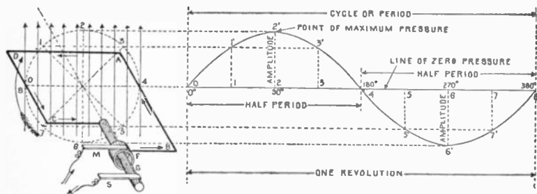
FIG. 168.—Application and construction of the sine curve. The sine curve is a wave-like curve used to represent the changes in strength and direction of an alternating current. An elementary alternator is shown at the left to illustrate the application of the sine curve to the alternating current cycle. It consists of a loop of wire A B C D, whose ends are attached to the ring F and shaft G, being arranged to revolve in a uniform magnetic field indicated by the vertical arrows which represent magnetic lines at equidistances. The alternating current induced in the loop is carried to the external circuit through the brushes M and S. Now, as the loop rotates, the induced electromotive force will vary in such a manner that its intensity at any point of the rotation is proportional to the sine of the angle corresponding to that point, this is represented by the wave-like curve. The mean value of the sine curve, or average electromotive force developed during the revolution, or period, is equal to 2 \div \pi , or .637 of that of the maximum ordinate, that is, average electromotive force = .637 \times amplitude. The sine curve lies above the horizontal axis during the first half of the revolution and below it during the second half, which indicates that the current flows in one direction for a half revolution and in the opposite direction during the remainder of the revolution.
