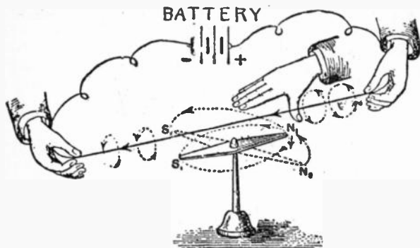
FIG. 115. —Right hand palm rule to determine the direction of the magnetic field around a conductor carrying a current: Place the palm of the outstretched right hand above and to the right side of the wire with the fingers pointing in the direction of the current, and the thumb extended at right angles, that is, pointing downward. The direction in which the thumb points will indicate the direction of the magnetic whirls.
