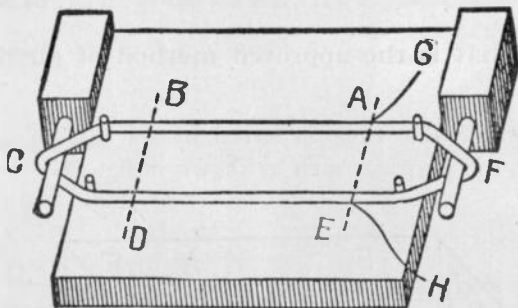
FIG. 384. —Method of winding "straight out" coils. There are several ways of making these coils. A former may be prepared, as shown in the figure, with a board having inserted four pins, and having attached two blocks at the ends carrying horizontal pins as shown. Around the several pins, the coil is wound to the required number of turns and taped. This coil differs from the evolute coil in that the two halves are of equal size, the parts which act respectively as upper and under inductor being of equal length. The coil as shown is suitable for wave winding.
