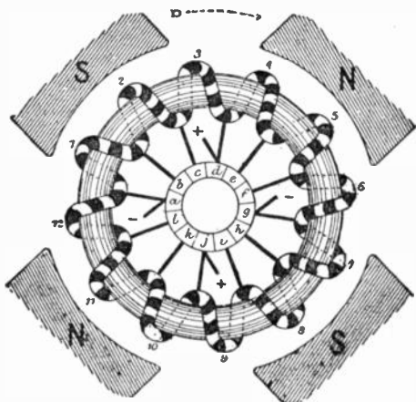
FIG. 254.—End of ring winding for a four pole machine. An end view is simply a view showing the arrangement of the armature inductors and connections looking from the front or commutator end. A developed view of the above winding is shown in fig. 257.
