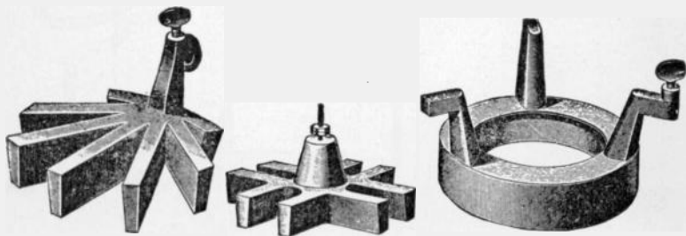
FIGS. 67 to 69.—Various zincs: fig. 67 Crowfoot; fig. 68 Lockwood; fig. 69 fire alarm.
