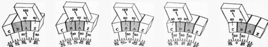
FIGS. 319 to 323.—Brush contact theory of commutation for case in which the brush covers two segments of the commutator. Fig. 319 beginning of commutation; fig. 320 one-quarter period; fig. 321, one-half period; fig. 322, three-quarter period; fig. 323 completion of commutation.
