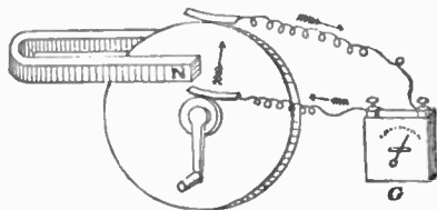
FIG. 126.—Faraday's dynamo which embodies his discovery in 1831 of electromagnetic induction , the principle upon which all dynamos work, as well as induction coils, transformers, and other electrical apparatus.
