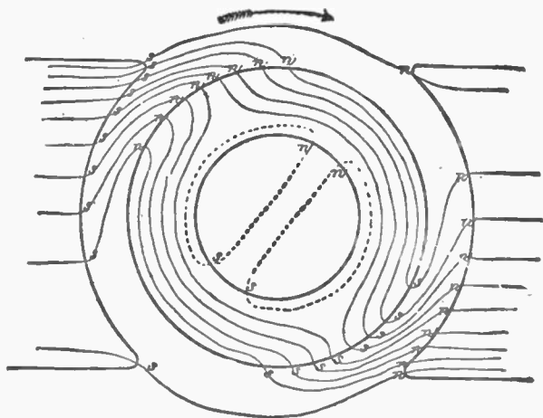
FIG. 286. —Distortion of magnetic field due to cross magnetization. For clearness, the effect is shown somewhat exaggerated. A drag or resistance to the movement of the armature is caused by the attraction of the north and south poles on the armature and pole pieces respectively.
