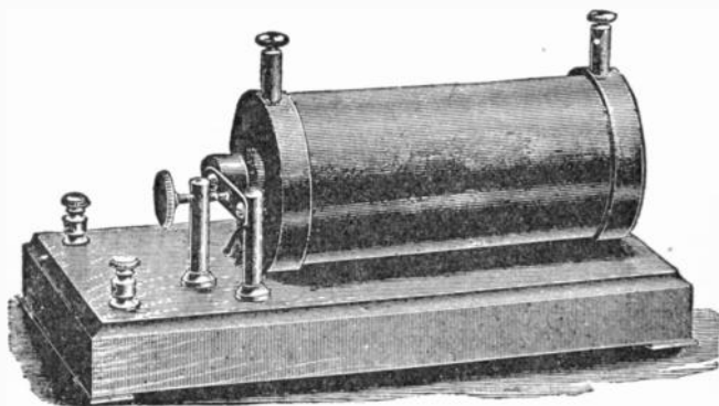
FIG. 140. —Rhumkorff induction coil. A secondary coil with vibrator and condenser; a type generally used in the laboratory. The name Rhumkorff was formerly very widely applied to induction coils for the reason that some of the earliest coils were constructed by Rhumkorff.
