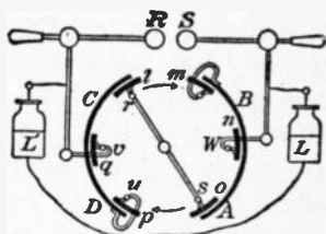
FIG. 33.—Principle of Toeppler-Holtz electric machine.
