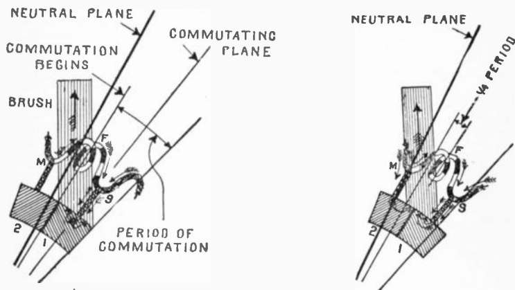
Figs. 309 to 313. —How sparkless commutation is obtained by advancing the brushes beyond the neutral plane; commutation progressively shown.
