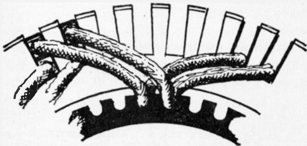
FIGS. 372 and 373. — Barrel and evolute windings; end views showing placement of coils. When all the coils are wound on the former, the placing of them on the armature is a simple matter. After insulating the slots, the winder begins at any convenient slot, and inserts the coils as shown. Before he can fill all the slots, some of the first coils must be raised and the last ones inserted underneath. There is not much difference between barrel and evolute winding and one style may be used at one end of the armature and the other at the opposite end.
