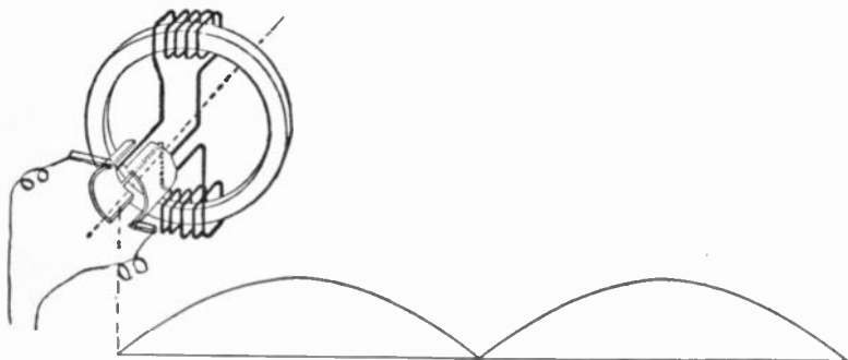
FIG. 183.—Gramme ring armature with two coils placed 180^\circ apart. This arrangement gives double the pressure of the one coil armature, fig. 182.
