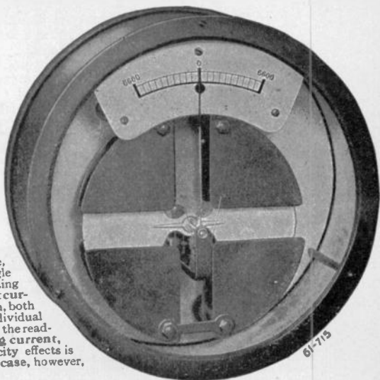
FIG. 2.580.—Westinghouse single phase electrostatic ground detector.
