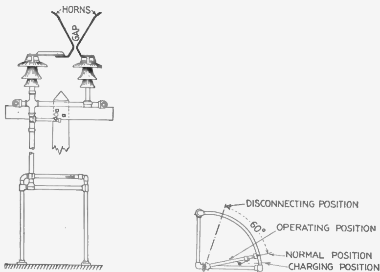
FIGS. 2.383 and 2.381.—Elevation and plan of General Electric horn gaps and operating stand for high voltage arresters.
