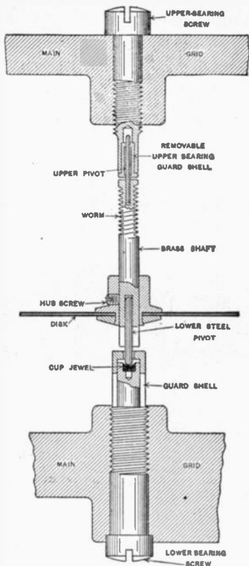
FIG. 2,548.—Bearing system of Sangamo single phase induction watt-hour meter. The upper pivot, or bearing is made of tempered steel wire and of sufficiently small diameter to be quite flexible in the length between the top of the brass shaft and the guide ring in which it rotates. The guide ring, made of phosphor bronze, has the heavy hole lined and burnished. The upper bearing screw, in which the bronze bushing is carried, is so constructed that a long brass sleeve closely surrounds the upper pivot of the spindle. Any blow against the moving system, caused by accident or short circuit, will slightly deflect the shaft until the moving pivot touches against the side of the shell, thus preventing danger of breaking off or bending the upper pivot. At the same time a cushioning or flexible action between the shaft and the bearing shell is secured, thus eliminating the effect of vibration in the moving system, which would tend to produce rattling. The lower bearing consists of a cup sapphire jewel, supported in a threaded pillar, the upper end of which is provided with a sleeve so located that it prevents the moving element dropping out during shipment. This protecting sleeve is held friction tight on the shaft and can be removed if it be desired to inspect the jewel.
