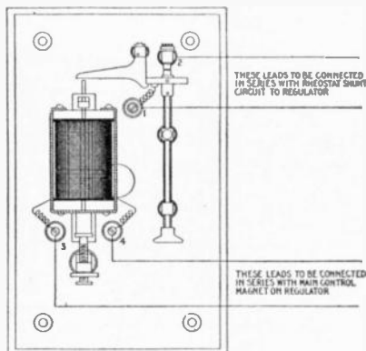
FIG. 2,434.—Diagram of connections of General Electric high voltage cut out relay (form 2434) for voltage regulators. Its use in connection with the regulator protects the system from any sudden rise in voltage due to some accident to the regulator which might cause the relay contacts to stick, thus producing full field on the exciter. In construction, the control magnet is connected in series with the alternating current control magnet on the regulator and the contacts are connected in series with the rheostat shunt circuit. Then, should the voltage rise beyond a certain value, predetermined by the setting of the thumb screw supporting the plunger of the control magnet, the contacts of the relay are tripped open which, by inserting all the resistance in the exciter field, reduces the exciter voltage which in turn reduces the alternating current voltage. This relay has to be reset by hand.
