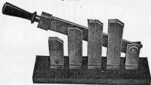
FIG. 2,218.—Westinghouse rear connected motor starting switch, for pressures up to 600 volts. It is used for starting rotary converters and direct current motors of large capacity having starting torque small enough to permit cutting out the starting resistance in few steps. The clips can be connected to any type of resistor, the steps of which are successively short circuited as the switch closes; the amount of resistance in the armature circuit is thus gradually reduced. A pause should be made after each step of resistance is thrown in to allow the motor speed to accelerate. If the starting switch do not have to carry the full load current and can be short circuited by another switch, a starting switch of smaller capacity equivalent to 50 per cent of running current of the machine can be used. The switch is of the single pole, single throw, rear connected, four point, knife blade type.
