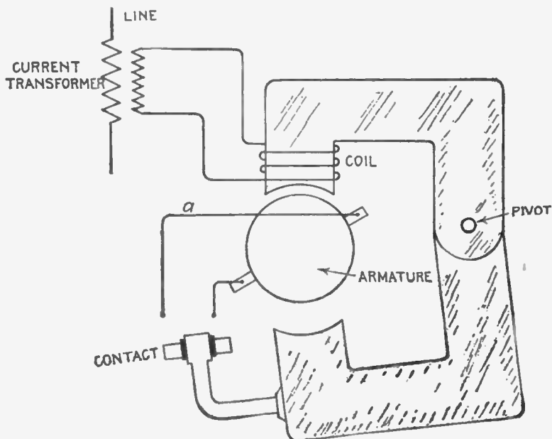
FIG. 2,307.—Electric circuits of Condit type "A" relay. The construction is described in fig. 2,309. As here shown, the relay is not in operation, but should the current passing through the coil be of sufficient value to cause the lower movable half of the magnetic circuit to approach the upper stationary half of the circuit, the relay will be transformed from an ordinary electromagnet into a repulsion motor. The contact will short circuit the brushes of the armature and thus cause it to revolve, the speed of rotation being dependent on the amount of current flowing to a predetermined point, and thereafter the speed of rotation of the motor remains constant irrespective of the current value. Time adjustment: This is obtained by varying the distance through which the contact travels, provision being made whereby adjustment can be made as close as .1 of a second. Current adjustment: This is obtained by means of a calibrated spring. Standard relays are calibrated at 6, 8, 10, and 12 amperes, the coils being designed to carry five amperes continuously, with a temperature rise not exceeding 86° Fahr. Power to operate relay: The relay requires twenty volt amperes for its operation at full load; the influence of this type of relay on the ratio and phase angle of current transformers is small.
