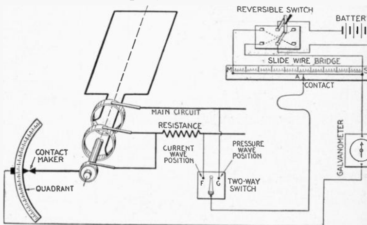
FIG. 2,595.—Diagram illustrating zero method of wave measurement with contact maker. The voltage of the battery must be at least as great as the maximum pressure to be measured and must be kept constant.
