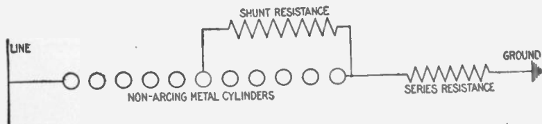
FIG. 2,350.—Low equivalent arrester. This is a modification of the multi-gap arrester shown in fig. 2,349. About half of the total number of gaps are shunted by a resistance, and another resistance inserted between the cylinders and the earth. With this arrangement the middle point is at ground pressure, and there are between line and ground only one half of the total number of gaps. This is sufficient to prevent a bridging of the gaps under normal conditions.
