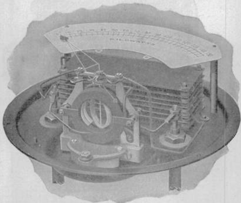
FIG 2,527—Interior Weston single phase wattmeter. The general appearance of the dynamometer movement and the relative positions of the various parts are clearly shown. The parts are assembled on one base, the whole movement being removable by unfastening two bolts. The fixed winding is made up of two coils, which together produce the field of the wattmeter. The movable coil is wound to gauge with silk covered wire and treated with cement. While winding, the coil is spread at diametrical points to allow the insertion of the staff, which is centered by means of two curved plates cemented to the inside surface of the coil and forming a part thereof. The coil is held in a definite position by two tiny pins which pass through the staff and engage with ears on the curved plates.
