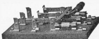
FIG. 2,206.—Westinghouse fused starting switch for squirrel cage motors. It is arranged, or National Electric Code fuses on one end only and has springs on the other end to open the switch automatically if left closed at this end. The corresponding terminals at both ends of the switch are connected in grooves in the back of the slate base so that the wiring need be connected to one set of these terminals only, thus decreasing the number of connections necessary, as shown in fig. 2,207. In starting an induction motor, the switch is thrown to the end that is not fused and held there until the motor is up to running speed; then it is quickly thrown to the fused position, thus protecting the circuit under running conditions.
