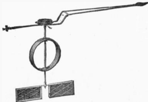
FIG. 2,520. —Pointer and movable system of Weston wattmeter. The coil is described in fig. 2,527. The pointer consists of a triangular truss with tubular members, an index tip of very thin metal being mounted at its extremity. The index tip is reinforced by a rib stamped into the metal. The pointer is permanently joined to a balance cross, consisting of a flat center web, provided with two short arms and one long arm, each arm carrying a nut by means of which the balance of the system may be adjusted. The longest arm, which is opposite the pointer, carries a balance nut, consisting of a thin walled sleeve provided with a relatively large flange at its outer end. The sleeve is tapped with 272 threads to the inch, the internal diameter of the sleeve being made slightly smaller than the outside diameter of the screw, and the sleeve is split lengthwise; therefore when sprung into place and properly adjusted it will remain permanently in position. A sleeve which is forced over the end of the staff carries the pointer firmly clamped between a flanged shoulder and a nut. By perforating the web plate of the balance cross with a hole having two flat sides that fit snugly over a similarly shaped portion of the sleeve, the pointer is given a definite and permanently fixed angular position. The air damper consists of two very light symmetrically disposed vanes, which are enclosed in chambers made as nearly air tight as possible. These vanes are formed of very thin metal stiffened by ribs, stamped into them and by the edges, which are bent over to conform to the surface of the side walls of the chambers. They are attached by metal eyelets to a cross bar carried on a sleeve similar in construction to the one at the upper end of the staff. This cross bar is held in place by a nut, and is provided at the center with a hole having two flat sides, being similar in shape to the one in the balance cross. This hole likewise fits over a sleeve and definitely locates the vanes with reference to the other parts of the system. The damper box is cast in one piece to form the base that carries the field coils and the movable system.
