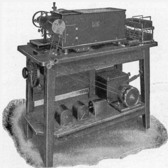
FIG. 2,599.—General Electric moving coil oscillograph complete with tracing table. The tracing table is employed for observing the waves, and by using a piece of transparent paper, the waves under observation appear as a continuous band of light which can be traced, thus making a permanent record. This is not, however, to be regarded as a recording attachment, and can not be used where instantaneous phenomena are being investigated. The synchronous motor for operating the synchronous mirror in connection with tracing and viewing attachment is wound for 100 to 115 volts, 25 to 125 cycles, and should, of course, be run from the same machine which furnishes power to the circuit under observation. A rheostat for steadying and adjusting the current should be connected in series with the motor. The beam from the vibrator mirrors striking this synchronous mirror moves back and forth over the curved glass, and gives the length of the wave; the movement of the vibrator mirror gives the amplitude, and the combination gives the wave complete. An arc lamp or projection lantern produces the image reflected by the mirrors upon the film, tracing table or screen. For the rotation of the photographic film, a small direct current shunt wound motor is ordinarily used.
