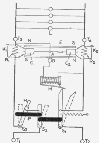
FIG. 2,582.—Wallis-Jones automatic earth leakage cut out. It is an instrument which protects a direct current circuit that the circuit is broken whenever a leak occurs from either main to earth, and so that the circuit cannot be permanently re-established until the leak has been removed. The instrument and its connections may be explained by the aid of the accompanying diagram, in which T_1 and T_2 represent the points of connection from the mains, and T_3 and T_4 , the points of connection to the circuit to be protected. S_1 , S_2 , and S_3 will preferably be ordinary tumbler switches, but they are diagrammatically represented as plain bar switches, their fixed contacts being diagrammatically represented by dotted circles. When the three switches S_1 , S_2 , and S_3 are closed, the current passes from T_1 to T_3 through the small resistance R_1 , through circuit L to T_4 , and back through the resistance R_2 to T_2 . In shunt with R_1 and R_2 are the two moving coils C and C_2 , working in the magnetic field of the magnets NS , NS' , and rigidly fixed on one spindle, which is broken electrically by an ebonite block E . The points of connection to the shunts are adjusted so that when the same current passes out through one and back through the other, the effect on the two coils is equal and opposite, and there is thus no movement. Should, however, any minute portion of the current through R_1 leak to earth instead of returning via R_2 , the balance is disturbed, C becomes stronger than C_2 , the system is deflected, and a contact is made by the arm A at B , no matter in which direction the coils deflect. The system is similarly deflected for a leak on the other lead. In the diagram these contacts are shown at right angles to their normal plane. As soon as the contact is made, the electromagnet M is energized, the arm of S_1 is released and the spring at once pulls it off its contact, at the same time breaking S_2 . The positions of the blades when the switches are open are shown dotted. The only means the user has of closing the circuit is by putting on S_3 by the handle H , which is outside the locked box. The first effect of putting on S_3 is to break its circuit; it then by means of the slotted bar P begins to pull on S_2 and S_1 , which can thus be closed again, and held closed by the trigger as before. The circuit, is, however, still broken till S_3 is pushed back. Then if the leak is still on, the slot in P allows S_1 and S_2 to open at once as before. It is therefore impossible to keep the circuit closed while the leak exists. The working condition of the instrument can be tested at any time by switching a lamp on in the circuit and depressing one of the keys K_1 , K_2 . This short circuits R_1 or R_2 , throws the coils out of balance, and the switch opens. The contact arm is closed in an inner dust tight case, and it will be noted that it makes contact only; the break occurs at the switches, thus avoiding any sparking. Since the two coils work in the two gaps of one and the same field, changes in the strength of the magnets have no effect, the apparatus is enclosed in a locked metallic box, and the only part to which the user has access is the handle H , and, if desired, the testing keys K_1 , K_2 .
