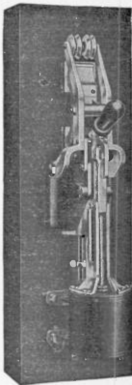
FIG. 2.331.—Condit 600 volt, 1,500 ampere, single pole type K circuit breaker pneumatically operated. It is the same as the electrically operated circuit breaker, except that a pneumatic cylinder mechanism is supplied in place of either the electromagnet or the motor. This cylinder mechanism is so arranged that the air pressure
