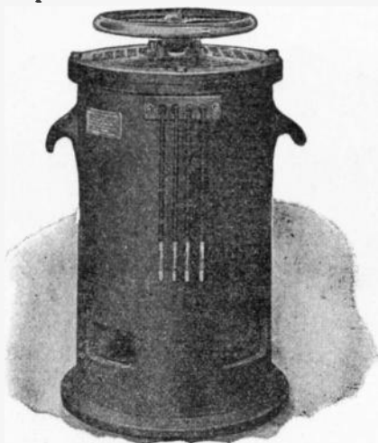
FIG. 2,421.—Westinghouse two kw., hand operated, air cooled induction regulator for testing purposes.
