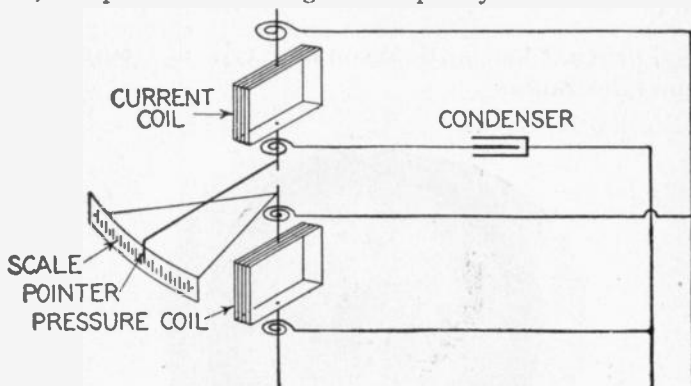
FIG. 2,568.—Langsdorf and Begole frequency meter. The operation of this meter is based on the fact that if an alternating pressure of E Volts be impressed on a condenser of capacity C , in farads, the current in amperes will be equal to 2\pi \sim EC , provided the pressure be constant. In construction, the scale is mounted on the same axis as the pressure coil, across the mains so as to render the instrument independent of variation of voltage. For a discussion of this meter, see Electrical Review , vol. LVIII, page 114.
