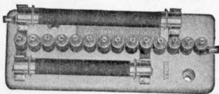
FIG. 2,351.—General Electric 2,200 volt multi-gap arrester for station installation. It consists of fourteen \frac{5}{8} " knurled cylinders and two shunt resistance rods mounted on a pre-ceramic base. One of these rods has a low resistance, and shunts nine gaps; the other rod has a high resistance, and shunts eleven gaps. The effect of the shunt resistance in extinguishing the line current arc is the same, therefore, as that of an equal series resistance but is without the objectionable features of the latter. Series resistance limits the discharge current to such an extent that an arrester with series resistance fails to protect against destructive rises of voltage when the conditions are severest. Graded shunt resistance responds to all frequencies and opens a discharge path for excessive voltage when the frequencies are high as well as when they are low. Its further effect is in withholding the line current from the gaps after the relieving discharge has occurred, is to aid the non-arcing quality of the metal cylinders in quickly suppressing the arc that follows a discharge. The arc is extinguished at the end of the half cycle of line current in which the discharge takes place.
