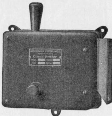
FIG. 2,244.—Westinghouse magnetic blow out circuit breaker, designed for the protection of street railway and electric locomotive equipments; it serves the combined purpose of fuse block and canopy switch. The contact tips are surrounded by a moulded arc chute which confines and directs the arc until the magnetic blow out extinguishes it. The current carrying contacts consist of copper strips separated by air spaces. An auxiliary contact or "arcing tip" at the end of the switch lever takes the burning of the arc when the breaker opens, and thus confines the burning to a very small piece which can be easily removed and replaced at small cost. The hand tripping lever and the resetting lever have insulated handles, so that they can be safely handled, even in the dark.
