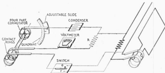
FIG. 2,590.—Four part commutator method of wave form measurement. The contact device consists of two slip rings and a four part commutator. One slip ring is connected to one terminal of the source, the other to the voltmeter, and the commutator to the condenser. By adjusting R when a known direct current pressure is impressed across the terminals, the voltmeter can be rendered direct reading.
