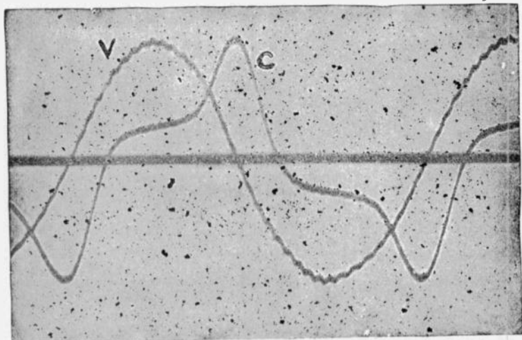
FIGS. 2,593 and 2,594.—Two curves representing pressure and current respectively of a rotary converter. Fig. 2,593, pressure wave V, fig. 2,594 current wave C. These waves were obtained from a converter which was being driven by an alternator by means of an independent motor. The rotary converter was supplying idle current to some unloaded transformers and the ripples clearly visible in the pressure wave V, correspond to the number of teeth in the armature of the rotary converter.
