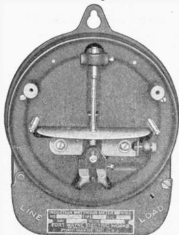
FIG. 2,544. —Fort Wayne single phase induction watt-hour meter with cover register and permanent magnets removed to show solid meter frame. A heavy steel back plate held in place by two screws inserted from the front of the central casting encloses the back part of the completely assembled meter. A felt gasket lying on a suitable ledge seals the joint against the entrance of dust or moisture when the back plate is drawn down firmly by the screws. The cover which encloses the back part of the meter is a non-magnetic metallic stamping. It is held in place by wing nuts on the two light brass studs extending forward from the meter frame. This joint between the main frame and the cover is also sealed against the entrance of dust and moisture by the use of a suitable felt gasket. Two glass windows are provided in this cover, one to permit the reading of the register dials, the other to permit observation of the disc's rotation. The cover is sealed in place in the usual way by passing a sealing wire through a hole drilled in the cover sealing stud and thence through a hole provided in the wing of the seal nut. The terminal chamber is an extension of the casting which supports all the inner parts of the meter. The heavy brass terminals used for connecting the meter in circuit are held permanently by a non-combustible insulating compound which is moulded in place around them. This construction gives excellent insulation and is a safeguard against accidental short circuits across terminals. A punched terminal cover which fits over the terminal chamber is hinged at the upper left hand corner so that it will of its own accord swing out of the way when the terminal cover sealing screw is removed. This hinged style of cover will be found convenient when installing and connecting the meter in circuit. When this cover is swung back into closed position it is fastened in place by passing a seal right through the seal screw and through a lug provided on the cover.
