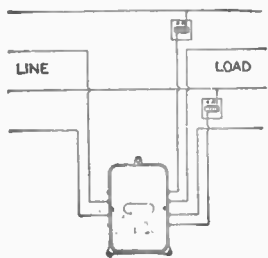
FIGS. 2,537 to 2,541.—Connections of Fort Wayne multi-phase watt hour meters (type k 3 —forms MAB and MAK), for 100–625 volt circuits, 5–150 amperes. Fig. 2,538 two and three phase, three wire circuit, 25–36 cycles; fig. 2,539 two and three phase, 3 wire circuit, 36 cycles and above; fig. 2,540, two phase 4 wire circuit, 25–36 cycles; fig. 2,541 two phase, 4 wire circuit 36 cycles and above.
