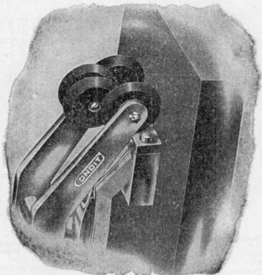
FIG. 2,248.—Carbon break discs of Condit circuit breaker. The two pairs of similar discs which slide past each other are so arranged that these surfaces coincide at the instant the intermediate contact separate after which, as the contact arm opens further, they gradually disengage.
