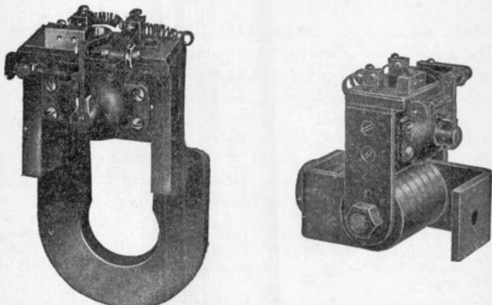
FIGS. 2,338 and 2,339.—General Electric instantaneous direct current reverse current or "discriminating" relays. Fig. 2,238, for 500 amperes; fig. 2,339 for 2,000 amperes. These relays are designed for mounting directly on circuit breaker studs. These relays consist of a horseshoe magnet with a shunt wound armature pivoted between its poles. The magnet is mounted on the current carrying stud of the circuit breaker between the back of the panel and the first contact or supporting nut, and is placed in a vertical position. The contacts are insulated from the magnet permitting the use of an auxiliary circuit for the tripping device, independent of the circuit controlled by the circuit breaker. The magnet is excited by the current flowing through the stud, and the armature is connected across the line in series with suitable resistance. Rotation of the armature in the normal direction is prevented by a stop. Reversal of the current flowing through the stud changes the direction in which the armature tends to rotate, causing it to move away from the stop and close the circuit through an auxiliary trip coil and trip the circuit breaker. These relays are used to protect dynamos, storage batteries, or main station busses from damage on reversal of current due to short circuit, or from the grounding of machines or connection. Relay contacts must not be used to open the shunt trip coil circuits. An auxiliary switch should be provided for this purpose in all cases where the opening of the circuit breaker does not disconnect the trip coil from the source of supply.
