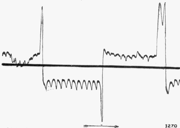
FIGS. 2,585 and 2,586.—Oscillograms (from paper by Morris and Catterson-Smith, Proc. I. E. E., Vol. XXXIII, page 1,023), showing how the current varies in one of the armature coils of a direct current motor. Fig. 2,585 was obtained with the brushes in the neutral position, and fig. 2,586 with the brushes shifted forward.
