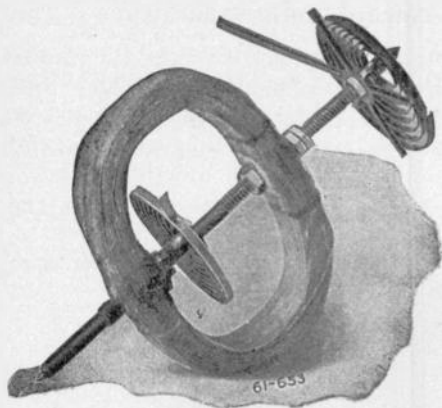
FIG. 2.515.— Armature of Wagner dynamometer movement. Greater accuracy is claimed for this movement than the magnetic vane, but it cannot readily be employed for the indication of current flow, as required in ammeters. The magnetic vane movement is used on the A. C. ammeter, and can be used also in the A. C. voltmeters; it makes use of its controlling spring only for the purpose of resisting the pull on the vane and the returning of the pointer to zero. The dynamometer movement is recommended for voltmeters.
