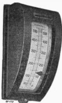
Figs. 2,520 to 2,526.—Various types of Wagner instruments. Fig. 2,520, small round type; fig. 2,521, horizontal edgewise type; fig. 2,522, smallest switchboard type; fig. 2,523, portable type; fig. 2,524, combination voltmeter and ammeter in one case; fig. 2,525, vertical type; fig. 2,526, polyphase type.
