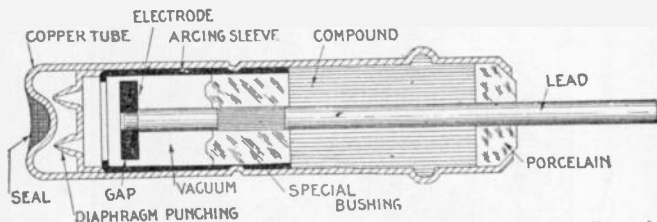
FIG. 2,306.—Sectional view of General Electric vacuum tube arrester for railway signal circuits. The arrester is essentially a gap in a vacuum. In construction, the gap is formed between the inner wall of a drawn metal shell and a disc electrode mounted concentric with it. The electrode is supported on a brass rod which serves as the lead in connection, and has ample current carrying capacity. The electrode system is insulated from the tube and rigidly supported in position by a bushing made of vitreous material. The bushing does not form the vacuum seal, that being made by a special compound. The open end of the tube is finally closed by a porcelain bushing. The tube is exhausted in a special machine which solders a small hole in the end after the vacuum has been established. The possibility of solder entering the active part of the vacuum space is prevented by a diaphragm punching, and both the electrode and the lining of the tube are of non-arcing metal. The arrester has a spark pressure of from 350 to 600 volts direct current, and an equivalent needle gap of about .005 inch. The arrester will not stand a continuous flow of current due to excessive heating, hence if there be a possibility of this due to high pressure crosses, fuses should be used. R. R. S. A. standard terminals are used.
