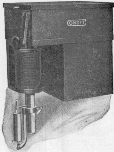
FIG. 2.310.—Condit type "B" time limit attachment, designed to give sufficient time to allow an induction motor to start without opening the circuit breaker, and not have the circuit breaker trip on the momentary rush of current. Its action is inverse; that is, the greater the current the less time it takes to operate and is so arranged that four to five times full load current or a short circuit will trip the circuit breaker instantly. The time limit attachment is applied directly to the armature which trips the circuit breaker and is adapted for the so called primary trip. It consists of an air vacuum dash pot with a graphite piston, the dash pot being fastened to the stationary calibrating ring of the trip coil and the moving outside cylinder is fastened to the armature of the circuit breaker. When the current reaches a point where it overcomes the weight of the armature and lifts the same, the magnetic force tending to raise the armature is opposed by the vacuum created in the interior of the cylinder. As the magnetic force continues, the vacuum is overcome due to the leakage of air past the plunger and the armature gradually moves up until it reaches the point where it trips the circuit breaker. If at any point of the armature travel, the current drop back to normal, the armature immediately resets itself by means of a ball valve in the top of the brass cylinder
