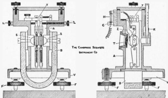
FIGS. 2,614 and 2,615.—Sectional view of permanent magnet form of Duddell moving coil oscillograph. This instrument has a lower natural period of vibration ( \frac{1}{3,000} second) than the type shown in fig. 2,612, and therefore is not capable of accurately following wave forms of such high frequency, but it is sufficiently quick acting to follow wave forms of all ordinary frequencies with perfect accuracy. It is easier to repair, and more portable, owing to the fact that the magnetic field is produced by a permanent magnet instead of an electro-magnet. This also renders the instrument suitable for use on high tension circuits without earth connection, as, owing to the fact that no direct current excitation is required, the instrument is more easily insulated than other types.
