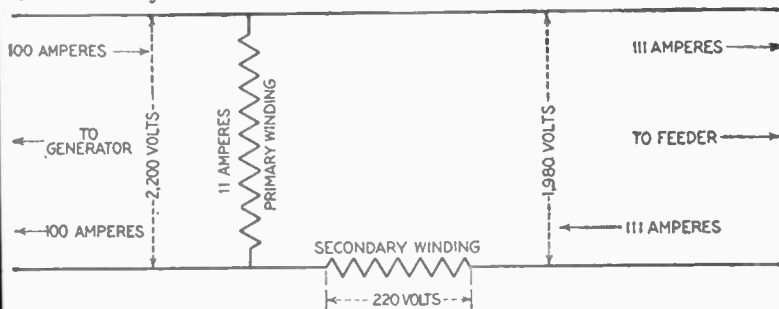
FIG. 2,416.—Diagram of induction regulator lowering the voltage 10%. The diagram shows the regulator lowering the feeder pressure to 1,980 volts with an increase of the secondary current to 111 amperes, the additional 11 amperes flowing from the feeder, through the primary back to the feeder.
