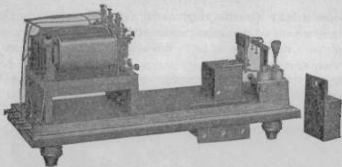
FIG. 2,601.—General Electric moving coil oscillograph with case removed, showing interior construction and arrangement of parts. The oscillograph is furnished complete with a three element electromagnet galvanometer, optical system, shutter and shutter operating mechanism, film driving motor and cone pulleys, photographic and tracing attachments, 6 film holders, and the following repair parts, for vibrators: 6 extra suspension strips; 6 vibrator mirrors; 1 box gold leaf fuses; 1 bottle mirror cement; 1 bottle damping liquid.
