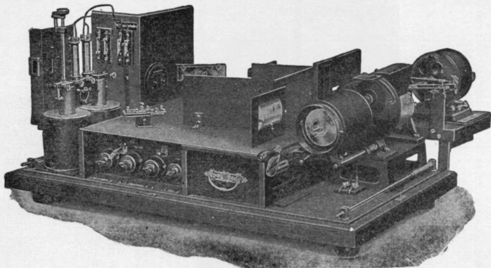
FIG. 2,604. —Siemens-Blondel moving coil type oscillograph. The coil is in the shape of a loop of thin wire, which is suspended in the field of an electro-magnet excited by continuous current. The current to be investigated is sent through this loop, which in consequence of the interaction of current and magnetic field, begins to vibrate. The oscillations are rendered visible by directing a beam of light from a continuous current arc lamp onto a small mirror fixed to the loop. The light reflected by the mirror is in the form of a light strip, but by suitable means this is drawn out in respect of time, so that a curve truly representing the current is obtained. The loop of fine wire is stretched between two supports and is kept in tension by a spring. As the spring tension is considerable, the directive force of the vibrating system is large, and its natural periodicity very high. The mirror is fixed in the center of the loop, and has an area of 1 square mm. In order to protect the loops from mechanical injury they are built into special frames. The mirrors are of various sizes, the loop for demonstration purposes (projection device) being provided with the largest mirror and the most sensitive loop with a mirror of the smallest dimensions.
