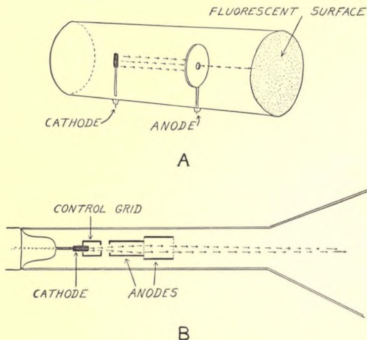
FIG. 15—A, Braun's cathode ray tube, with arrows indicating electron stream; B, portion of modern cathode ray tube used in television, showing the units of the electron gun, or electron-emitting and control apparatus. Arrows indicate electron beam.
