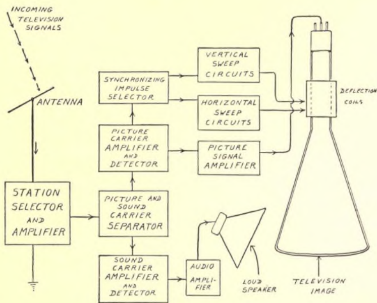
FIG. 53—Plan of a television receiver.
