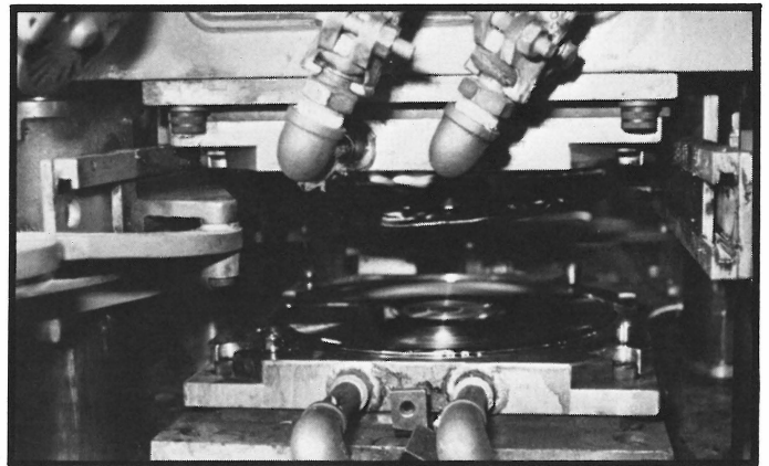
A stamper mounted in a record press.
