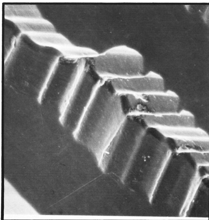
This photo shows the raised grooves of a metal master. The debris to be removed by de-ticking are clearly visible. (Photo courtesy of Stanton Magnetics)
