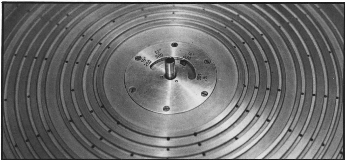
Close-up of the turntable of a Neumann Lathe, showing disc size selector and vacuum holes for disc hold-down.
