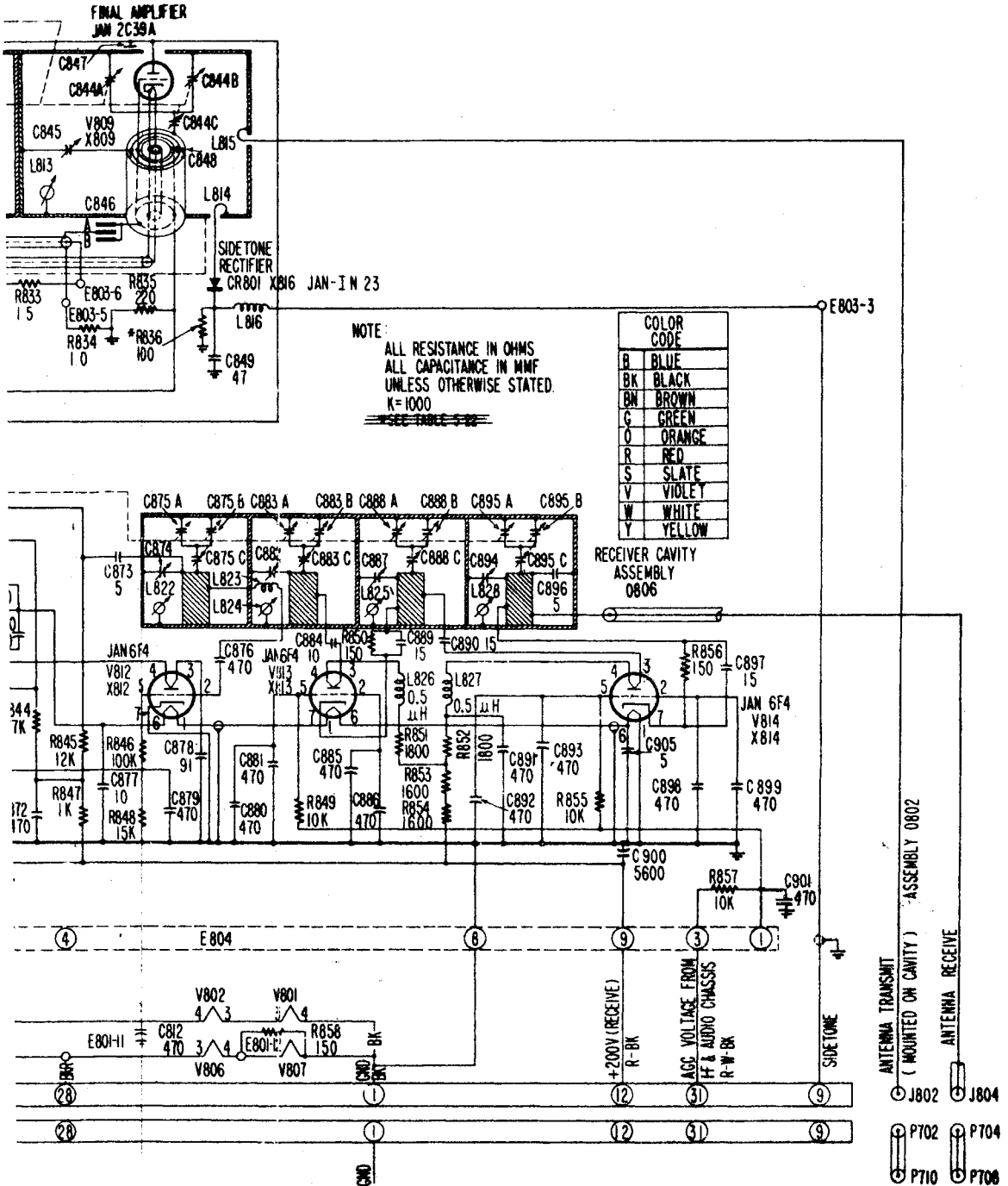
Figure 1-199. R-f head. Schematic diagram of main channel transmitter and receiver r-f circuits in Radio Set AN/ARC-33
