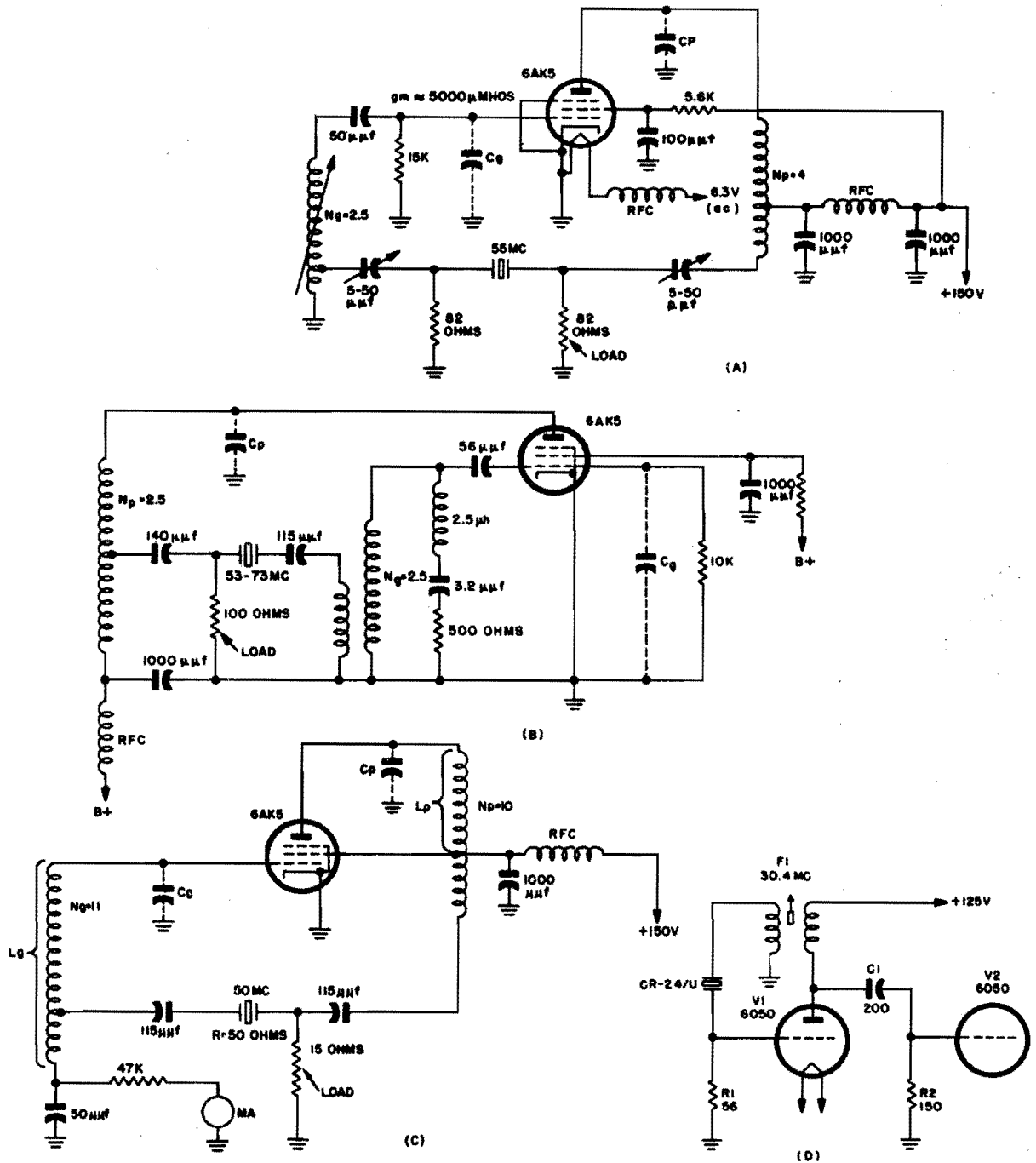
Figure 1-177. Modifications of transformer-coupled oscillator for: (A) High stability. (B) Untuned broad band. (C) Large output. (D) Slug-tuned, narrow band
