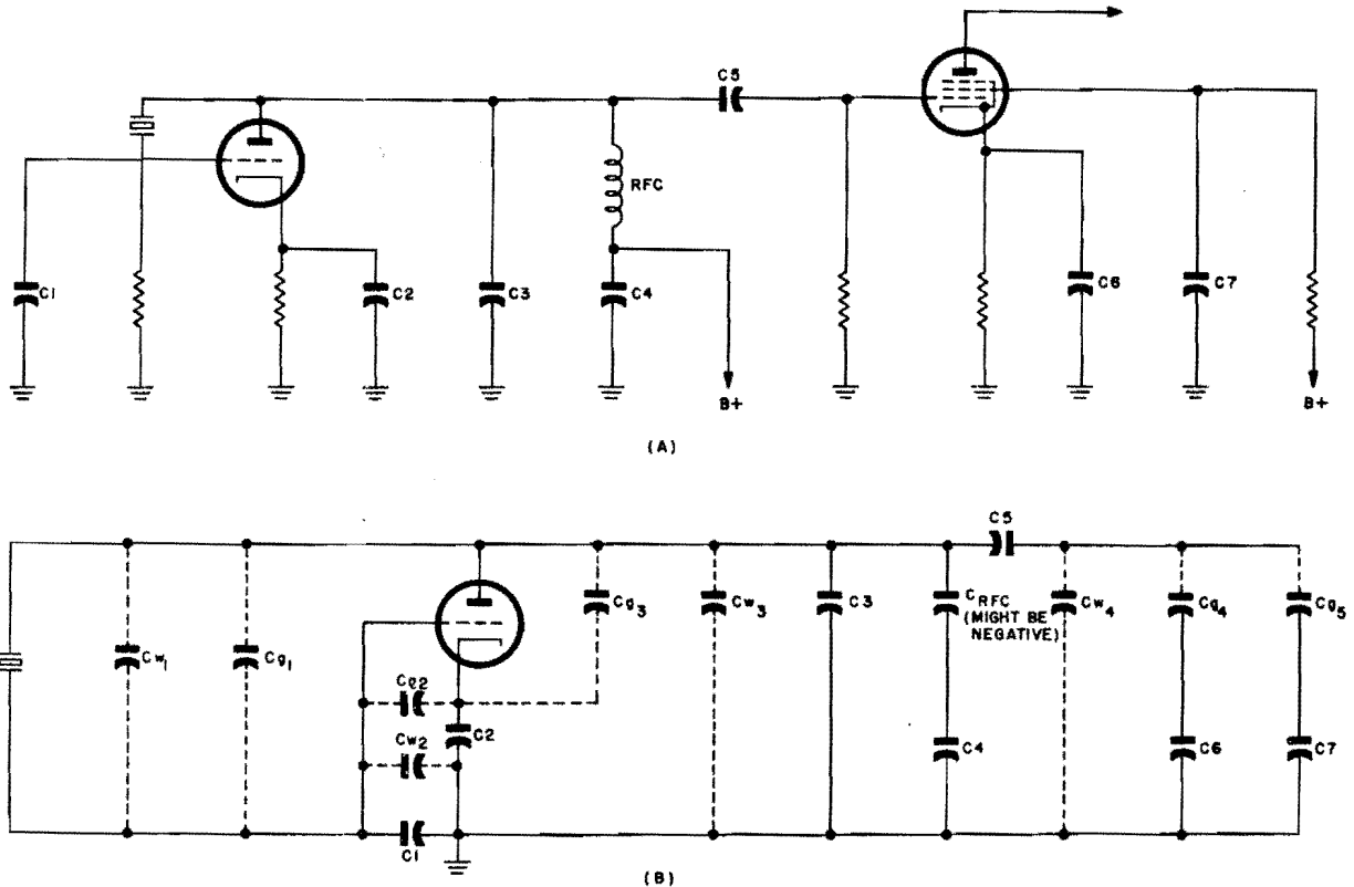
Figure 1-124. (A) Conventional Pierce oscillator and buffer-amplifier circuit. (B) Static capacitances of circuit (A). C_o = interelectrode capacitances. C_w = distributed capacitances of wires
