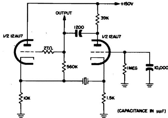
Figure 2-24. Schematic diagram of typical oscillator designed for use with Crystal Unit CR-30/U
