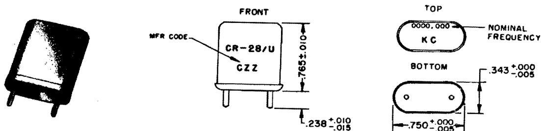
Figure 2-19. Crystal Unit CR-28/U
