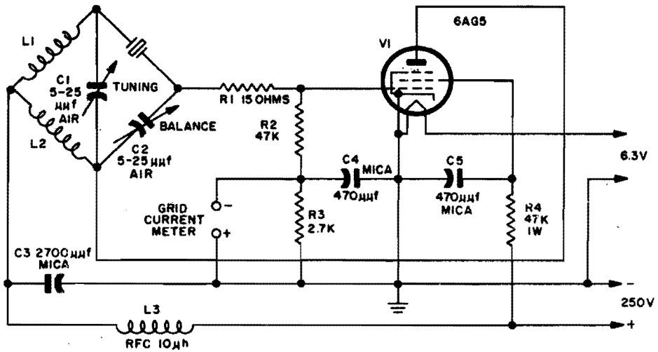
Figure 1-167. A single-tube capacitance-bridge oscillator which is practical for operation in the 50-90-mc frequency range. Resistors not otherwise specified are \frac{1}{2} w. L-1 and L-2 are a single center-tapped coil of suitable inductance
