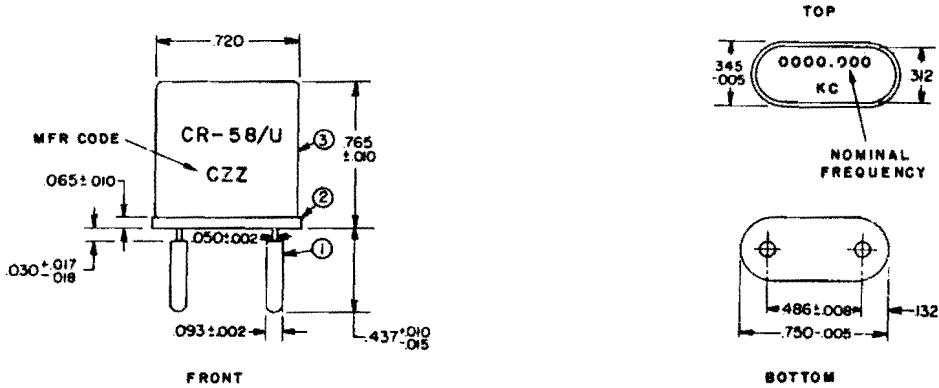
Figure 2-73. Crystal Unit CR-58/U
