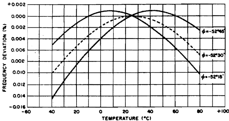
Figure 1-52. Temperature-frequency characteristics of element D
