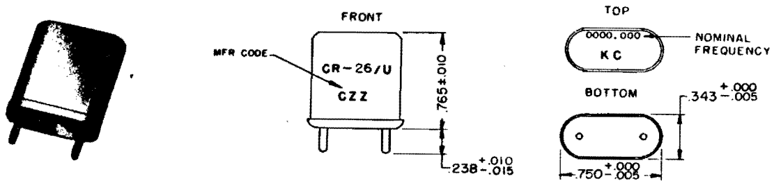
Figure 2-15. Crystal Unit CR-26/U
