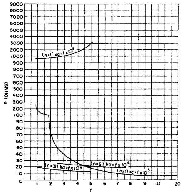
Figure 1-96. Typical curves of the series-arm resistance of plated crystals versus frequency. Actual series-arm resistances will vary between R/3 and 3R , where R is the value shown, except when R is less than 10 ohms, in which case the minimum resistance will be approximately one-half the value indicated. Values indicated are average for fundamental modes and approximately 1/2 the average for overtone modes
