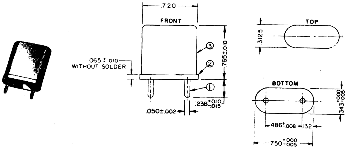
Figure 3-2. Crystal Holder HC-6/U
