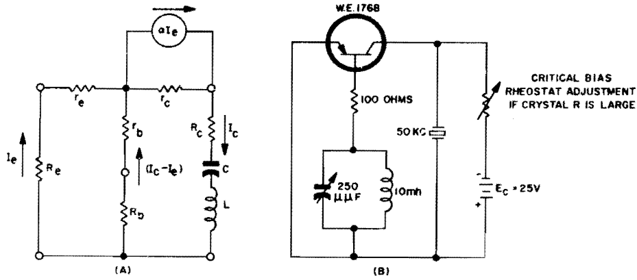
Figure 1-232. (A) Equivalent a-c circuit of tuned-collector negative-resistance oscillator. For crystal control, L , C , and R_c can be interpreted as being the series-arm parameters of a crystal unit; (B) Crystal-controlled tuned-collector negative-resistance oscillator. The parallel tuned tank is inserted in the base circuit in lieu of a resistor in order to obtain negative resistance values in excess of 40,000 ohms
