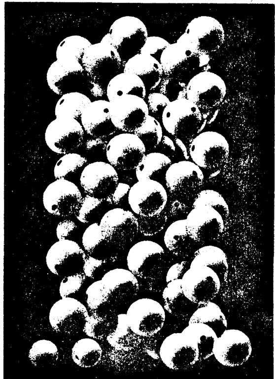
ARRANGEMENT OF ATOMS IN ALPHA QUARTZ, VIEWED ALONG AN X AXIS
