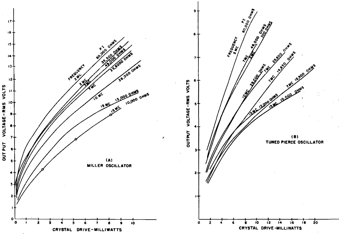
Figure 1-148. Output and crystal drive of experimental Miller and Pierce oscillators as d-c plate voltage is varied for crystal units of various frequencies and PI's. The values of PI assume a rated load capacitance of 32 \mu\mu\text{f} . Both oscillators were tuned to provide 50 percent (max) E_c and to operate into a 5000-ohm plate load
