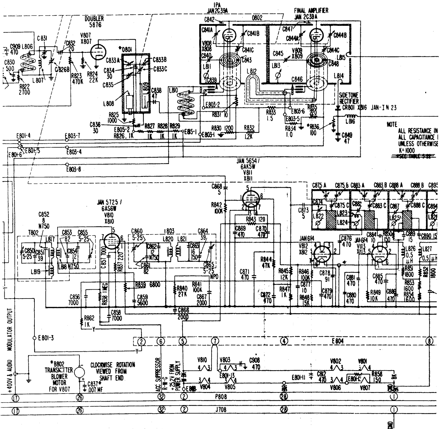
Figure 1-199. R-f head. Schem transmitter and receiver r-f circ
