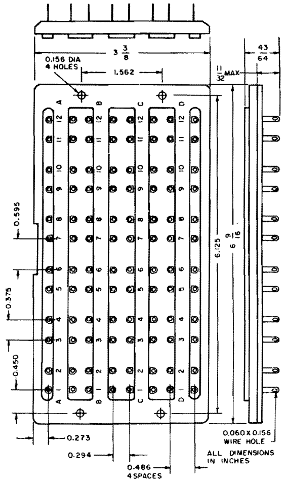
Figure 3-16. Multiple crystal socket for use with HC-6/U, HC-13/U, and HC-14/U holders
