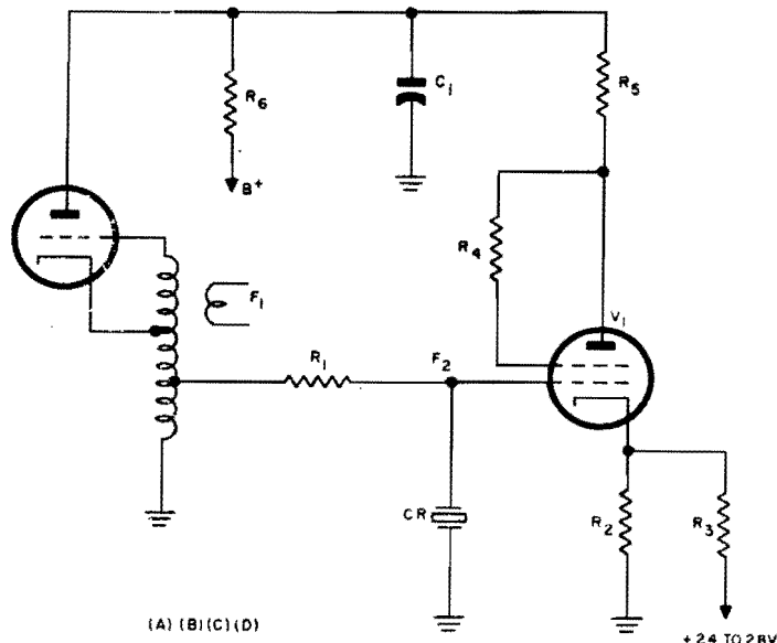
Figure 1-159. Crystal and magic-eye resonance indicator
