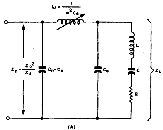
Figure 1-182. Impedance-inverting oscillator circuits. (A) Basic impedance-inverting network
