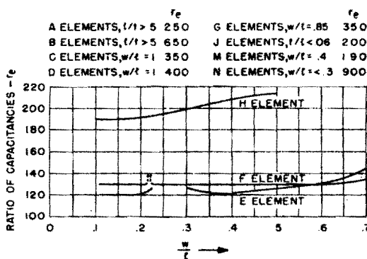
Figure 1-95. Approximate values of the ratio of capacitances, \Gamma_e = \frac{C_e}{C} , for various plated crystal elements
