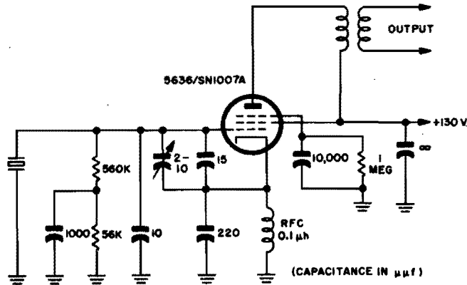
Figure 2-18. Schematic diagram of typical oscillator designed for use with Crystal Unit CR-27/U
