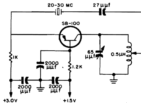
Figure 1-227. High-frequency transistor oscillator
