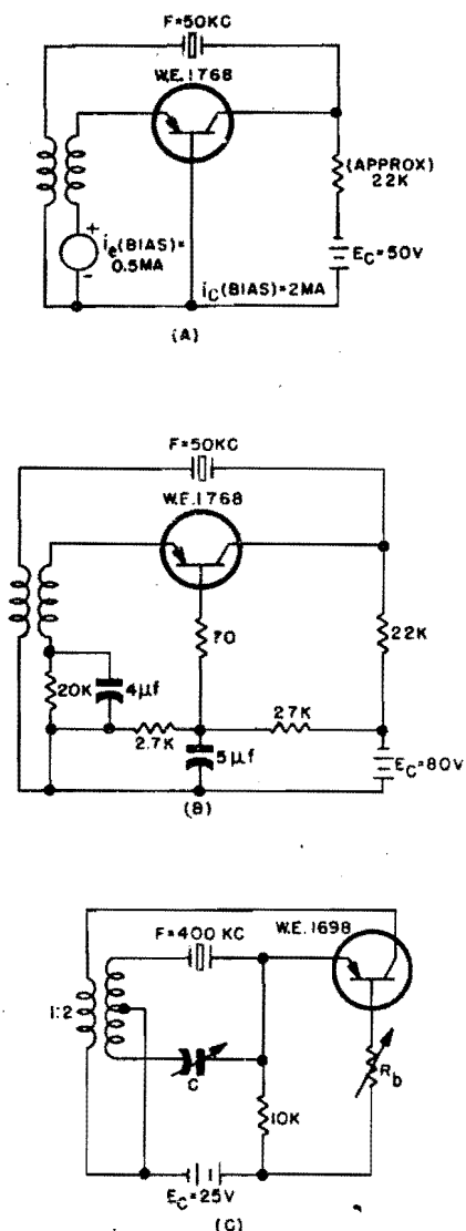
Figure 1-234. Transformer-coupled transistor oscillators
