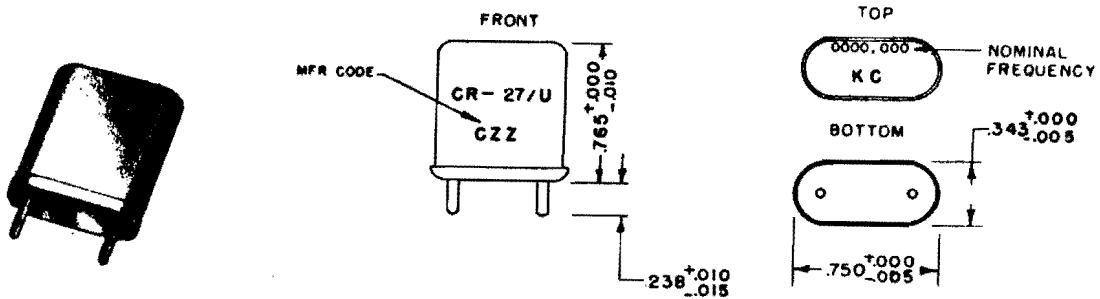
Figure 2-17. Crystal Unit CR-27/U
