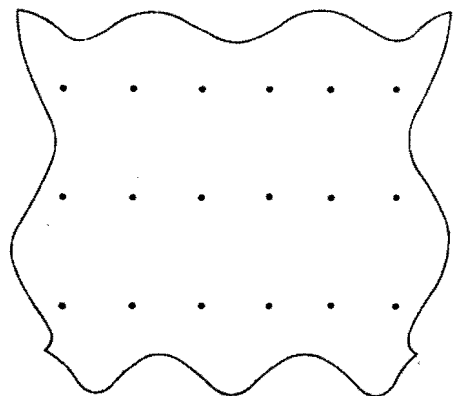
Figure 1-13. Face-shear mode for m = 6 , n = 3 . Dots indicate nodes *
