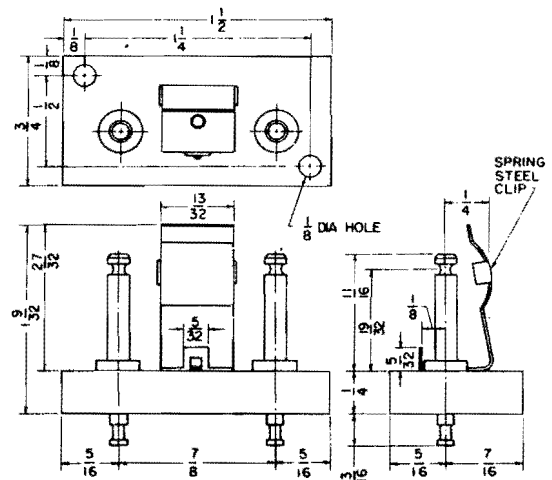
Figure 3-17. Crystal socket for use with HC-10/U holder
