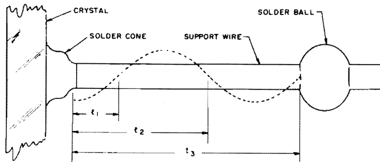
Figure 1-84. Solder-cone resonant-wire support. The solder ball "tunes" the wire to the crystal frequency if it is placed at a distance equal to an odd multiple of a quarter wavelength ( l_1, l_2, etc.) from the peak of the solder cone *
