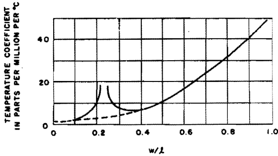
Figure 1-21. Temperature coefficient for length-extensional mode of X-cut crystal, where w is parallel to the Z axis, and t = 0.051
