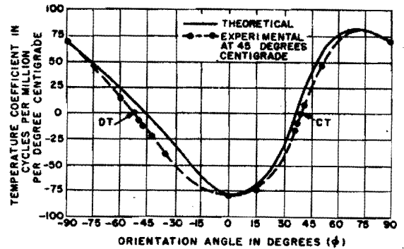
Figure 1-46. Temperature coefficient versus angle of rotation about X axis for face-shear elements of the Y group
