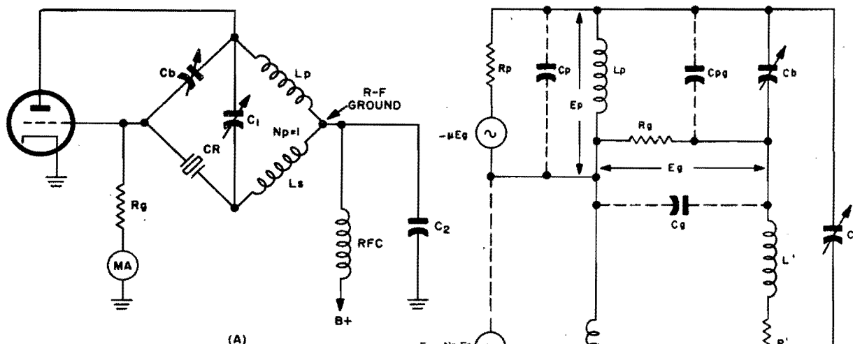
Figure 1-165. (A) Basic circuit of capacitance-bridge oscillator. (B) Equivalent circuit of capacitance-bridge oscillator
