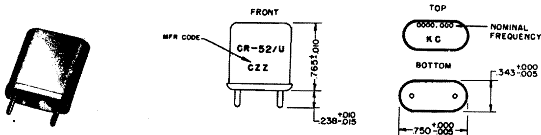
Figure 2-61. Crystal Unit CR-52/U
