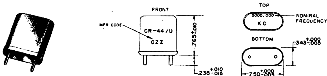
Figure 2-45. Crystal Unit CR-44/U
