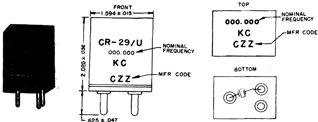
Figure 2-21. Crystal Unit CR-29/U
