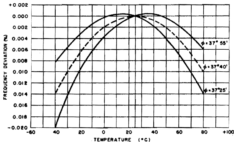
Figure 1-51. Temperature-frequency characteristics of element C
