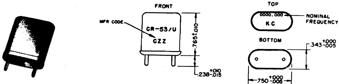
Figure 2-63. Crystal Unit CR-53/U
