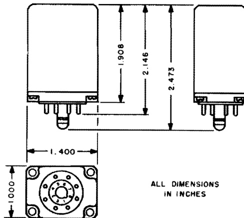
Figure 4-20. Dimensions of Crystal Oven HD-54/U
