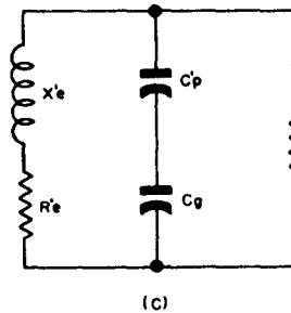
Figure 1-121. Generalized Pierce oscillator. X_e' and R_e' are the effective impedance parameters of the crystal unit based upon the assumption that C_{pg} is a part of C_o . C_x is an equivalent negative capacitance having a positive reactance equal to that of L_T . I_p is the r - f plate current of the vacuum tube.
