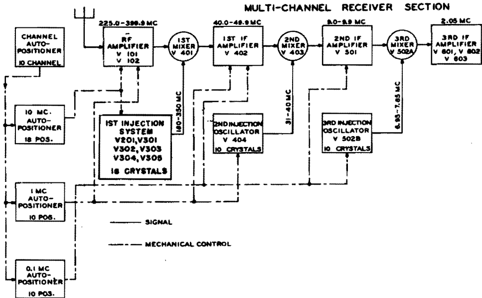
Figure 1-202. Block diagram and frequency chart of Collins frequency-control system as employed in Radio Receiver R-278/GR
