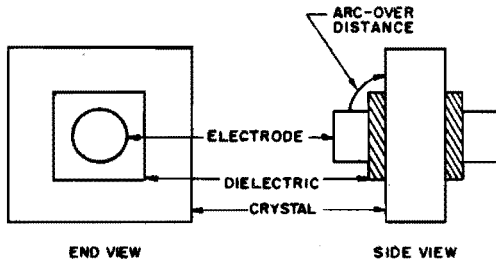
Figure 1-74. Center-pressure type of dielectric sandwich for mounting crystals
