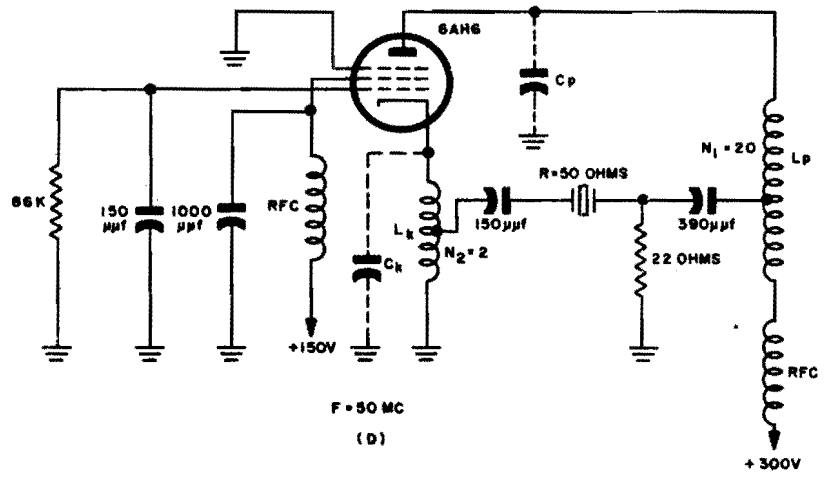
Figure 1-179. Modifications of grounded-grid oscillator. (B) Broad-band circuit. (C) Circuit for compensating crystal capacitance by mutual inductance. (D) High-efficiency class-C circuit
