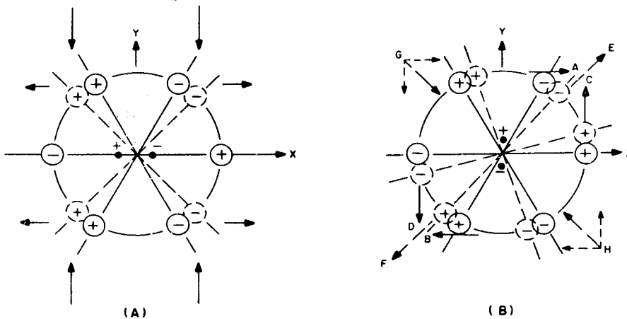
Figure 1-11. Equivalent distribution of charges that account for observed piezoelectric effects of alpha quartz. (A) Piezoelectric polarity along X axis of right quartz due to compression along Y axis. (B) Piezoelectric polarity of Y axis of right quartz due to shearing stress, where the resultant strain is equivalent to a compression along the axis designated GH. (Note that in both A and B, the piezoelectric effect is due to a rocking of the axial dipoles, and not to their compression or extension. To achieve the same deformations by the converse effect, equal voltages, but opposite in sign to the polarizations indicated, are applied across the respective axes) *
