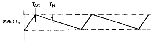
Figure 4-17. A-C component of heater temperature
