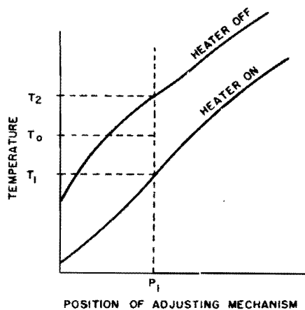
Figure 4-3. Typical differential curves of adjustable thermostat
