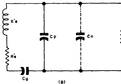
Figure 1-121. Generalized Pierce oscillator. X_e' and R_e' are the effective impedance parameters of the crystal unit based upon the assumption that C_{pg} is a part of C_o . C_x is an equivalent negative capacitance having a positive reactance equal to that of L_T . I_p is the r - f plate current of the vacuum tube.
