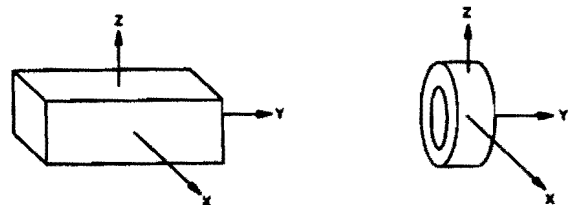
Figure 1-48. Y-cut block and doughnut-shaped crystals which can provide zero temperature coefficients for certain combination modes
