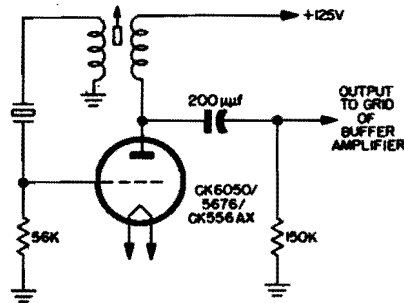
Figure 2-68. Schematic diagram of typical oscillator designed for use with Crystal Unit CR-55/U
