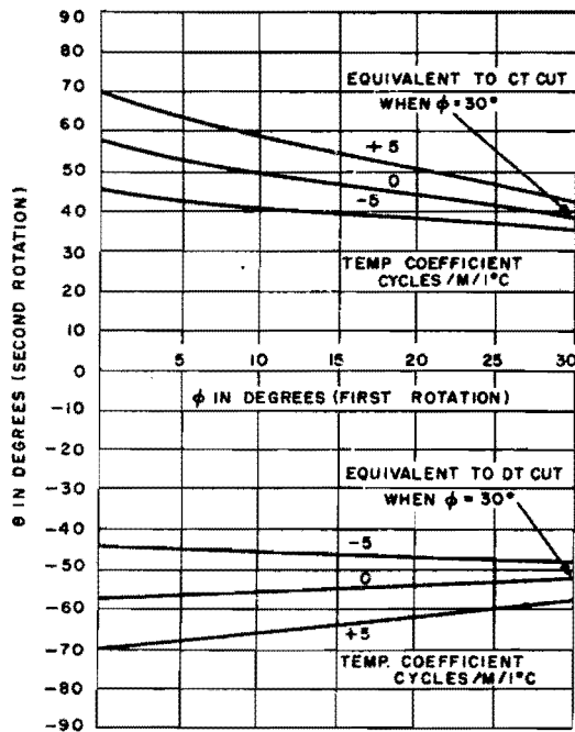
Figure 1-41. Relations of \theta to \phi , for face-shear mode of Y cut, which provide temperature coefficients of 0, +5, and -5 parts, per million per degree centigrade
