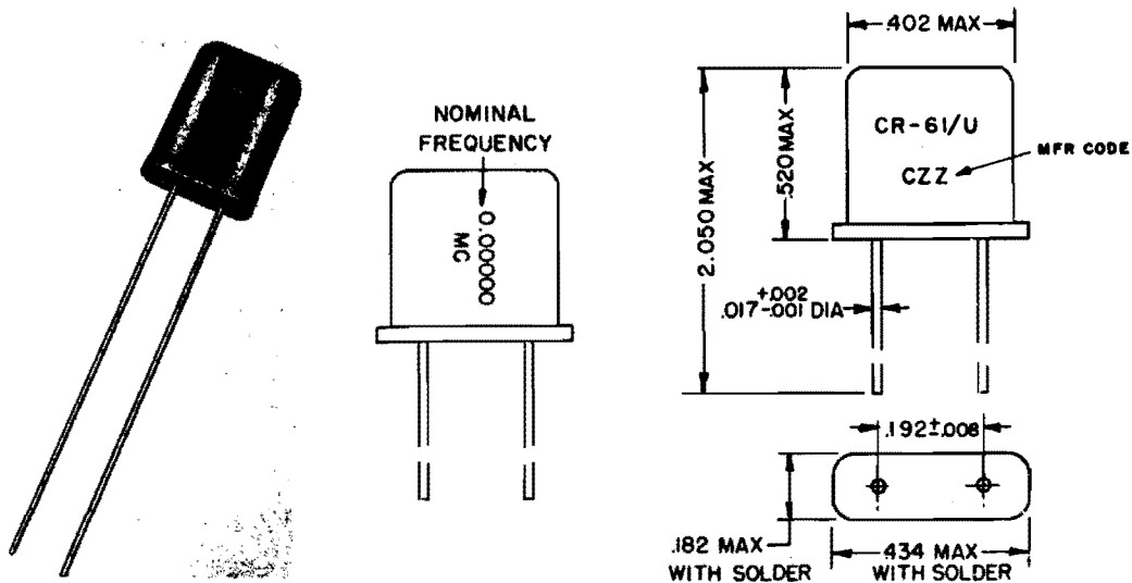
Figure 2-79. Crystal Unit CR-61/U
