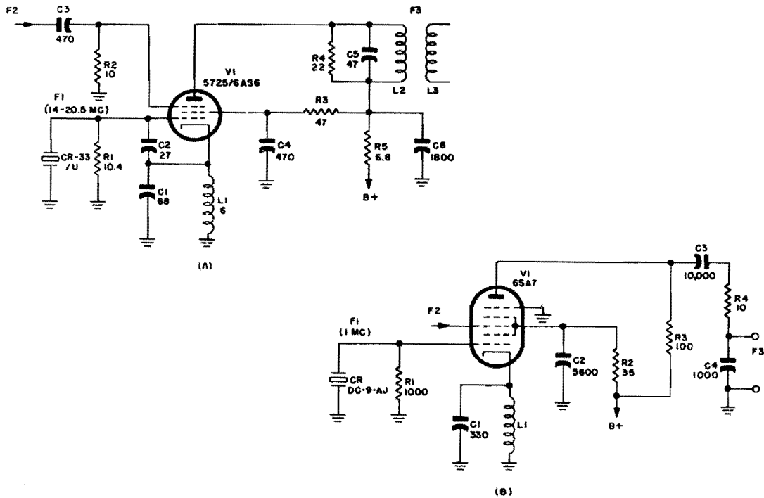
Figure 1-138. Electron-coupled Pierce oscillator modifications for heterodyne circuits
