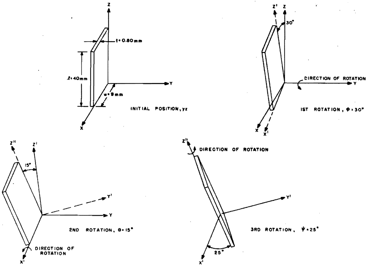
Figure 1-17 Orientation of crystal having the rotational specifications yzwtl : 30°/15°/25°
