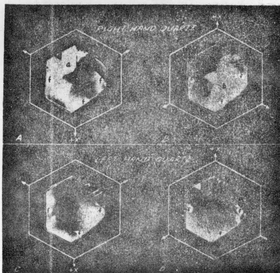
Figure 1-65. Reflection patterns of twinned Z section, showing both types of twinning. The section is predominantly right quartz, but is fairly evenly divided by the electrical twins a and b. The small regions of optical twinning of one electrical sense are shown in C, and those of the opposite sense are shown in D. The X-axis polarities indicated apply only to the respective bright regions. The regions marked f contain flaws *
