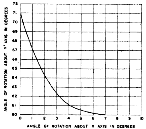
Figure 1-38. Angles of rotation for N element with a w/l ratio of 0.05 which will provide zero temperature coefficient at 25°C*
