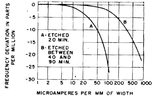
Figure 1-117. Frequency deviation versus crystal current density for two GT-cut crystals which were subjected to different periods of etching*
