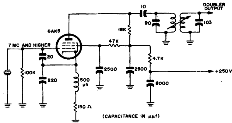
Figure 2-6. Schematic diagram of typical oscillator designed for use with Crystal Unit CR-18/U
