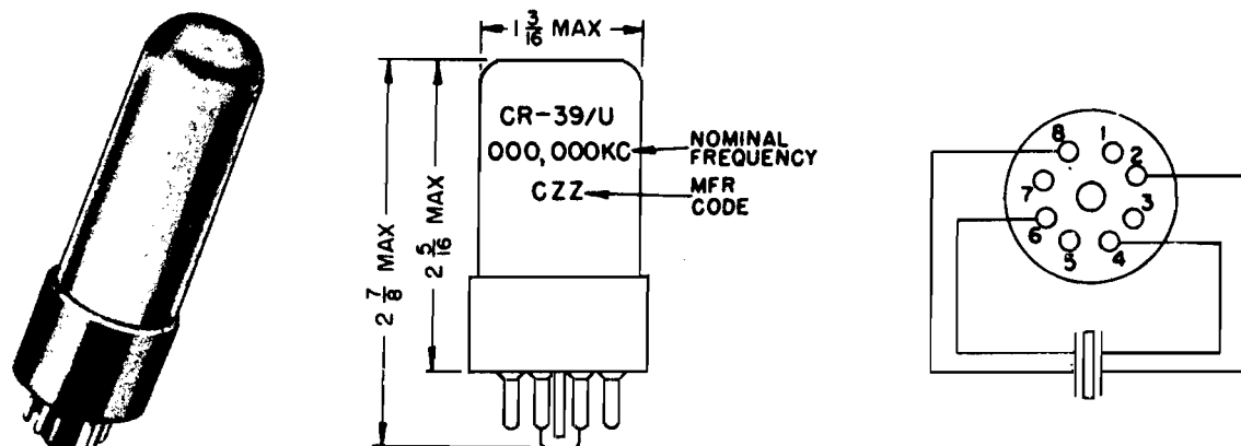
Figure 2-37. Crystal Unit CR-39/U
