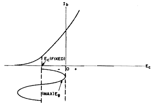
Figure 1-127. Point on E_c, I_b curve at which stable oscillations can be achieved with fixed bias. For minimum grid losses, the peak of the maximum excitation voltage must not exceed the fixed E_c .
