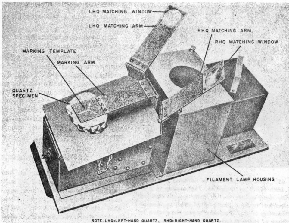
Figure 1-63. Pinhole oriascope with matching and marking arms for use on Z sections *
