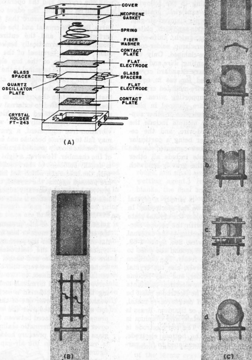
Figure 1-70. Methods, old and new, for mounting crystal units. (A) Construction of early model crystal unit employing the gravity air-gap type of mounting, now largely outmoded. The crystal holder shown is the type FT-243. (B) Solder-cone wire mount for v-l-f length-flexure crystal. (Courtesy HEEMCO). (C) Recently developed techniques for mounting shock-proof, 1-mc, A elements in the miniature HC-6/U metal holder to meet the specifications for 1-mc CR-18/U crystal units: a. Reeves-Hoffman flexible nylon mount. b. Hupp loose-slotted edge-clamped mount. c. Bliley molded nylon bumper mount. d. RCA edge-clamping spring mount. (Courtesy McCoy Electronics.)
