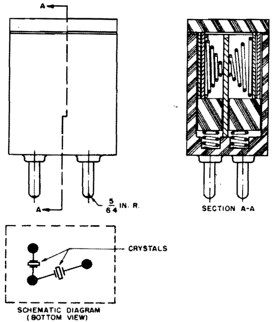
Figure 3-22. Crystal Holder FT-249
