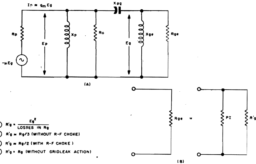
Figure 1-141. Equivalent circuit of Miller oscillator. R_p is assumed to be large compared with the total load impedance. R_o is an equivalent resistance accounting for the output losses. R_{\mu} is an equivalent resistance accounting for the crystal and grid losses; it is approximately equal to the resistance of the parallel circuit shown in (B). PI is the performance index of the crystal unit; R'_g is the equivalent grid resistance; and R_g is the actual gridleak resistance
