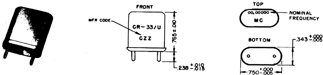
Figure 2-27. Crystal Unit CR-33/U
