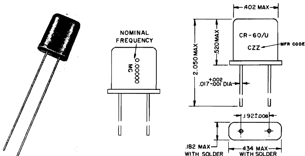
Figure 2-77. Crystal Unit CR-60/U
