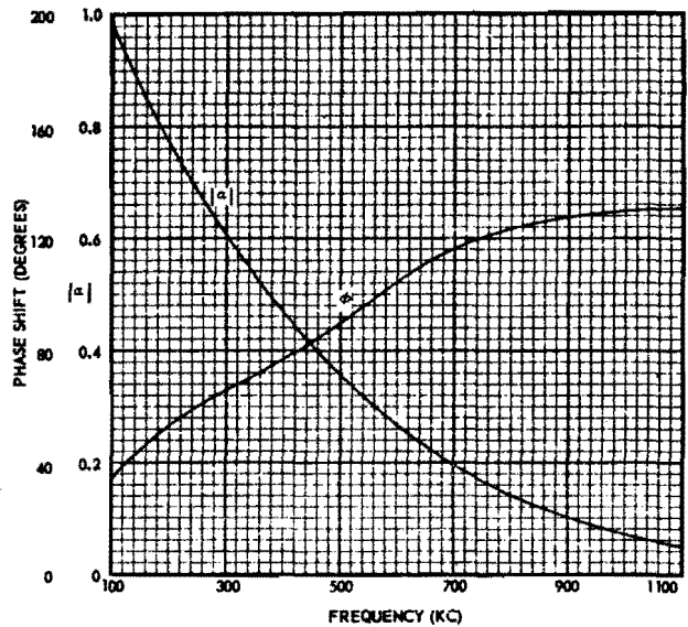
Figure 1-226. Typical alpha characteristics versus frequency of a type CK-720 junction transistor
