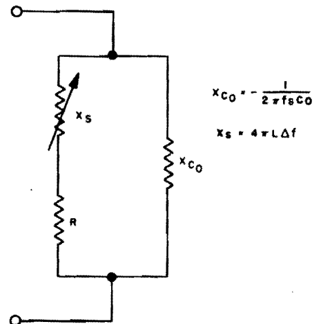
Figure 1-97. Impedance diagram of equivalent circuit of crystal unit
