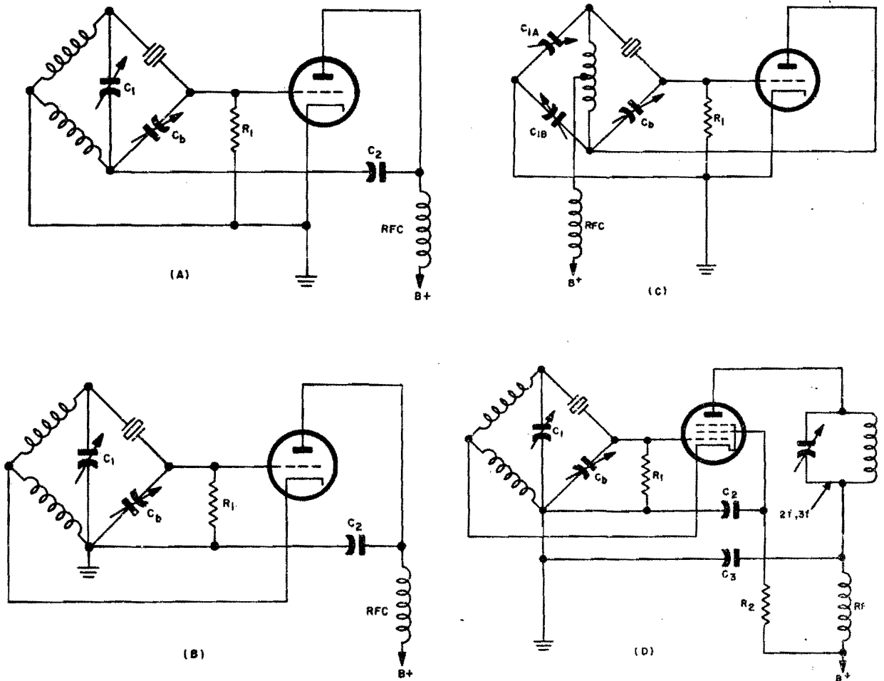
Figure 1-172. Miscellaneous capacitance-bridge oscillators
