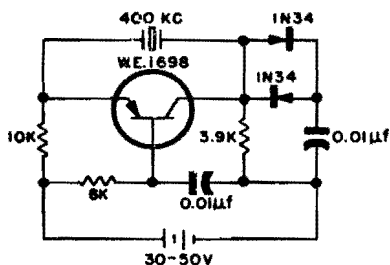
Figure 1-240. Modification of the crystal-feedback oscillator of figure 1-238 to provide greater frequency stability by providing greater amplitude stability with diode clipping
