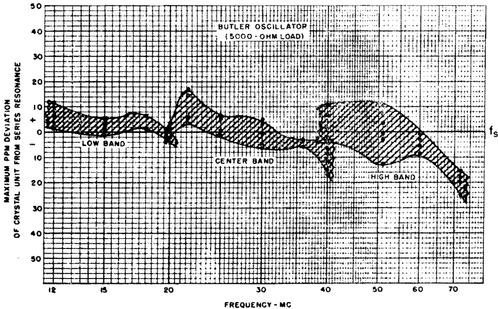
Figure 1-253. Typical frequency tolerances to be expected of crystal units connected in Butler circuit of Gruen packet series. The deviations plotted are deviations of the peak-output operating frequency from the series-resonance frequency of the individual crystal unit as measured with a CI meter, and are not deviations from the rated nominal frequency of the crystal unit. Thus, the overall tolerance to be expected of such an oscillator must be the total of the crystal unit nominal frequency tolerance plus the expected operating resonance tolerance, the latter being indicated by the measured deviation above
