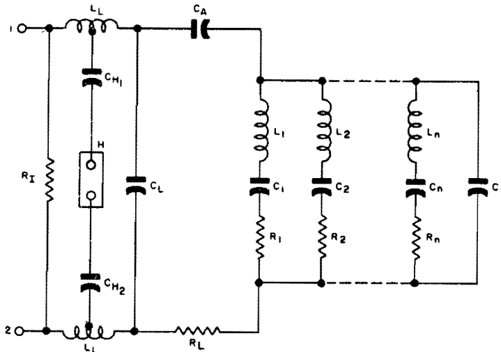
Figure 1-90. Equivalent circuit of crystal unit
