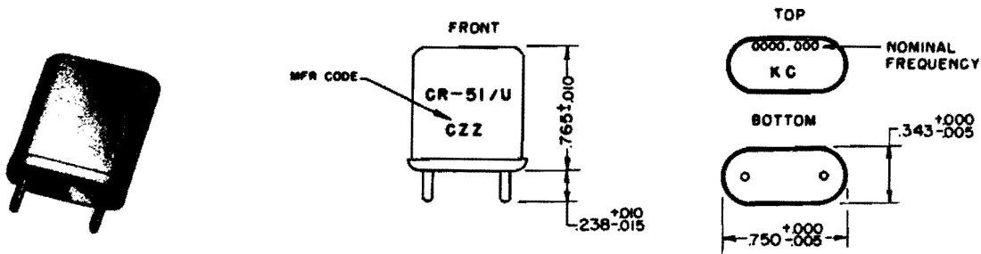
Figure 2-59. Crystal Unit CR-51/U
