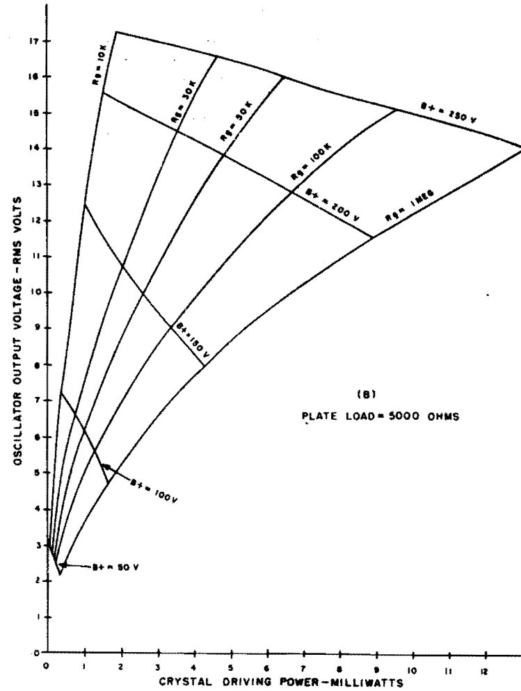
Figure 1-145. Output voltage versus crystal power for various values of gridleak resistance as the d-c plate voltage is varied in experimental Miller oscillator. The circuit is tuned for output voltages 50 percent of the maximum possible by variations in plate tank alone. Frequency = 7 mc; plate tank L/C = 0.04; and PI of CR-18/U crystal unit (with load capacitance of 32 \mu\text{f} ) = 49 kilohms
