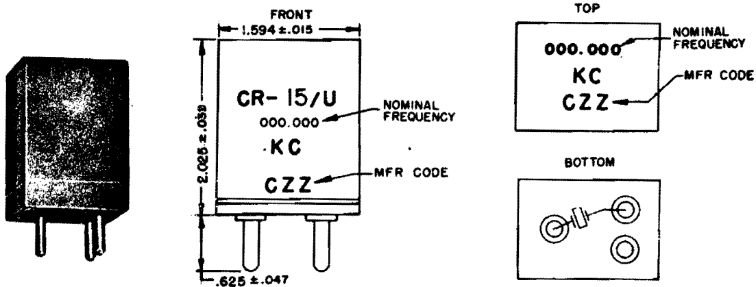
Figure 2-1. Crystal Unit CR-15/U
