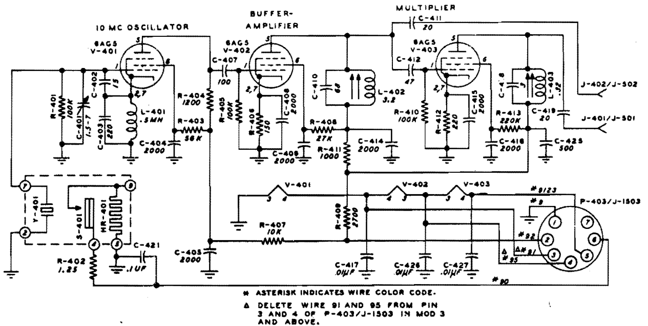
Figure 1-214. 10-mc spectrum oscillator, V401, buffer amplifier, V402, and 90-mc multiplier, V403, of Receiver-Transmitter RT-178/ARC-27. See figure 1-212 for function of the above circuits in the spectrum generator system
