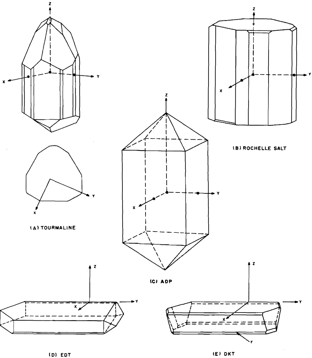
Figure 1-2. Commercially used piezoelectric crystals other than quartz
