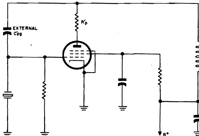
Figure 1-142. The large resistance, R_p' , connected in plate circuit effectively increases R_p of the tube. This method can be used to improve the frequency stability of a Miller oscillator employing a screen-grid tube and an externally connected feed-back capacitance, C_{pg}'
