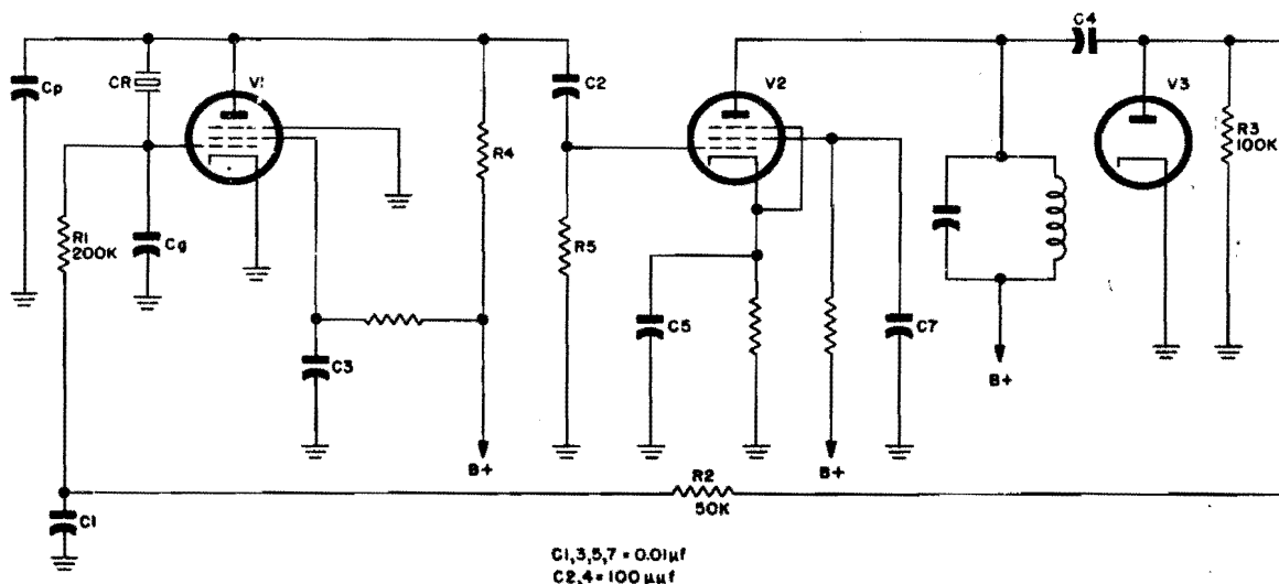
Figure 1-131. Pierce oscillator with automatic gain control
