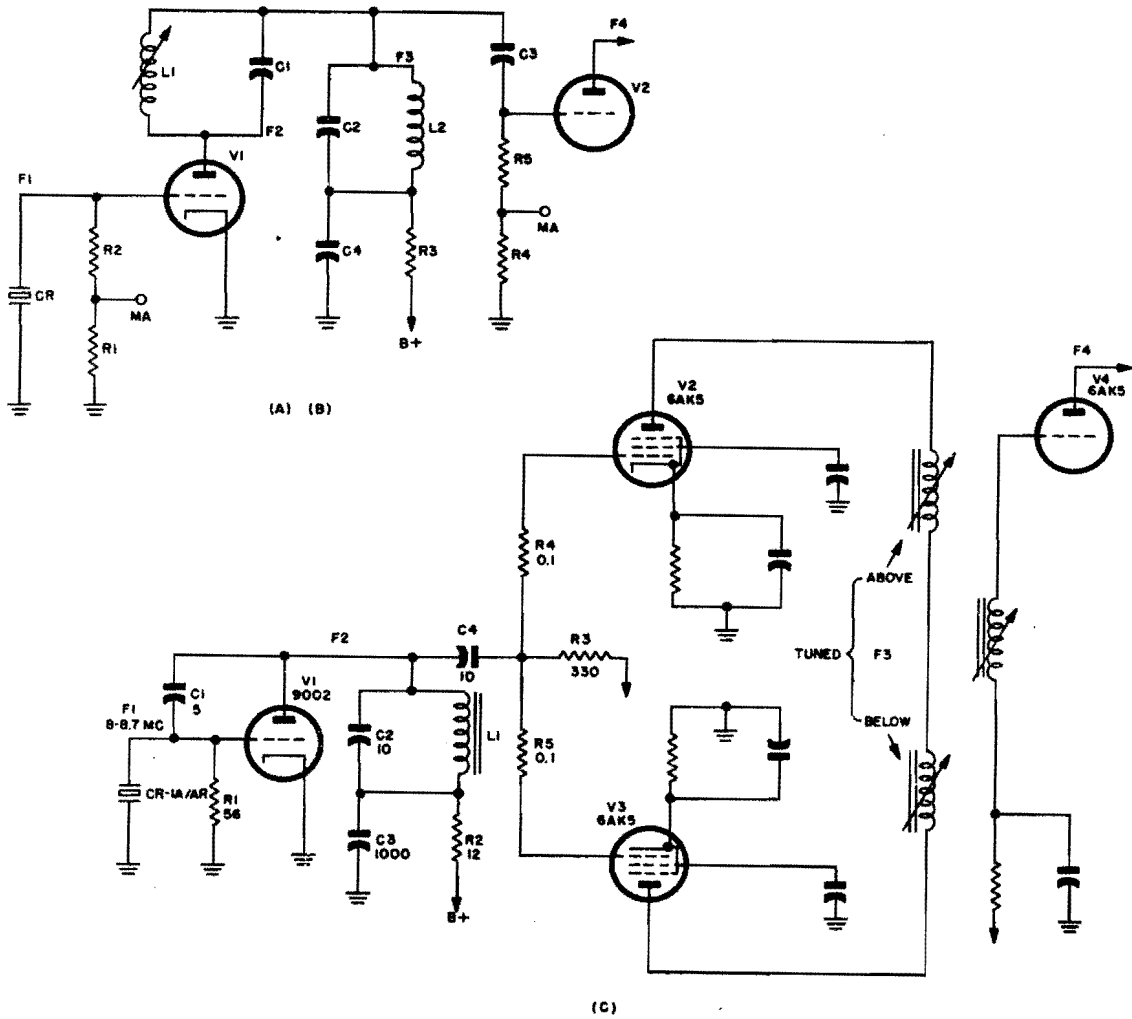
Figure 1-150. Modified Miller oscillators using triodes
