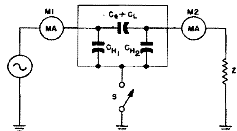
Figure 1-93. Circuit diagram indicating the effect that grounding a metal holder may have on shunt capacitance
