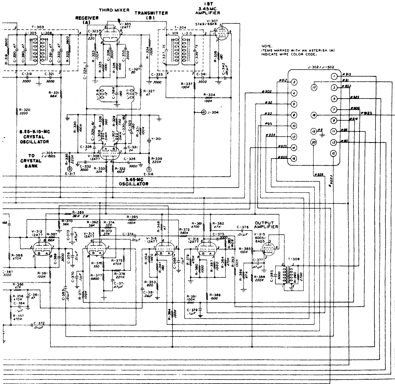
Figure 1-217. Fixed i-f amplifier subassembly, Receiver-Transmitter RT-178/ARC-27. See figure 1-210 for function of receiver circuits V301, V303, V305A, V306A, and V307. (V308 and V309, the 2nd and 3rd 3.45-mc amplifiers, which are similar in design to the V307 stage, are not shown. Also omitted are the vacuum-tube heater circuits.) See figure 1-211 for function of transmitter circuits V302, V304, V305B, V306A, and V306B
