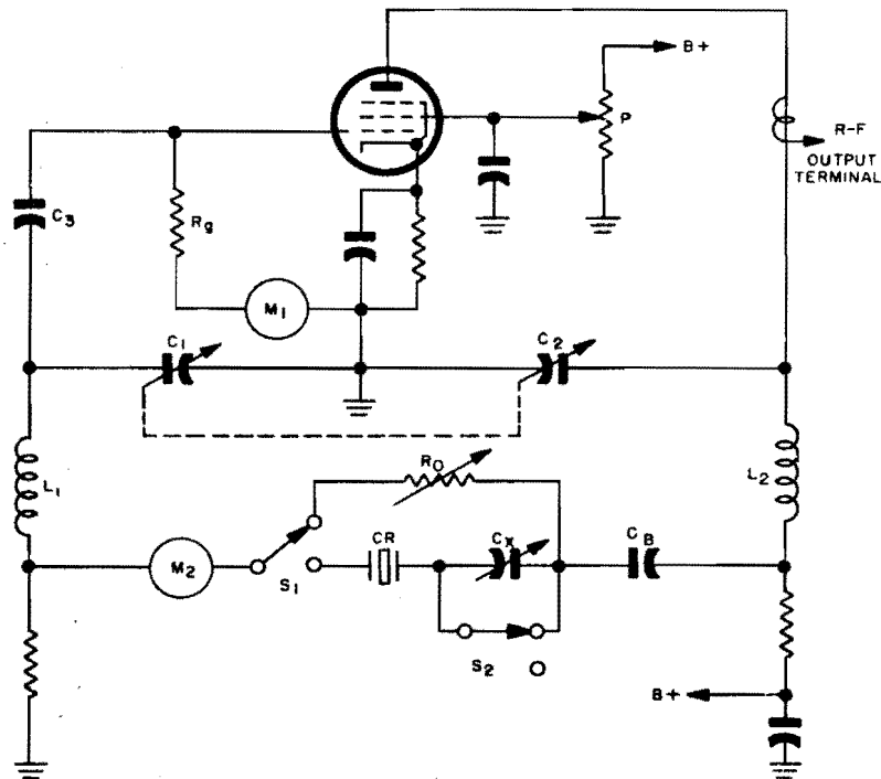
Figure 1-106. Simplified schematic diagram of CI meter
