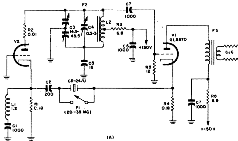
Figure 1-175. Modifications of Butler oscillator. Dotted lines in circuit (G) indicate stray capacitances
