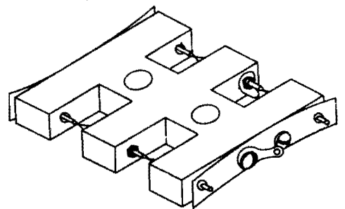
Figure 1-80. Pressure-pin mounting, with provisions for supporting four plated filter crystals *
