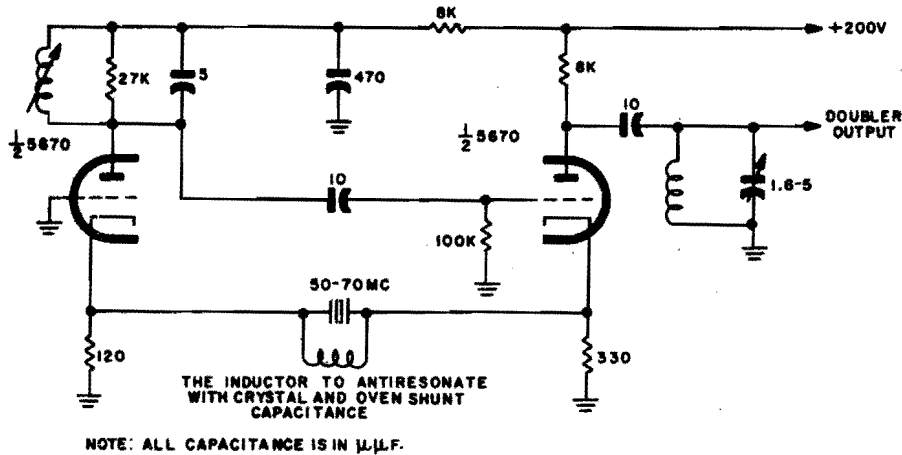
Figure 2-76. Schematic diagram of typical oscillator designed for use with Crystal Unit CR-59/U
