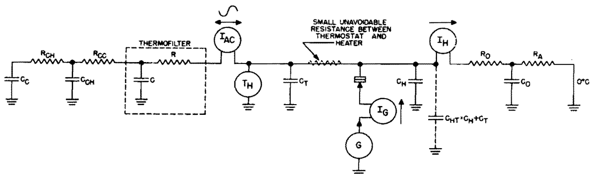
Figure 4-16. Oven thermal A-C circuit
