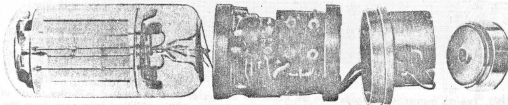
Figure 1-254. Small, portable, packaged transistor crystal oscillator developed by P. G. Sulzer of National Bureau of Standards. Unit is provided with mercury-cell power supply shown at right. Metal container is not shown
