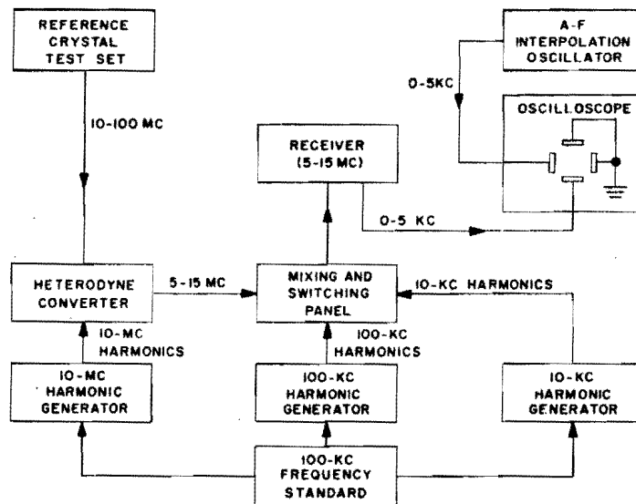
Figure 2-91. System, employing a heterodyne converter, for measuring h-f and v-h-f crystal frequencies visually with an oscilloscope and a-f interpolation oscillator
