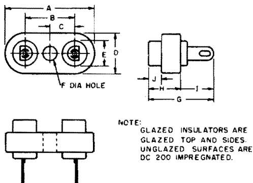
Figure 3-15. Crystal socket for use with HC-6/U, HC-13/U, and HC-14/U holders
