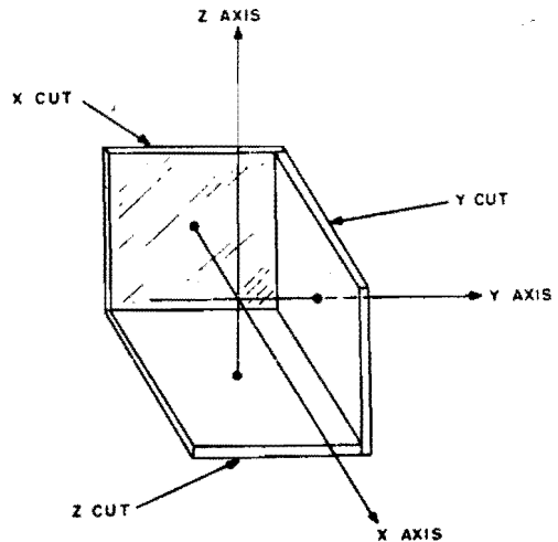
Figure 1-18 Orientation of X, Y, and Z cut plates
