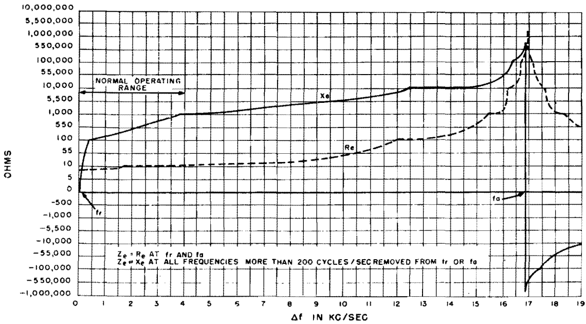
Figure 1-104. Typical characteristic curves for X_e and R_e of 10-mc crystal unit. (Shunt resistance, R_s , across crystal is assumed to be negligible)
