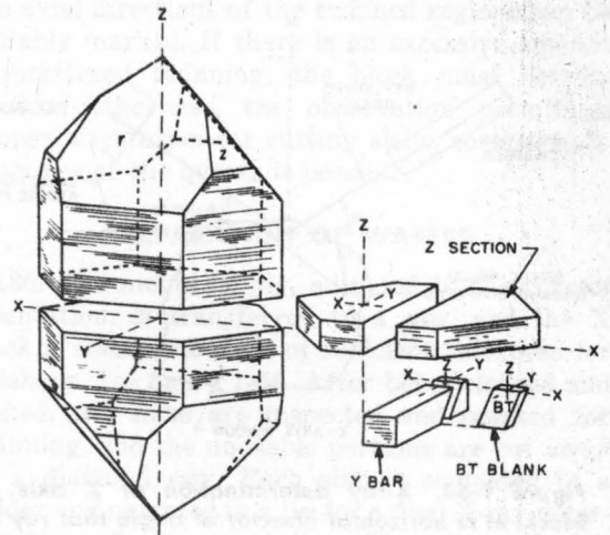
Figure 1-62. Z-section-Y-bar method of cutting properly oriented crystal blanks
