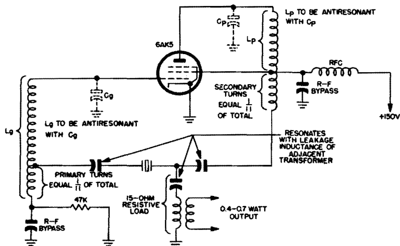
Figure 2-64. Schematic diagram of typical oscillator designed for use with Crystal Unit CR-53/U
