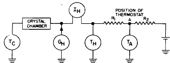
Figure 4-15. Thermal D-C path of heater-to-thermostat when thermostat is outside heater
