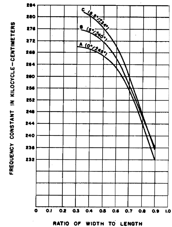
Figure 1-33. Frequency constant versus w/l ratio for M elements having low temperature coefficients. C is the curve of the most commonly used MT orientation *
