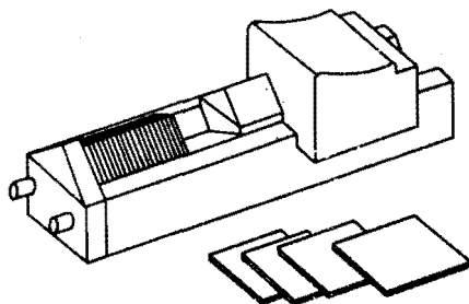
Figure 1-68. Loaf of crystal dice, all blanks oriented in the same direction in preparation for edge grinding by edging machine *
