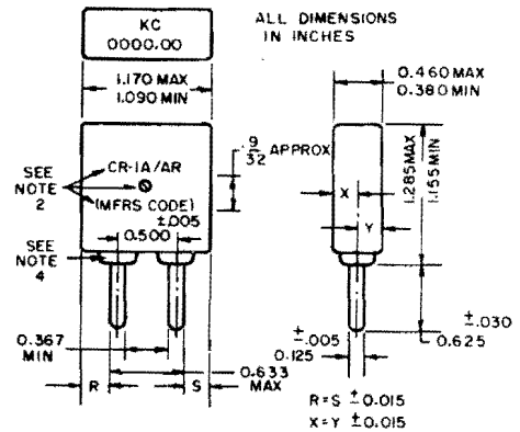
Figure 3-23. Crystal Holder for Crystal Unit CR-1A/AR
