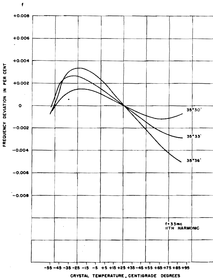
Figure 1-113. Large clockwise angle of rotation of frequency-temperature curve of harmonic-mode A element caused by small increments (3 minutes of arc) in the cutting orientation angle about the X axis
