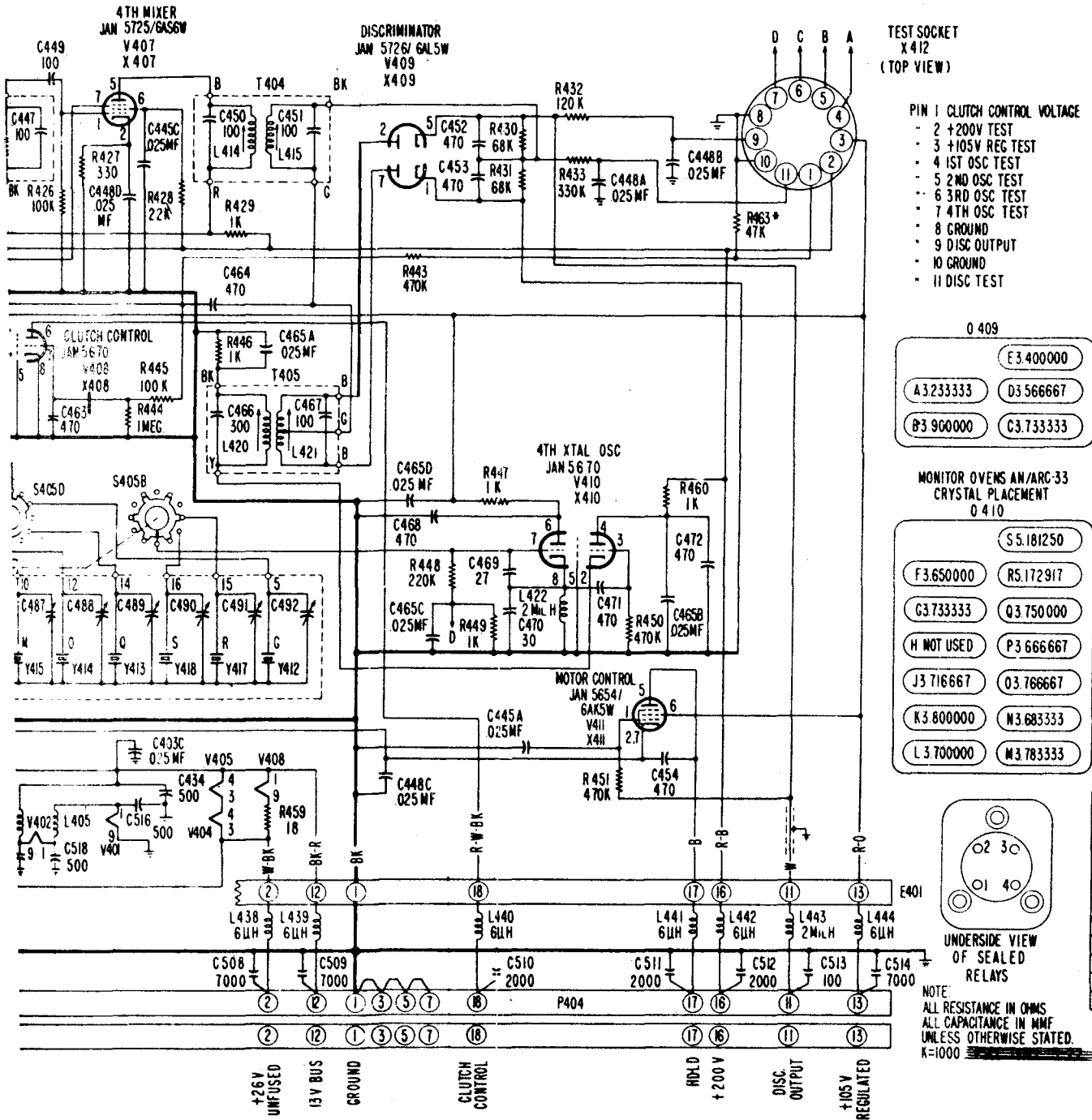
Figure 1-196. Monitor chassis. Schematic diagram of a-f-c system in Radio Set AN/ARC-33
