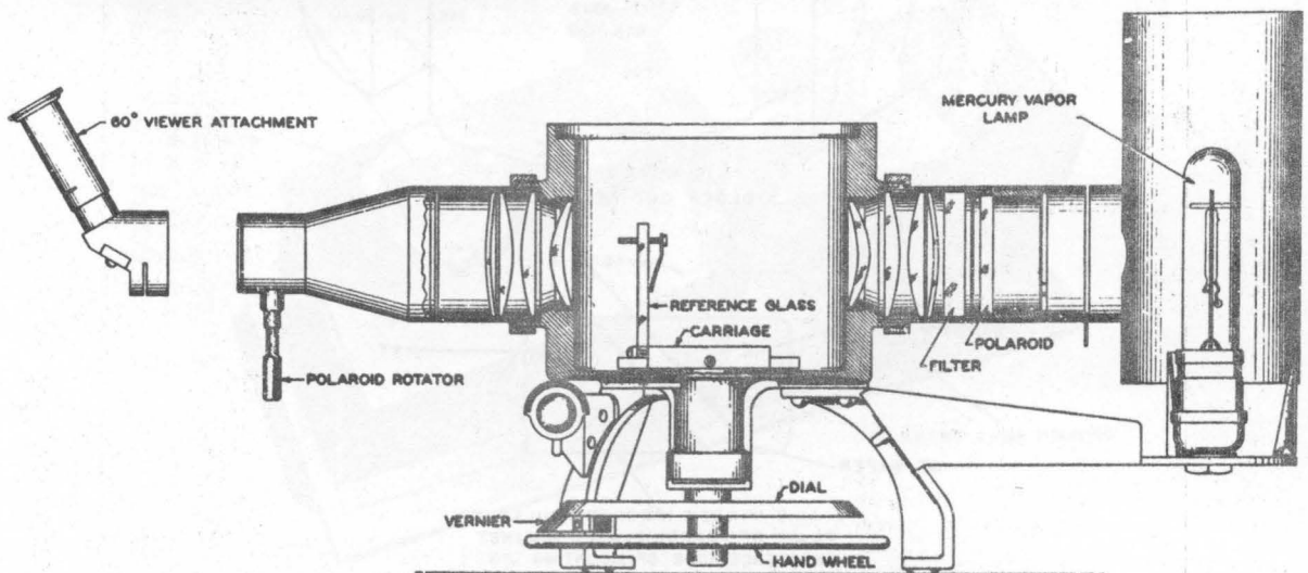
Figure 1-59. Conoscope. Used for locating accurately the optic axis and for determining the handedness of quartz stones *
