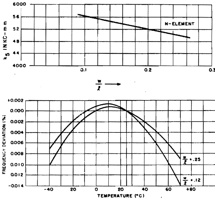
Figure 1-37. Frequency-temperature characteristics of element N. The larger w/l ratio is typical of 100-kc elements, and the smaller w/l ratio is typical of 16-kc elements
