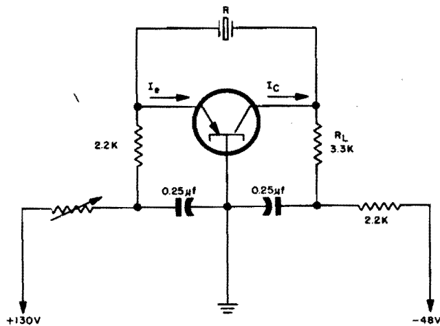
Figure 1-222. Basic circuit for crystal-controlled transistor oscillator
