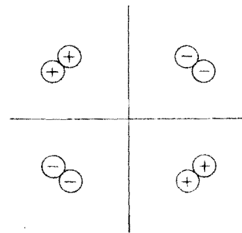
Figure 1-8. Example of distribution of charges having a center of symmetry *
