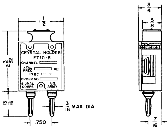
Figure 3-19. Crystal Holder FT-171-B
