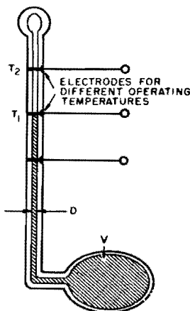
Figure 4-7. Diagram of typical mercury thermostat
