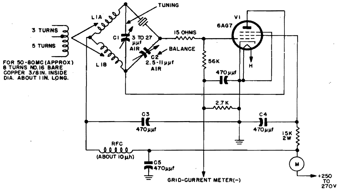
Figure 1-169. A capacitance-bridge oscillator for higher power output which is practical for operation in the 50-80-mc frequency range. Resistors not otherwise specified are 1/2 w. All fixed capacitors have mica dielectrics
