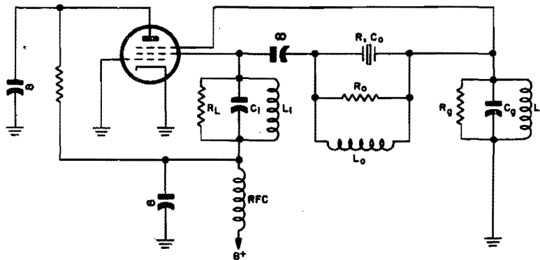
Figure 1-181. Transistron crystal oscillator
