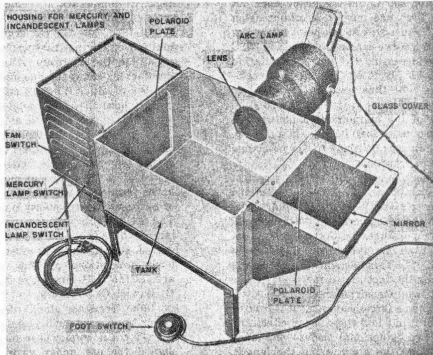
Figure 1-57. Polariscope-inspectoscope. Used for examining raw quartz
