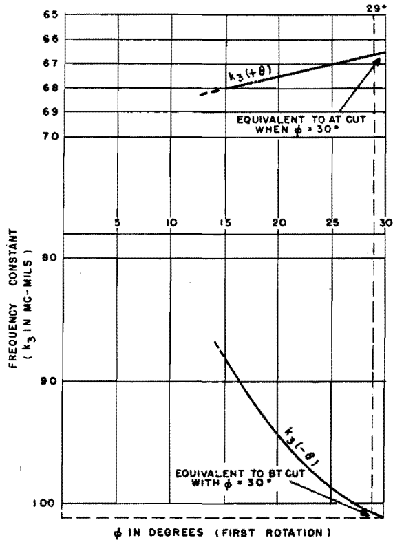
Figure 1-39. Frequency constant versus \phi (angle of rotation about Z axis) for the thickness-shear mode of V-cut crystals when \theta , the second angle of rotation, is so chosen that a zero temperature coefficient is obtained. The upper and lower curves are for positive and negative values of \theta , respectively
