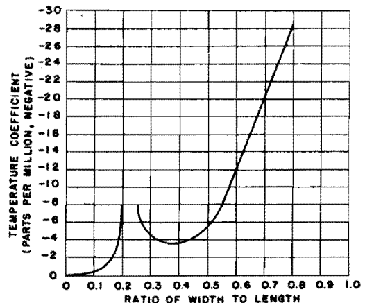
Figure 1-25. Temperature coefficient versus w/l ratio for element E at temperatures between 45° and 55°C *
