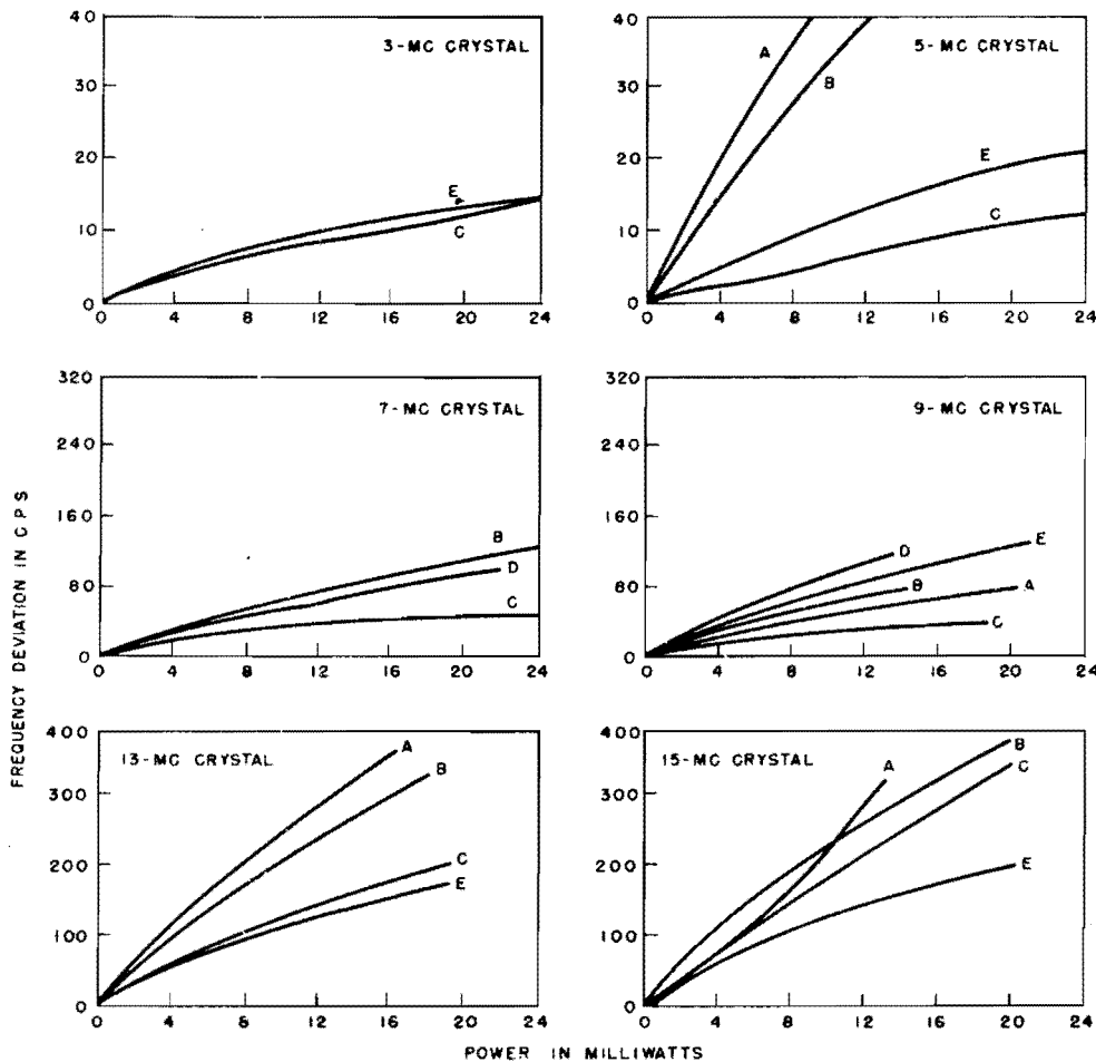
Figure 1-118. Average frequency deviation versus drive. Each curve represents the average of a random sample of several similarly constructed units of one manufacturer. Curves having the same letter represent the characteristics of crystal units of the same manufacturer
