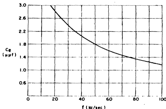
Figure 1-94. C_e versus frequency for typical wire-mounted N elements
