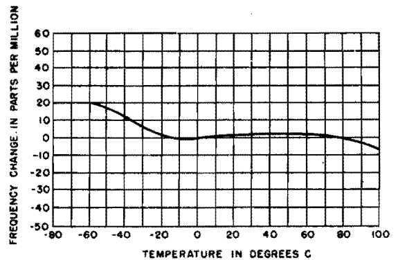
Figure 1-55. Temperature-frequency characteristics of element G *
