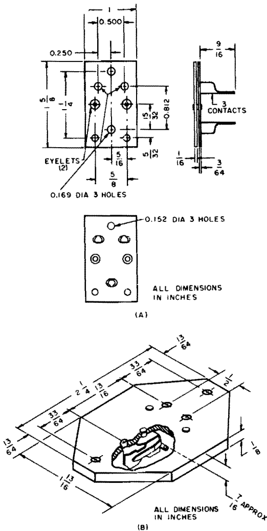
Figure 3-14. Crystal sockets for use with HC-5/U holder
