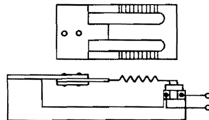
Figure 4-5. E-shaped, bimetallic, snap thermostat
