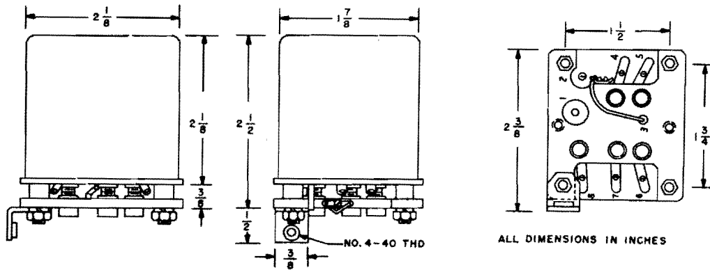
Figure 4-21. Dimensions of Bendix Radio Crystal Oven L205628
