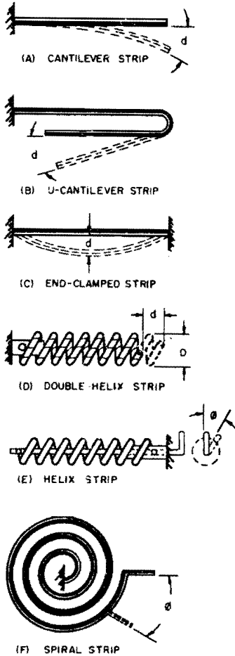
Figure 4-4. Basic types of bimetallic strips
