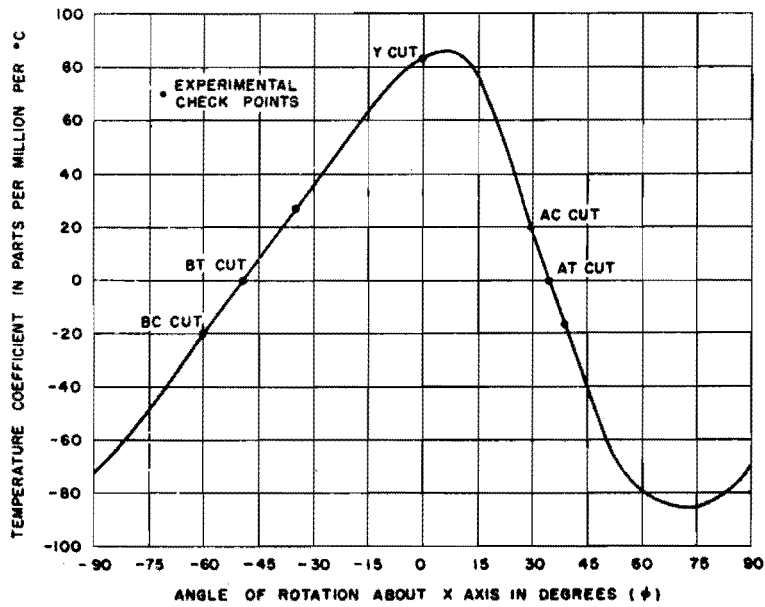
Figure 1-44. Temperature coefficient versus angle of rotation about X axis for thickness-shear elements of Y group *
