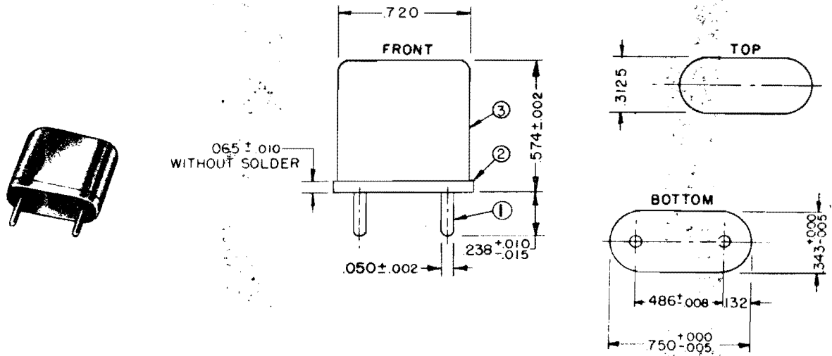
Figure 3-5. Crystal Holder HC-14/U
