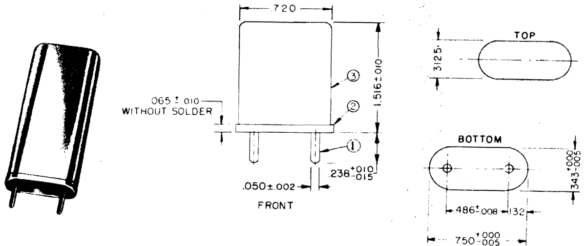
Figure 3-4. Crystal Holder HC-13/U
