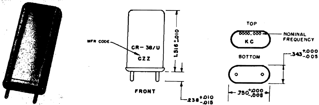
Figure 2-35. Crystal Unit CR-38/U
