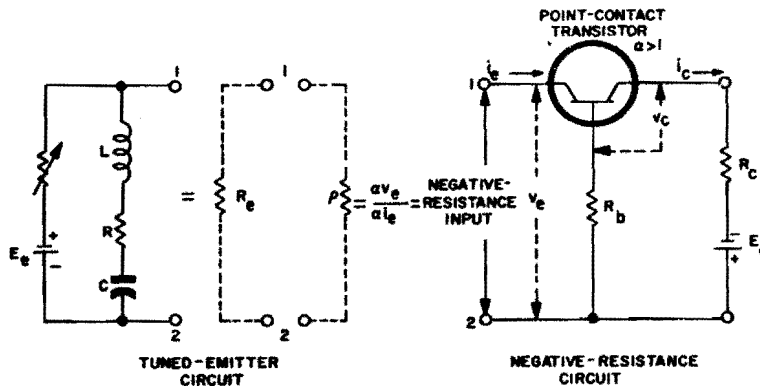
Figure 1-228. Tuned-emitter negative-resistance circuit. Essential features are that alpha be greater than unity, the insertion of an external resistance, R_b , in the common-base circuit to increase the collector-to-emitter energy feedback; and for oscillations to build up, the effective positive resistance, R_e , of the tuned-emitter circuit must be less, numerically, than the negative resistance, at the emitter input
