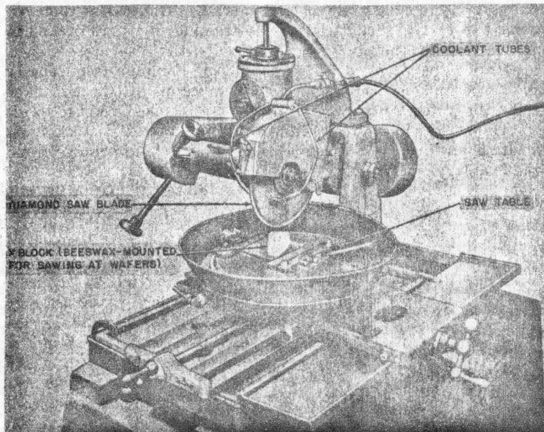
Figure 1-66. Diamond saw for cutting wafers from X block
