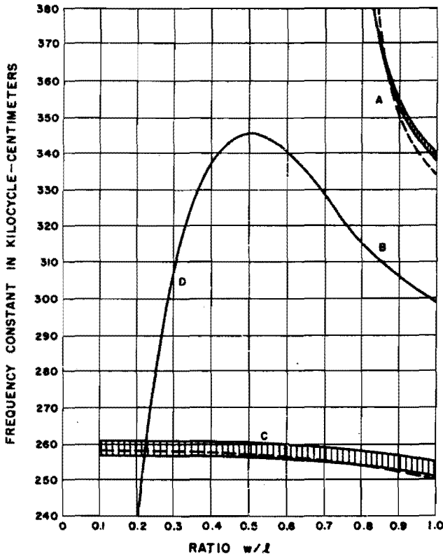
Figure 1-32. Frequency constant versus w/l ratio for various resonances of -18^\circ X-cut crystal. A is the width-extensional mode. B is the face-shear mode, which, at small w/l ratios, is strongly coupled to D, the second flexural mode. C represents the band between the antiresonant (upper curve) and the resonant (lower curve) frequencies of the length-extensional mode of element F. Note the weak coupling between C and D-B *
